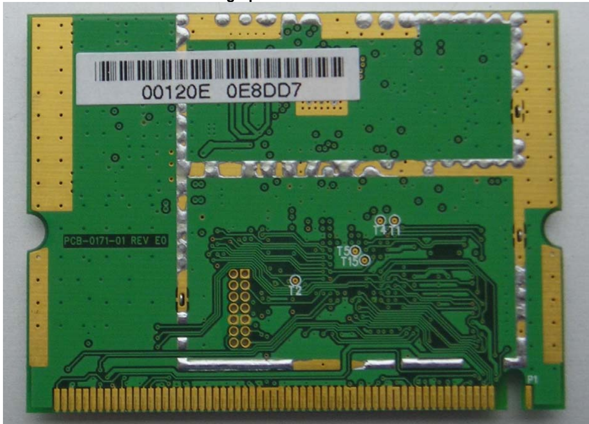
Photograph of RF PCB Foil Side
