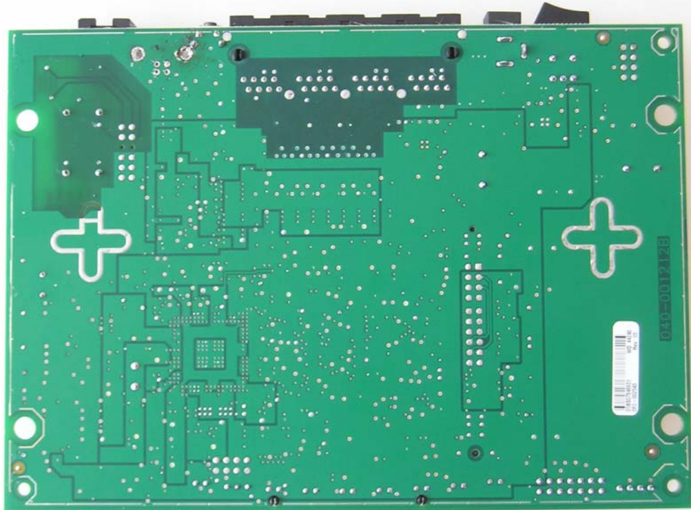
Photograph of Main board Foil Side
