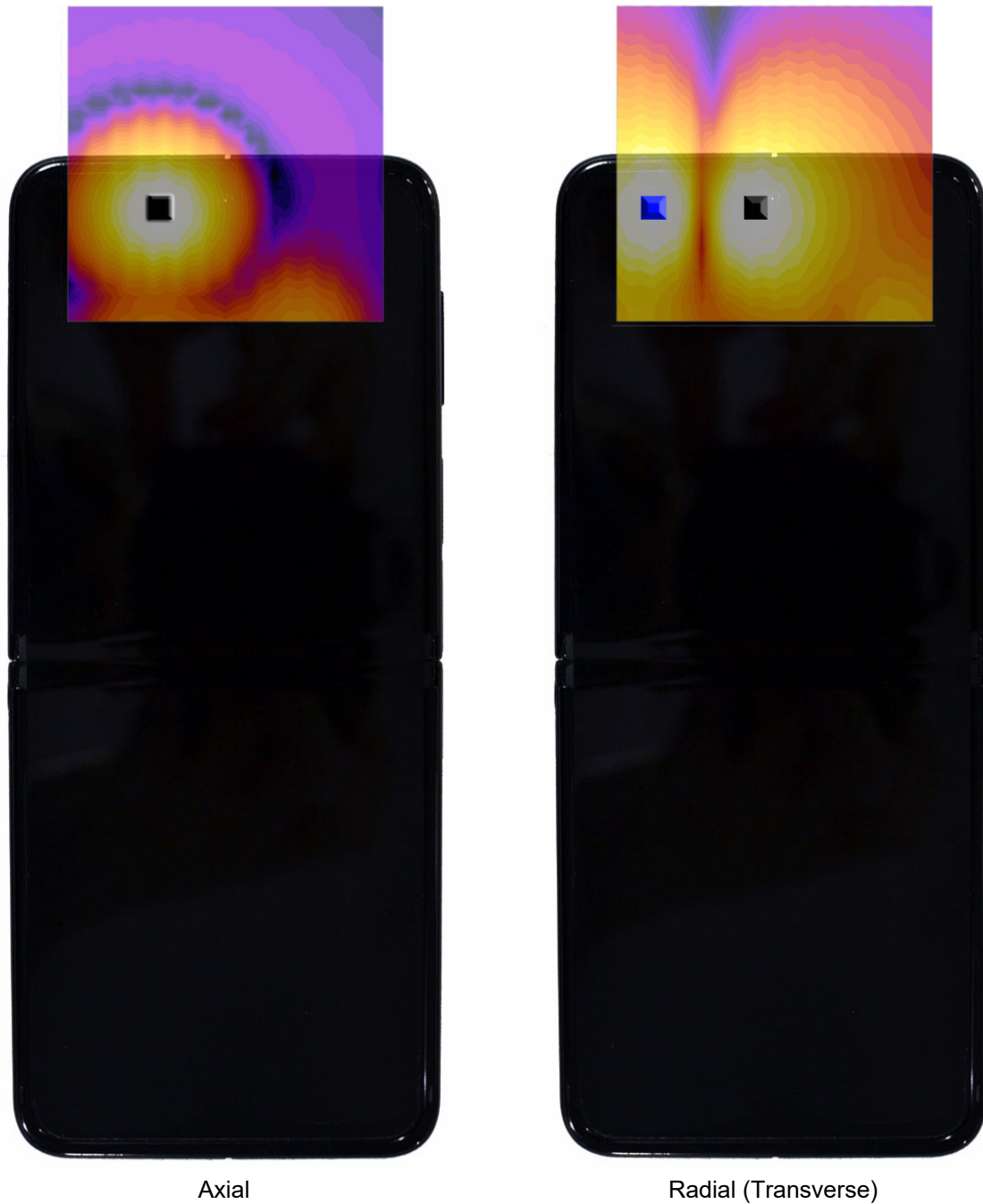
Figure 16-3 T-Coil Scan Overlay Magnetic Field Distributions
