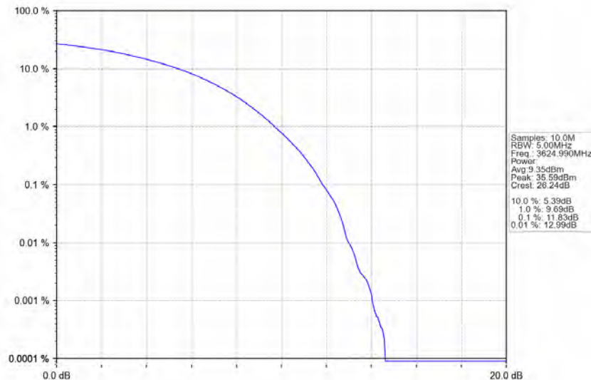
n78d_30kHz_MIMO_NTNV_50MHz_CP-OFDM QPSK_3624.99MHz_Outer_Full
