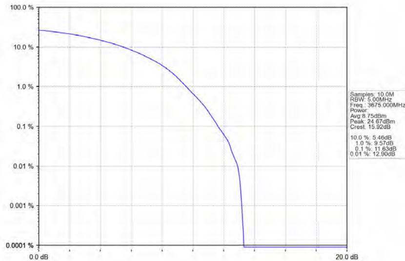
n78d_30kHz_MIMO_NTNV_50MHz_CP-OFDM_16_QAM_3675MHz_Outer_Full
