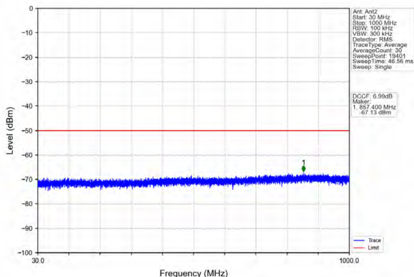
n78d_30kHz_MIMO_NTNV_10MHz_CP-OFDM_QPSK_3555MHz_Outer_Full
