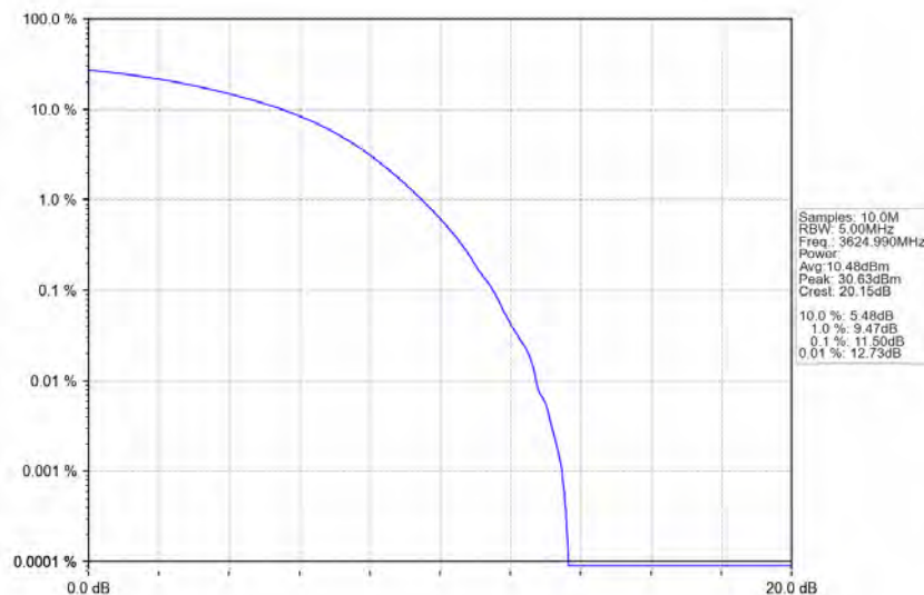
n78d_30kHz_MIMO_NTNV_40MHz_CP-OFDM_16_QAM_3624.99MHz_Outer_Full
