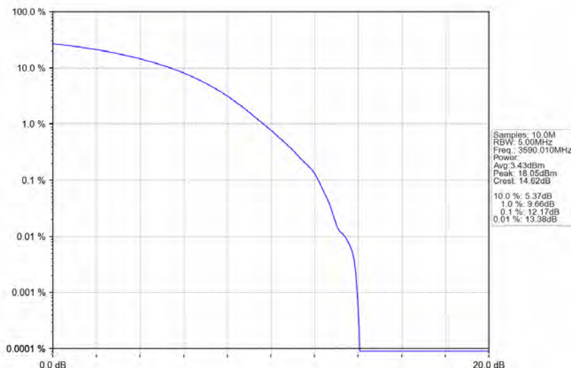
n78d_30kHz_MIMO_NTNV_80MHz_CP-OFDM_256_QAM_3590.01MHz_Outer_Full
