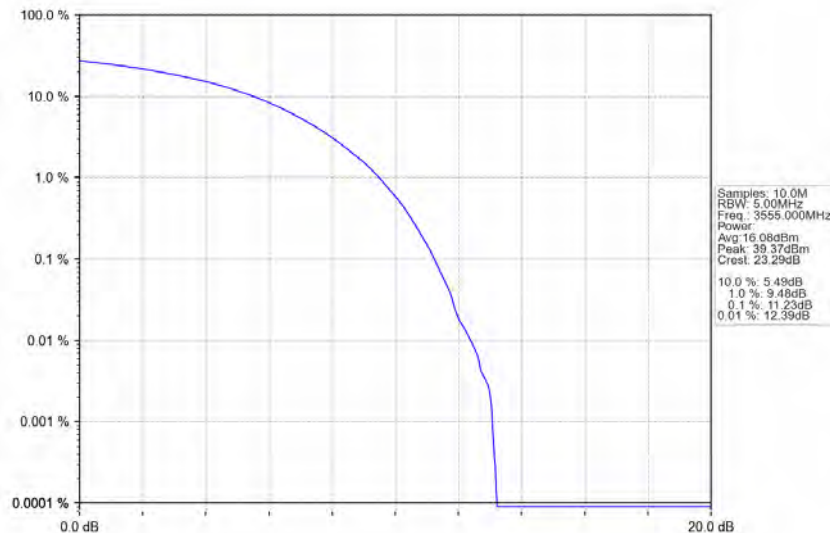
n78d_30kHz_MIMO_NTNV_10MHz_CP-OFDM_16_QAM_3555MHz_Outer_Full
