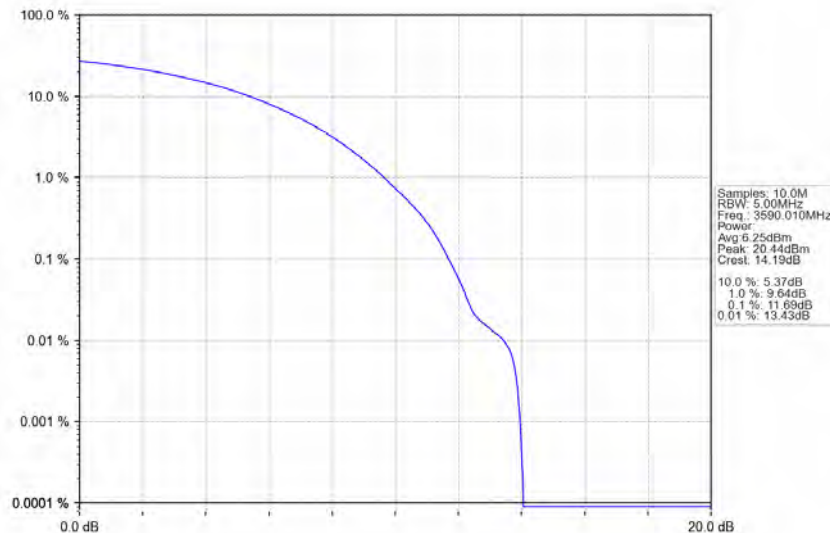
n78d_30kHz_MIMO_NTNV_80MHz_CP-OFDM_64_QAM_3590.01MHz_Outer_Full
