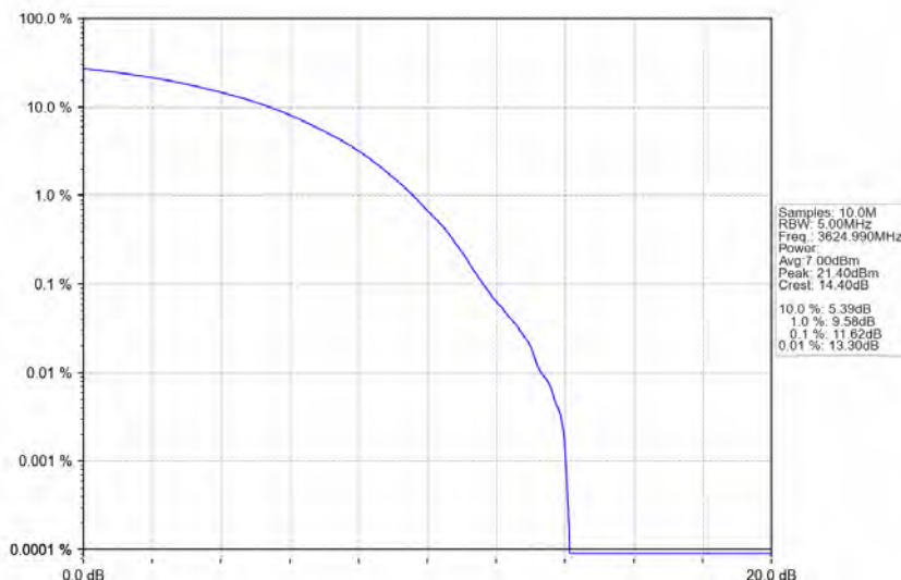
n78d_30kHz_MIMO_NTNV_80MHz_CP-OFDM_16_QAM_3624.99MHz_Outer_Full
