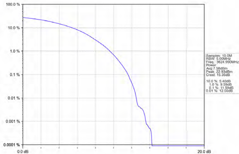
n78d_30kHz_MIMO_NTNV_70MHz_CP-OFDM QPSK_3624.99MHz_Outer_Full
