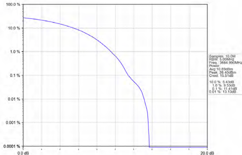
n78d_30kHz_MIMO_NTNV_30MHz_CP-OFDM_64_QAM_3684.99MHz_Outer_Full
