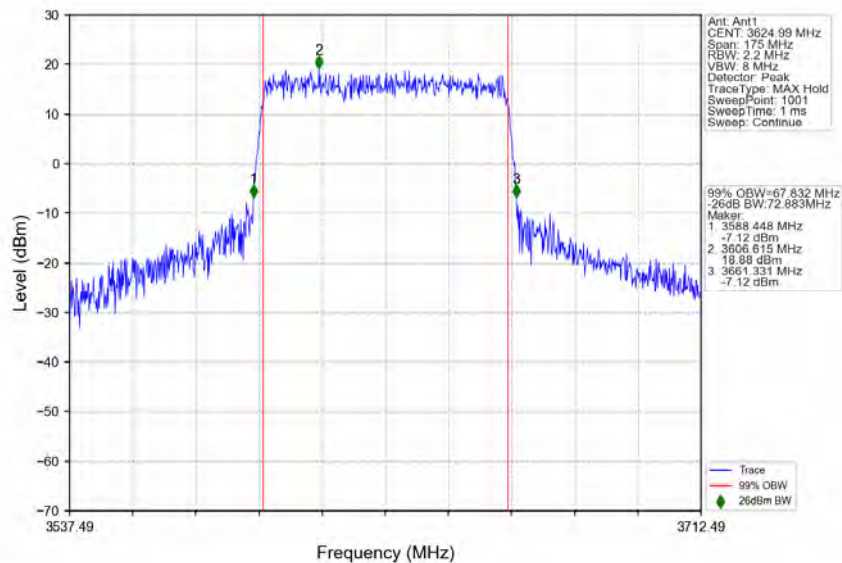
n78d_30kHz_MIMO_NTNV_70MHz_CP-OFDM_16_QAM_3624.99MHz_Outer_Full
