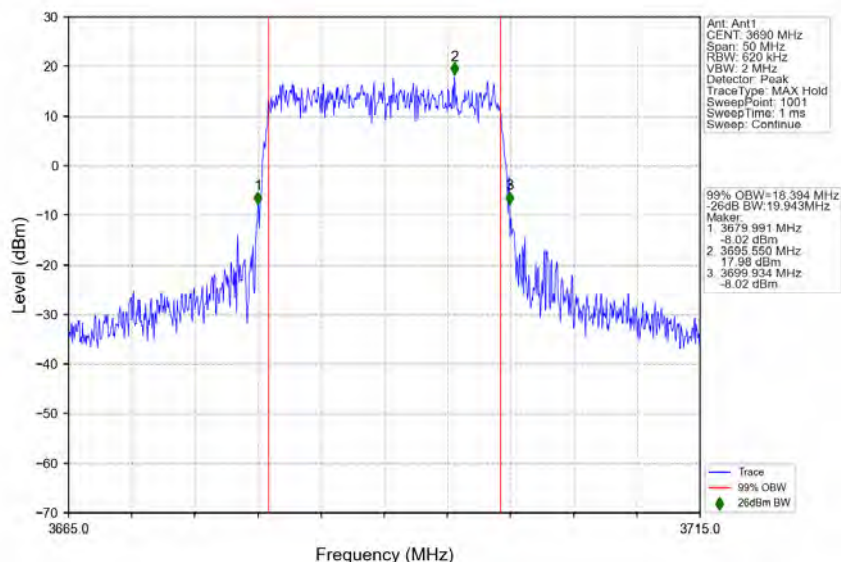
n78d_30kHz_MIMO_NTNV_20MHz_CP-OFDM_64_QAM_3690MHz_Outer_Full
