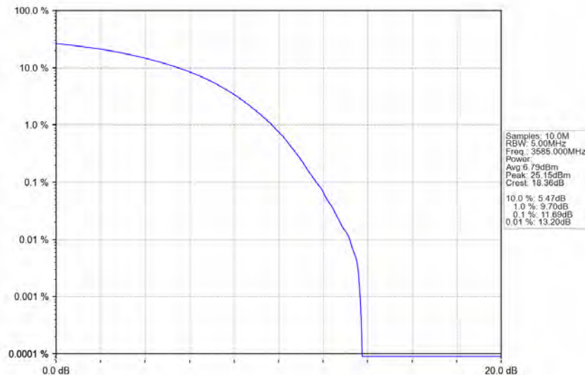
n78d_30kHz_MIMO_NTNV_70MHz_CP-OFDM_64_QAM_3585MHz_Outer_Full
