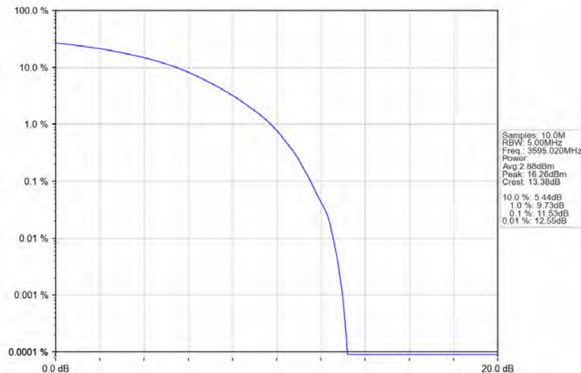
n78d_30kHz_MIMO_NTNV_90MHz_CP-OFDM_256_QAM_3595.02MHz_Outer_Full
