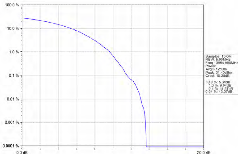
n78d_30kHz_MIMO_NTNV_90MHz_CP-OFDM_16_QAM_3654.99MHz_Outer_Full
