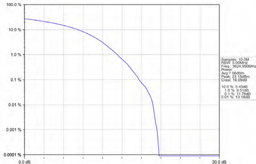
n78d_30kHz_MIMO_NTNV_40MHz_CP-OFDM_256_QAM_3624.99MHz_Outer_Full
