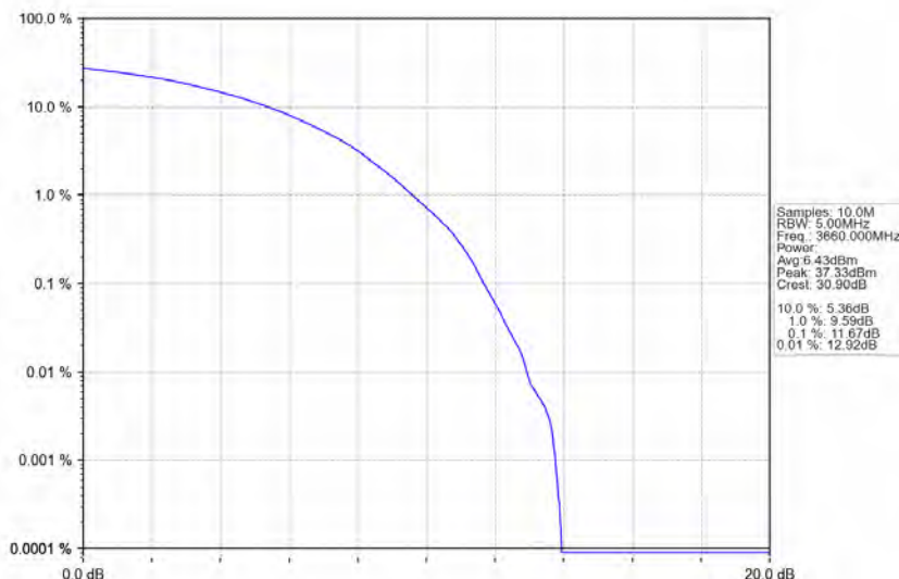
n78d_30kHz_MIMO_NTNV_80MHz_CP-OFDM QPSK_3660MHz_Outer_Full
