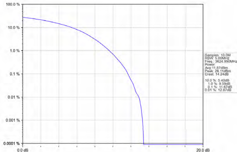
n78d_30kHz_MIMO_NTNV_30MHz_CP-OFDM_QPSK_3624.99MHz_Outer_Full
