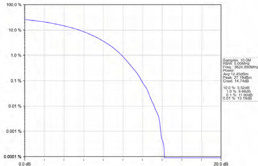
n78d_30kHz_MIMO_NTNV_10MHz_CP-OFDM_256_QAM_3624.99MHz_Outer_Full
