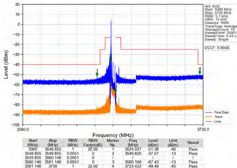
n78d_30kHz_MIMO_NTNV_10MHz_CP-OFDM_QPSK_3555MHz_Inner_1RB_Left
