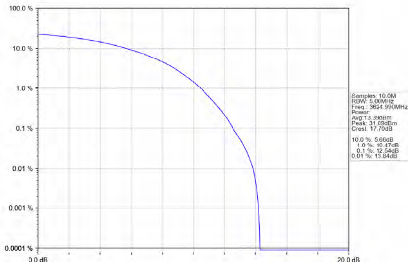
n78d_30kHz_MIMO_NTNV_20MHz_CP-OFDM QPSK_3624.99MHz_Outer_Full
