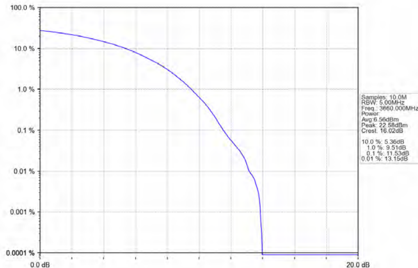
n78d_30kHz_MIMO_NTNV_80MHz_CP-OFDM_16_QAM_3660MHz_Outer_Full
