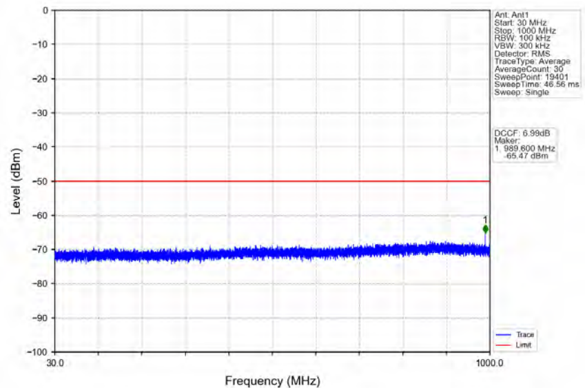
n78d_30kHz_MIMO_NTNV_10MHz_CP-OFDM_QPSK_3555MHz_Edge_1RB_Left
