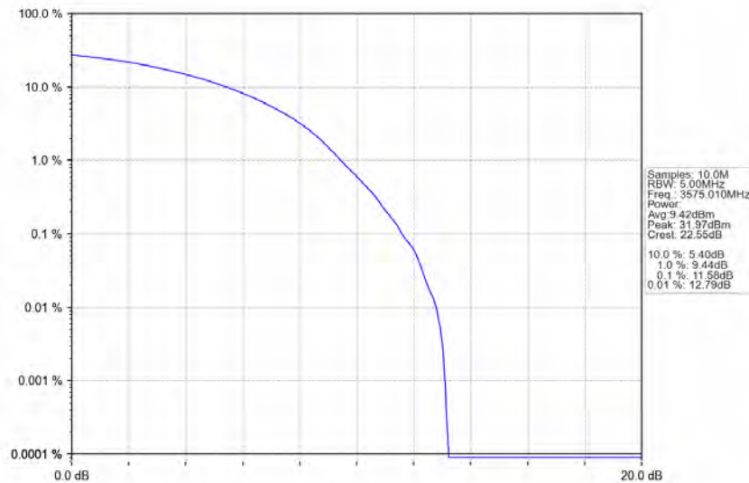
n78d_30kHz_MIMO_NTNV_50MHz_CP-OFDM_16_QAM_3575.01MHz_Outer_Full
