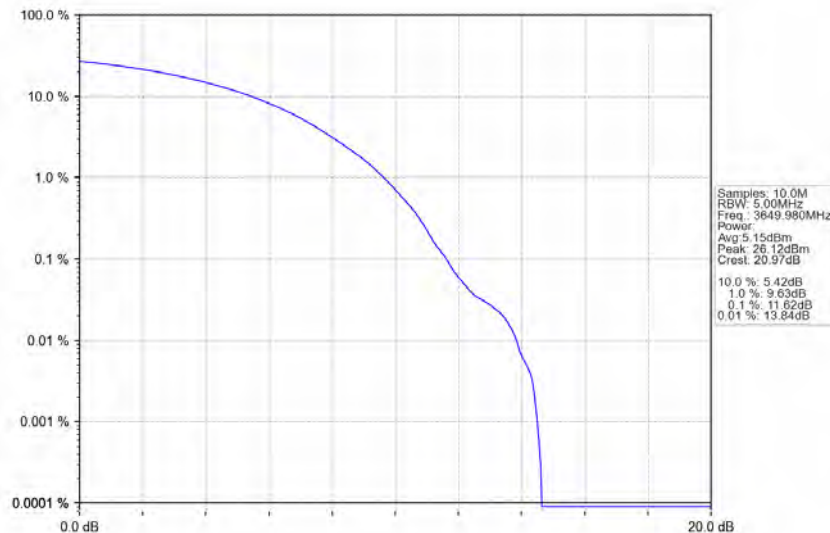
n78d_30kHz_MIMO_NTNV_100MHz_CP-OFDM 64 QAM_3649.98MHz_Outer_Full
