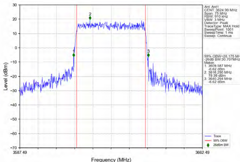
n78d_30kHz_MIMO_NTNV_30MHz_CP-OFDM_16_QAM_3624.99MHz_Outer_Full
