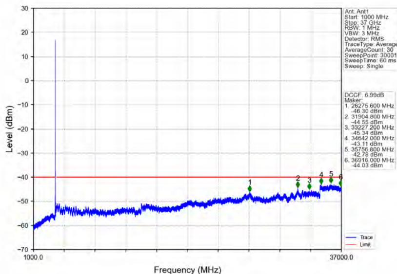
n78d_30kHz_MIMO_NTNV_10MHz_CP-OFDM_QPSK_3555MHz_Edge_1RB_Left
