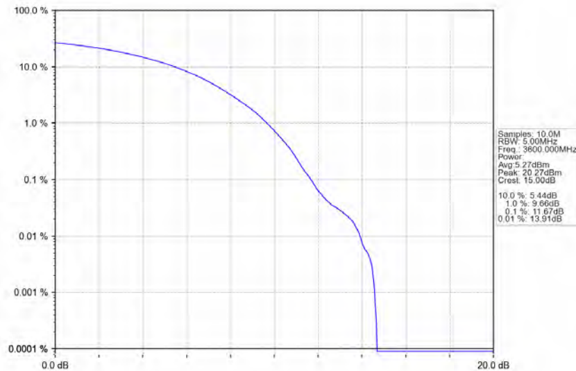
n78d_30kHz_MIMO_NTNV_100MHz_CP-OFDM 64 QAM_3600MHz_Outer_Full
