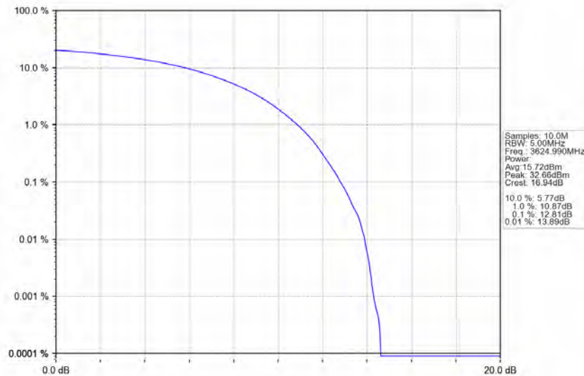
n78d_30kHz_MIMO_NTNV_10MHz_CP-OFDM_QPSK_3624.99MHz_Outer_Full
