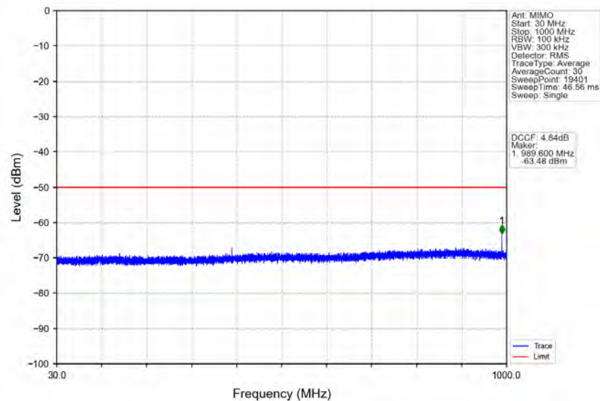
n78d_30kHz_MIMO_NTNV_10MHz_CP-OFDM QPSK_3555MHz_Edge_1RB_Left
