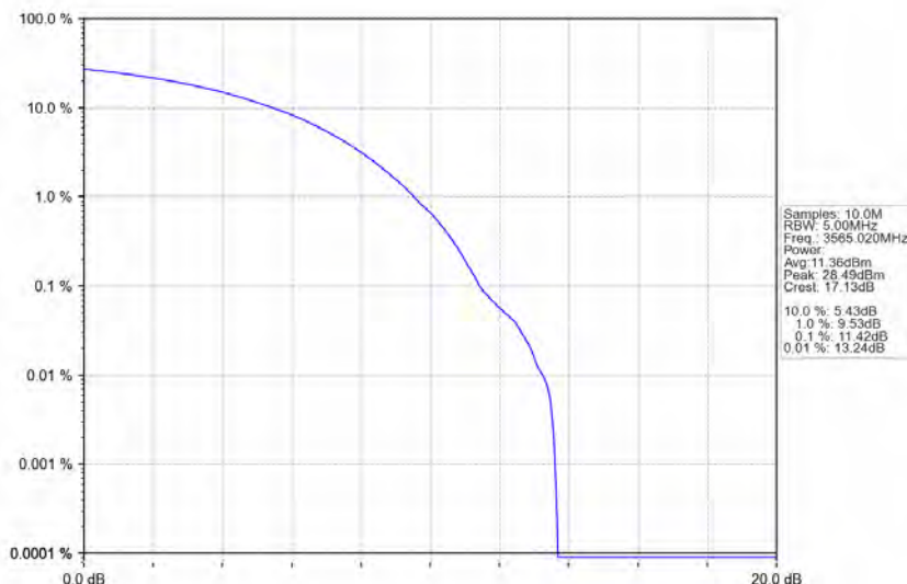
n78d_30kHz_MIMO_NTNV_30MHz_CP-OFDM 64 QAM_3565.02MHz_Outer_Full
