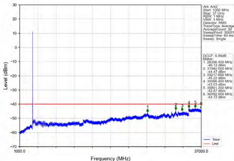
n78d_30kHz_MIMO_NTNV_10MHz_CP-OFDM_QPSK_3555MHz_Outer_Full
