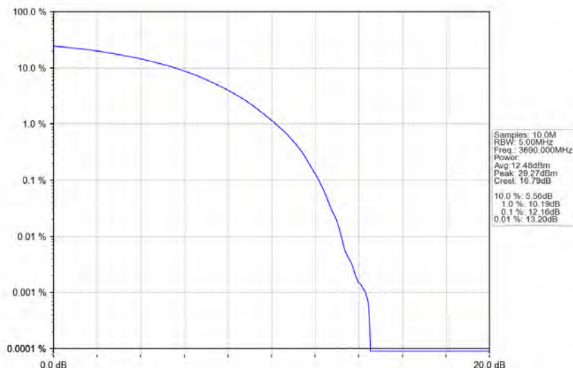
n78d_30kHz_MIMO_NTNV_20MHz_CP-OFDM QPSK_3690MHz_Outer_Full
