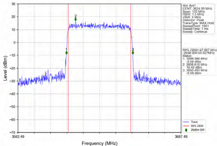
n78d_30kHz_MIMO_NTNV_50MHz_CP-OFDM_256_QAM_3624.99MHz_Outer_Full
