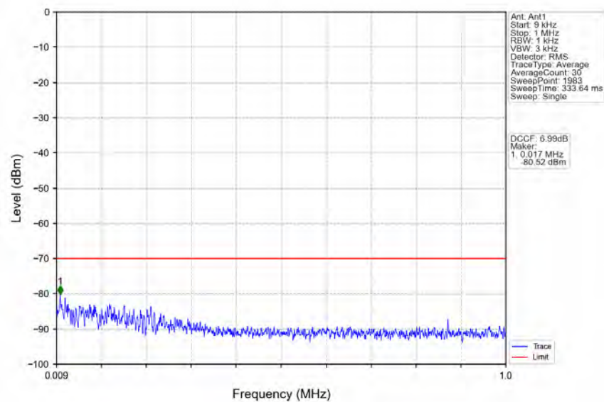
n78d 30kHz MIMO_NTNV_10MHz_CP-OFDM QPSK 3555MHz Edge_1RB Left
