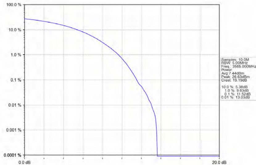
n78d_30kHz_MIMO_NTNV_70MHz_CP-OFDM_16_QAM_3585MHz_Outer_Full
