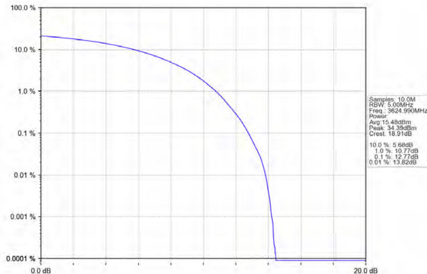
n78d_30kHz_MIMO_NTNV_10MHz_CP-OFDM_64_QAM_3624.99MHz_Outer_Full
