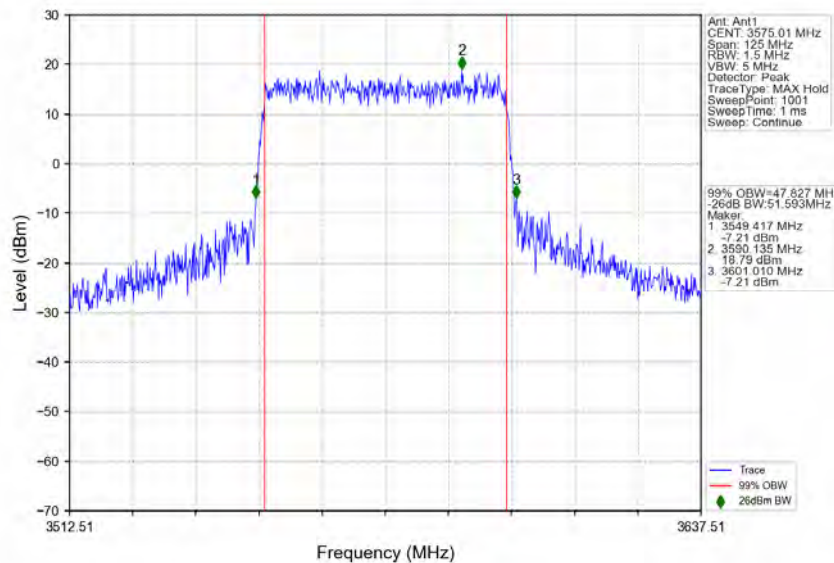
n78d_30kHz_MIMO_NTNV_50MHz_CP-OFDM_64_QAM_3575.01MHz_Outer_Full
