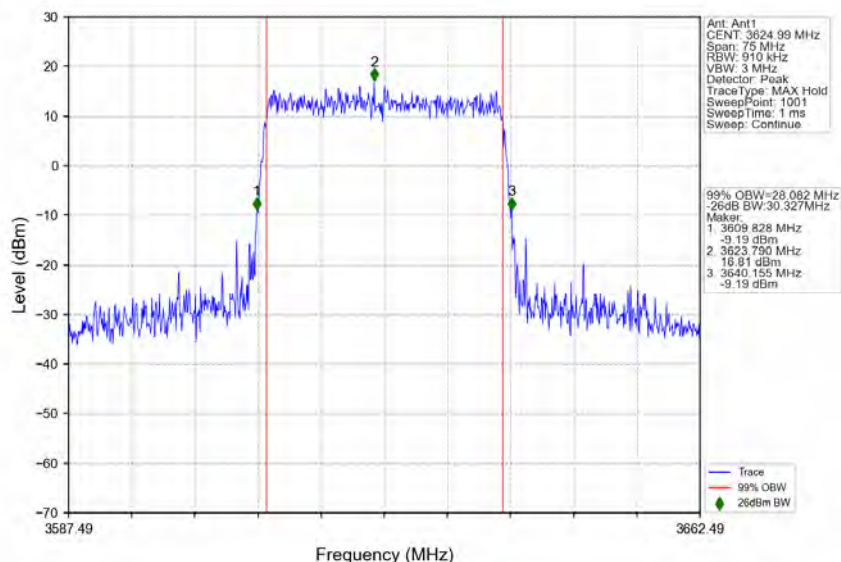
n78d_30kHz_MIMO_NTNV_30MHz_CP-OFDM_256_QAM_3624.99MHz_Outer_Full
