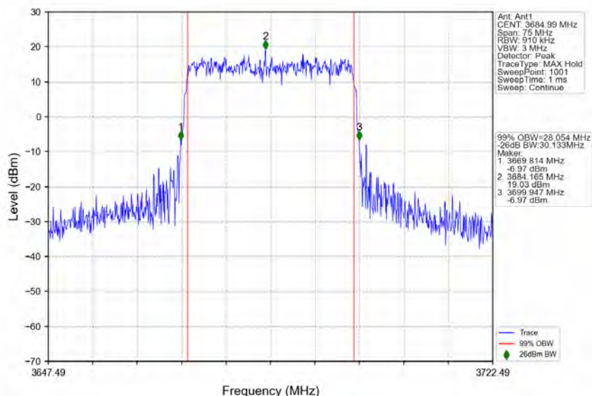
n78d_30kHz_MIMO_NTNV_30MHz_CP-OFDM 64 QAM_3684.99MHz_Outer_Full
