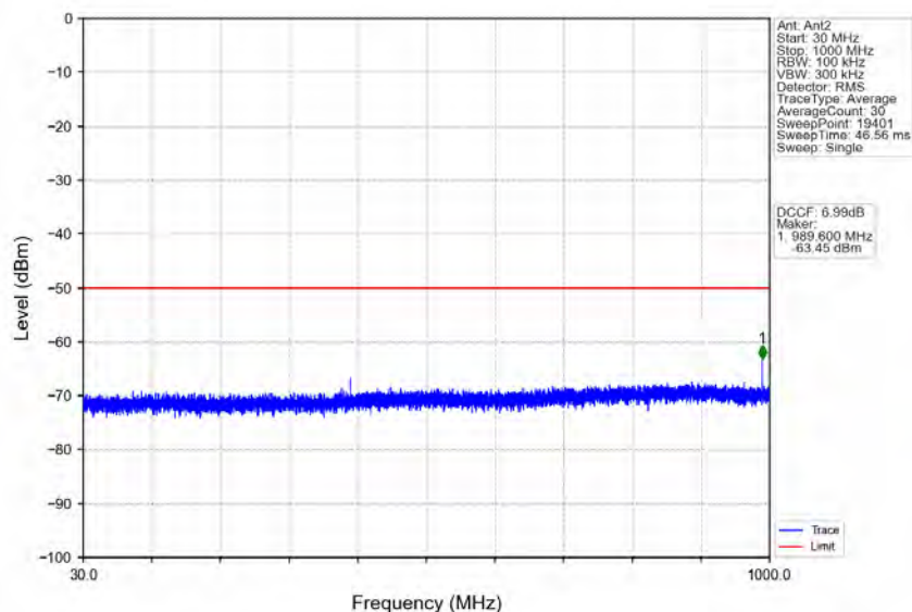
n78d_30kHz_MIMO_NTNV_10MHz_CP-OFDM_QPSK_3555MHz_Edge_1RB_Left
