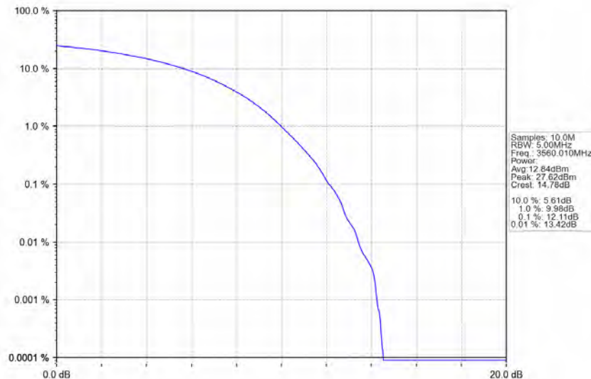
n78d_30kHz_MIMO_NTNV_20MHz_CP-OFDM_16_QAM_3560.01MHz_Outer_Full
