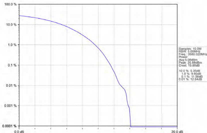
n78d_30kHz_MIMO_NTNV_60MHz_CP-OFDM_256_QAM_3580.02MHz_Outer_Full
