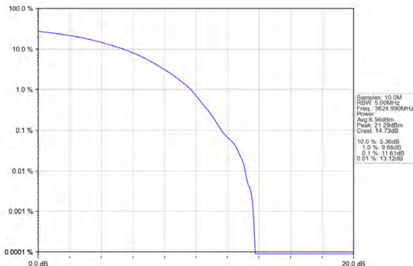
n78d_30kHz_MIMO_NTNV_90MHz_CP-OFDM_16_QAM_3624.99MHz_Outer_Full
