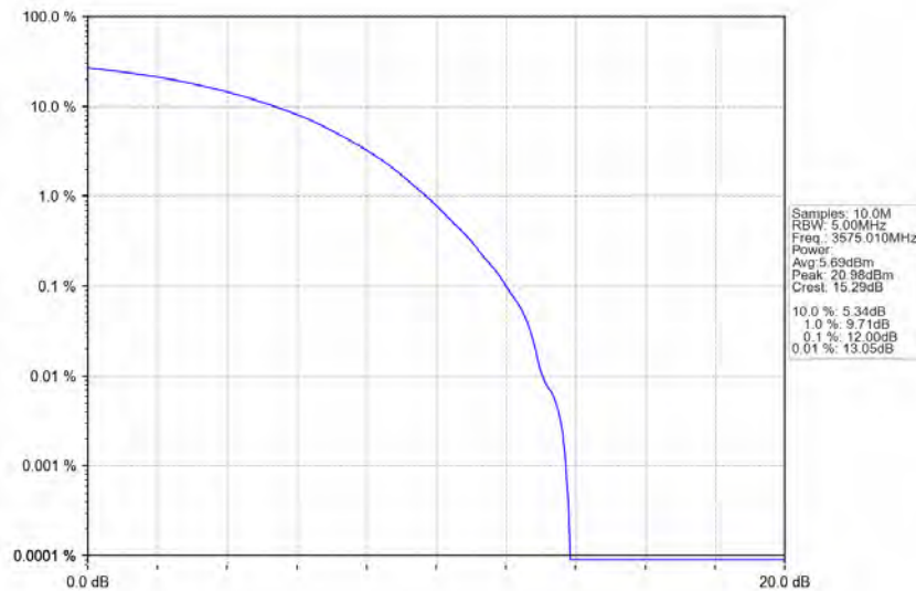
n78d_30kHz_MIMO_NTNV_50MHz_CP-OFDM_256_QAM_3575.01MHz_Outer_Full
