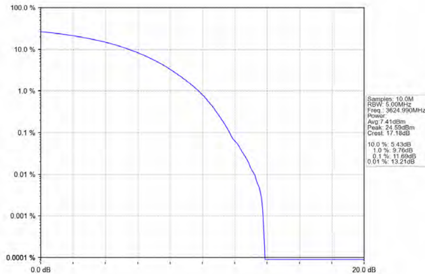
n78d_30kHz_MIMO_NTNV_70MHz_CP-OFDM_16_QAM_3624.99MHz_Outer_Full
