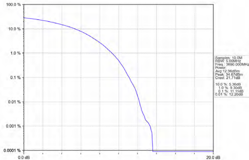
n78d_30kHz_MIMO_NTNV_20MHz_CP-OFDM_64_QAM_3690MHz_Outer_Full
