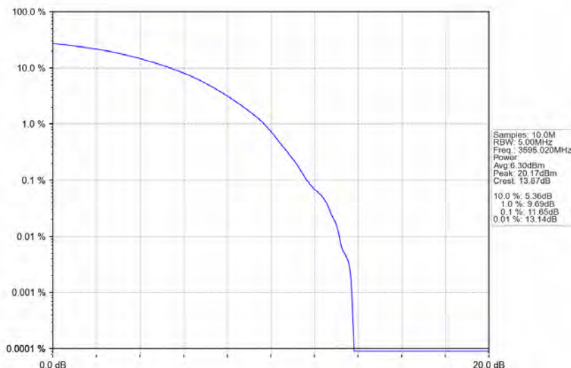
n78d_30kHz_MIMO_NTNV_90MHz_CP-OFDM_16_QAM_3595.02MHz_Outer_Full
