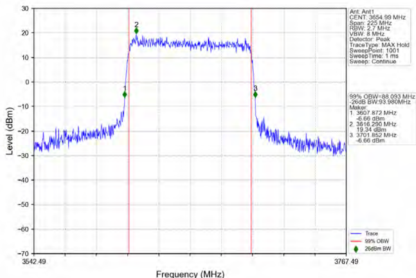
n78d_30kHz_MIMO_NTNV_90MHz_CP-OFDM_64_QAM_3654.99MHz_Outer_Full
