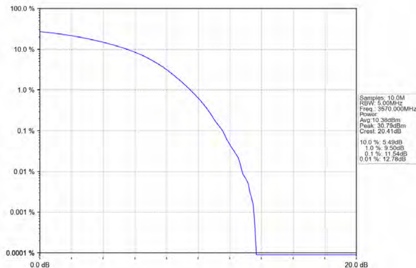
n78d_30kHz_MIMO_NTNV_40MHz_CP-OFDM_16_QAM_3570MHz_Outer_Full
