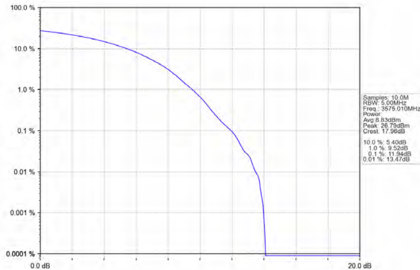
n78d_30kHz_MIMO_NTNV_50MHz_CP-OFDM_64_QAM_3575.01MHz_Outer_Full
