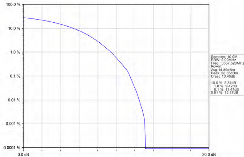
n78d_30kHz_MIMO_NTNV_15MHz_CP-OFDM_16_QAM_3557.52MHz_Outer_Full
