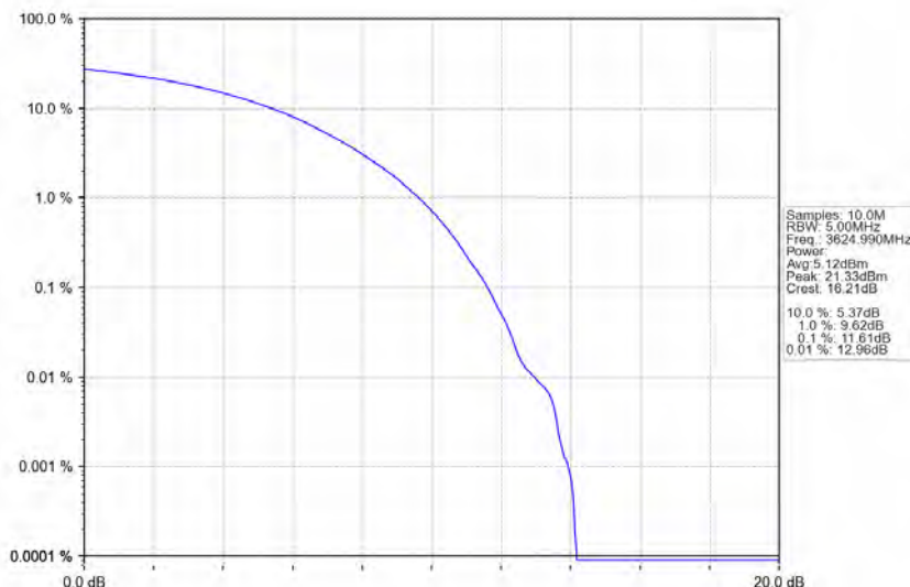
n78d_30kHz_MIMO_NTNV_60MHz_CP-OFDM_256_QAM_3624.99MHz_Outer_Full
