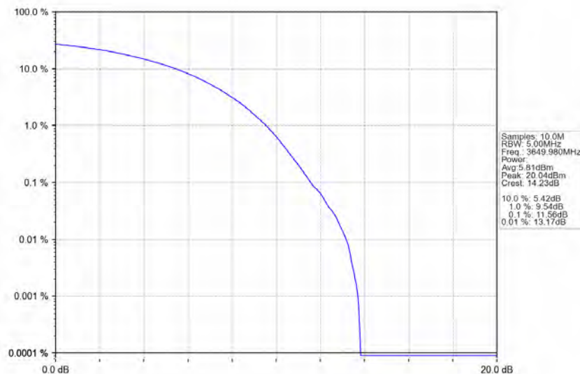
n78d_30kHz_MIMO_NTNV_100MHz_CP-OFDM QPSK_3649.98MHz_Outer_Full
