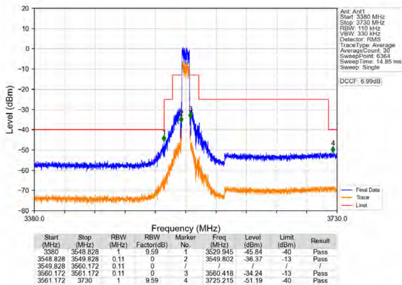
n78d_30kHz_MIMO_NTNV_10MHz_CP-OFDM QPSK_3555MHz_Outer_Full
