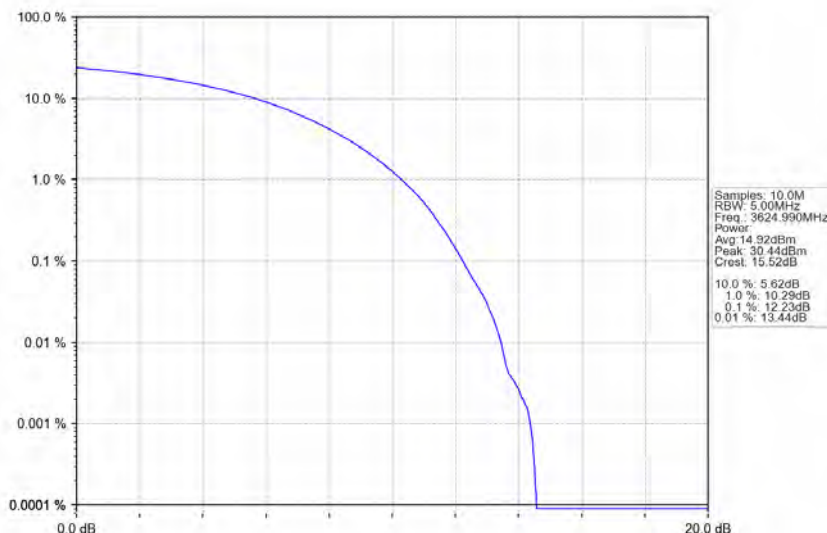
n78d_30kHz_MIMO_NTNV_15MHz_CP-OFDM_QPSK_3624.99MHz_Outer_Full
