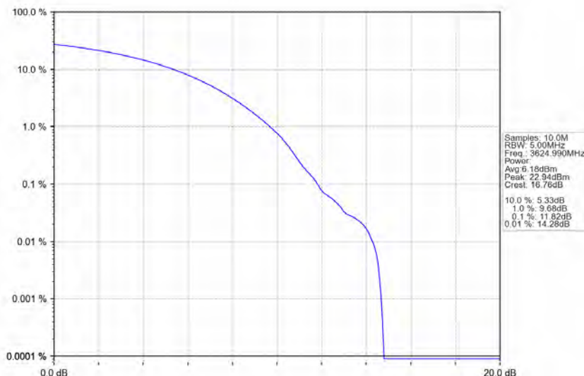
n78d_30kHz_MIMO_NTNV_90MHz_CP-OFDM 64 QAM_3624.99MHz_Outer_Full
