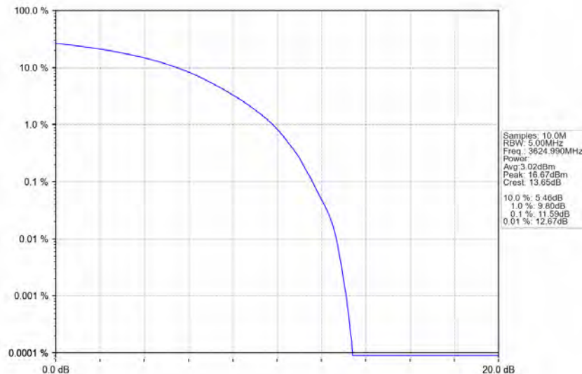
n78d_30kHz_MIMO_NTNV_90MHz_CP-OFDM_256_QAM_3624.99MHz_Outer_Full
