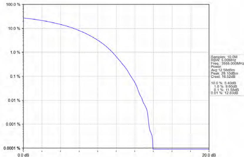
n78d_30kHz_MIMO_NTNV_10MHz_CP-OFDM_256_QAM_3555MHz_Outer_Full
