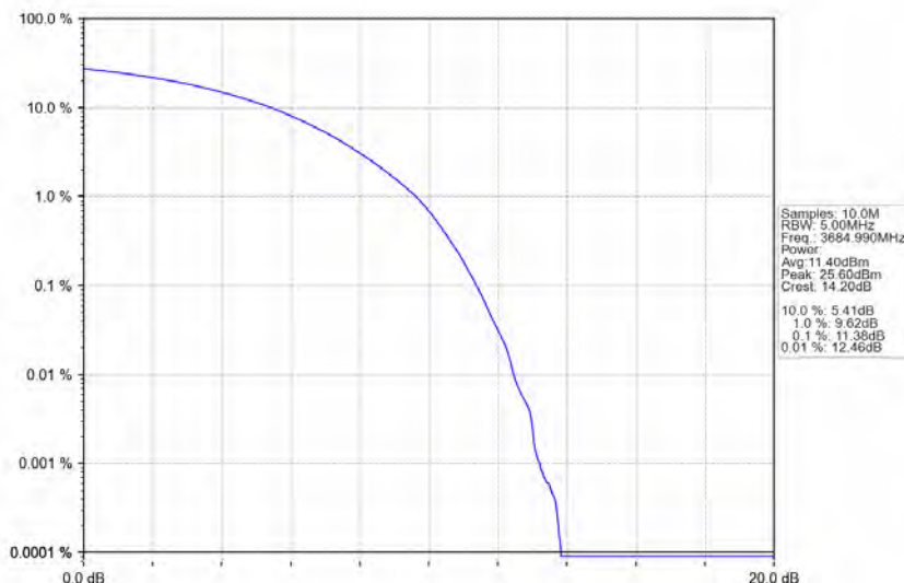
n78d_30kHz_MIMO_NTNV_30MHz_CP-OFDM 16 QAM_3684.99MHz_Outer_Full
