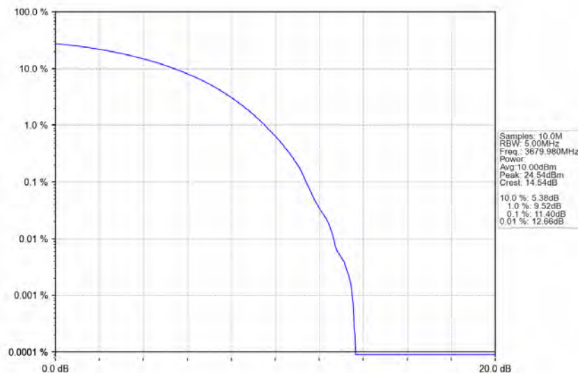
n78d_30kHz_MIMO_NTNV_40MHz_CP-OFDM QPSK_3679.98MHz_Outer_Full
