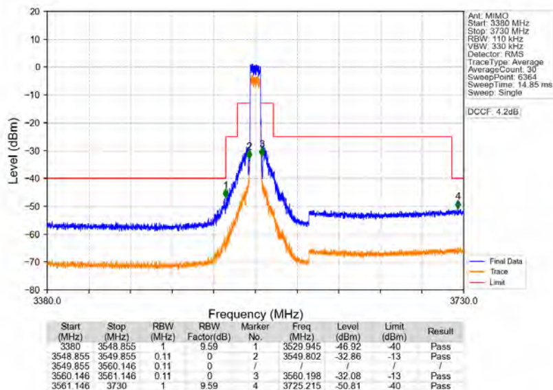
n78d_30kHz_MIMO_NTNV_10MHz_CP-OFDM_QPSK_3555MHz_Outer_Full
