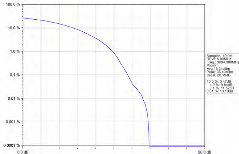
n78d_30kHz_MIMO_NTNV_10MHz_CP-OFDM_64_QAM_3694.98MHz_Outer_Full
