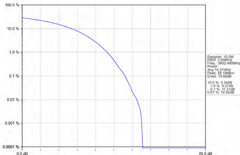
n78d_30kHz_MIMO_NTNV_15MHz_CP-OFDM_QPSK_3692.49MHz_Outer_Full
