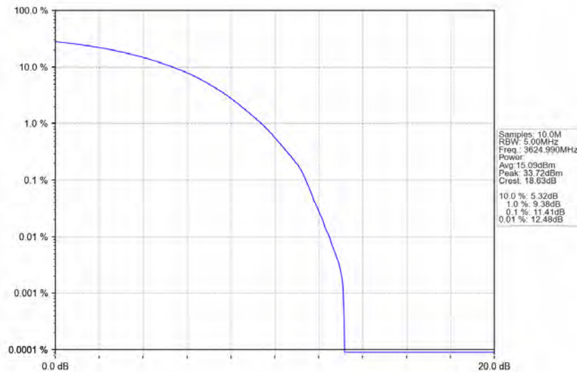
n78d_30kHz_MIMO_NTNV_15MHz_CP-OFDM_16_QAM_3624.99MHz_Outer_Full
