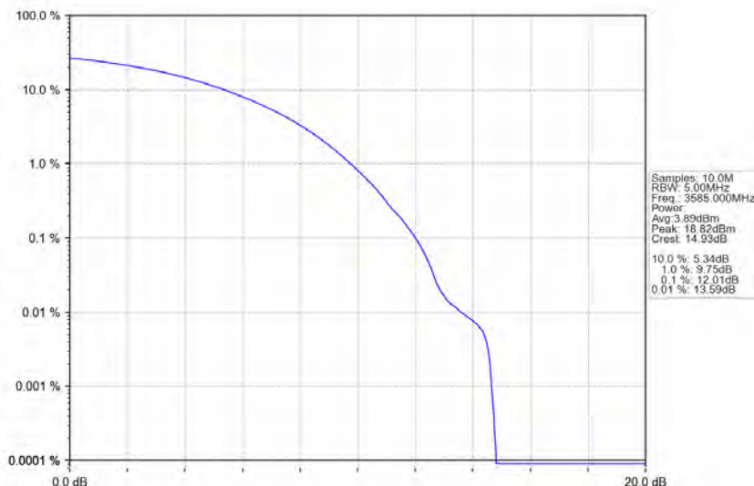
n78d_30kHz_MIMO_NTNV_70MHz_CP-OFDM_256_QAM_3585MHz_Outer_Full
