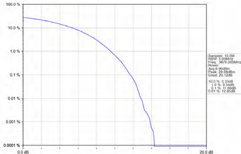
n78d_30kHz_MIMO_NTNV_50MHz_CP-OFDM QPSK_3675MHz_Outer_Full
