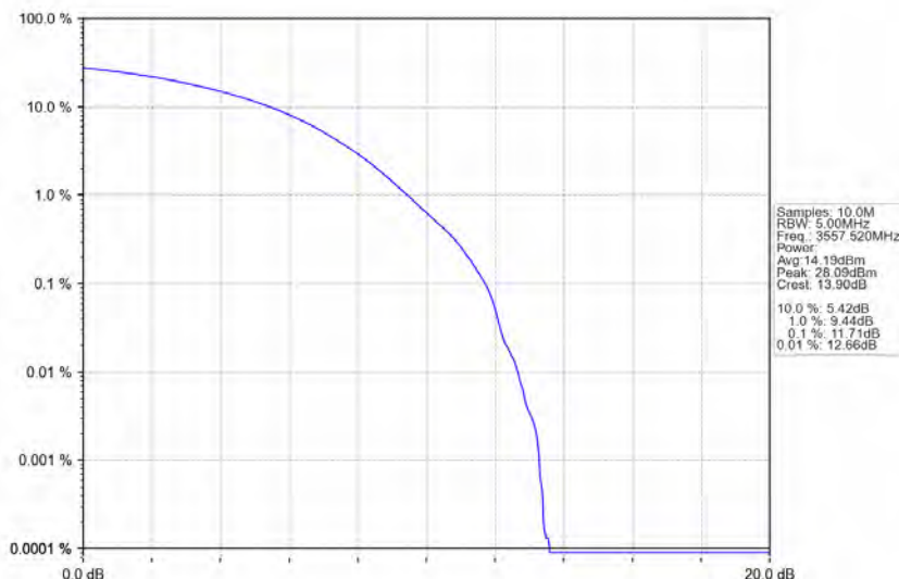
n78d_30kHz_MIMO_NTNV_15MHz_CP-OFDM_64_QAM_3557.52MHz_Outer_Full
