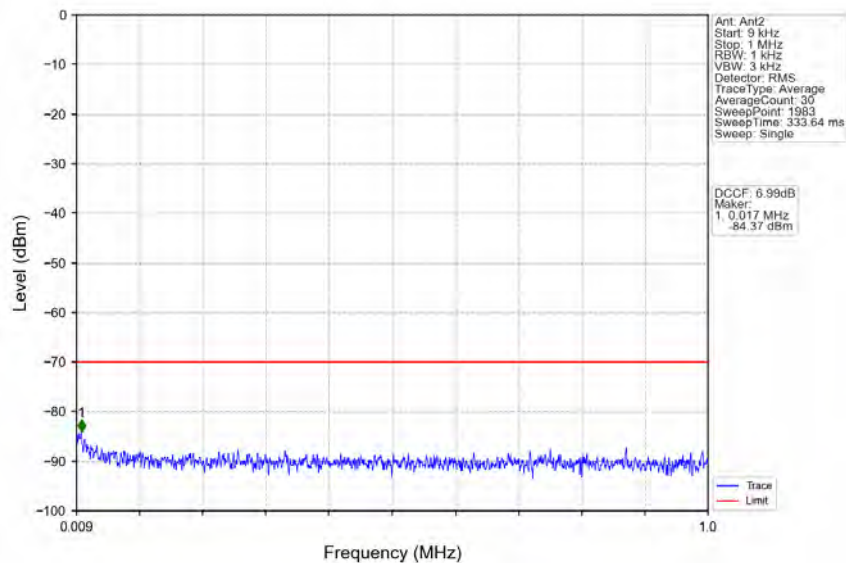
n78d_30kHz_MIMO_NTNV_10MHz_CP-OFDM_QPSK_3555MHz_Outer_Full
