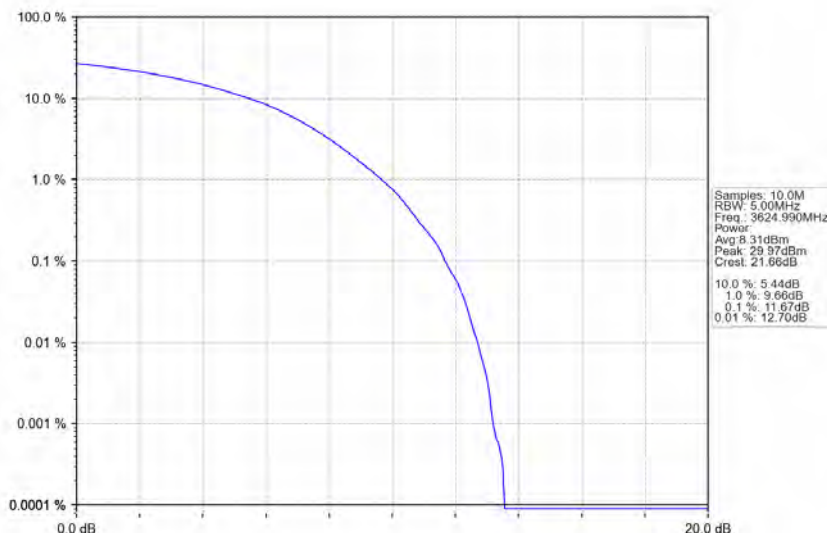
n78d_30kHz_MIMO_NTNV_30MHz_CP-OFDM_256_QAM_3624.99MHz_Outer_Full
