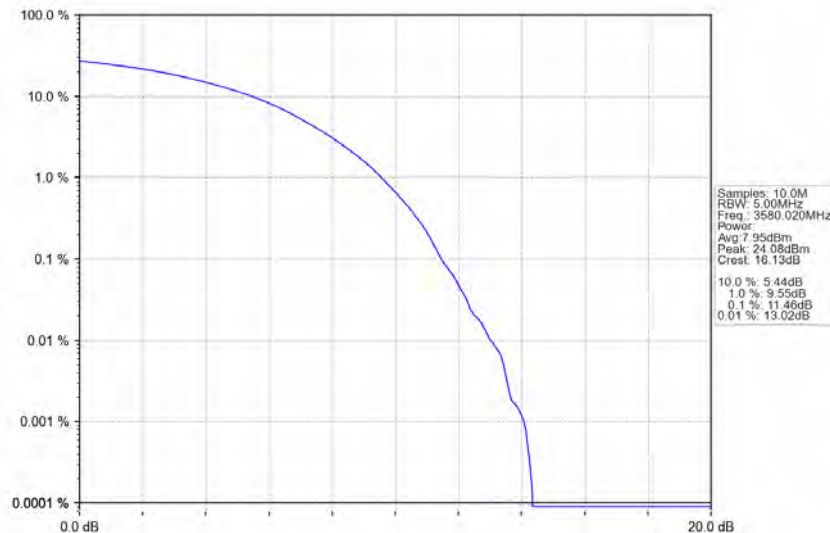
n78d_30kHz_MIMO_NTNV_60MHz_CP-OFDM_64_QAM_3580.02MHz_Outer_Full
