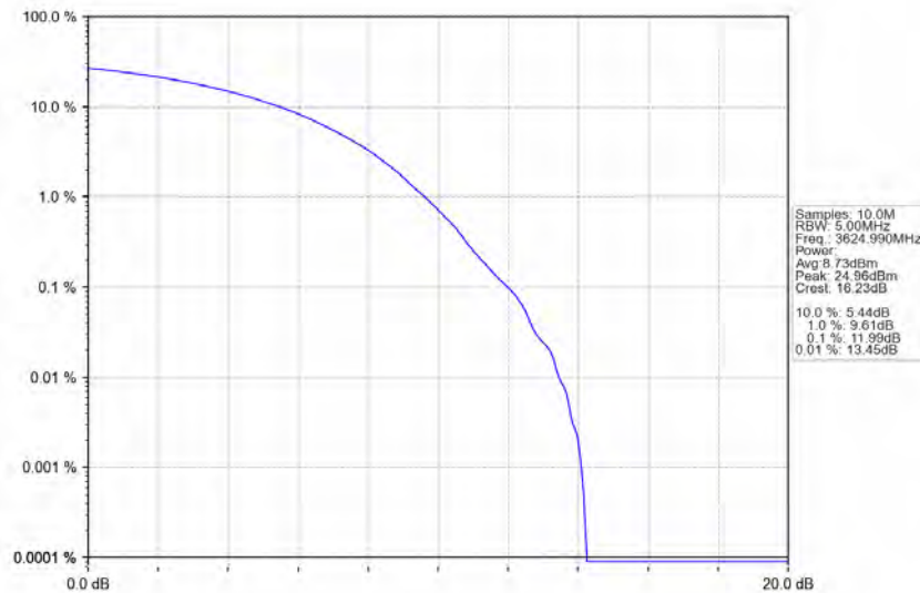
n78d_30kHz_MIMO_NTNV_50MHz_CP-OFDM 64 QAM_3624.99MHz_Outer_Full
