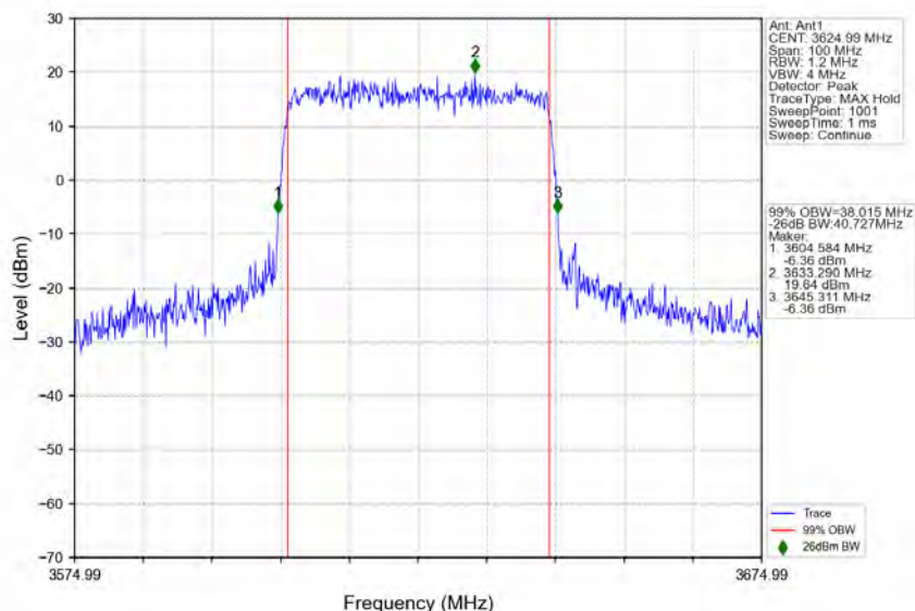
n78d_30kHz_MIMO_NTNV_40MHz_CP-OFDM_16_QAM_3624.99MHz_Outer_Full
