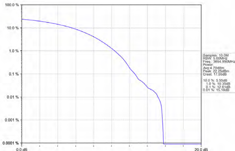
n78d_30kHz_MIMO_NTNV_90MHz_CP-OFDM 64 QAM_3654.99MHz_Outer_Full
