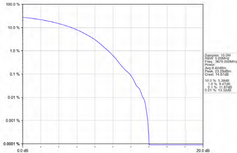
n78d_30kHz_MIMO_NTNV_50MHz_CP-OFDM 64 QAM_3675MHz_Outer_Full
