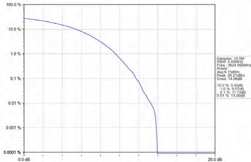
n78d_30kHz_MIMO_NTNV_100MHz_CP-OFDM_16_QAM_3624.99MHz_Outer_Full
