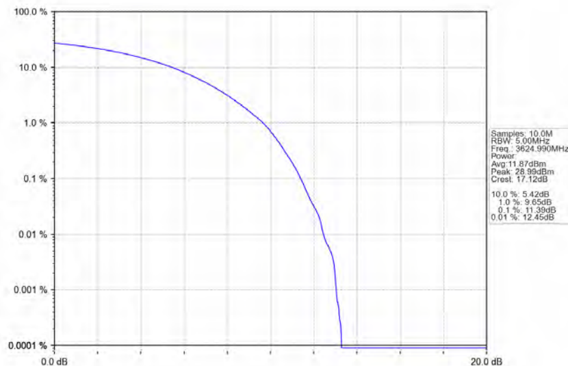
n78d_30kHz_MIMO_NTNV_30MHz_CP-OFDM_16_QAM_3624.99MHz_Outer_Full
