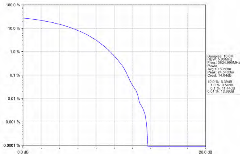
n78d_30kHz_MIMO_NTNV_40MHz_CP-OFDM QPSK_3624.99MHz_Outer_Full
