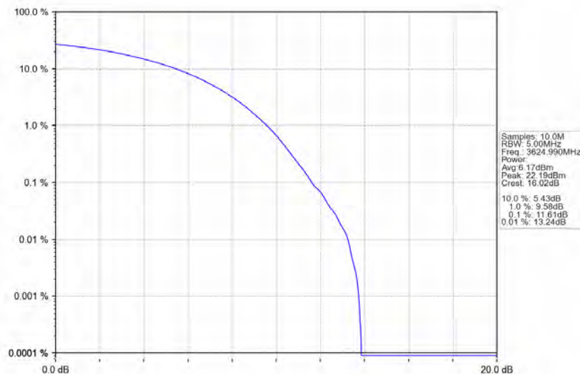
n78d_30kHz_MIMO_NTNV_100MHz_CP-OFDM QPSK_3624.99MHz_Outer_Full
