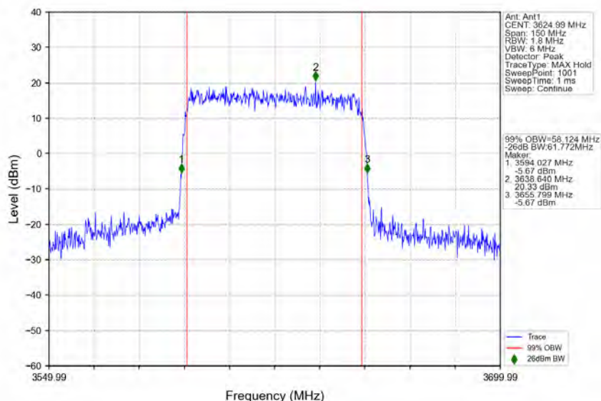
n78d_30kHz_MIMO_NTNV_60MHz_CP-OFDM_16_QAM_3624.99MHz_Outer_Full
