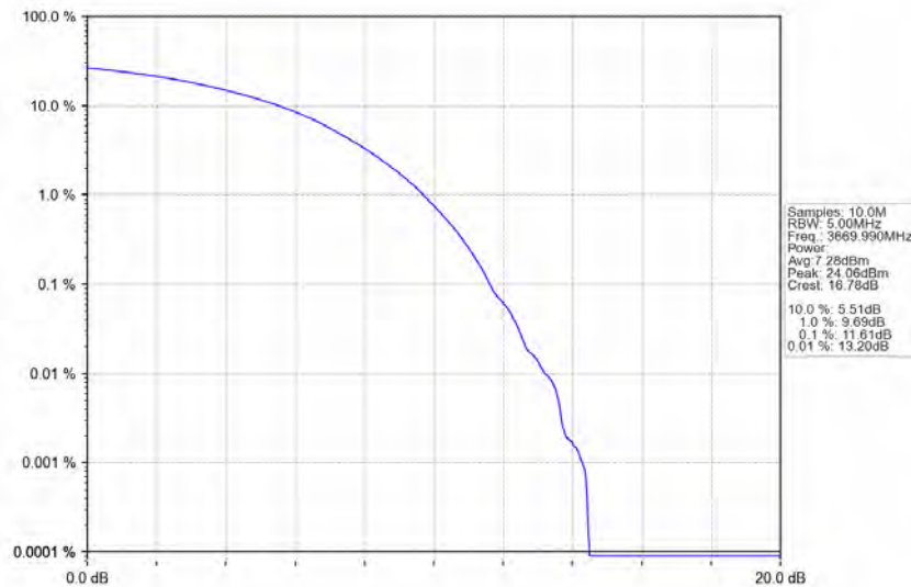
n78d_30kHz_MIMO_NTNV_60MHz_CP-OFDM 64 QAM_3669.99MHz_Outer_Full
