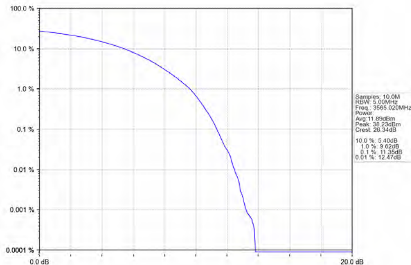
n78d_30kHz_MIMO_NTNV_30MHz_CP-OFDM_16_QAM_3565.02MHz_Outer_Full
