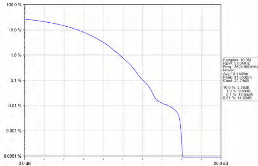
n78d_30kHz_MIMO_NTNV_20MHz_CP-OFDM_256_QAM_3624.99MHz_Outer_Full
