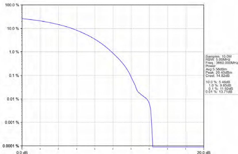
n78d_30kHz_MIMO_NTNV_80MHz_CP-OFDM_64_QAM_3660MHz_Outer_Full
