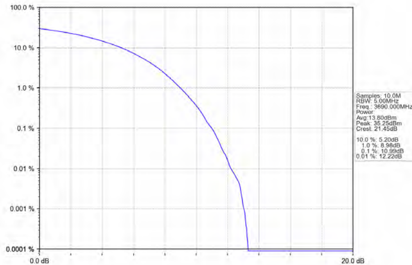
n78d_30kHz_MIMO_NTNV_20MHz_CP-OFDM_16_QAM_3690MHz_Outer_Full
