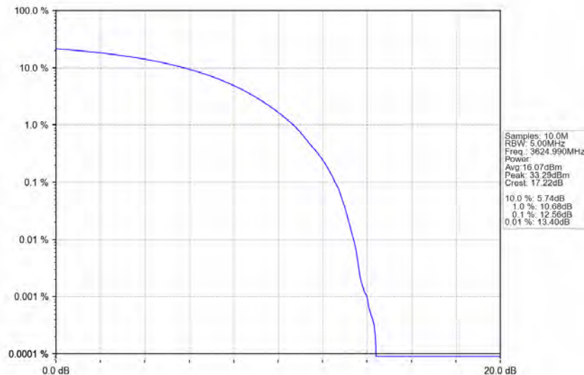
n78d_30kHz_MIMO_NTNV_10MHz_CP-OFDM_16_QAM_3624.99MHz_Outer_Full
