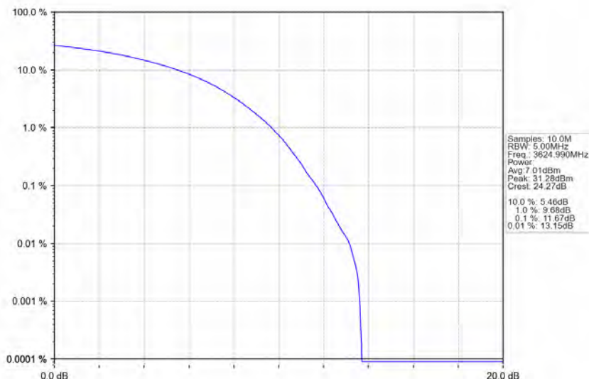
n78d_30kHz_MIMO_NTNV_70MHz_CP-OFDM_64_QAM_3624.99MHz_Outer_Full
