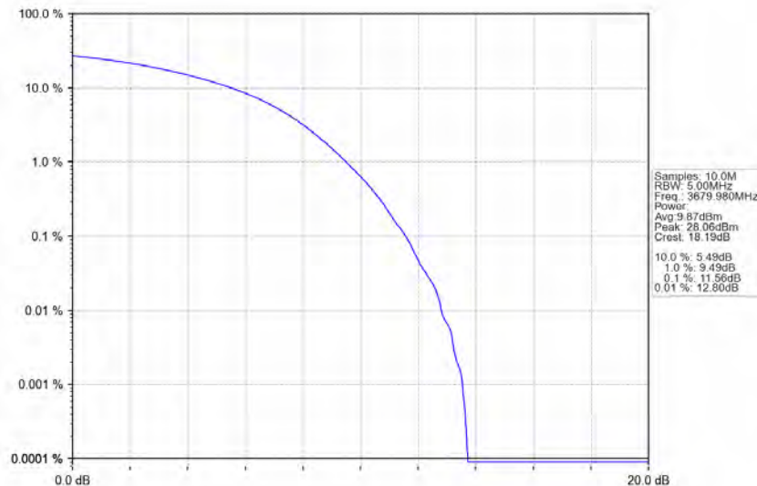
n78d_30kHz_MIMO_NTNV_40MHz_CP-OFDM_16_QAM_3679.98MHz_Outer_Full
