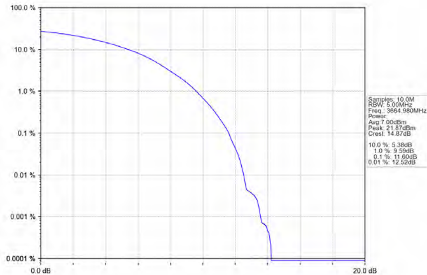
n78d_30kHz_MIMO_NTNV_70MHz_CP-OFDM QPSK_3664.98MHz_Outer_Full
