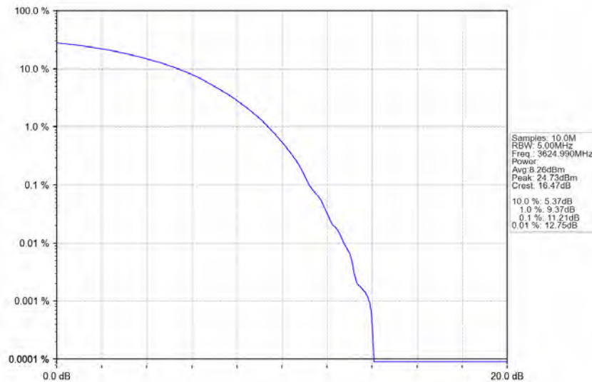
n78d_30kHz_MIMO_NTNV_60MHz_CP-OFDM 64 QAM_3624.99MHz_Outer_Full
