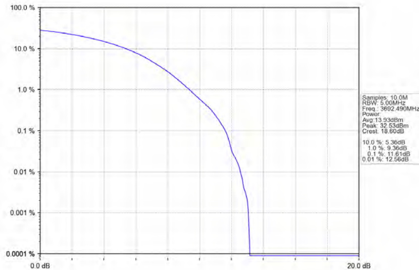
n78d_30kHz_MIMO_NTNV_15MHz_CP-OFDM_64_QAM_3692.49MHz_Outer_Full
