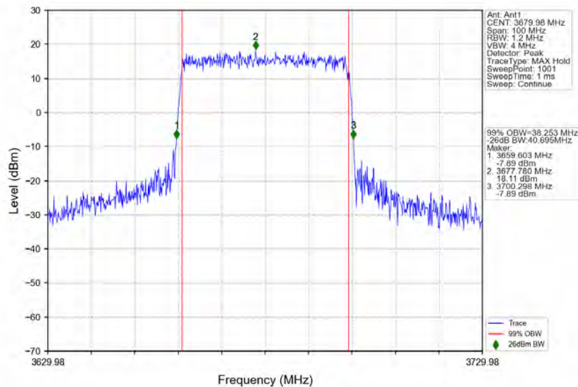
n78d_30kHz_MIMO_NTNV_40MHz_CP-OFDM_64_QAM_3679.98MHz_Outer_Full
