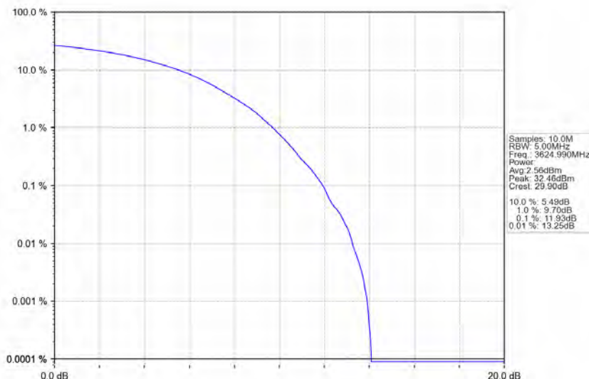
n78d_30kHz_MIMO_NTNV_100MHz_CP-OFDM_256_QAM_3624.99MHz_Outer_Full
