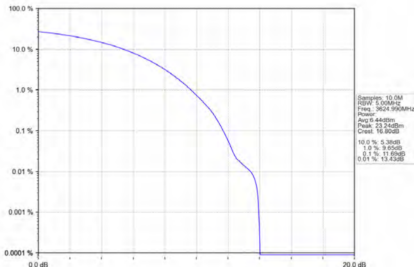
n78d_30kHz_MIMO_NTNV_80MHz_CP-OFDM_64_QAM_3624.99MHz_Outer_Full
