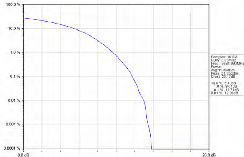
n78d_30kHz_MIMO_NTNV_30MHz_CP-OFDM_QPSK_3684.99MHz_Outer_Full
