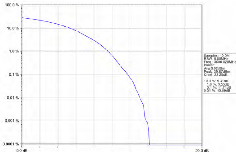
n78d_30kHz_MIMO_NTNV_60MHz_CP-OFDM_16_QAM_3580.02MHz_Outer_Full
