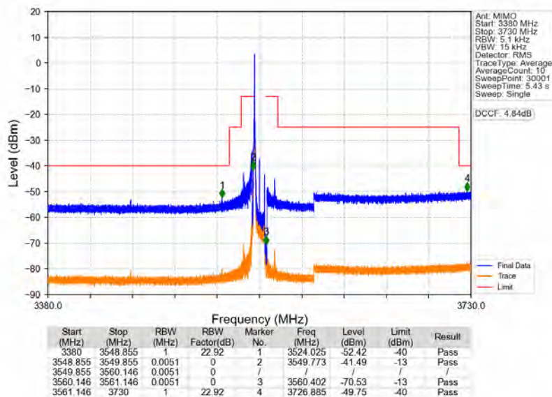
n78d_30kHz_MIMO_NTNV_10MHz_CP-OFDM_QPSK_3555MHz_Edge_1RB_Left
