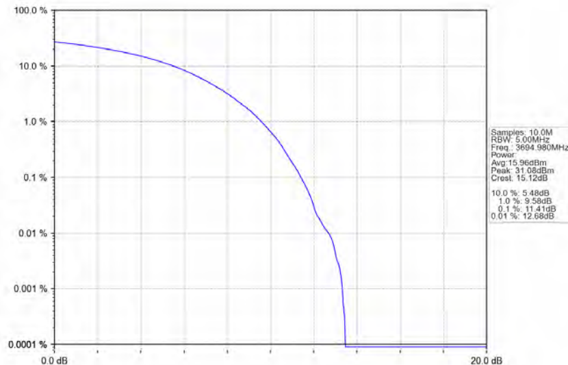
n78d_30kHz_MIMO_NTNV_10MHz_CP-OFDM_16_QAM_3694.98MHz_Outer_Full
