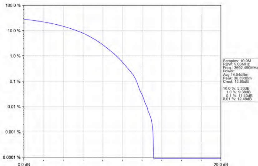
n78d_30kHz_MIMO_NTNV_15MHz_CP-OFDM_16_QAM_3692.49MHz_Outer_Full
