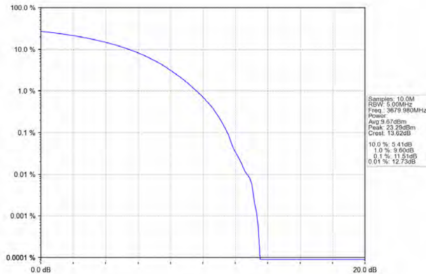
n78d_30kHz_MIMO_NTNV_40MHz_CP-OFDM_64_QAM_3679.98MHz_Outer_Full
