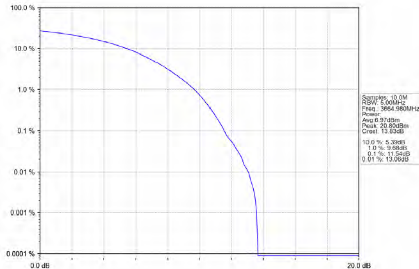
n78d_30kHz_MIMO_NTNV_70MHz_CP-OFDM_16_QAM_3664.98MHz_Outer_Full
