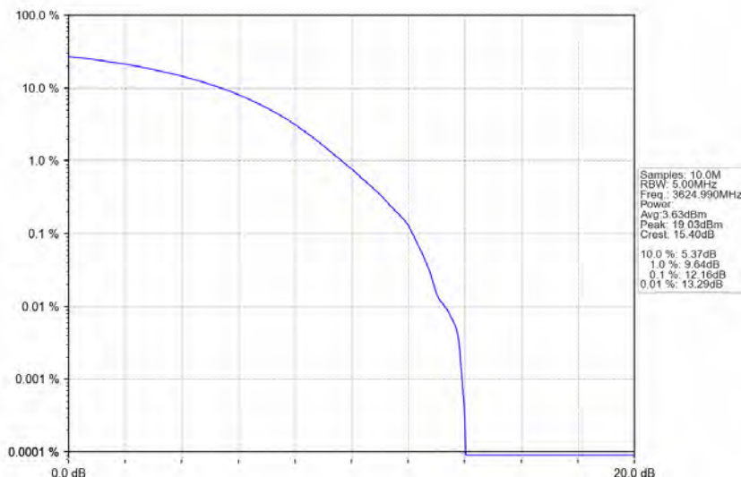
n78d_30kHz_MIMO_NTNV_80MHz_CP-OFDM_256_QAM_3624.99MHz_Outer_Full
