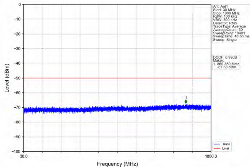
n78d_30kHz_MIMO_NTNV_10MHz_CP-OFDM QPSK_3555MHz_Outer_Full
