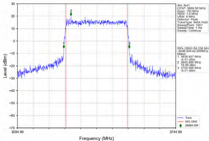
n78d_30kHz_MIMO_NTNV_60MHz_CP-OFDM_64_QAM_3669.99MHz_Outer_Full
