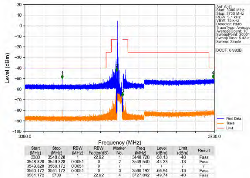
n78d_30kHz_MIMO_NTNV_10MHz_CP-OFDM_QPSK_3555MHz_Inner_1RB_Left
