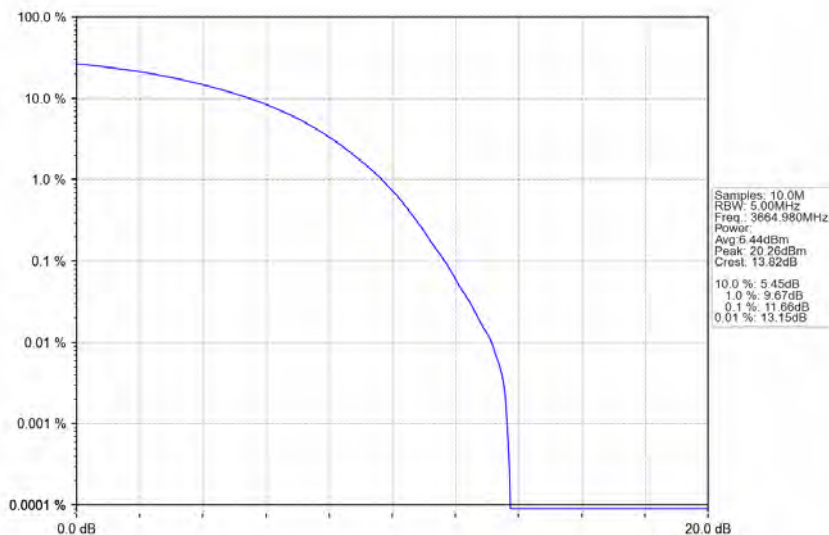
n78d_30kHz_MIMO_NTNV_70MHz_CP-OFDM_64_QAM_3664.98MHz_Outer_Full
