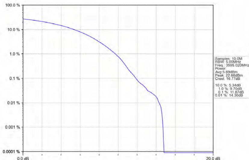
n78d_30kHz_MIMO_NTNV_90MHz_CP-OFDM_64_QAM_3595.02MHz_Outer_Full
