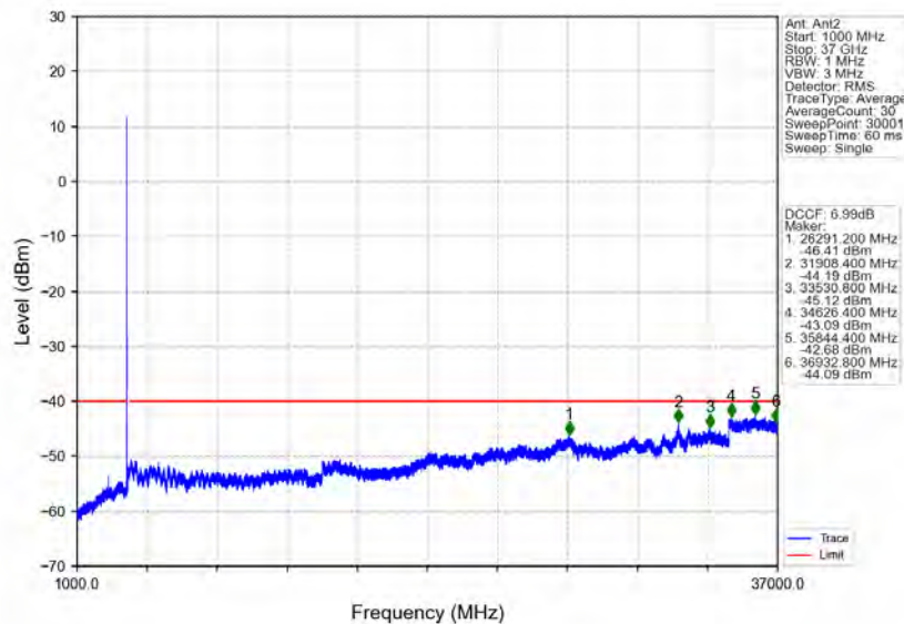
n78d_30kHz_MIMO_NTNV_10MHz_CP-OFDM_QPSK_3555MHz_Inner_1RB_Left
