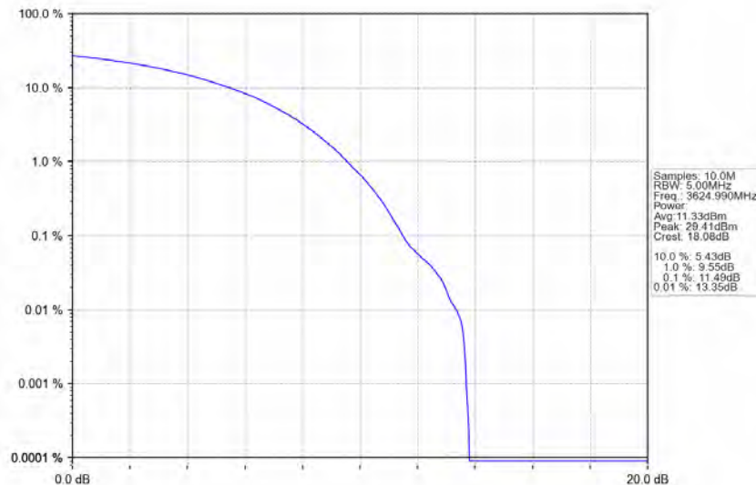
n78d_30kHz_MIMO_NTNV_30MHz_CP-OFDM_64_QAM_3624.99MHz_Outer_Full
