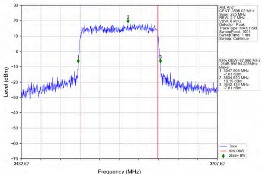
n78d_30kHz_MIMO_NTNV_90MHz_CP-OFDM 64 QAM_3595.02MHz_Outer_Full
