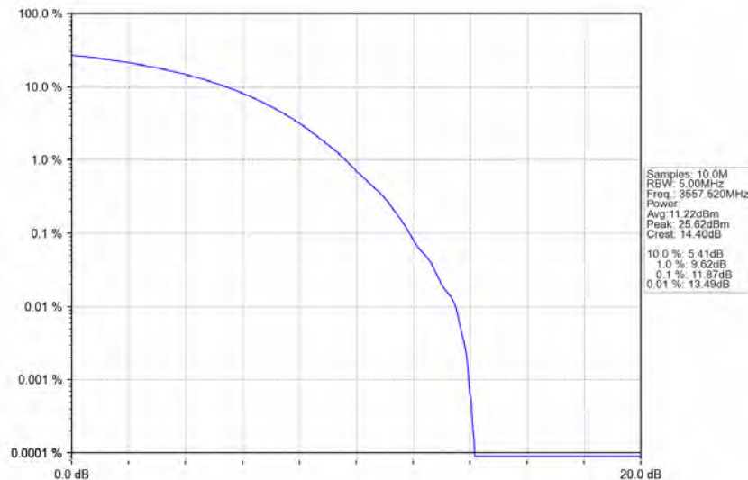
n78d_30kHz_MIMO_NTNV_15MHz_CP-OFDM_256_QAM_3557.52MHz_Outer_Full
