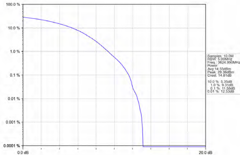
n78d_30kHz_MIMO_NTNV_15MHz_CP-OFDM_64_QAM_3624.99MHz_Outer_Full
