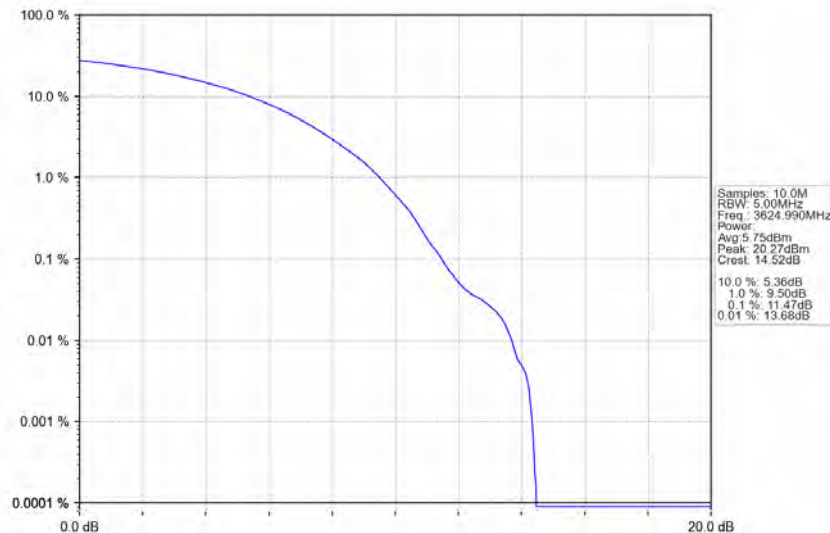
n78d_30kHz_MIMO_NTNV_100MHz_CP-OFDM 64 QAM_3624.99MHz_Outer_Full
