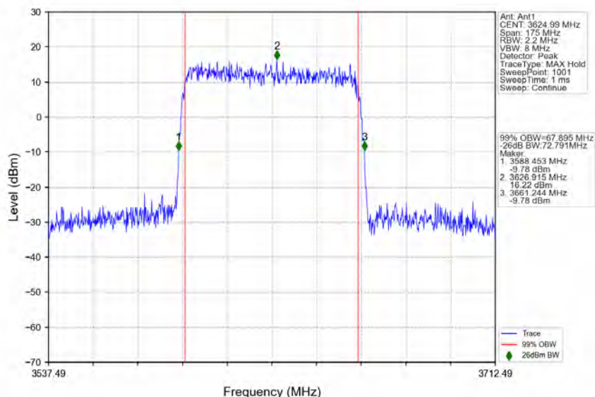
n78d_30kHz_MIMO_NTNV_70MHz_CP-OFDM_256_QAM_3624.99MHz_Outer_Full
