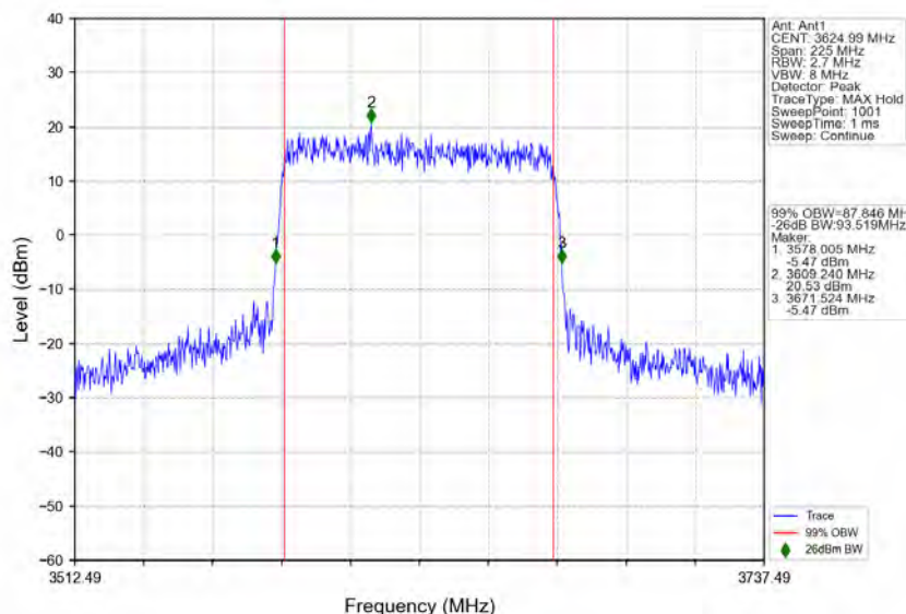
n78d_30kHz_MIMO_NTNV_90MHz_CP-OFDM_16_QAM_3624.99MHz_Outer_Full
