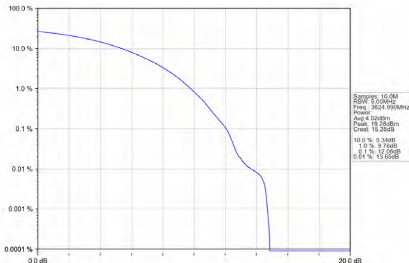
n78d_30kHz_MIMO_NTNV_70MHz_CP-OFDM_256_QAM_3624.99MHz_Outer_Full
