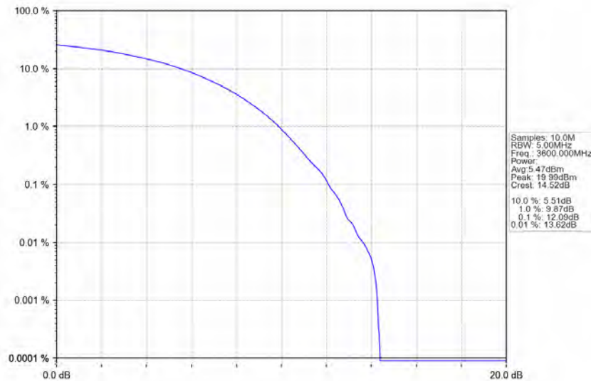
n78d_30kHz_MIMO_NTNV_100MHz_CP-OFDM_16_QAM_3600MHz_Outer_Full
