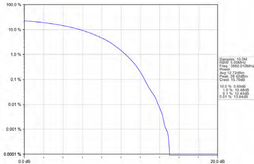
n78d_30kHz_MIMO_NTNV_20MHz_CP-OFDM_64_QAM_3560.01MHz_Outer_Full
