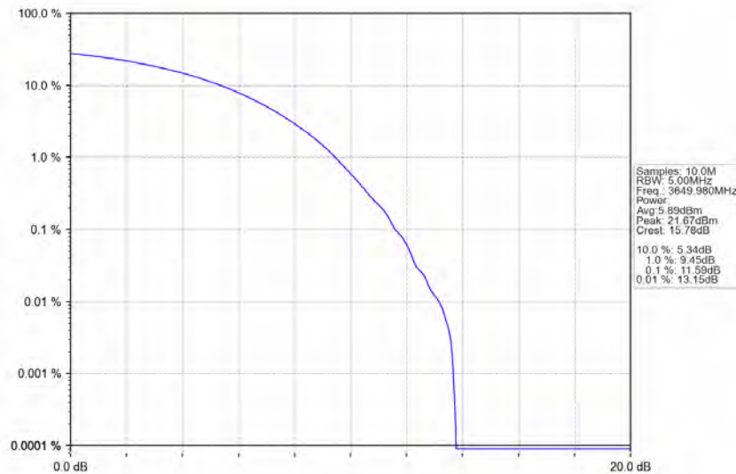
n78d_30kHz_MIMO_NTNV_100MHz_CP-OFDM 16 QAM_3649.98MHz_Outer_Full
