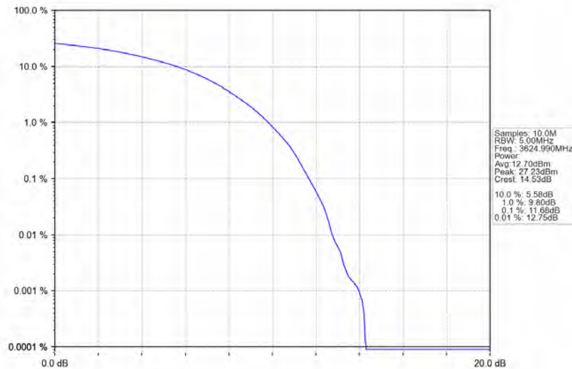
n78d_30kHz_MIMO_NTNV_20MHz_CP-OFDM_64_QAM_3624.99MHz_Outer_Full
