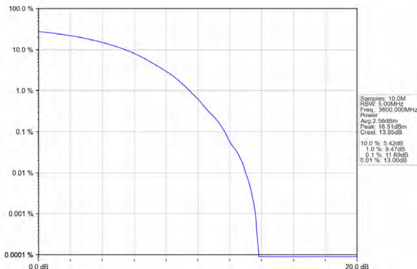
n78d_30kHz_MIMO_NTNV_100MHz_CP-OFDM_256_QAM_3600MHz_Outer_Full
