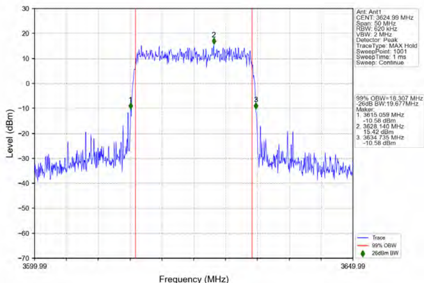
n78d_30kHz_MIMO_NTNV_20MHz_CP-OFDM_256_QAM_3624.99MHz_Outer_Full
