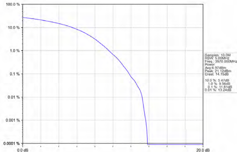
n78d_30kHz_MIMO_NTNV_40MHz_CP-OFDM_256_QAM_3570MHz_Outer_Full
