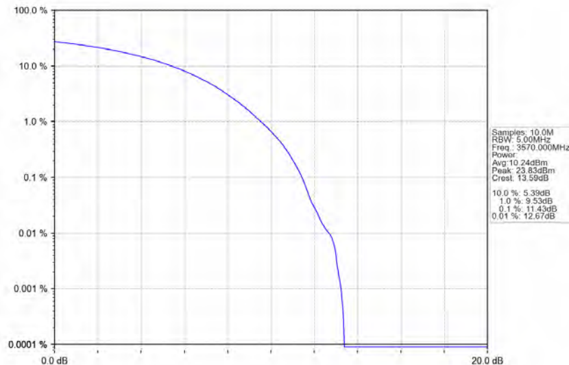
n78d_30kHz_MIMO_NTNV_40MHz_CP-OFDM_64_QAM_3570MHz_Outer_Full
