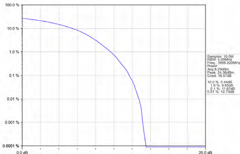
n78d_30kHz_MIMO_NTNV_30MHz_CP-OFDM_256_QAM_3565.02MHz_Outer_Full
