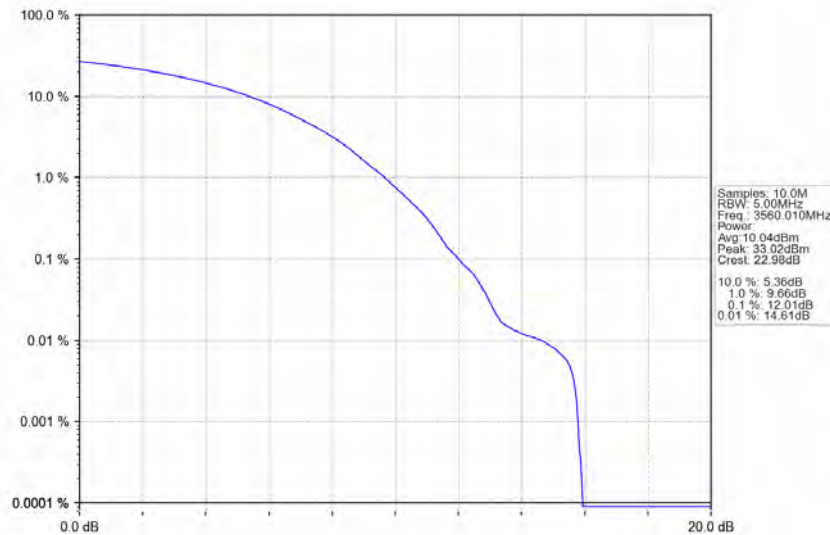
n78d_30kHz_MIMO_NTNV_20MHz_CP-OFDM_256_QAM_3560.01MHz_Outer_Full
