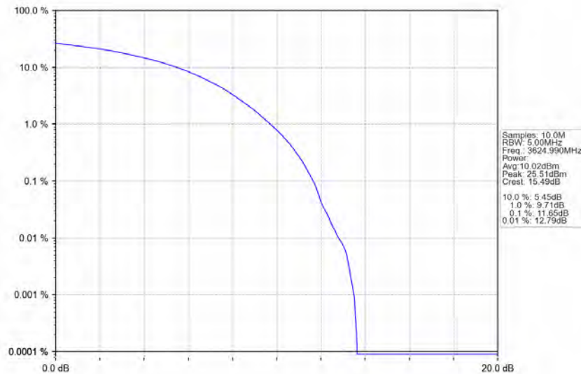
n78d_30kHz_MIMO_NTNV_40MHz_CP-OFDM_64_QAM_3624.99MHz_Outer_Full
