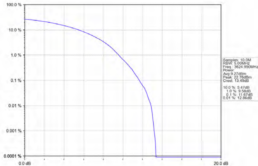
n78d_30kHz_MIMO_NTNV_50MHz_CP-OFDM_16_QAM_3624.99MHz_Outer_Full
