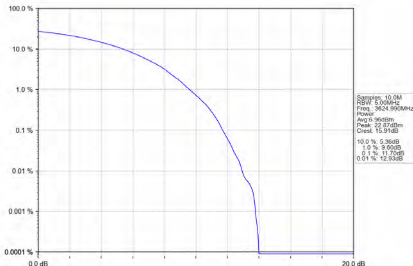
n78d_30kHz_MIMO_NTNV_80MHz_CP-OFDM QPSK_3624.99MHz_Outer_Full
