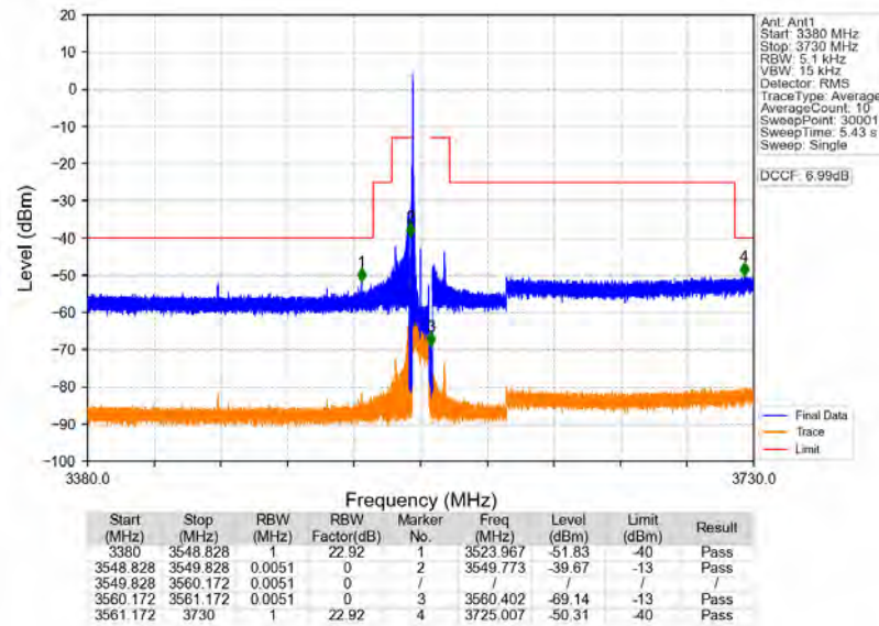
n78d 30kHz MIMO_NTNV_10MHz_CP-OFDM QPSK 3555MHz Edge_1RB Left
