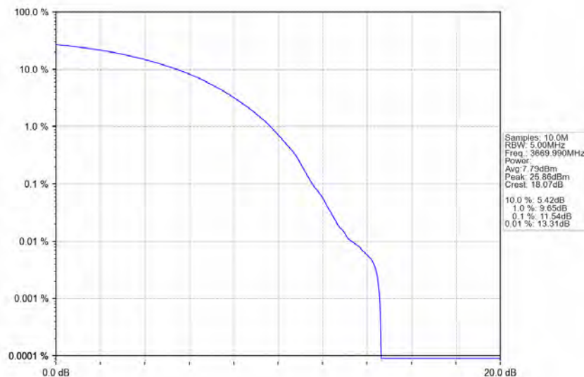
n78d_30kHz_MIMO_NTNV_60MHz_CP-OFDM QPSK_3669.99MHz_Outer_Full
