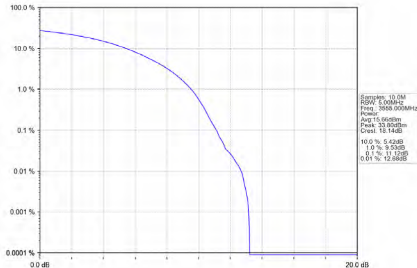
n78d_30kHz_MIMO_NTNV_10MHz_CP-OFDM_64_QAM_3555MHz_Outer_Full
