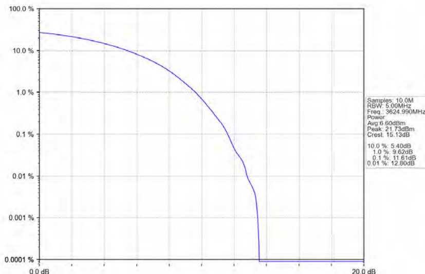
n78d_30kHz_MIMO_NTNV_90MHz_CP-OFDM QPSK_3624.99MHz_Outer_Full
