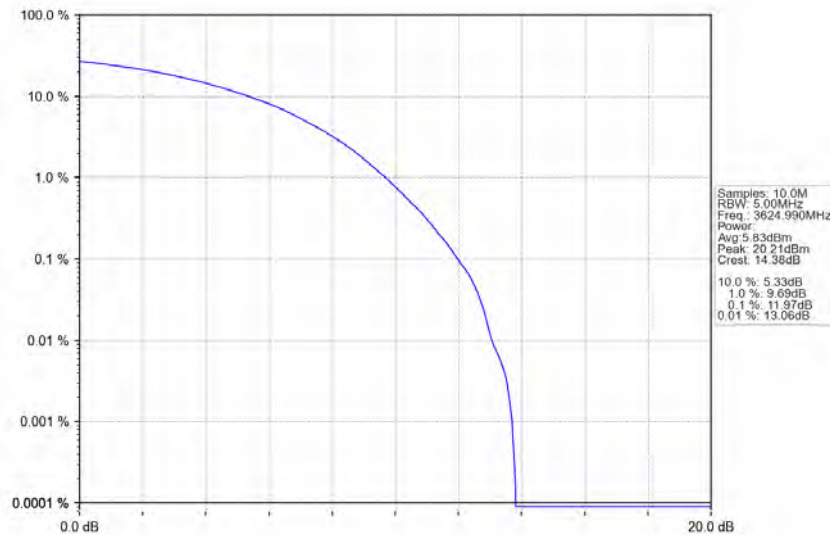
n78d_30kHz_MIMO_NTNV_50MHz_CP-OFDM_256_QAM_3624.99MHz_Outer_Full
