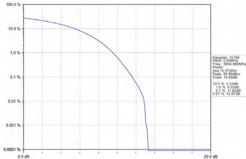
n78d_30kHz_MIMO_NTNV_10MHz_CP-OFDM_QPSK_3694.98MHz_Outer_Full
