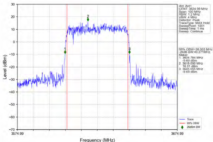
n78d_30kHz_MIMO_NTNV_40MHz_CP-OFDM_256_QAM_3624.99MHz_Outer_Full
