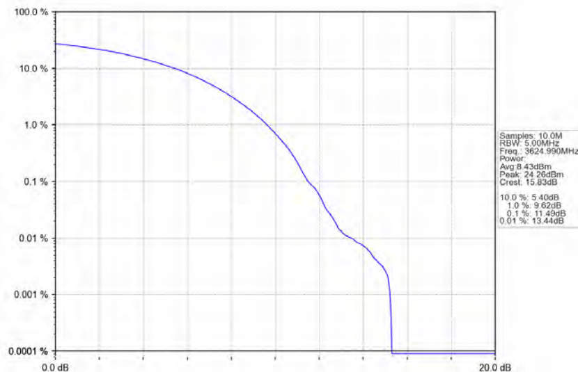
n78d_30kHz_MIMO_NTNV_60MHz_CP-OFDM QPSK_3624.99MHz_Outer_Full
