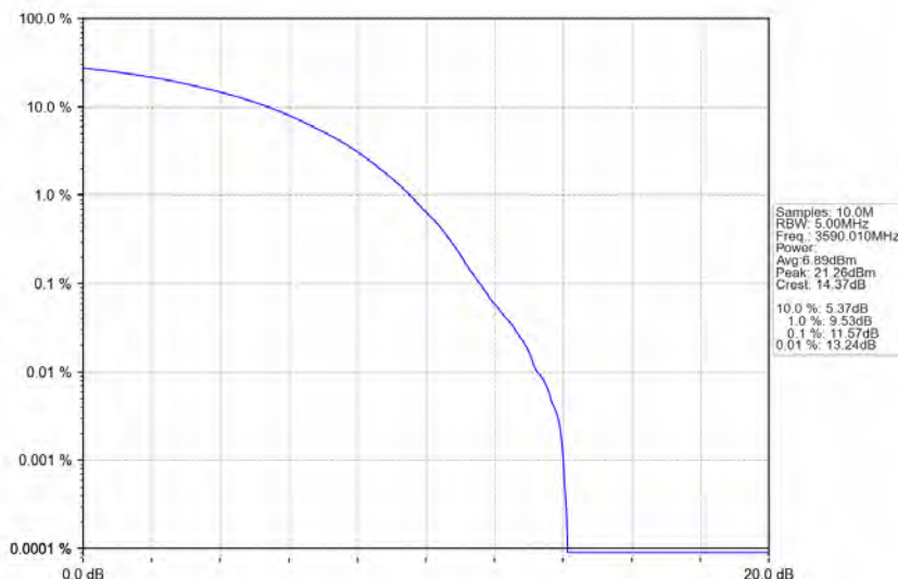
n78d_30kHz_MIMO_NTNV_80MHz_CP-OFDM_16_QAM_3590.01MHz_Outer_Full
