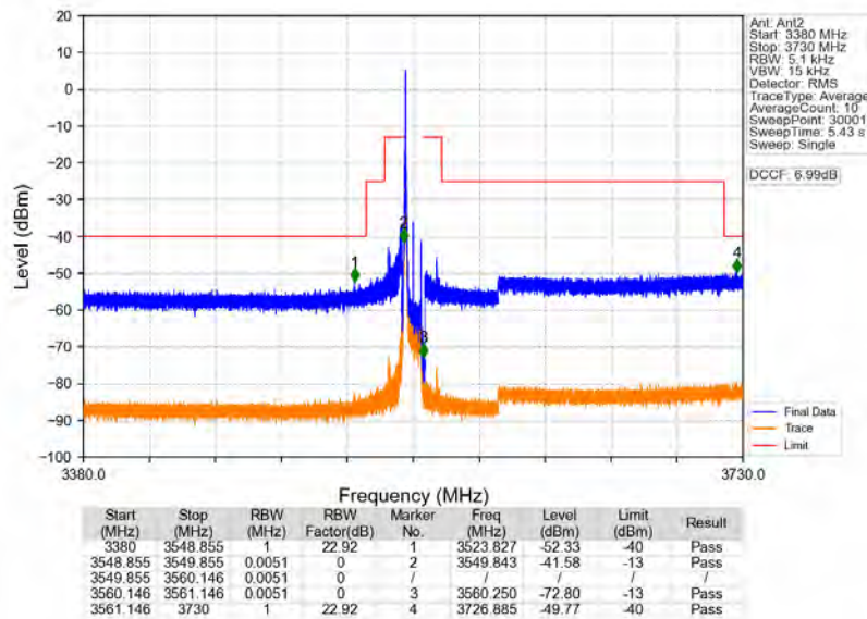
n78d_30kHz_MIMO_NTNV_10MHz_CP-OFDM_QPSK_3555MHz_Edge_1RB_Left
