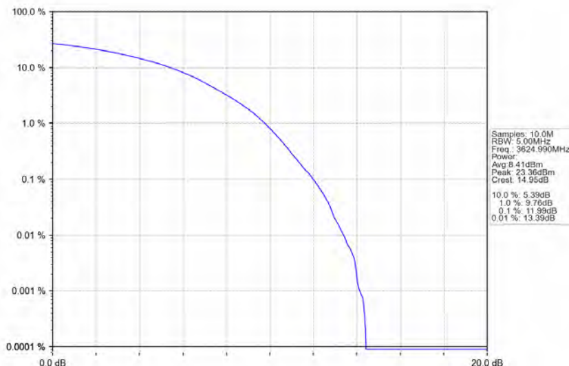
n78d_30kHz_MIMO_NTNV_60MHz_CP-OFDM_16_QAM_3624.99MHz_Outer_Full
