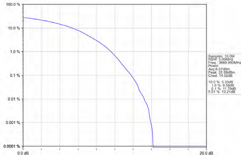
n78d_30kHz_MIMO_NTNV_60MHz_CP-OFDM_16_QAM_3669.99MHz_Outer_Full
