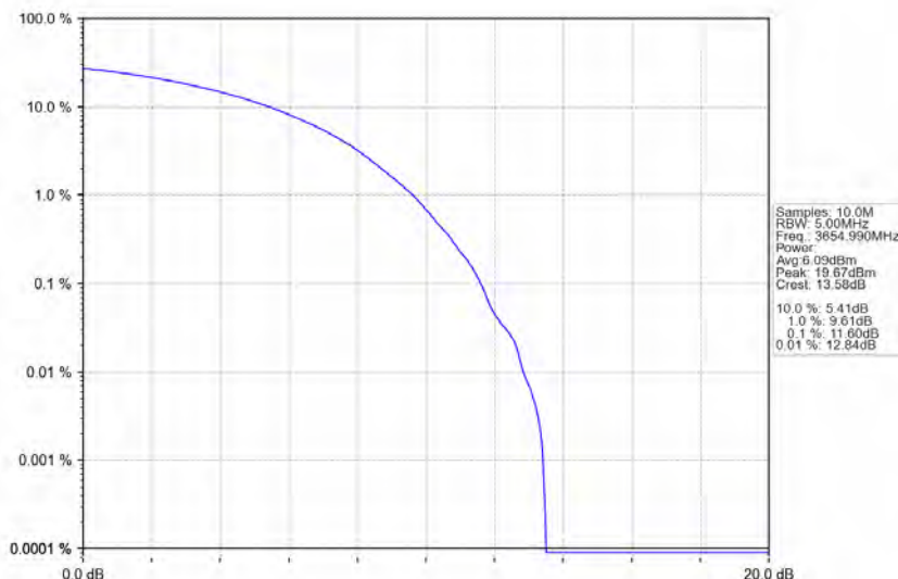
n78d_30kHz_MIMO_NTNV_90MHz_CP-OFDM QPSK_3654.99MHz_Outer_Full
