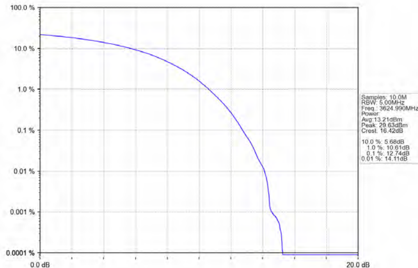
n78d_30kHz_MIMO_NTNV_20MHz_CP-OFDM_16_QAM_3624.99MHz_Outer_Full
