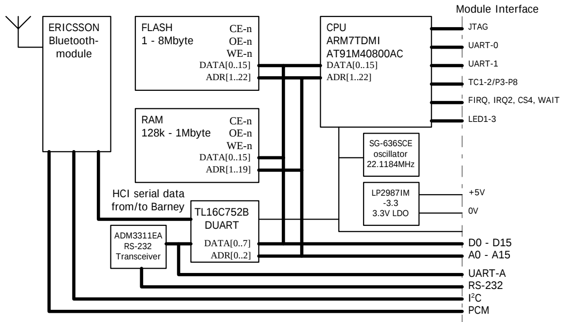
Figure 1 Block diagram of connectBlue design cB0005-01 OEM-Bluetooth module
