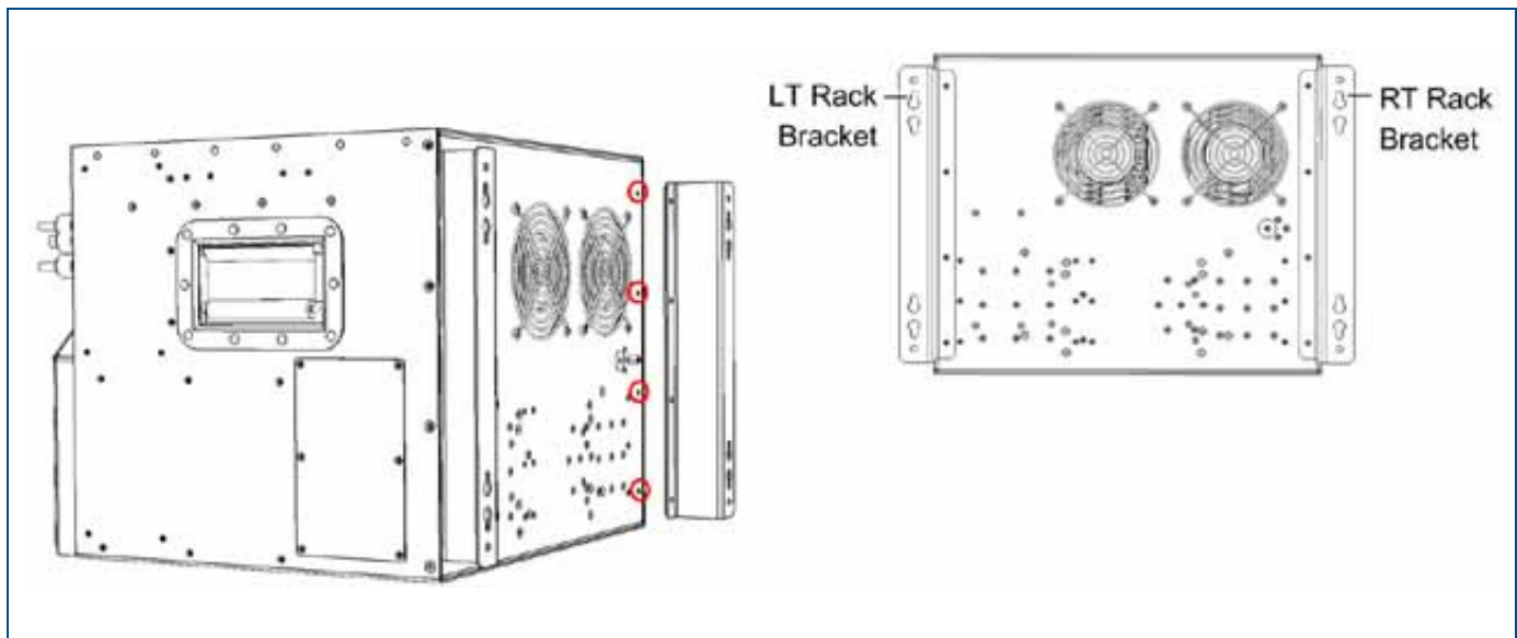
HX Indoor Unit with Assembled Wall-Mount Brackets | Figure 3-3
