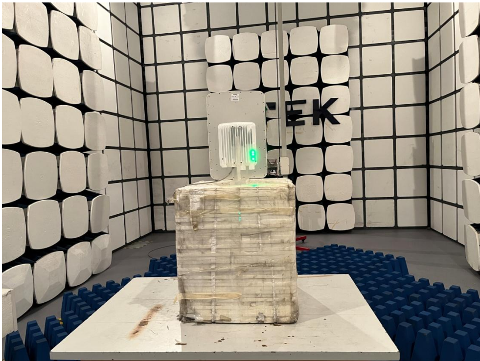
Radiated Measurement Photos 1GHz~18GHz
