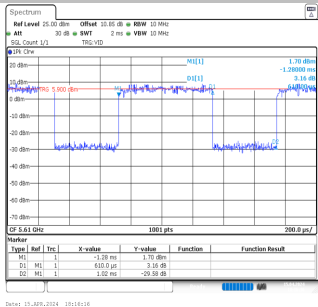
NTVN-11AX80MIMO-Ant2-5610
