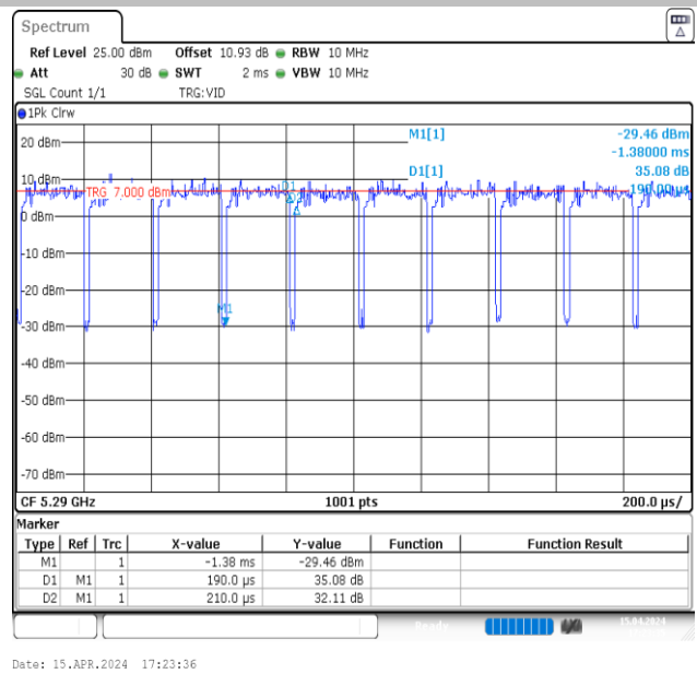
NTVN-11AC80MIMO-Ant2-5290
