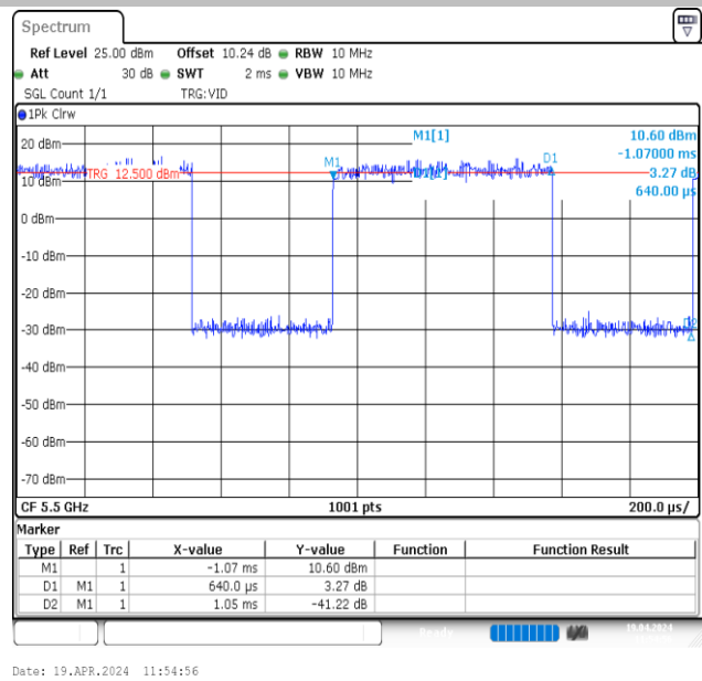
NTVN-11AX20MIMO-Ant2-5500
