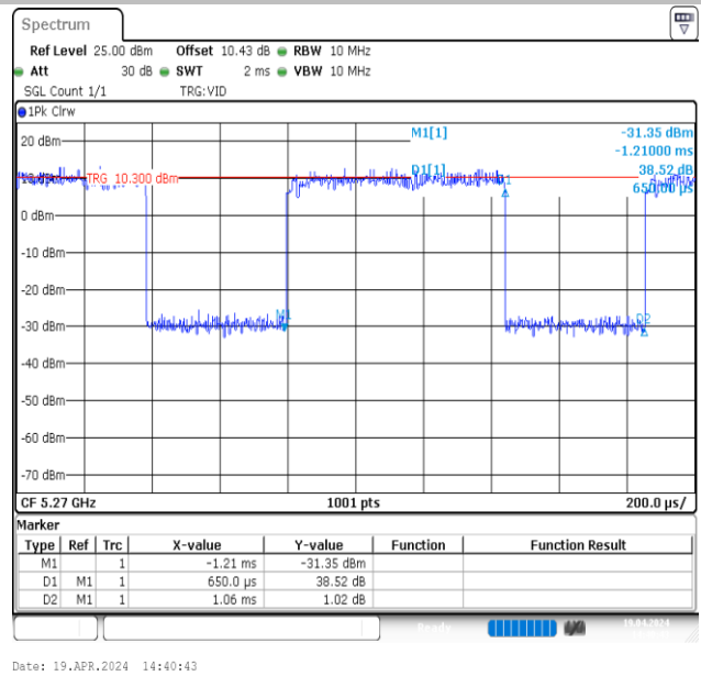
NTVN-11AX40MIMO-Ant2-5270
