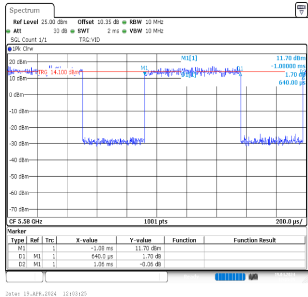
NTVN-11AX20MIMO-Ant2-5580
