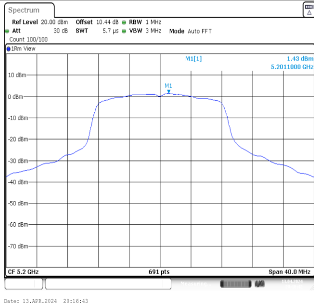
11A-Ant1-5200-PASS
