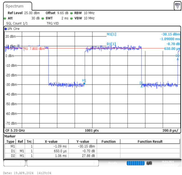
NTVN-11AX40MIMO-Ant2-5230
