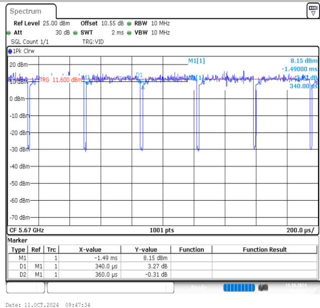
NTNV-11AC40MIMO-Ant2-5670
