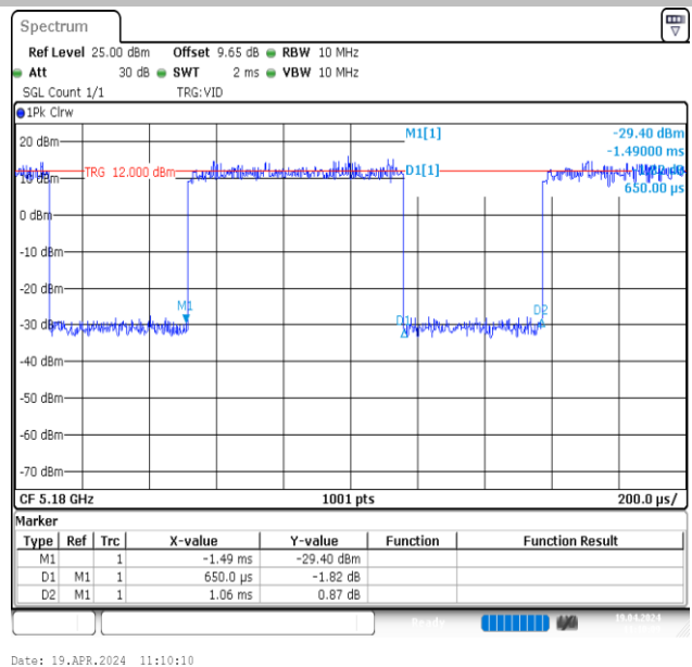
NTVN-11AX20MIMO-Ant2-5180
