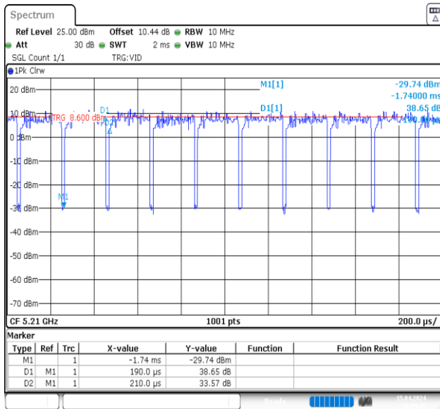
NTVN-11AC80MIMO-Ant1-5210
