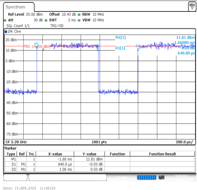
NTVN-11AX20MIMO-Ant2-5280
