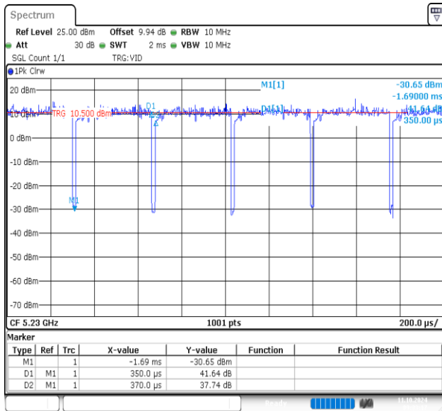
NTVN-11AC40MIMO-Ant1-5230
