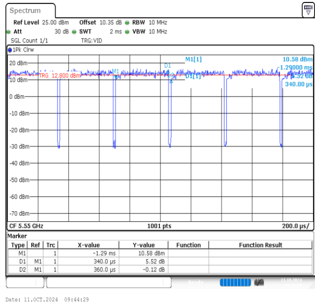
NTNV-11AC40MIMO-Ant2-5550
