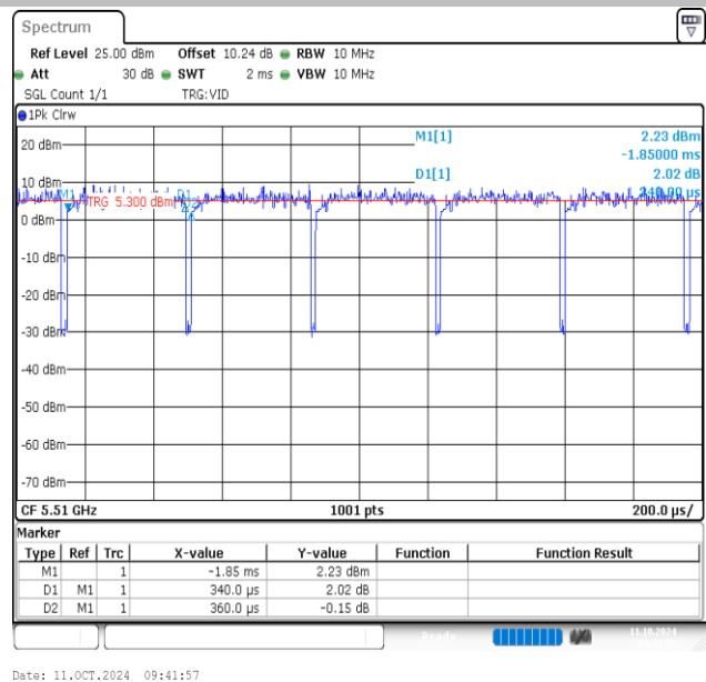
NTVN-11AC40MIMO-Ant2-5510
