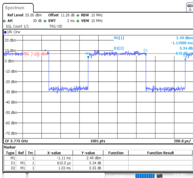
NTNV-11AX80MIMO-Ant1-5775
