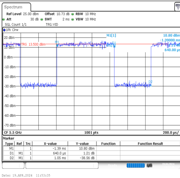
NTVN-11AX20MIMO-Ant1-5500
