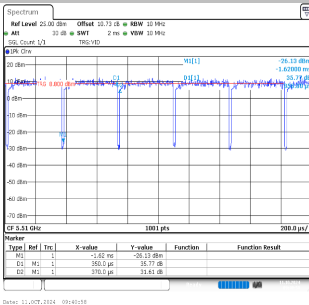
NTVN-11AC40MIMO-Ant1-5510
