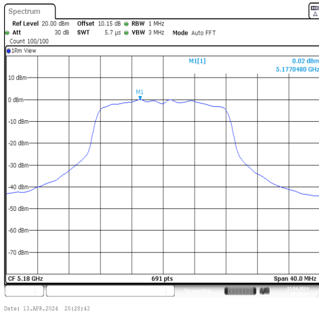
11A-Ant2-5180-PASS
