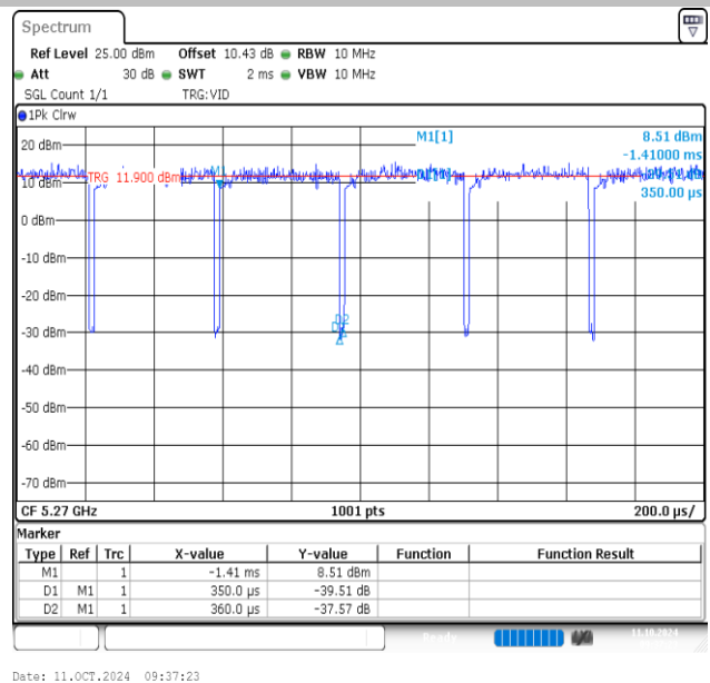
NTVN-11AC40MIMO-Ant2-5270
