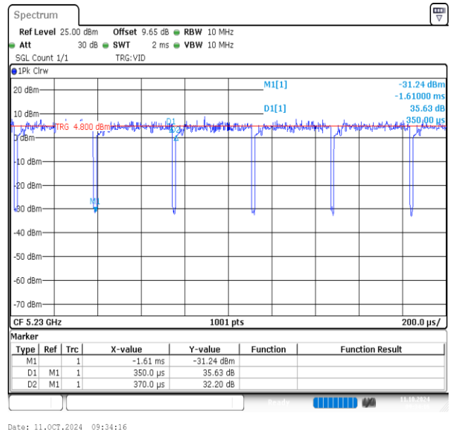
NTVN-11AC40MIMO-Ant2-5230
