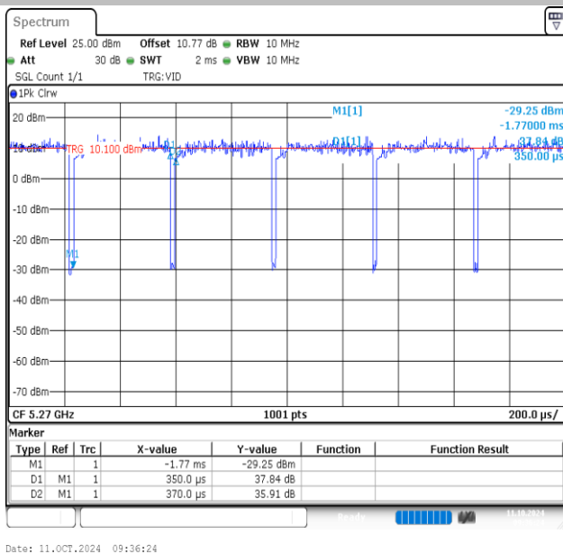
NTVN-11AC40MIMO-Ant1-5270
