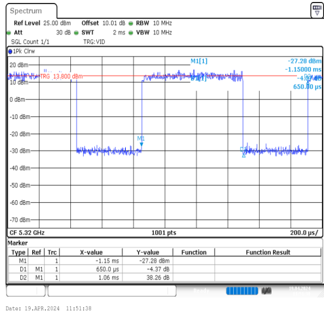
NTVN-11AX20MIMO-Ant2-5320
