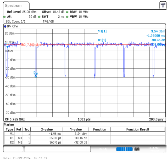
NTVN-11AC40MIMO-Ant2-5755
