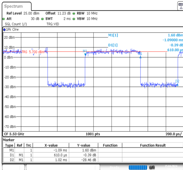
NTVN-11AX80MIMO-Ant1-5530
