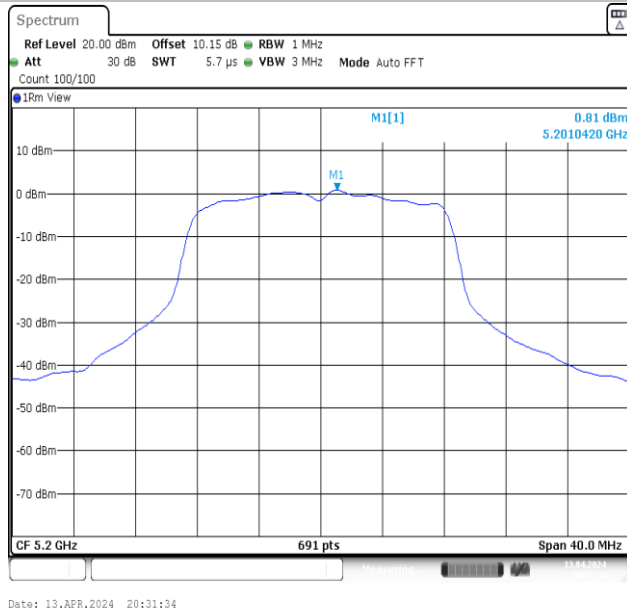
11A-Ant2-5200-PASS
