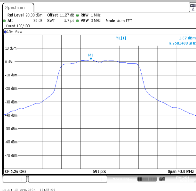
11A-Ant1-5260-PASS
