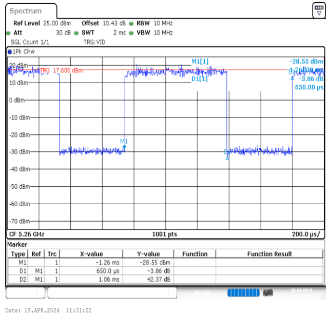
NTVN-11AX20MIMO-Ant2-5260
