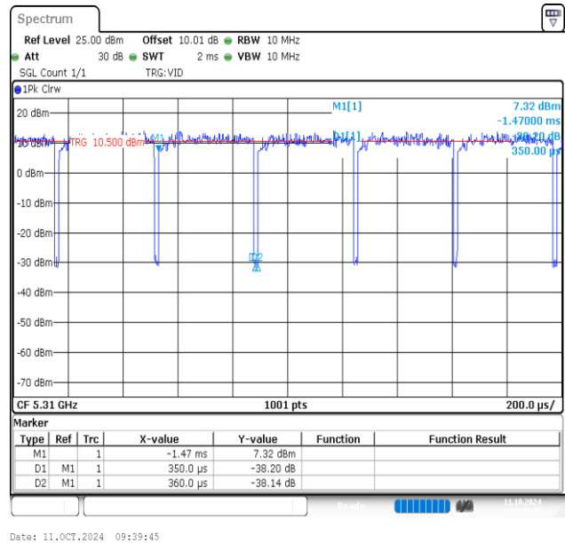
NTVN-11AC40MIMO-Ant2-5310
