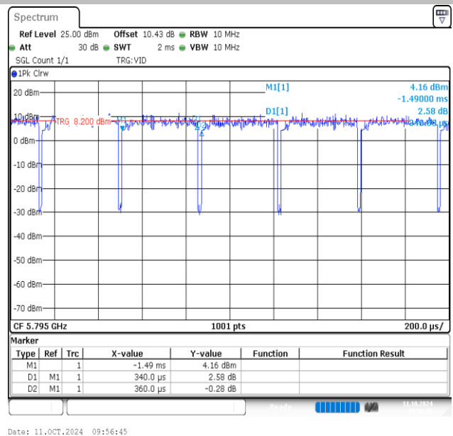
NTVN-11AC40MIMO-Ant2-5795
