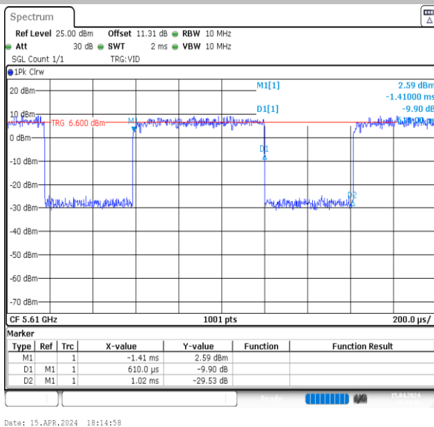
NTVN-11AX80MIMO-Ant1-5610
