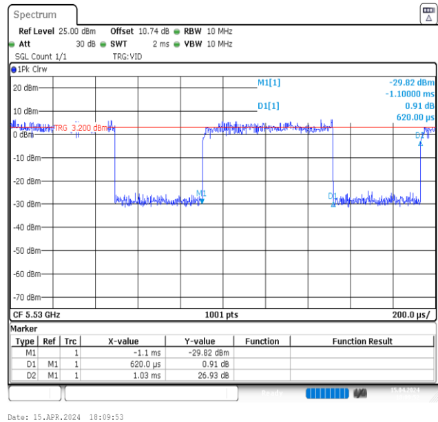
NTVN-11AX80MIMO-Ant2-5530
