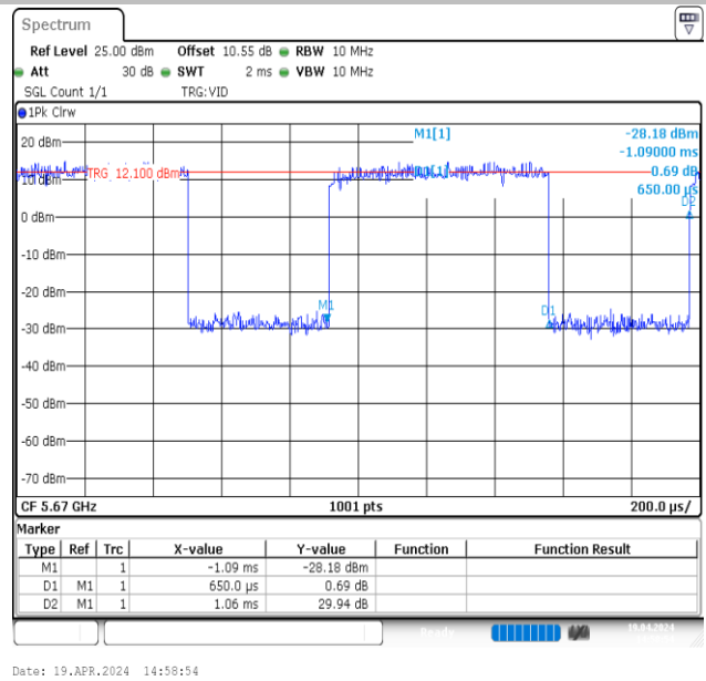
NTNV-11AX40MIMO-Ant2-5670
