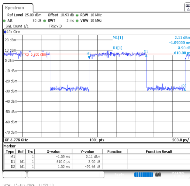
NTNV-11AX80MIMO-Ant2-5775
