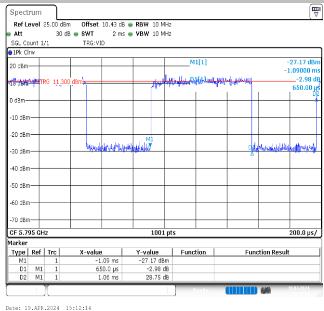
NTVN-11AX40MIMO-Ant2-5795
