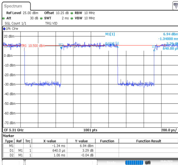
NTVN-11AX40MIMO-Ant1-5310
