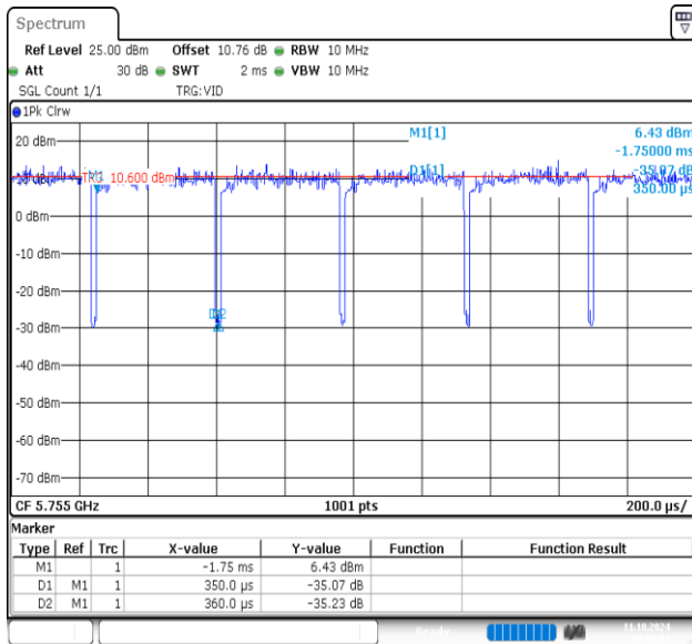
NTVN-11AC40MIMO-Ant1-5755
