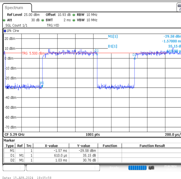
NTVN-11AX80MIMO-Ant2-5290
