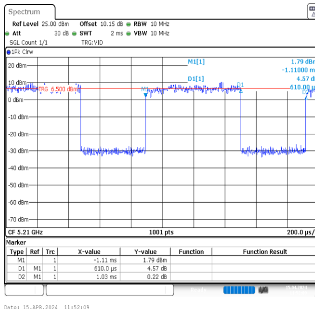
NTVN-11AX80MIMO-Ant2-5210
