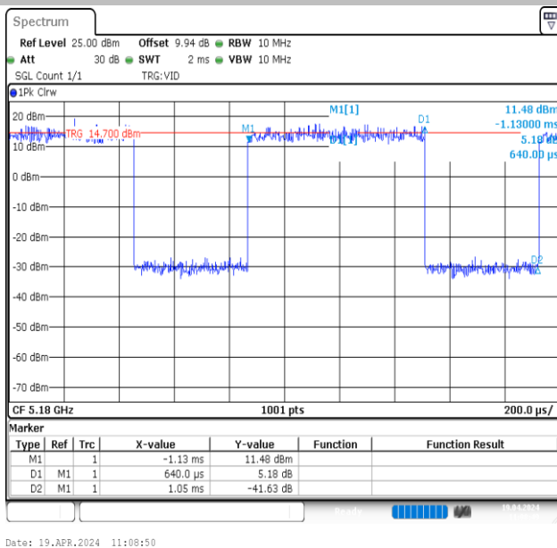
NTVN-11AX20MIMO-Ant1-5180
