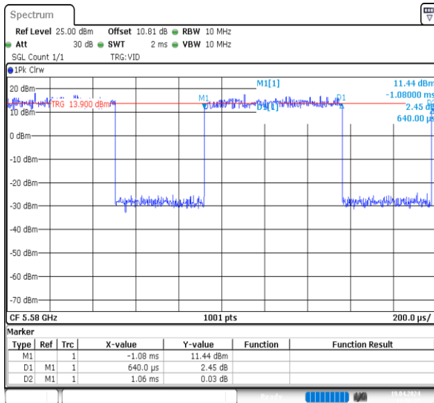
NTVN-11AX20MIMO-Ant1-5580
