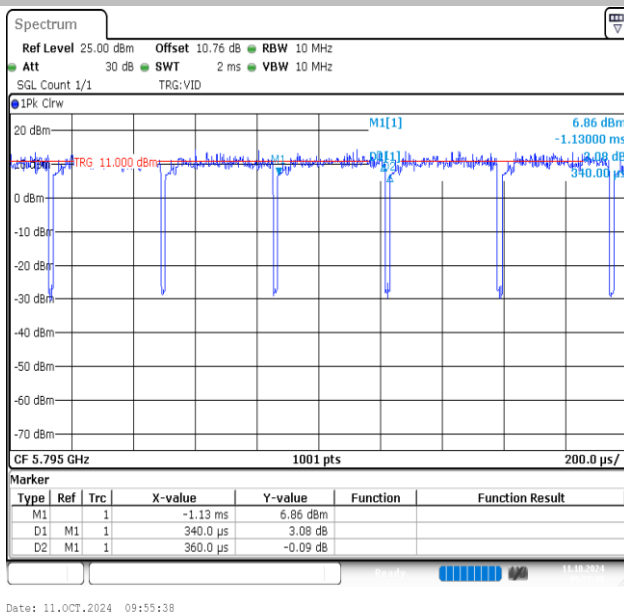
NTVN-11AC40MIMO-Ant1-5795
