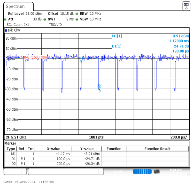
NTVN-11AC80MIMO-Ant2-5210
