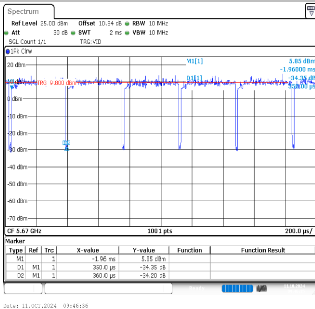
NTNV-11AC40MIMO-Ant1-5670
