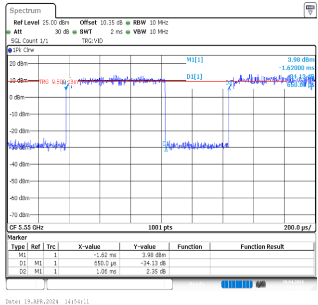
NTNV-11AX40MIMO-Ant2-5550
