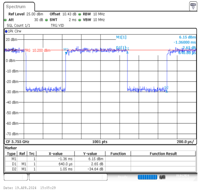
NTVN-11AX40MIMO-Ant2-5755
