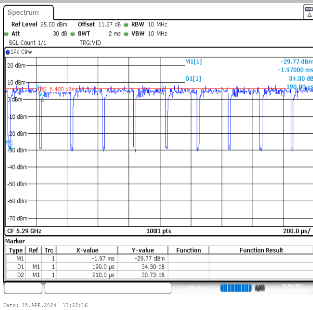
NTVN-11AC80MIMO-Ant1-5290
