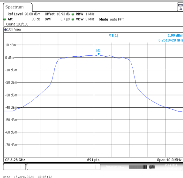
11A-Ant2-5260-PASS
