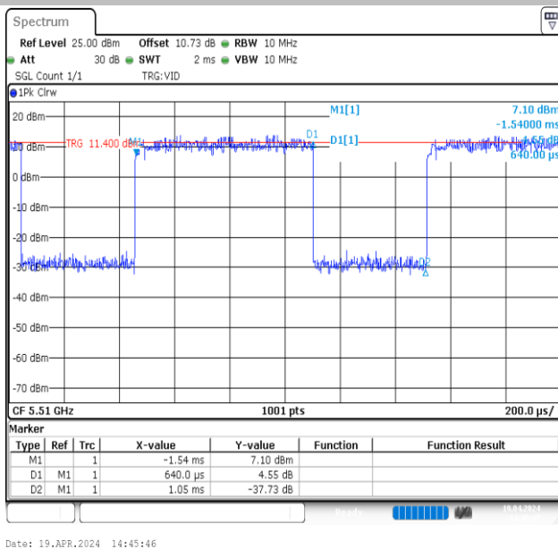
NTVN-11AX40MIMO-Ant1-5510
