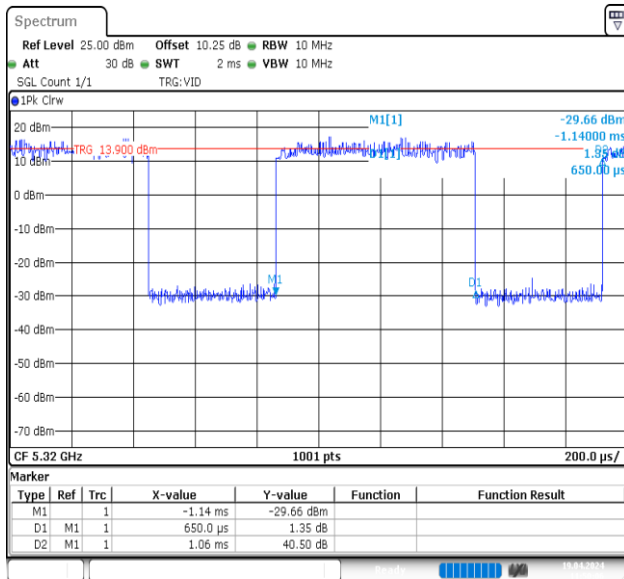
NTVN-11AX20MIMO-Ant1-5320
