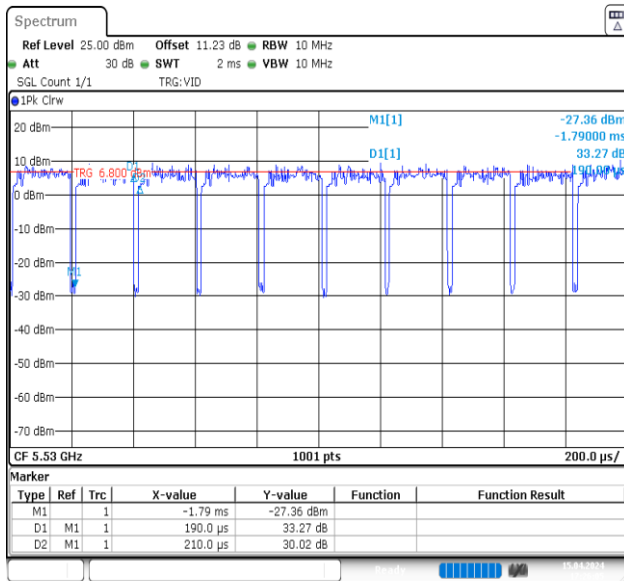
NTVN-11AC80MIMO-Ant1-5530
