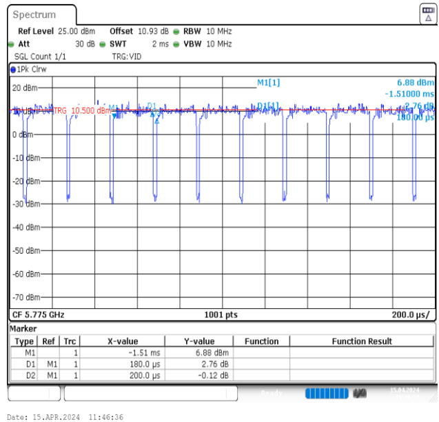
NTVN-11AC80MIMO-Ant2-5775
