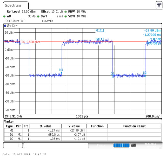
NTVN-11AX40MIMO-Ant2-5310
