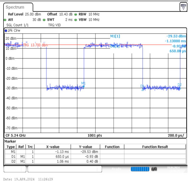
NTNV-11AX20MIMO-Ant2-5240
