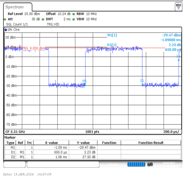
NTVN-11AX40MIMO-Ant2-5510
