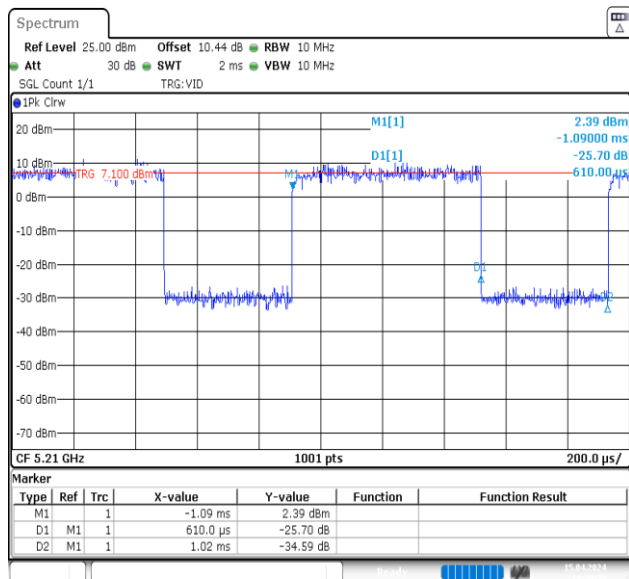
NTVN-11AX80MIMO-Ant1-5210
