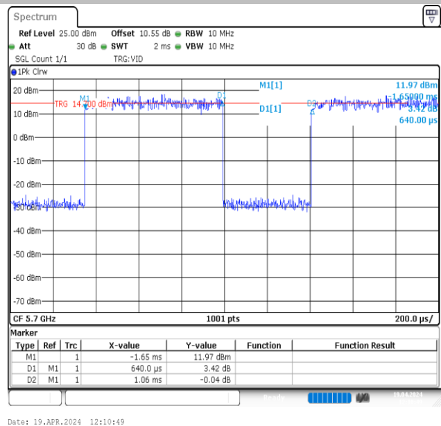
NTVN-11AX20MIMO-Ant2-5700
