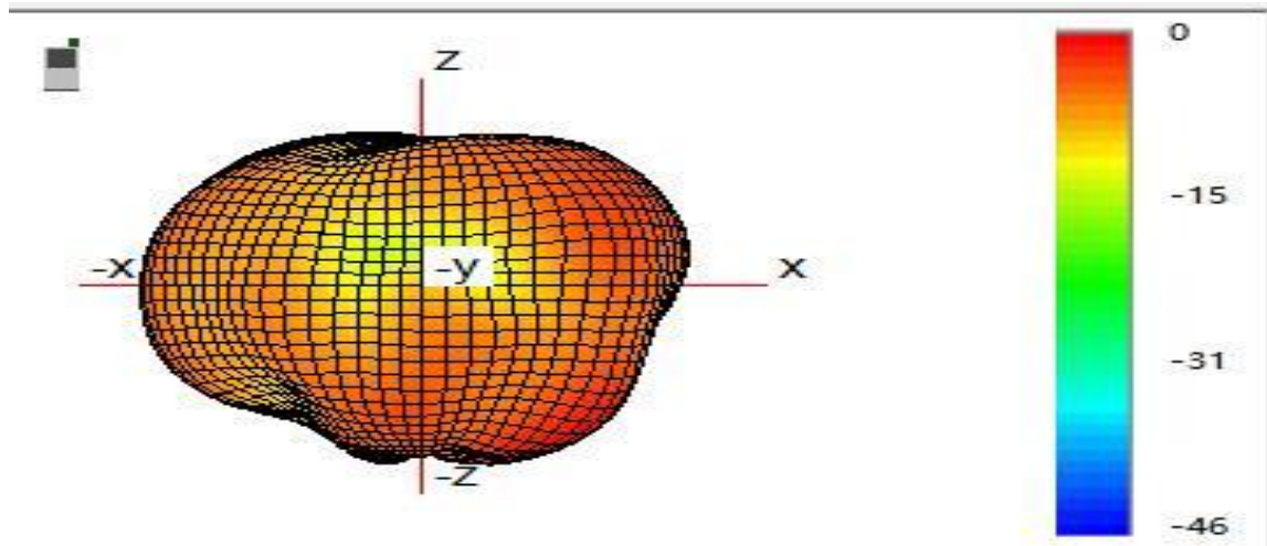
(4) Typical Free Space 3D Radiation Pattern at 2.5GHz(unit:dBi):
