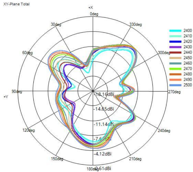
(3) X-Y Plane(unit:dBi):
