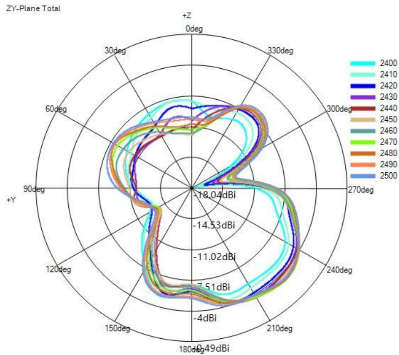
(2) Y-Z Plane(unit:dBi):
