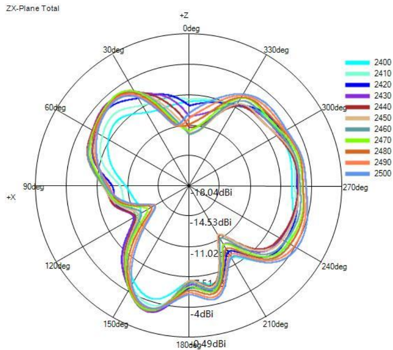
(1) X-Z Plane(unit:dBi):
