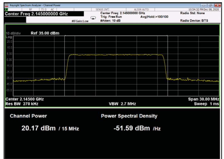
Figure 94: 64QAM 15MHz B.W.; 2145MHz, 30kHz
