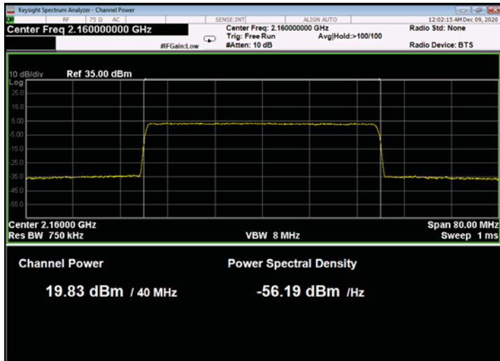
Figure 123: 64QAM 40MHz B.W.; 2160.0MHz, 15kHz
