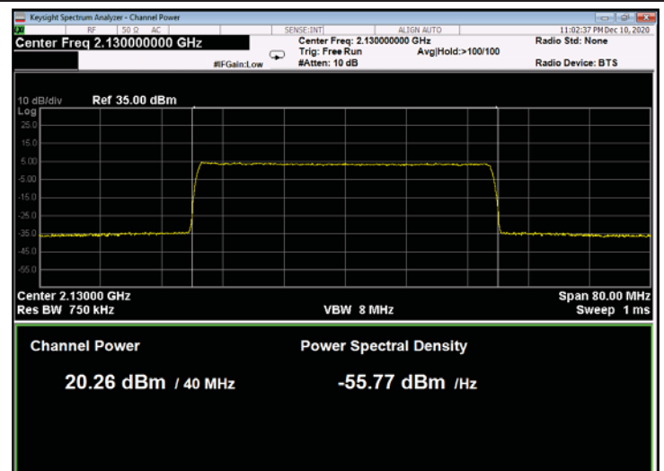
Figure 184: 256QAM 40MHz B.W.; 2130.0MHz, 30kHz
