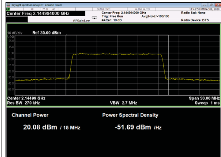
Figure 95: 64QAM 15MHz B.W.; 2145MHz, 60kHz
