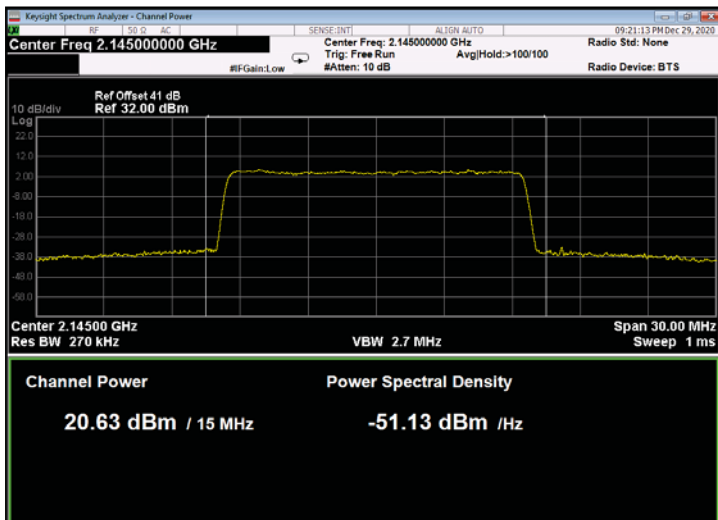
Figure 161: 256QAM 15MHz B.W.; 2145.0MHz, 60kHz
