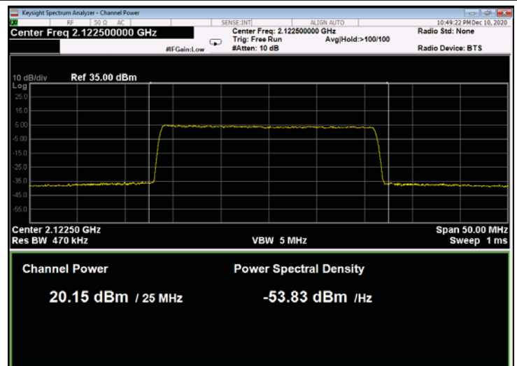
Figure 176: 256QAM 25MHz B.W.; 2122.5MHz, 60kHz
