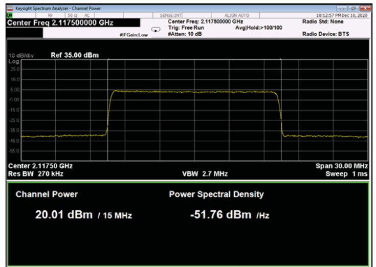
Figure 156: 256QAM 15MHz B.W.; 2117.5MHz, 15kHz
