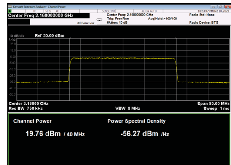
Figure 189: 256QAM 40MHz B.W.; 2160.0MHz, 15kHz
