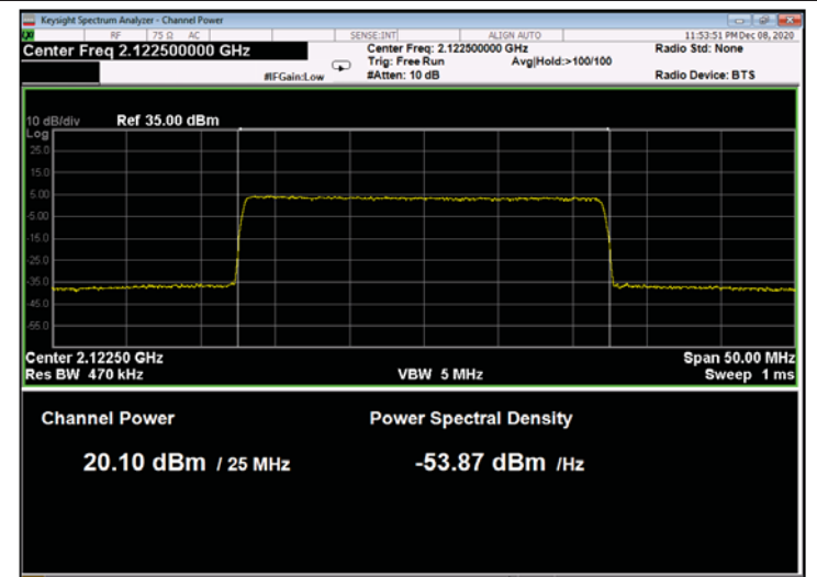
Figure 108: 64QAM 25MHz B.W.; 2122.5MHz, 15kHz
