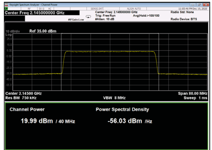
Figure 188: 256QAM 40MHz B.W.; 2145.0MHz, 60kHz
