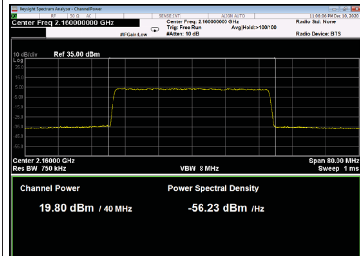
Figure 191: 256QAM 40MHz B.W.; 2160.0MHz, 60kHz
