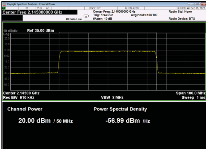
Figure 129: 64QAM 50MHz B.W.; 2145.0MHz, 15kHz
