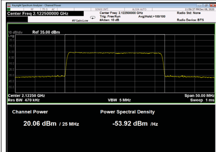
Figure 109: 64QAM 25MHz B.W.; 2122.5MHz, 30kHz
