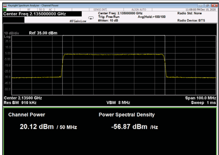
Figure 192: 256QAM 50MHz B.W.; 2135.0MHz, 15kHz
