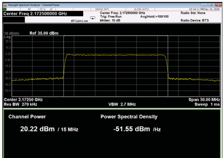
Figure 162: 256QAM 15MHz B.W.; 2172.5MHz, 15kHz
