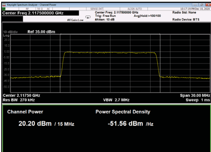
Figure 157: 256QAM 15MHz B.W.; 2117.5MHz, 30kHz
