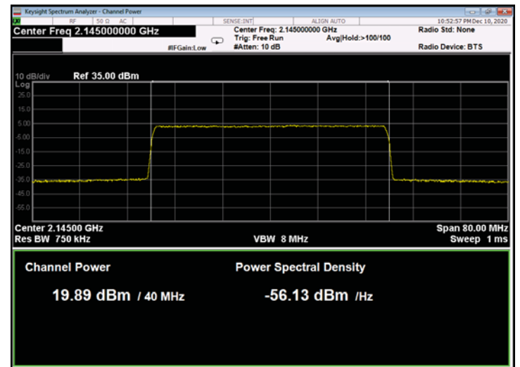
Figure 186: 256QAM 40MHz B.W.; 2145.0MHz, 15kHz
