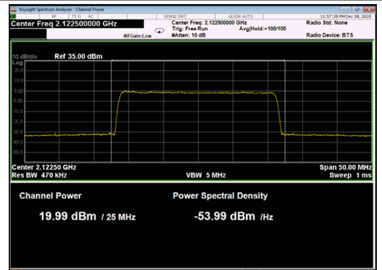
Figure 110: 64QAM 25MHz B.W.; 2122.5MHz, 60kHz
