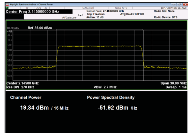
Figure 93: 64QAM 15MHz B.W.; 2145MHz, 15kHz
