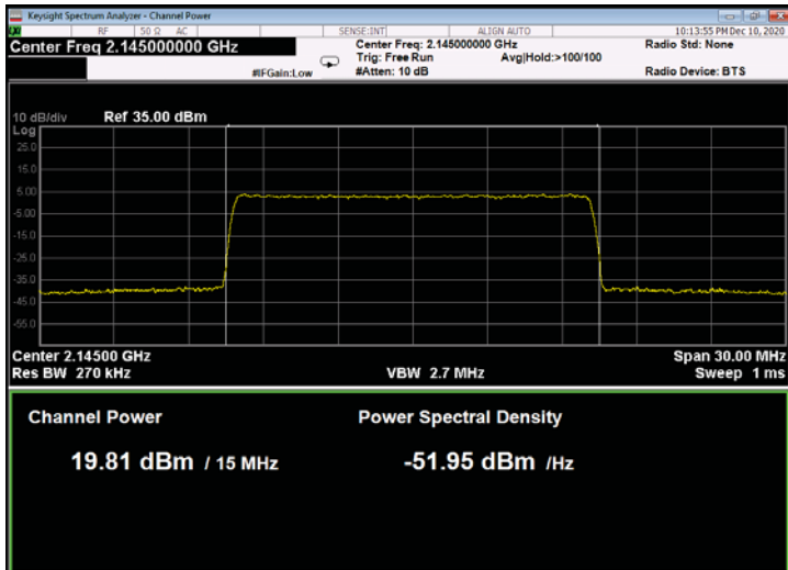
Figure 159: 256QAM 15MHz B.W.; 2145.0MHz, 15kHz
