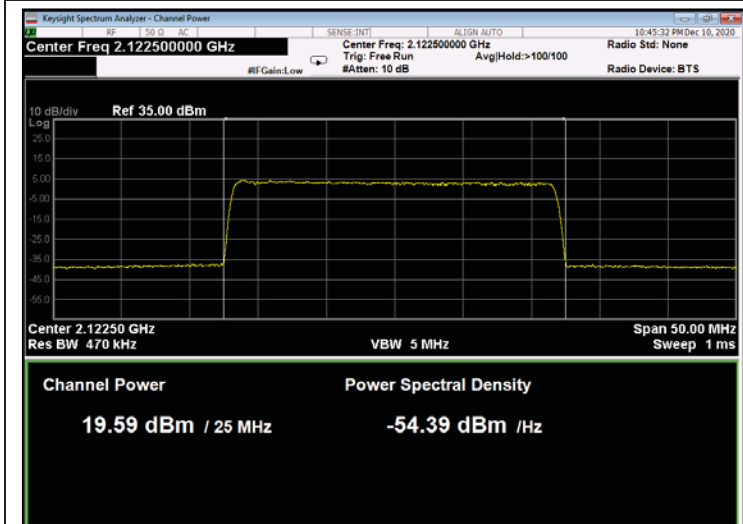
Figure 175: 256QAM 25MHz B.W.; 2122.5MHz, 30kHz
