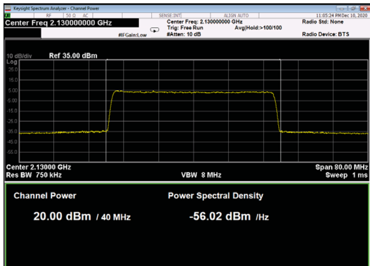
Figure 185: 256QAM 40MHz B.W.; 2130.0MHz, 60kHz
