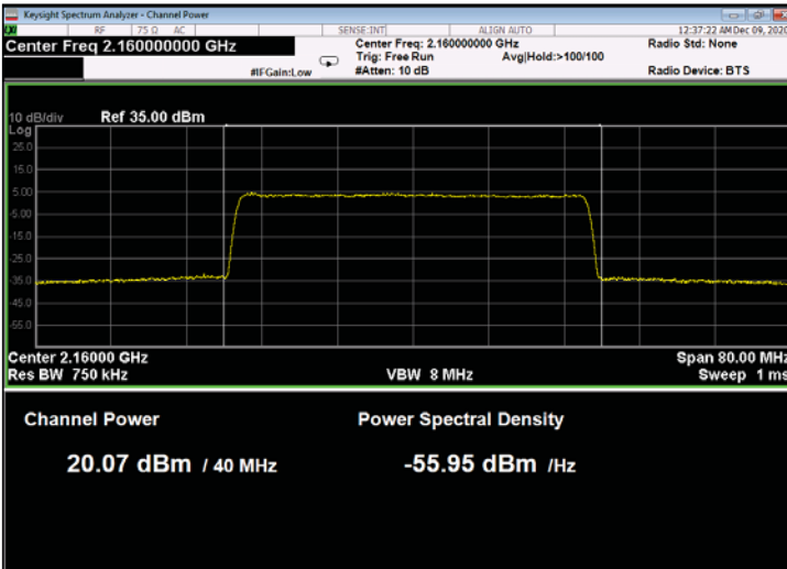
Figure 125: 64QAM 40MHz B.W.; 2160.0MHz, 60kHz
