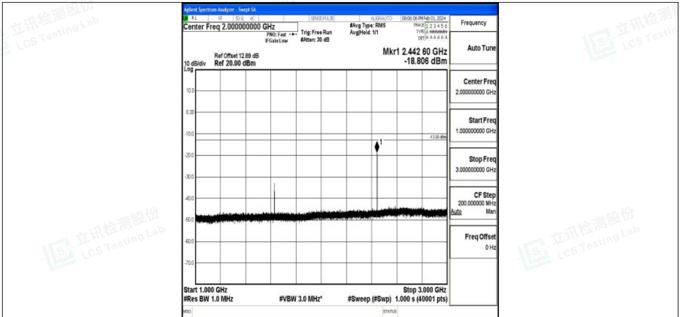
Band26_1.4MHz_16QAM_26697_1RB#0_1000~3000_1000~3000
