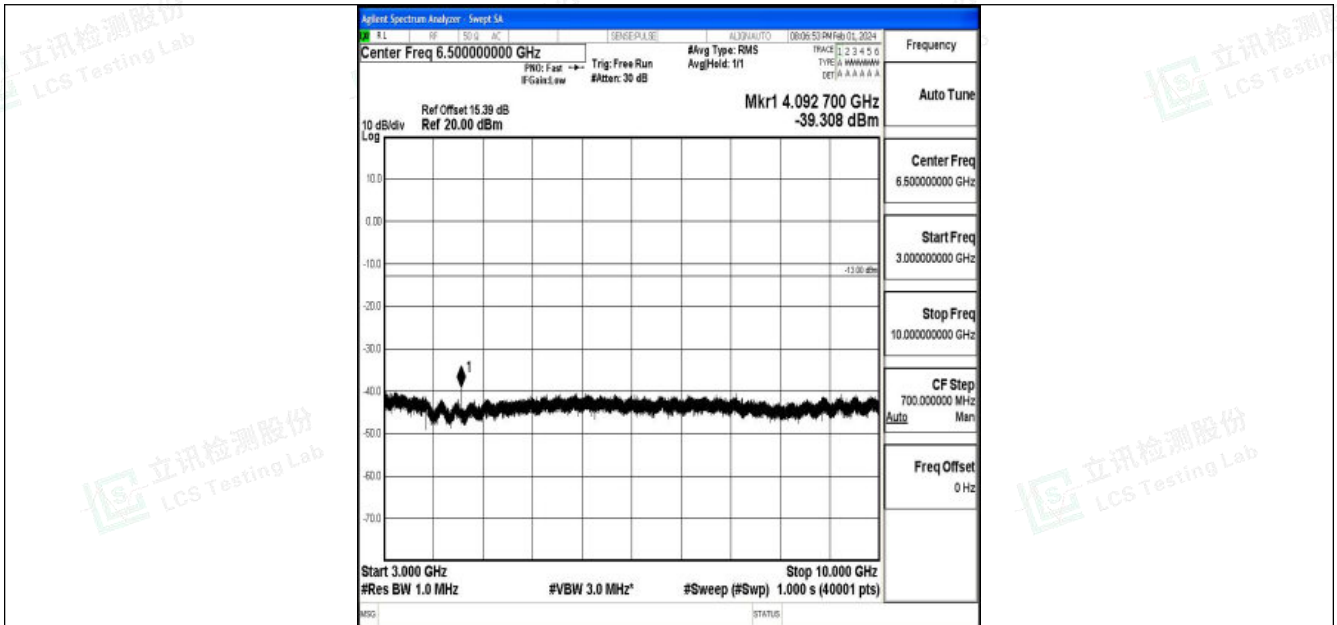
Band26_1.4MHz_QPSK_26740_1RB#0_3000~10000_3000~10000
