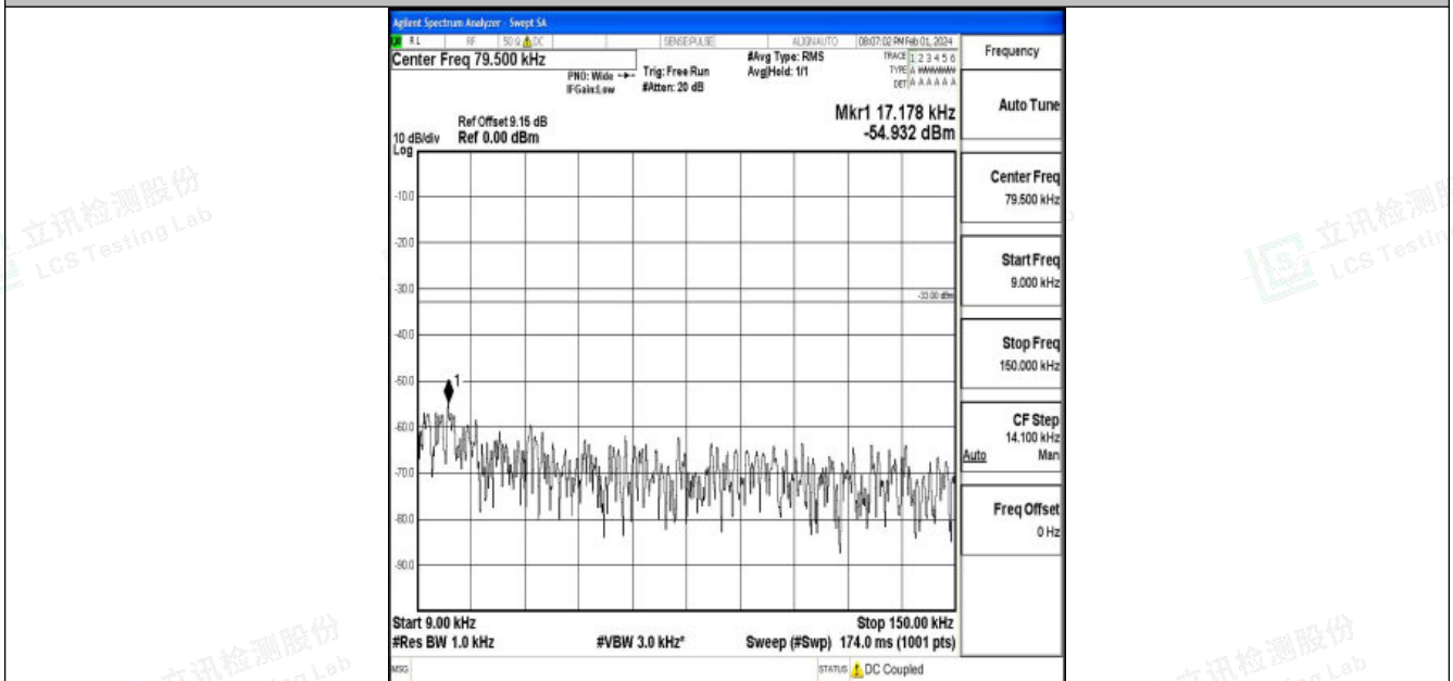
Band26_1.4MHz_16QAM_26740_1RB#0_0.009~0.15_0.009~0.15
