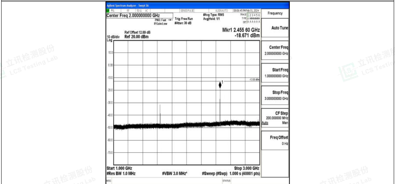
Band26_1.4MHz_QPSK_26740_1RB#0_1000~3000_1000~3000
