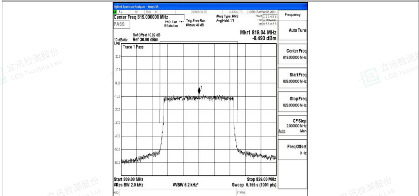
Band26_10MHz_QPSK_26740_50RB#0
