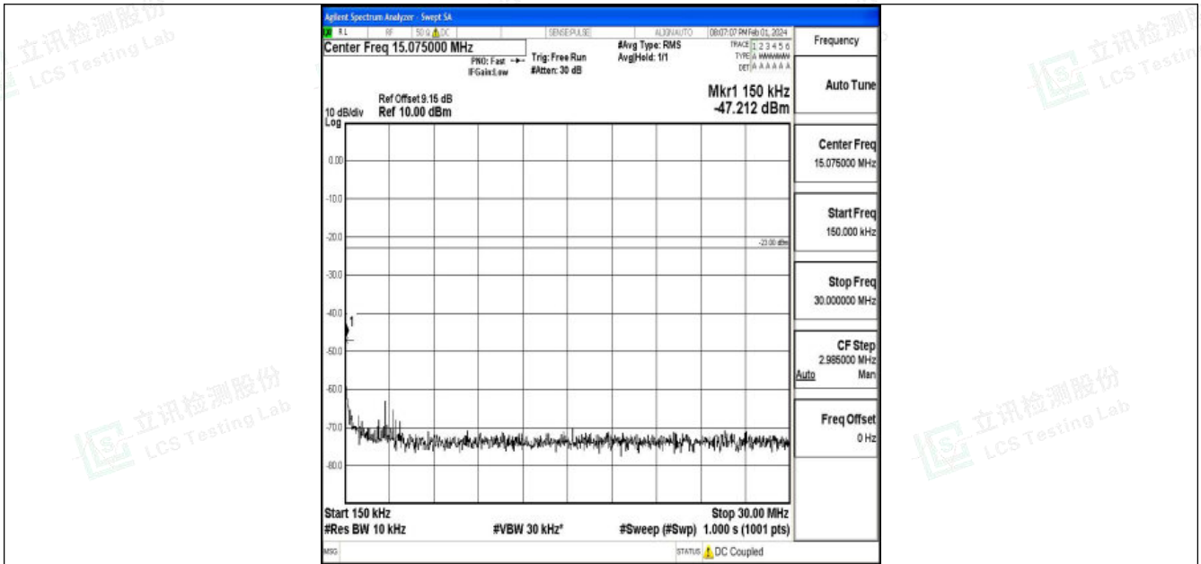
Band26_1.4MHz_16QAM_26740_1RB#0_0.15~30_0.15~30
