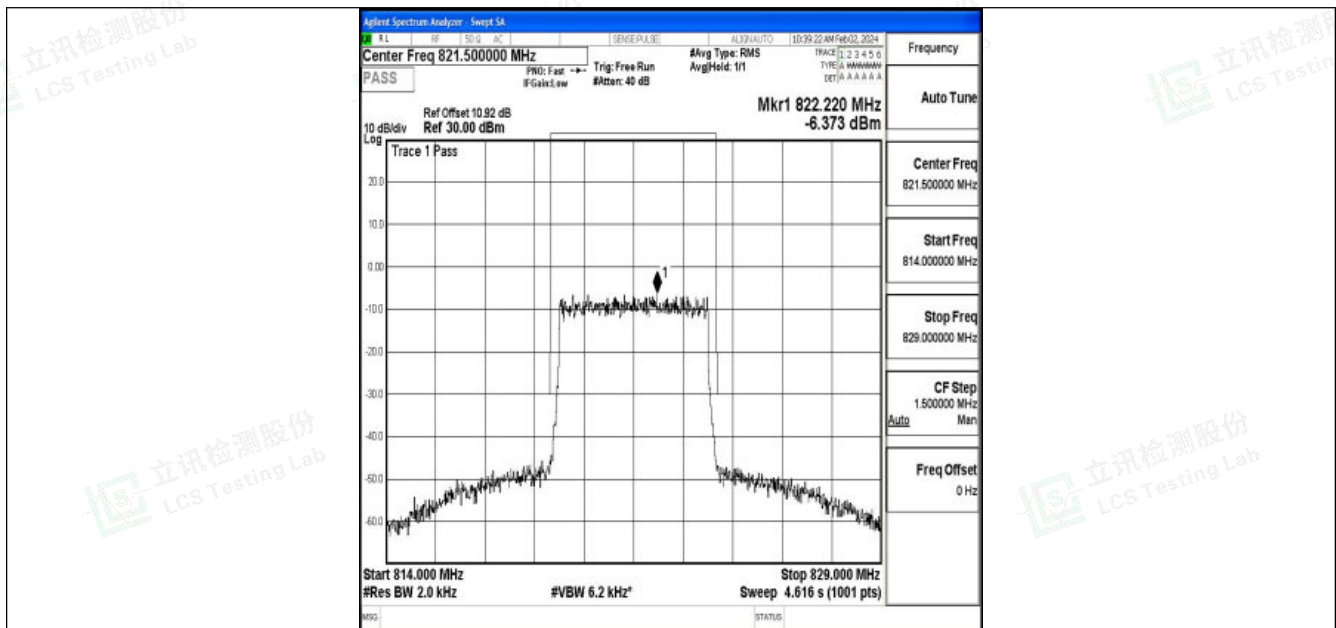
Band26_5MHz_16QAM_26765_25RB#0
