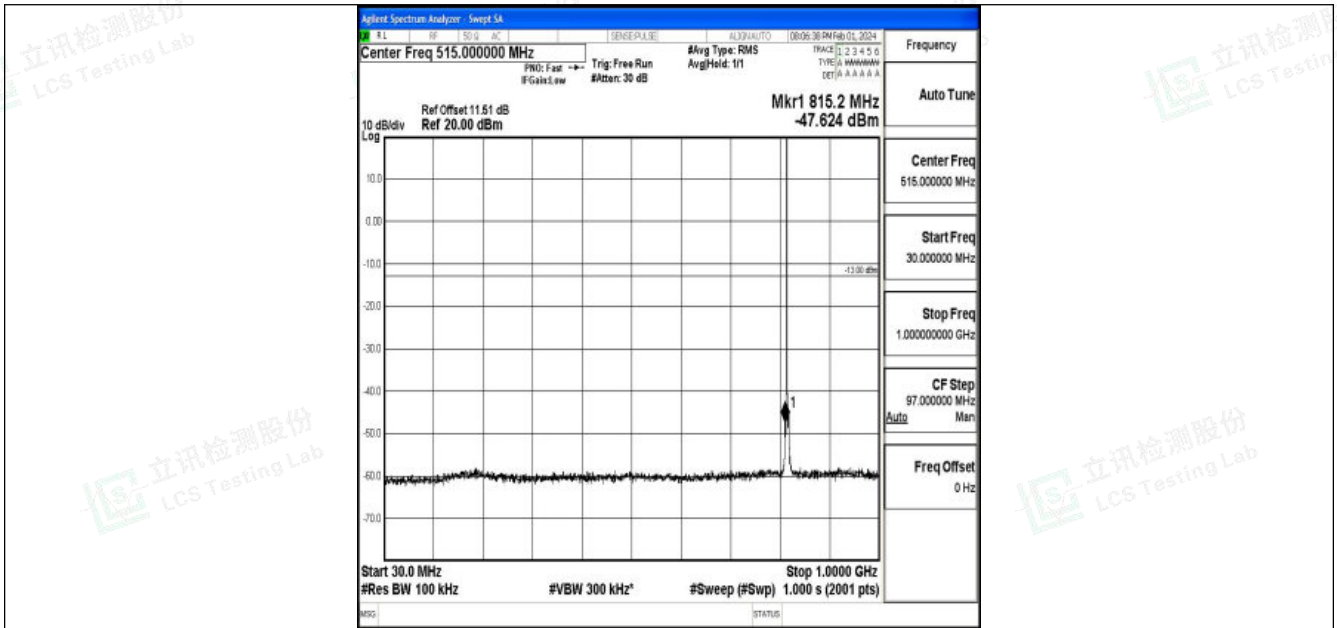
Band26_1.4MHz_QPSK_26740_1RB#0_30~1000_30~1000
