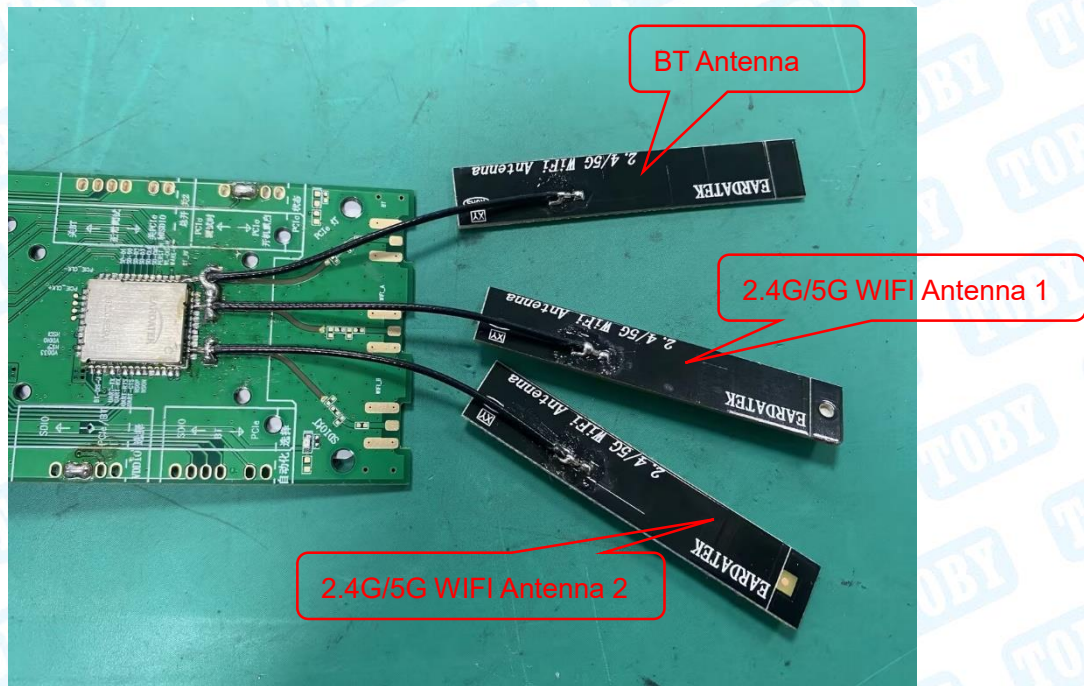
Photo 2 Appearance of PCB
