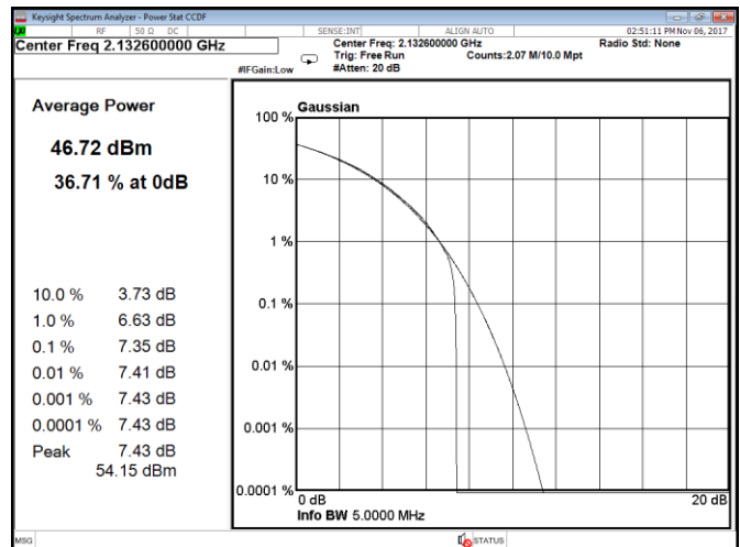
Figure 8.1-224: CCDF, QPSK, WCDMA, Port C, mid channel
