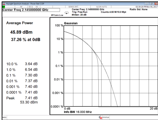
Figure 8.1-197: CCDF, QPSK, 15 MHz, LTE, Port B, mid channel
