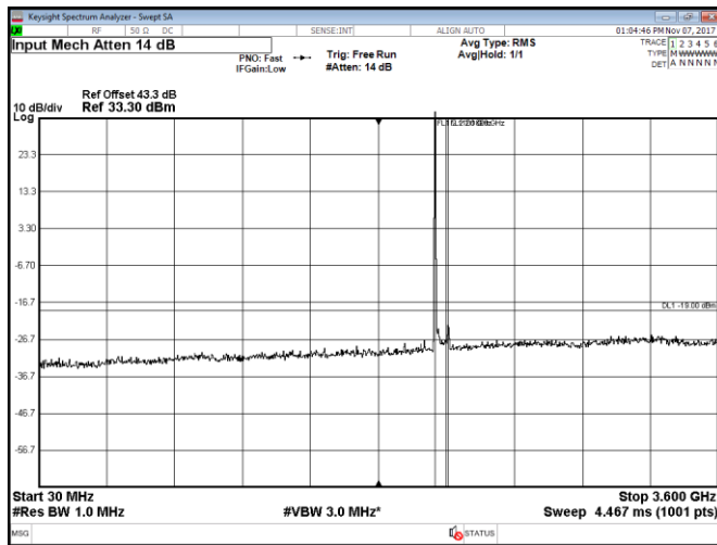
Figure 8.2-13: Conducted spurious emissions within 30–3600 MHz, Port C, LTE, 5 MHz low channel, QPSK
