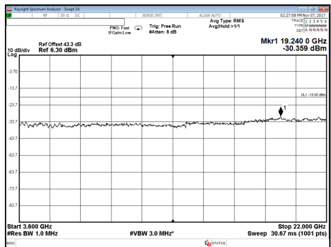
Figure 8.2-80: Conducted spurious emissions within 3600–22000 MHz, Port B, LTE, 20 MHz low channel, QPSK
