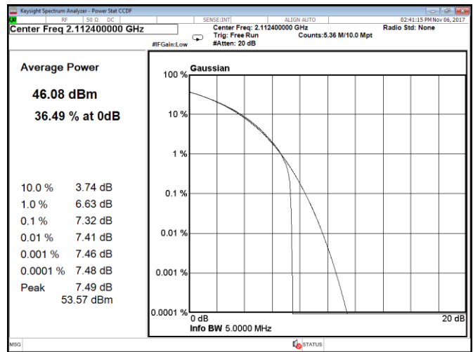
Figure 8.1-226: CCDF, QPSK, WCDMA, Port D, low channel
