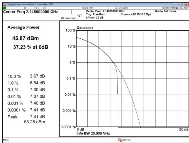
Figure 8.1-209: CCDF, QPSK, 20 MHz, LTE, Port B, mid channel
