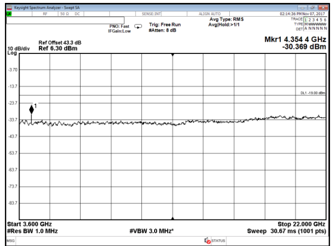
Figure 8.2-18: Conducted spurious emissions within 3600–22000 MHz, Port C, LTE, 5 MHz high channel, QPSK
