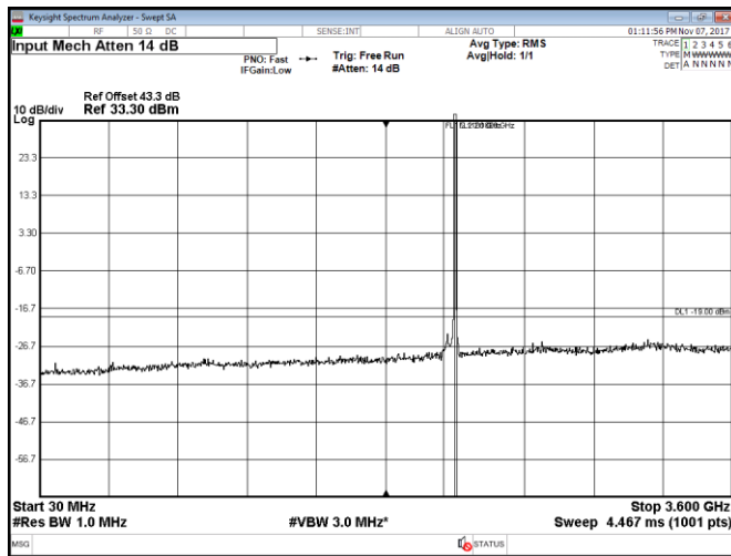
Figure 8.2-41: Conducted spurious emissions within 30–3600 MHz, Port C, LTE, 10 MHz high channel, QPSK
