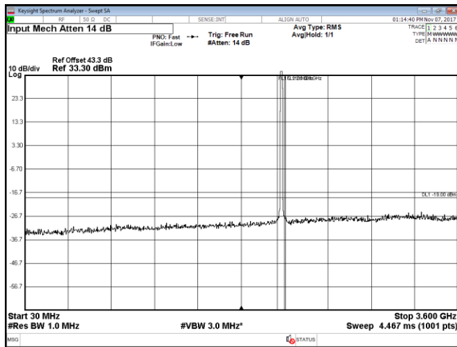
Figure 8.2-57: Conducted spurious emissions within 30–3600 MHz, Port B, LTE, 15 MHz mid channel, QPSK
