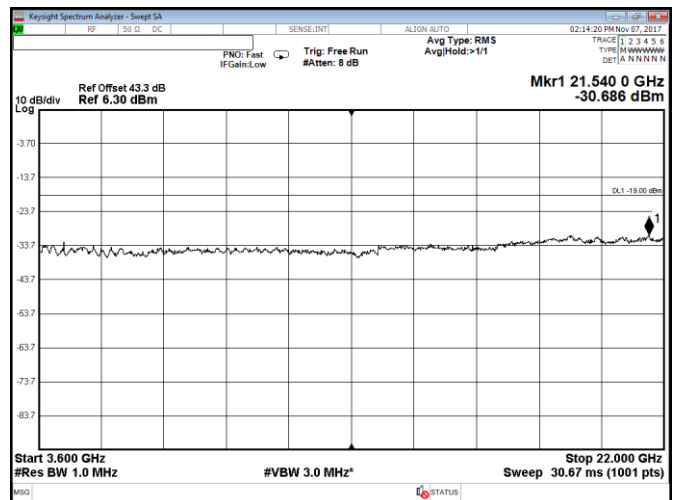
Figure 8.2-12: Conducted spurious emissions within 3600–22000 MHz, Port B, LTE, 5 MHz high channel, QPSK
