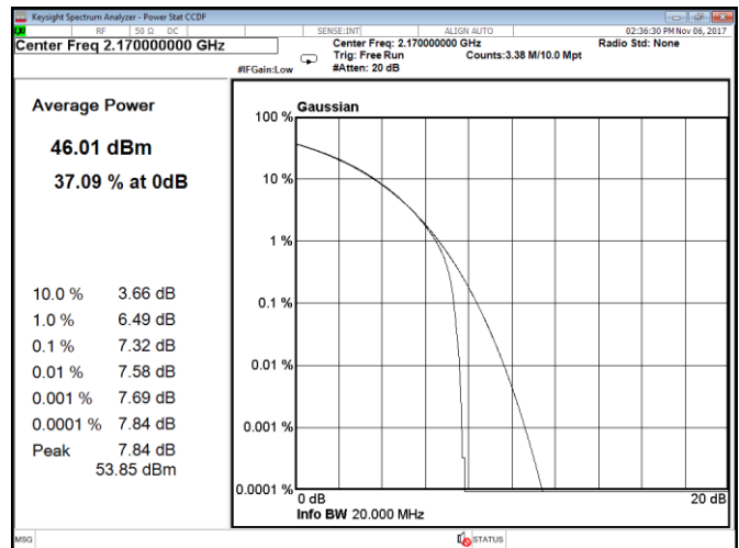
Figure 8.1-216: CCDF, QPSK, 20 MHz, LTE, Port D, high channel
