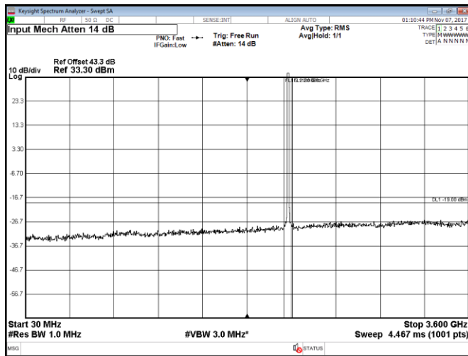
Figure 8.2-33: Conducted spurious emissions within 30–3600 MHz, Port B, LTE, 10 MHz mid channel, QPSK
