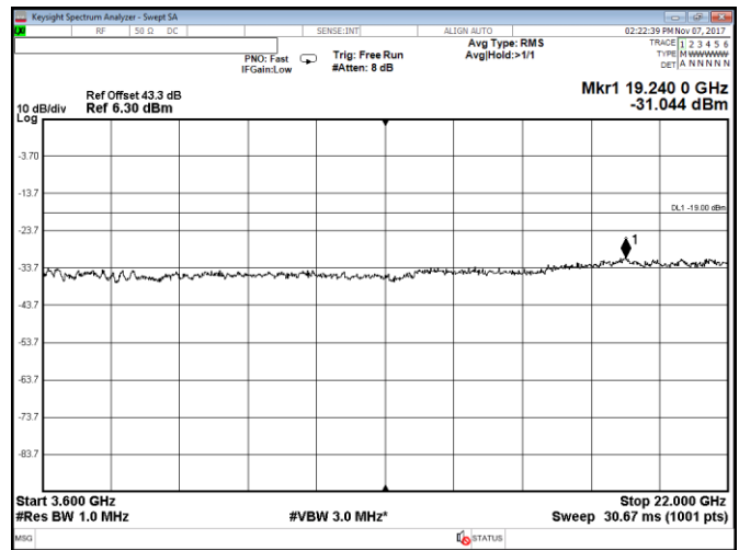
Figure 8.2-62: Conducted spurious emissions within 3600–22000 MHz, Port C, LTE, 15 MHz low channel, QPSK
