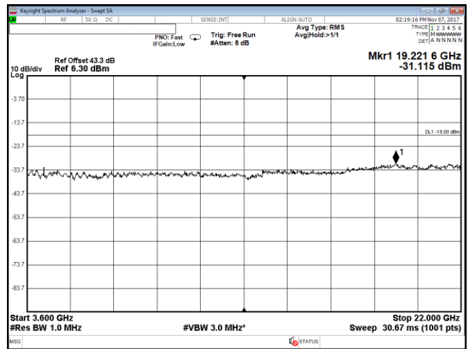
Figure 8.2-42: Conducted spurious emissions within 3600–22000 MHz, Port C, LTE, 10 MHz high channel, QPSK
