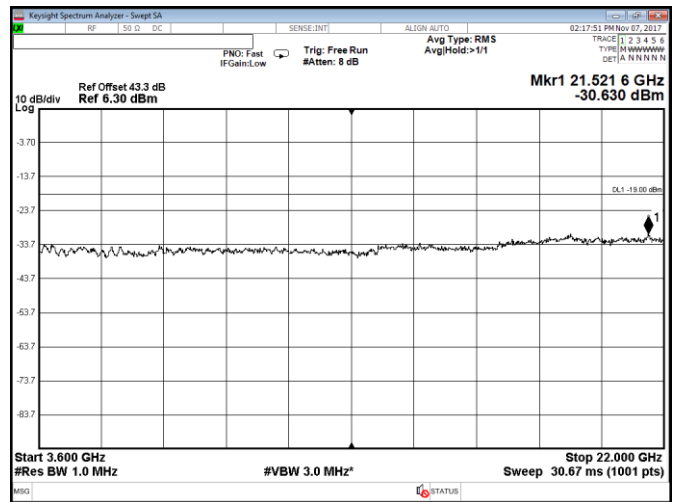
Figure 8.2-46: Conducted spurious emissions within 3600–22000 MHz, Port D, LTE, 10 MHz mid channel, QPSK
