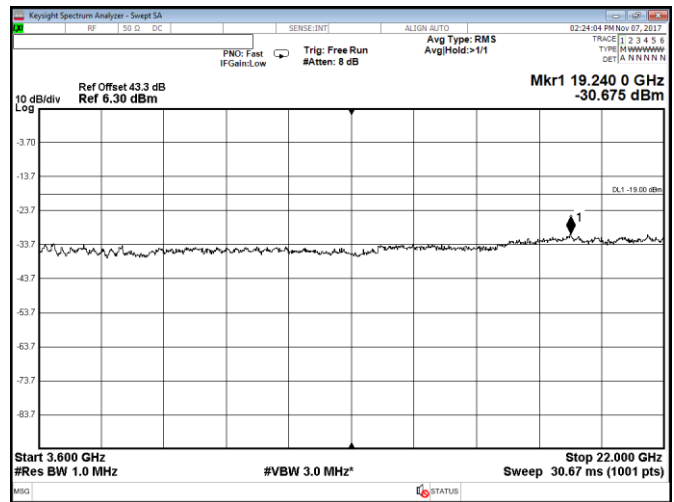
Figure 8.2-58: Conducted spurious emissions within 3600–22000 MHz, Port B, LTE, 15 MHz mid channel, QPSK
