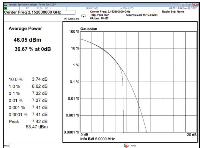
Figure 8.1-228: CCDF, QPSK, WCDMA, Port D, high channel
