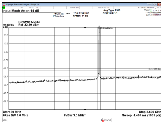
Figure 8.2-63: Conducted spurious emissions within 30–3600 MHz, Port C, LTE, 15 MHz mid channel, QPSK
