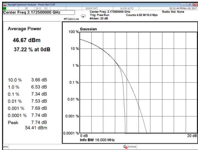
Figure 8.1-201: CCDF, QPSK, 15 MHz, LTE, Port C, high channel
