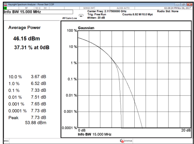
Figure 8.1-202: CCDF, QPSK, 15 MHz, LTE, Port D, low channel
