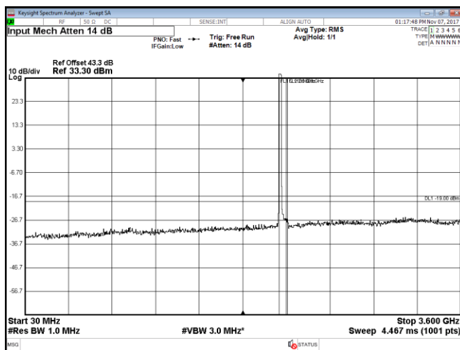
Figure 8.2-79: Conducted spurious emissions within 30–3600 MHz, Port B, LTE, 20 MHz low channel, QPSK
