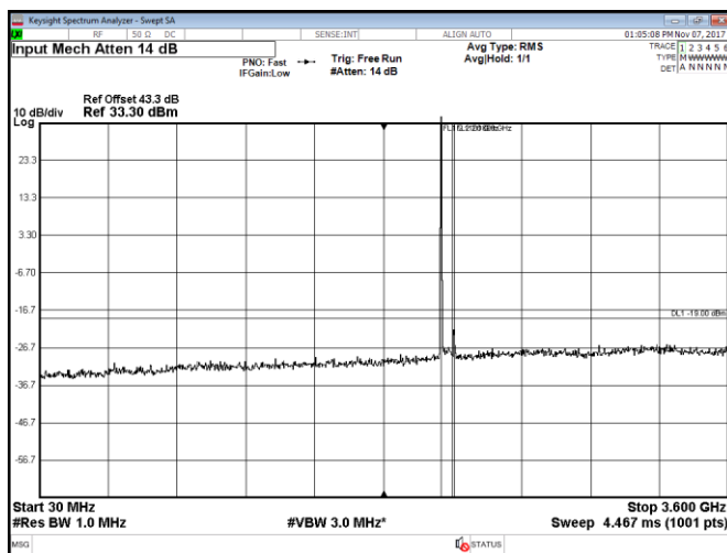
Figure 8.2-19: Conducted spurious emissions within 30–3600 MHz, Port D, LTE, 5 MHz low channel, QPSK
