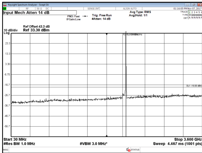
Figure 8.2-65: Conducted spurious emissions within 30–3600 MHz, Port C, LTE, 15 MHz high channel, QPSK
