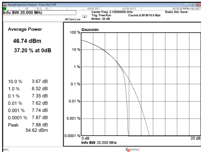
Figure 8.1-211: CCDF, QPSK, 20 MHz, LTE, Port C, low channel
