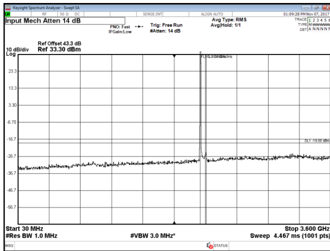
Figure 8.2-37: Conducted spurious emissions within 30–3600 MHz, Port C, LTE, 10 MHz low channel, QPSK
