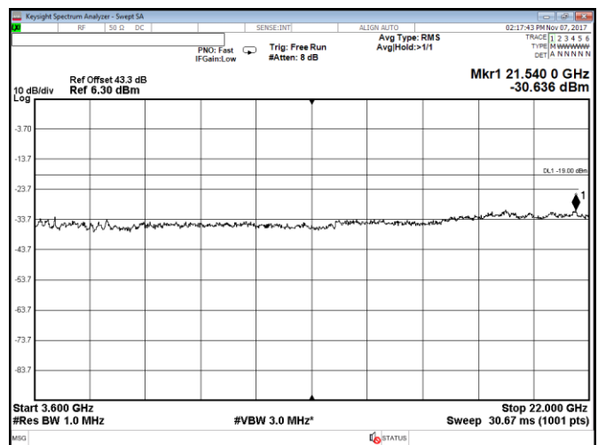
Figure 8.2-40: Conducted spurious emissions within 3600–22000 MHz, Port C, LTE, 10 MHz mid channel, QPSK
