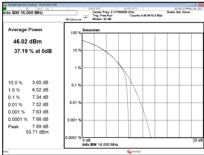
Figure 8.1-193: CCDF, QPSK, 15 MHz, LTE, Port A, low channel
