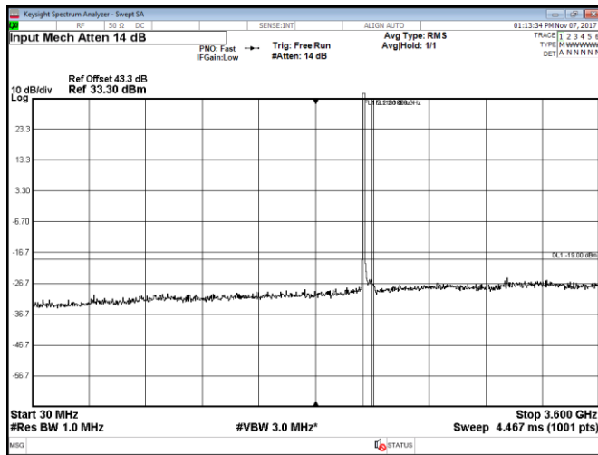
Figure 8.2-61: Conducted spurious emissions within 30–3600 MHz, Port C, LTE, 15 MHz low channel, QPSK
