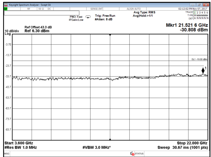
Figure 8.2-22: Conducted spurious emissions within 3600–22000 MHz, Port D, LTE, 5 MHz mid channel, QPSK
