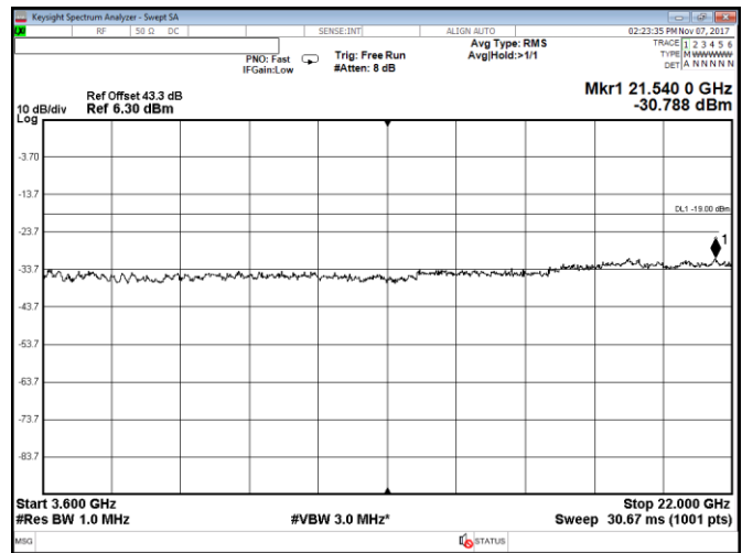
Figure 8.2-70: Conducted spurious emissions within 3600–22000 MHz, Port D, LTE, 15 MHz mid channel, QPSK
