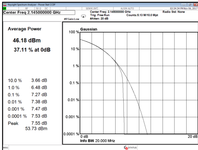
Figure 8.1-215: CCDF, QPSK, 20 MHz, LTE, Port D, mid channel
