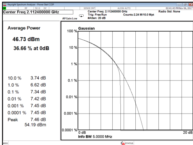
Figure 8.1-223: CCDF, QPSK, WCDMA, Port C, low channel
