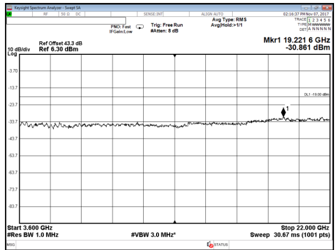
Figure 8.2-26: Conducted spurious emissions within 3600–22000 MHz, Port A, LTE, 10 MHz low channel, QPSK
