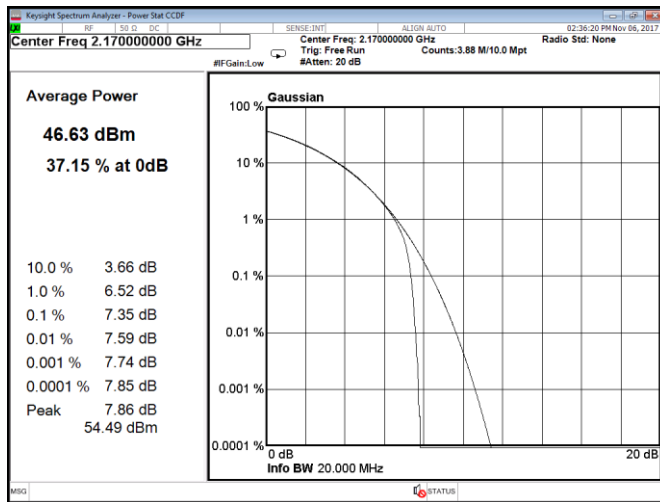
Figure 8.1-213: CCDF, QPSK, 20 MHz, LTE, Port C, high channel
