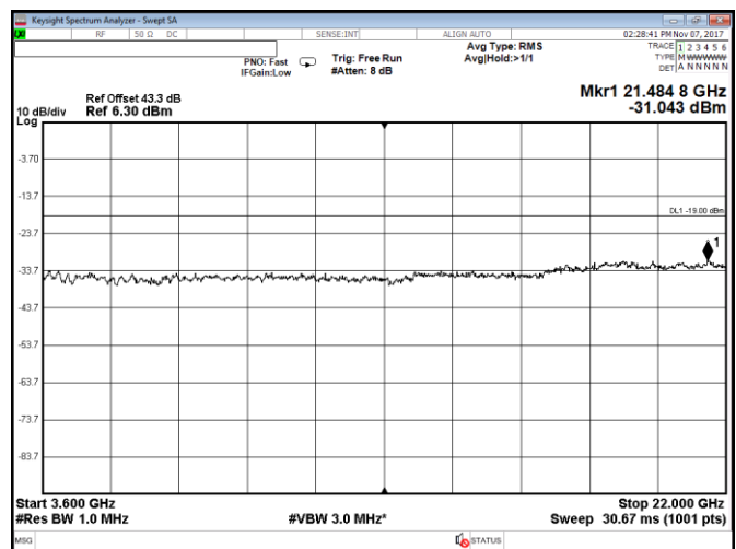
Figure 8.2-76: Conducted spurious emissions within 3600–22000 MHz, Port A, LTE, 20 MHz mid channel, QPSK
