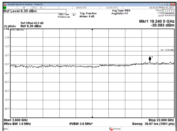
Figure 8.2-8: Conducted spurious emissions within 3600–22000 MHz, Port B, LTE, 5 MHz low channel, QPSK
