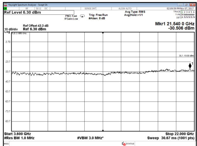
Figure 8.2-2: Conducted spurious emissions within 3600–22000 MHz, Port A, LTE, 5 MHz low channel, QPSK
