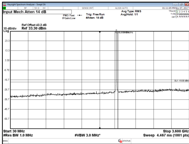
Figure 8.2-45: Conducted spurious emissions within 30–3600 MHz, Port D, LTE, 10 MHz mid channel, QPSK
