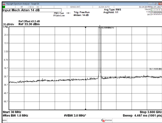
Figure 8.2-69: Conducted spurious emissions within 30–3600 MHz, Port D, LTE, 15 MHz mid channel, QPSK
