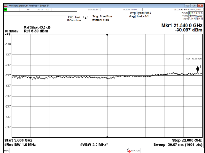
Figure 8.2-72: Conducted spurious emissions within 3600–22000 MHz, Port D, LTE, 15 MHz high channel, QPSK
