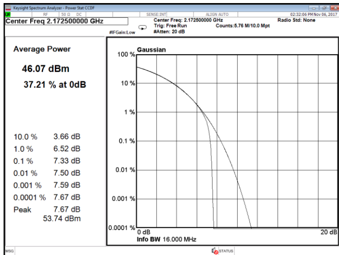
Figure 8.1-195: CCDF, QPSK, 15 MHz, LTE, Port A, high channel
