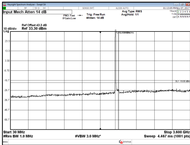
Figure 8.2-49: Conducted spurious emissions within 30–3600 MHz, Port A, LTE, 15 MHz low channel, QPSK
