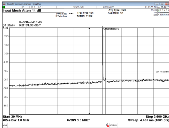
Figure 8.2-25: Conducted spurious emissions within 30–3600 MHz, Port A, LTE, 10 MHz low channel, QPSK
