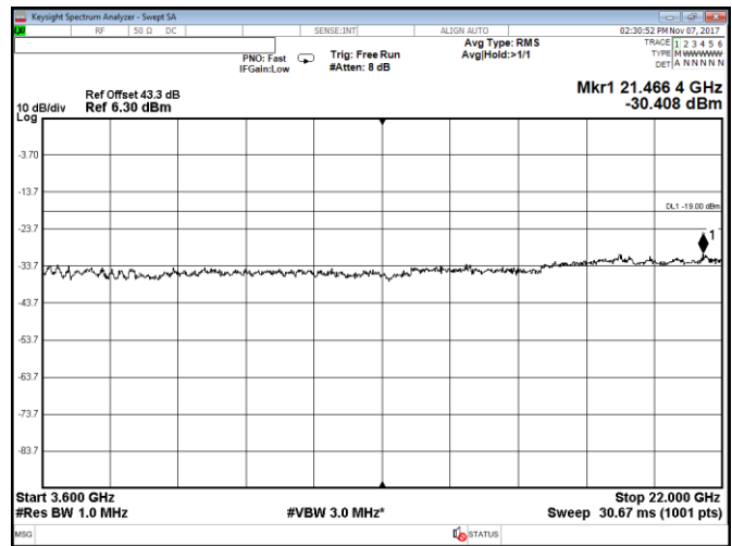
Figure 8.2-78: Conducted spurious emissions within 3600–22000 MHz, Port A, LTE, 20 MHz high channel, QPSK
