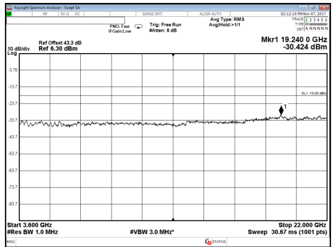
Figure 8.2-10: Conducted spurious emissions within 3600–22000 MHz, Port B, LTE, 5 MHz mid channel, QPSK
