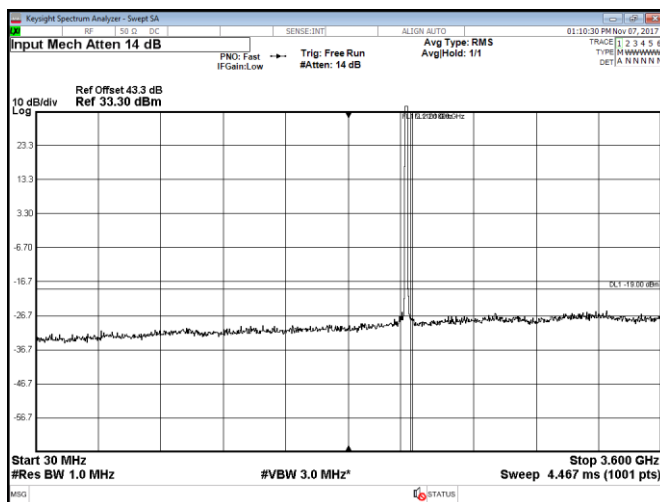
Figure 8.2-27: Conducted spurious emissions within 30–3600 MHz, Port A, LTE, 10 MHz mid channel, QPSK
