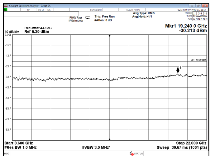
Figure 8.2-24: Conducted spurious emissions within 3600–22000 MHz, Port D, LTE, 5 MHz high channel, QPSK
