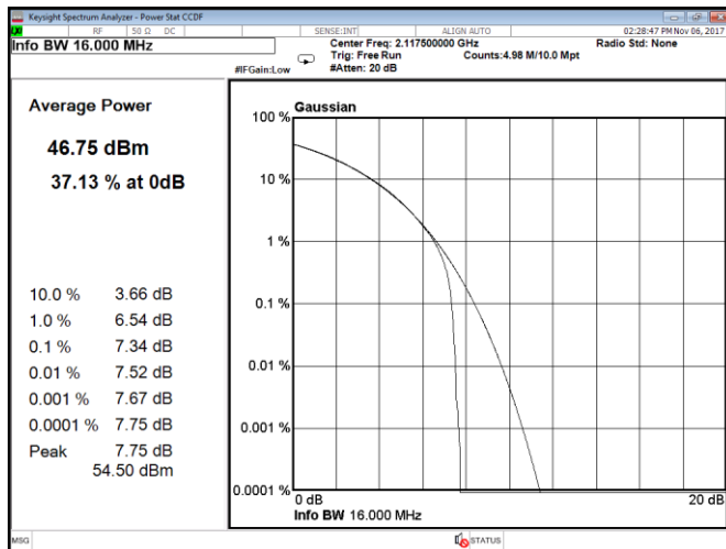
Figure 8.1-199: CCDF, QPSK, 15 MHz, LTE, Port C, low channel
