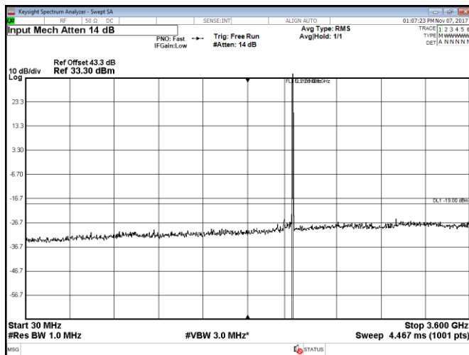
Figure 8.2-11: Conducted spurious emissions within 30–3600 MHz, Port B, LTE, 5 MHz high channel, QPSK
