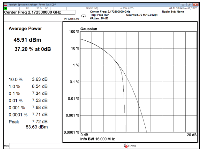
Figure 8.1-198: CCDF, QPSK, 15 MHz, LTE, Port B, high channel
