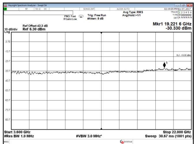
Figure 8.2-48: Conducted spurious emissions within 3600–22000 MHz, Port D, LTE, 10 MHz high channel, QPSK
