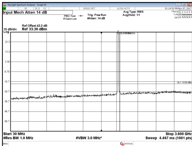
Figure 8.2-51: Conducted spurious emissions within 30–3600 MHz, Port A, LTE, 15 MHz mid channel, QPSK
