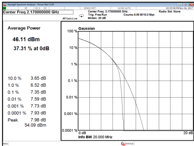
Figure 8.1-207: CCDF, QPSK, 20 MHz, LTE, Port A, high channel
