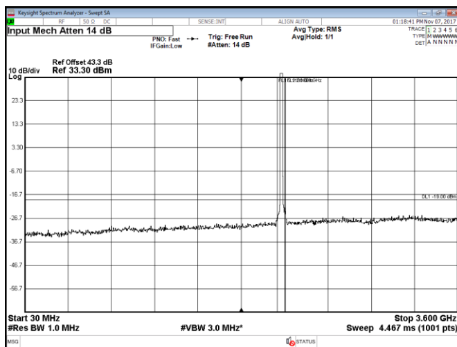
Figure 8.2-75: Conducted spurious emissions within 30–3600 MHz, Port A, LTE, 20 MHz mid channel, QPSK
