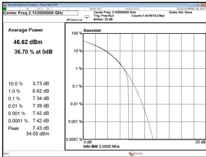
Figure 8.1-225: CCDF, QPSK, WCDMA, Port C, high channel
