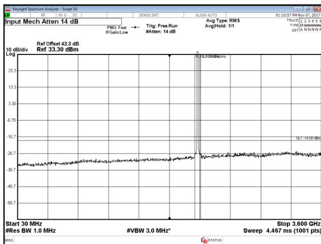
Figure 8.2-39: Conducted spurious emissions within 30–3600 MHz, Port C, LTE, 10 MHz mid channel, QPSK
