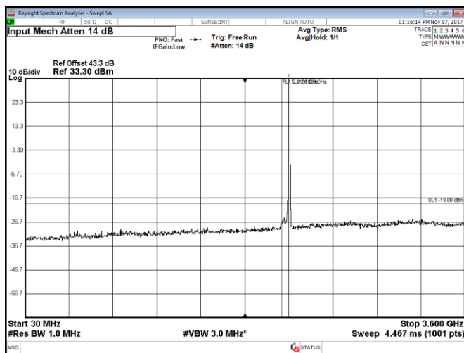
Figure 8.2-71: Conducted spurious emissions within 30–3600 MHz, Port D, LTE, 15 MHz high channel, QPSK
