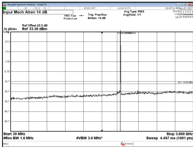
Figure 8.2-5: Conducted spurious emissions within 30–3600 MHz, Port A, LTE, 5 MHz high channel, QPSK
