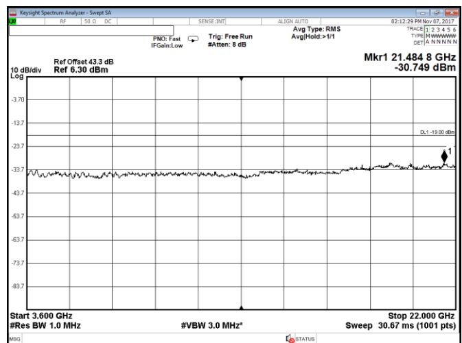
Figure 8.2-4: Conducted spurious emissions within 3600–22000 MHz, Port A, LTE, 5 MHz mid channel, QPSK
