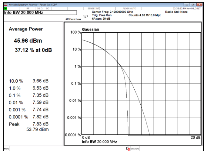
Figure 8.1-208: CCDF, QPSK, 20 MHz, LTE, Port B, low channel
