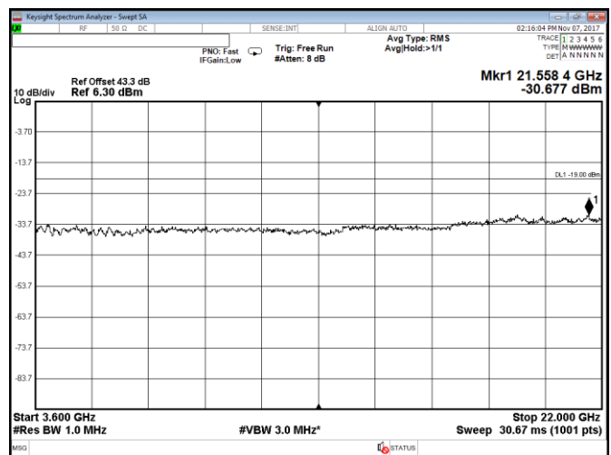
Figure 8.2-44: Conducted spurious emissions within 3600–22000 MHz, Port D, LTE, 10 MHz low channel, QPSK
