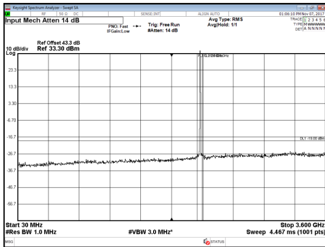
Figure 8.2-9: Conducted spurious emissions within 30–3600 MHz, Port B, LTE, 5 MHz mid channel, QPSK
