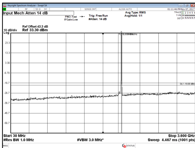
Figure 8.2-47: Conducted spurious emissions within 30–3600 MHz, Port D, LTE, 10 MHz high channel, QPSK
