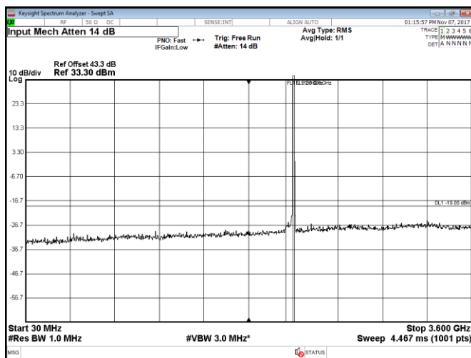
Figure 8.2-59: Conducted spurious emissions within 30–3600 MHz, Port B, LTE, 15 MHz high channel, QPSK
