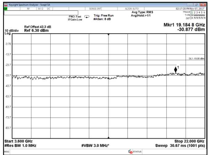
Figure 8.2-34: Conducted spurious emissions within 3600–22000 MHz, Port B, LTE, 10 MHz mid channel, QPSK
