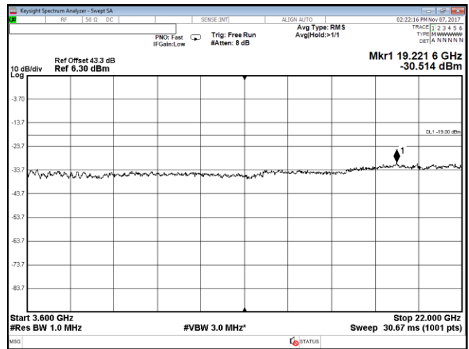
Figure 8.2-50: Conducted spurious emissions within 3600–22000 MHz, Port A, LTE, 15 MHz low channel, QPSK
