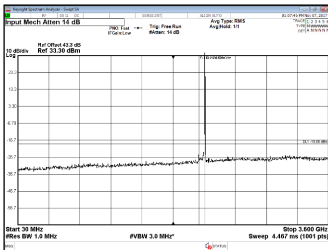
Figure 8.2-23: Conducted spurious emissions within 30–3600 MHz, Port D, LTE, 5 MHz high channel, QPSK
