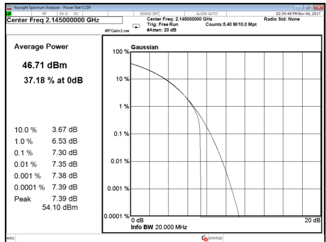
Figure 8.1-212: CCDF, QPSK, 20 MHz, LTE, Port C, mid channel
