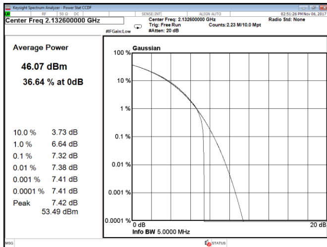
Figure 8.1-227: CCDF, QPSK, WCDMA, Port D, mid channel
