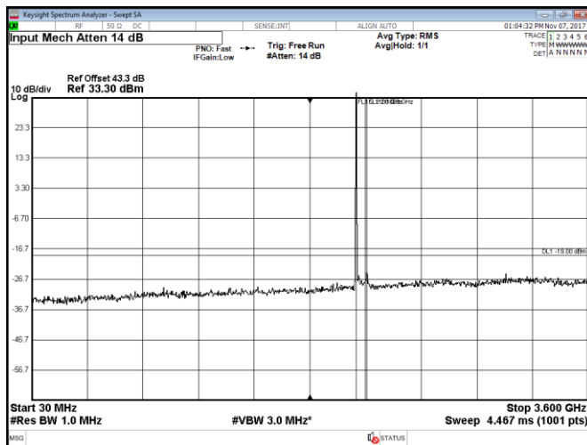
Figure 8.2-7: Conducted spurious emissions within 30–3600 MHz, Port B, LTE, 5 MHz low channel, QPSK
