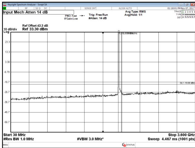
Figure 8.2-73: Conducted spurious emissions within 30–3600 MHz, Port A, LTE, 20 MHz low channel, QPSK
