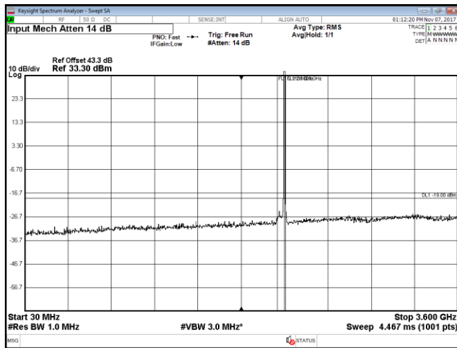
Figure 8.2-29: Conducted spurious emissions within 30–3600 MHz, Port A, LTE, 10 MHz high channel, QPSK
