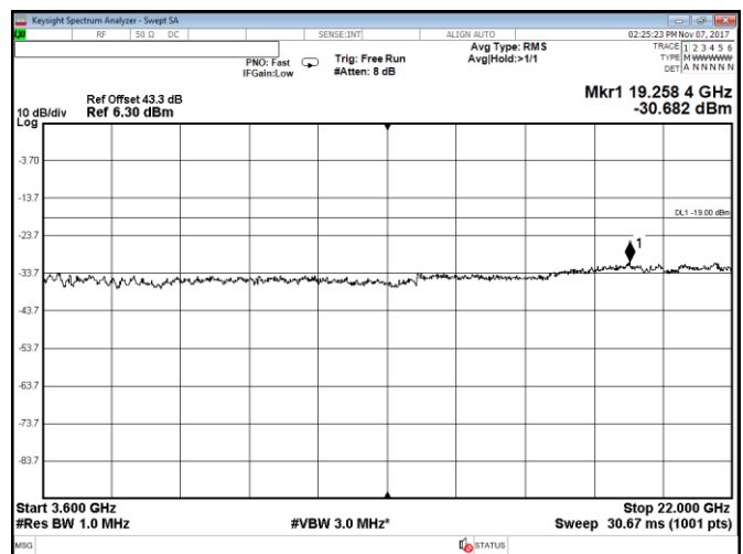
Figure 8.2-60: Conducted spurious emissions within 3600–22000 MHz, Port B, LTE, 15 MHz high channel, QPSK
