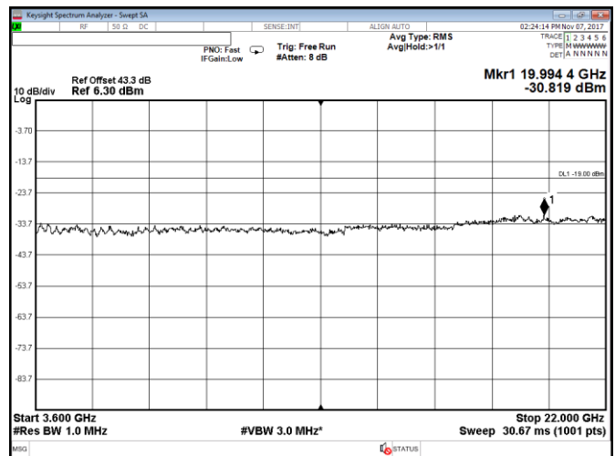
Figure 8.2-52: Conducted spurious emissions within 3600–22000 MHz, Port A, LTE, 15 MHz mid channel, QPSK
