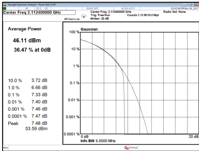
Figure 8.1-217: CCDF, QPSK, WCDMA, Port A, low channel
