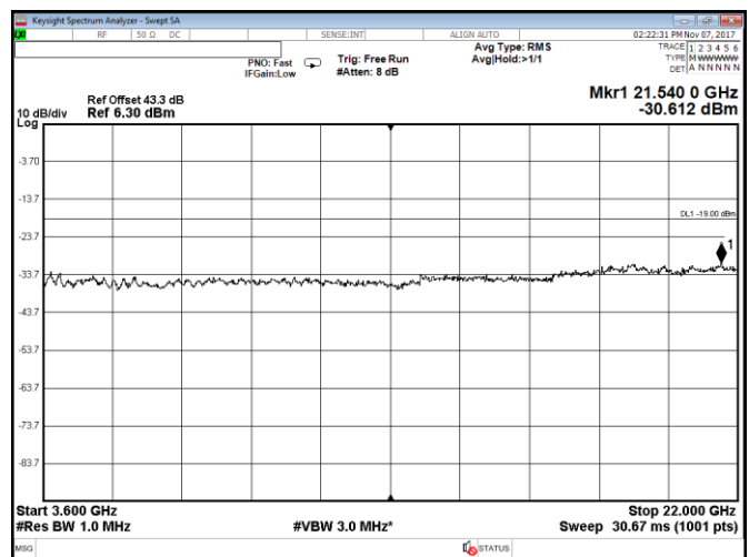
Figure 8.2-56: Conducted spurious emissions within 3600–22000 MHz, Port B, LTE, 15 MHz low channel, QPSK
