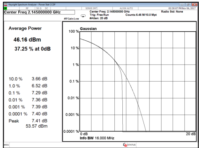
Figure 8.1-194: CCDF, QPSK, 15 MHz, LTE, Port A, mid channel
