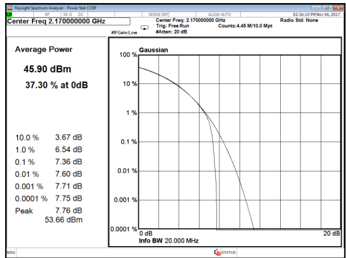
Figure 8.1-210: CCDF, QPSK, 20 MHz, LTE, Port B, high channel
