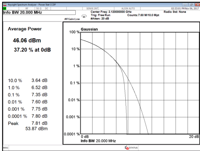
Figure 8.1-205: CCDF, QPSK, 20 MHz, LTE, Port A, low channel
