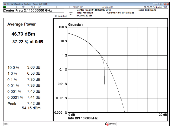
Figure 8.1-200: CCDF, QPSK, 15 MHz, LTE, Port C, mid channel
