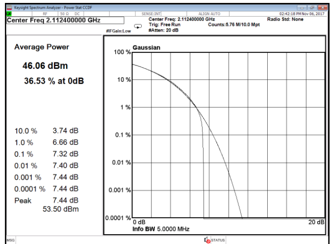
Figure 8.1-220: CCDF, QPSK, WCDMA, Port B, low channel
