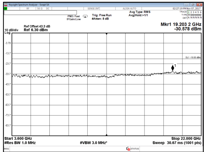
Figure 8.2-74: Conducted spurious emissions within 3600–22000 MHz, Port A, LTE, 20 MHz low channel, QPSK
