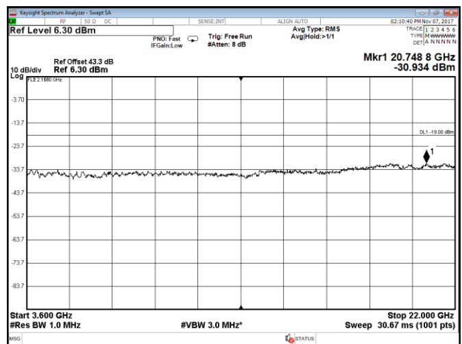
Figure 8.2-20: Conducted spurious emissions within 3600–22000 MHz, Port D, LTE, 5 MHz low channel, QPSK
