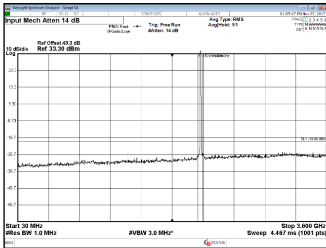
Figure 8.2-21: Conducted spurious emissions within 30–3600 MHz, Port D, LTE, 5 MHz mid channel, QPSK
