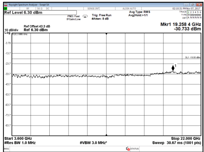
Figure 8.2-14: Conducted spurious emissions within 3600–22000 MHz, Port C, LTE, 5 MHz low channel, QPSK
