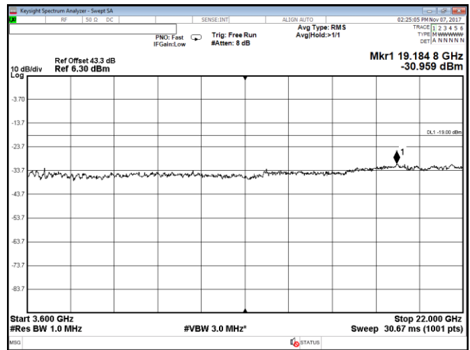
Figure 8.2-54: Conducted spurious emissions within 3600–22000 MHz, Port A, LTE, 15 MHz high channel, QPSK
