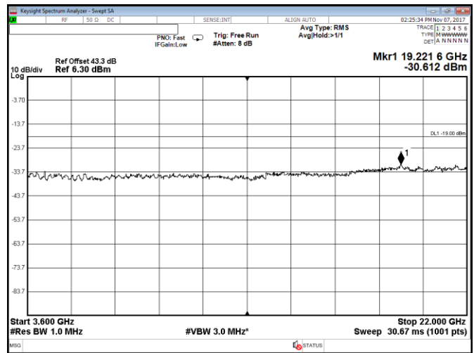
Figure 8.2-66: Conducted spurious emissions within 3600–22000 MHz, Port C, LTE, 15 MHz high channel, QPSK
