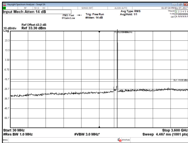
Figure 8.2-17: Conducted spurious emissions within 30–3600 MHz, Port C, LTE, 5 MHz high channel, QPSK
