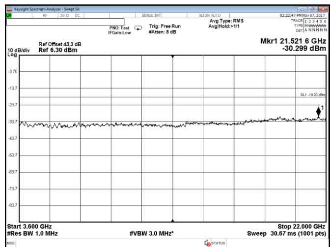
Figure 8.2-68: Conducted spurious emissions within 3600–22000 MHz, Port D, LTE, 15 MHz low channel, QPSK
