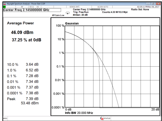
Figure 8.1-206: CCDF, QPSK, 20 MHz, LTE, Port A, mid channel
