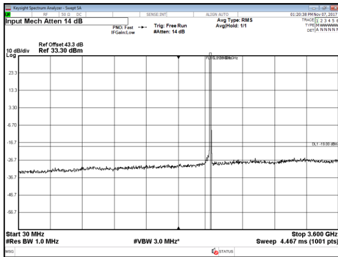
Figure 8.2-77: Conducted spurious emissions within 30–3600 MHz, Port A, LTE, 20 MHz high channel, QPSK
