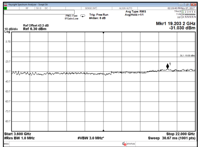
Figure 8.2-30: Conducted spurious emissions within 3600–22000 MHz, Port A, LTE, 10 MHz high channel, QPSK
