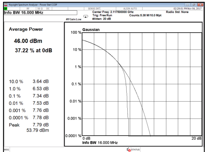
Figure 8.1-196: CCDF, QPSK, 15 MHz, LTE, Port B, low channel
