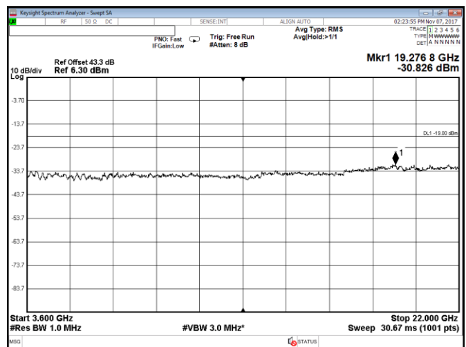
Figure 8.2-64: Conducted spurious emissions within 3600–22000 MHz, Port C, LTE, 15 MHz mid channel, QPSK
