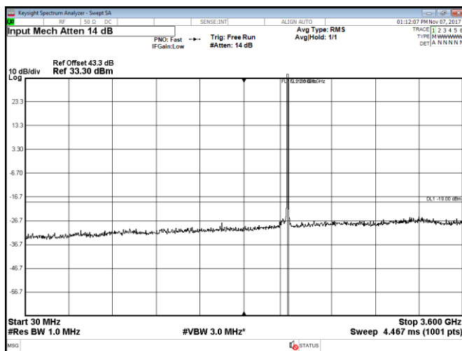
Figure 8.2-35: Conducted spurious emissions within 30–3600 MHz, Port B, LTE, 10 MHz high channel, QPSK
