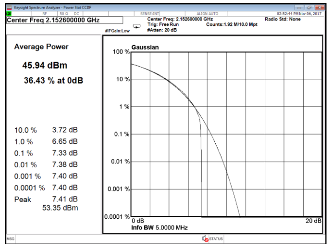
Figure 8.1-222: CCDF, QPSK, WCDMA, Port B, high channel
