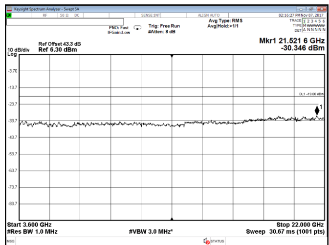
Figure 8.2-32: Conducted spurious emissions within 3600–22000 MHz, Port B, LTE, 10 MHz low channel, QPSK
