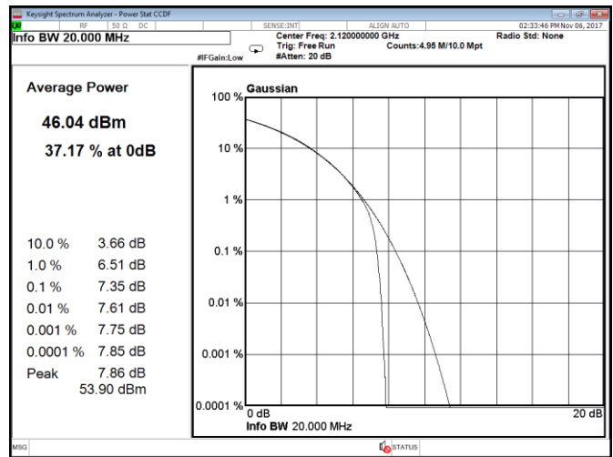
Figure 8.1-214: CCDF, QPSK, 20 MHz, LTE, Port D, low channel
