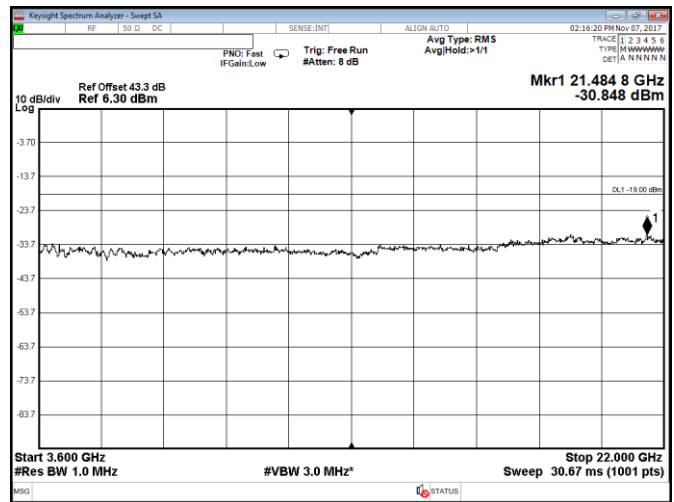
Figure 8.2-38: Conducted spurious emissions within 3600–22000 MHz, Port C, LTE, 10 MHz low channel, QPSK
