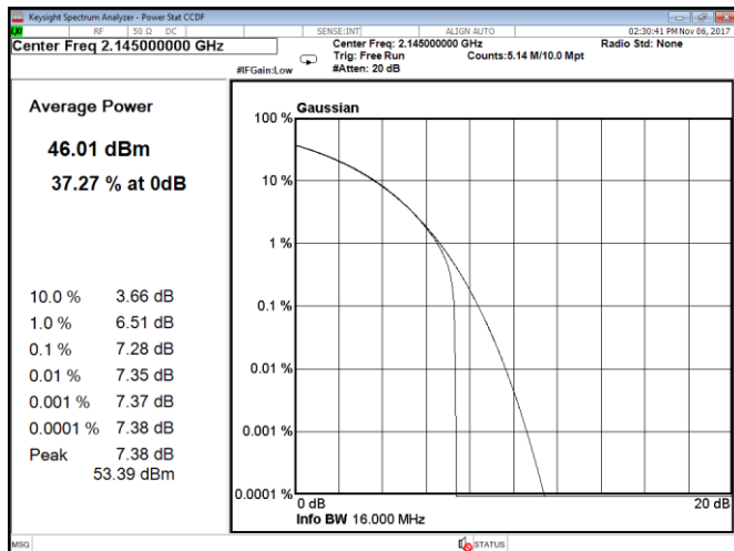
Figure 8.1-203: CCDF, QPSK, 15 MHz, LTE, Port D, mid channel
