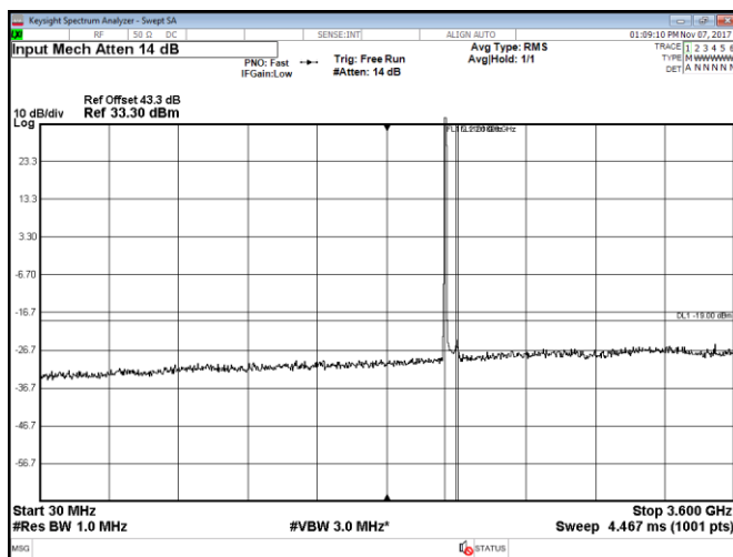
Figure 8.2-43: Conducted spurious emissions within 30–3600 MHz, Port D, LTE, 10 MHz low channel, QPSK
