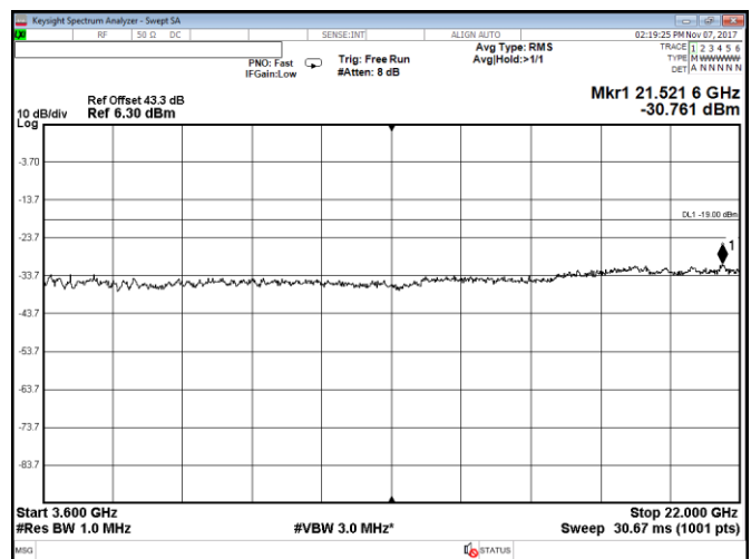
Figure 8.2-36: Conducted spurious emissions within 3600–22000 MHz, Port B, LTE, 10 MHz high channel, QPSK
