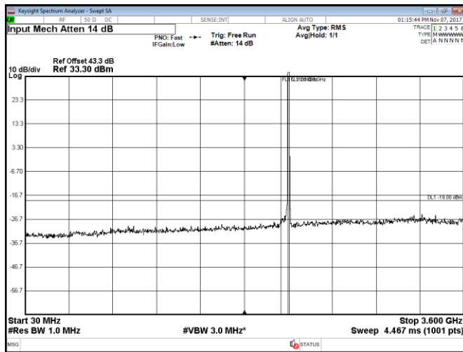
Figure 8.2-53: Conducted spurious emissions within 30–3600 MHz, Port A, LTE, 15 MHz high channel, QPSK
