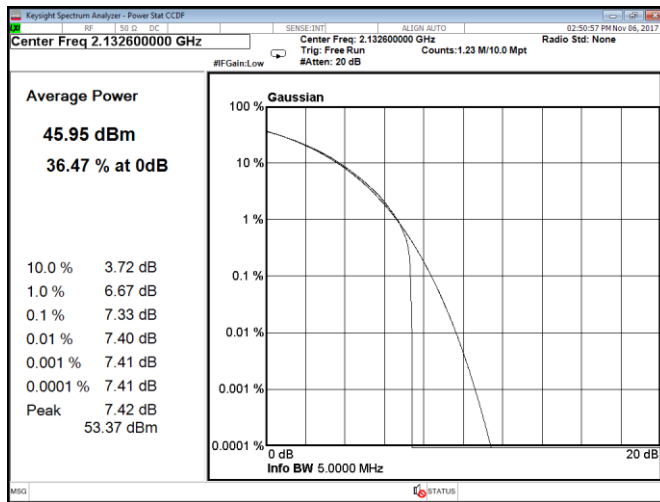
Figure 8.1-221: CCDF, QPSK, WCDMA, Port B, mid channel
