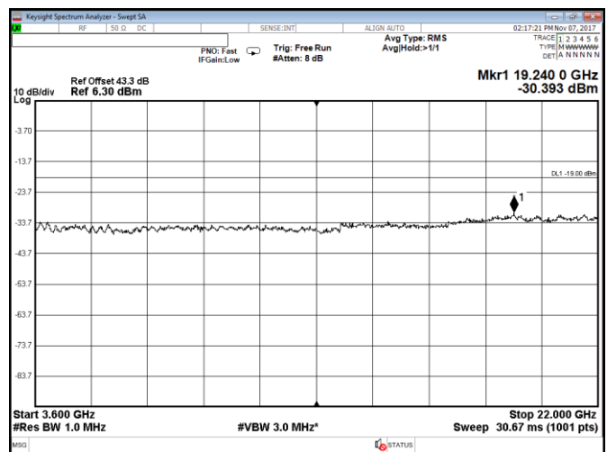
Figure 8.2-28: Conducted spurious emissions within 3600–22000 MHz, Port A, LTE, 10 MHz mid channel, QPSK
