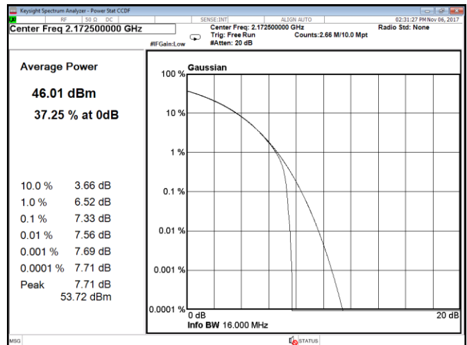
Figure 8.1-204: CCDF, QPSK, 15 MHz, LTE, Port D, high channel
