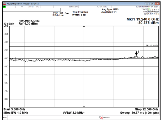
Figure 8.2-6: Conducted spurious emissions within 3600–22000 MHz, Port A, LTE, 5 MHz high channel, QPSK
