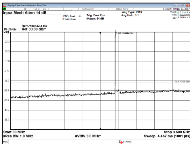
Figure 8.2-31: Conducted spurious emissions within 30–3600 MHz, Port B, LTE, 10 MHz low channel, QPSK
