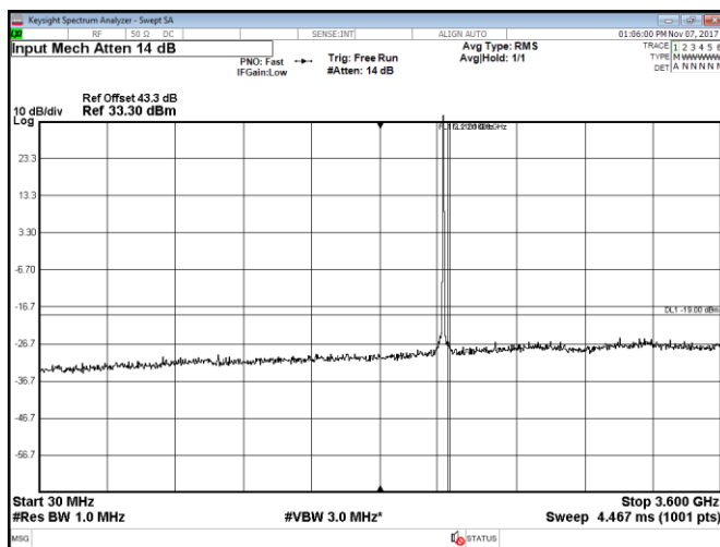
Figure 8.2-15: Conducted spurious emissions within 30–3600 MHz, Port C, LTE, 5 MHz mid channel, QPSK
