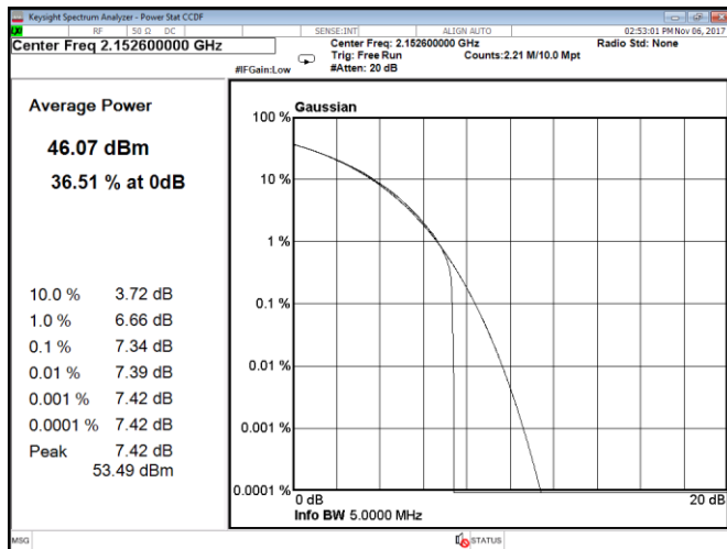
Figure 8.1-219: CCDF, QPSK, WCDMA, Port A, high channel
