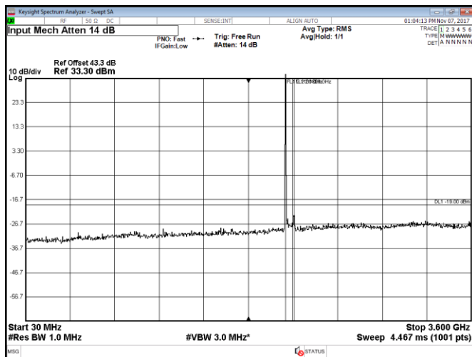
Figure 8.2-1: Conducted spurious emissions within 30–3600 MHz, Port A, LTE, 5 MHz low channel, QPSK
