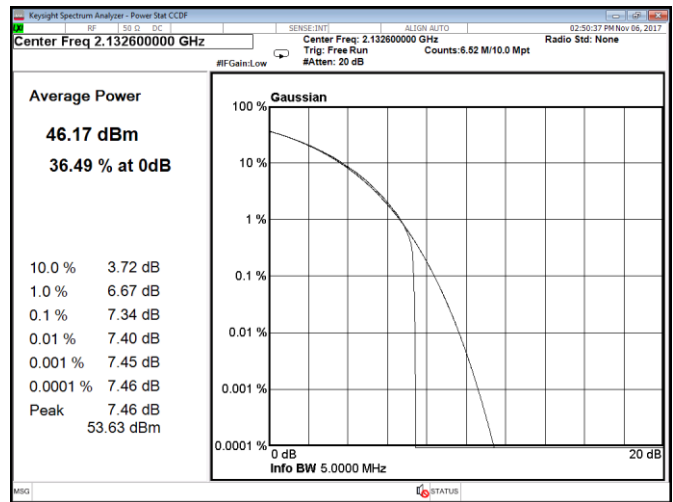
Figure 8.1-218: CCDF, QPSK, WCDMA, Port A, mid channel
