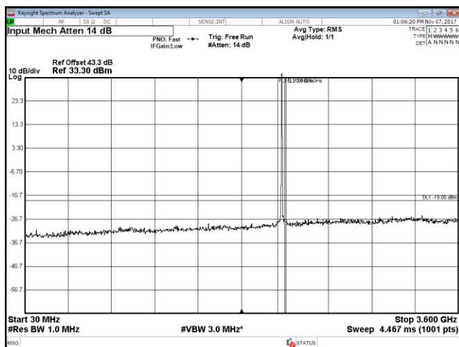
Figure 8.2-3: Conducted spurious emissions within 30–3600 MHz, Port A, LTE, 5 MHz mid channel, QPSK
