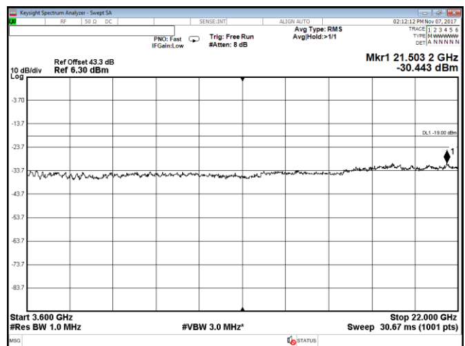
Figure 8.2-16: Conducted spurious emissions within 3600–22000 MHz, Port C, LTE, 5 MHz mid channel, QPSK
