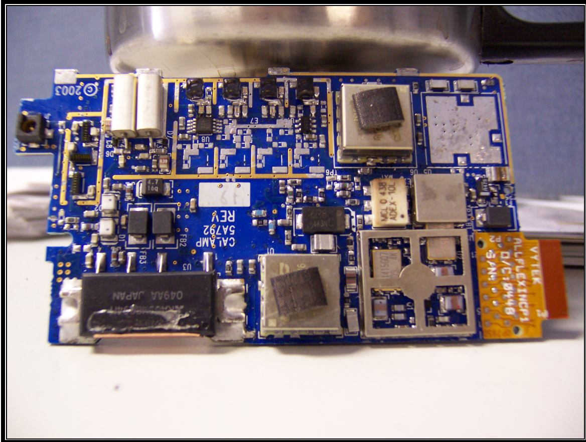
PHOTOGRAPH 14: RF BOARD TOP VIEW
