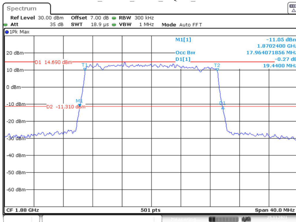
Band 2 20 MHz Middle 16QAM RB100#0
