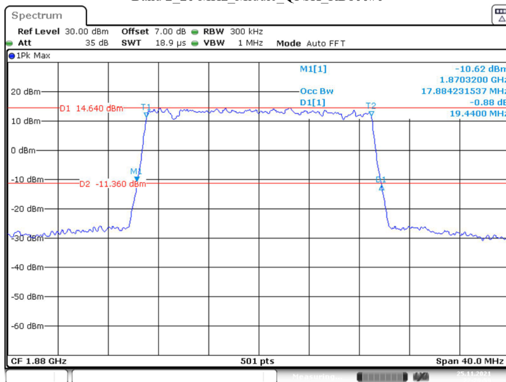
Band 2 20 MHz Middle QPSK RB100#0
