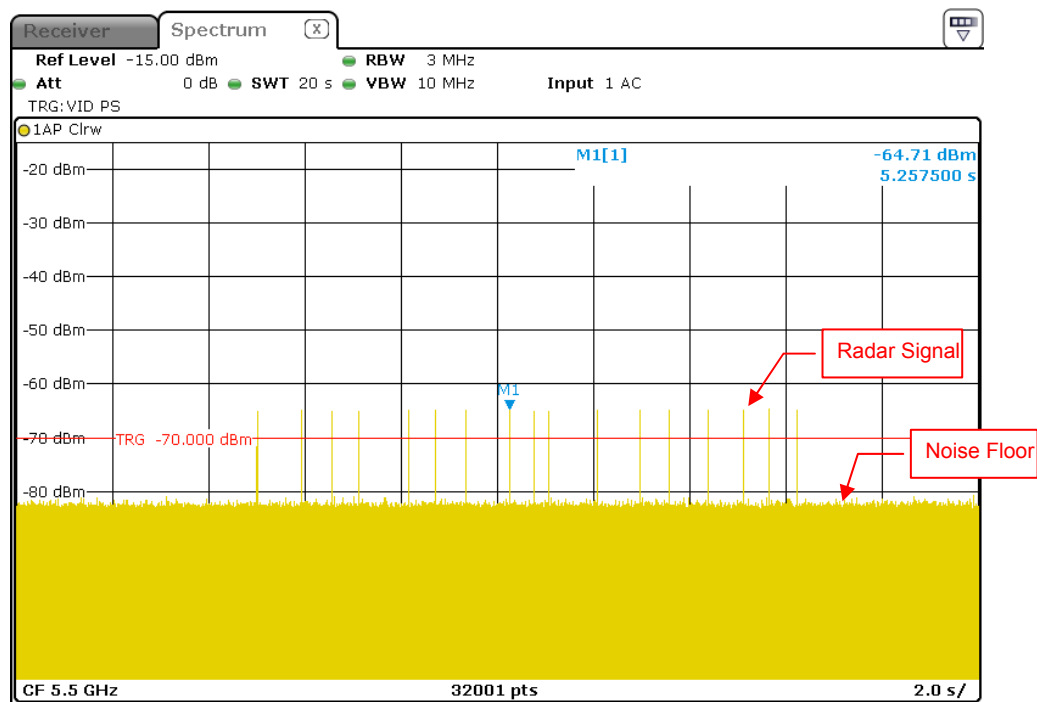
Radar Signal 5
