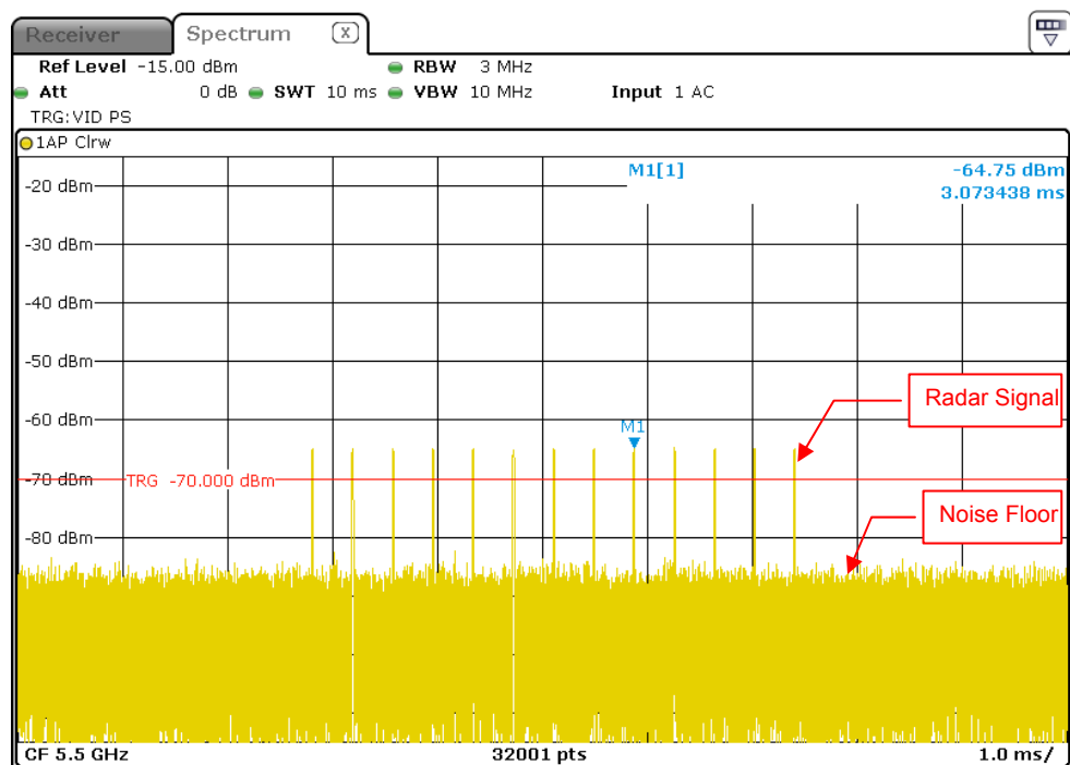
Radar Signal 4
