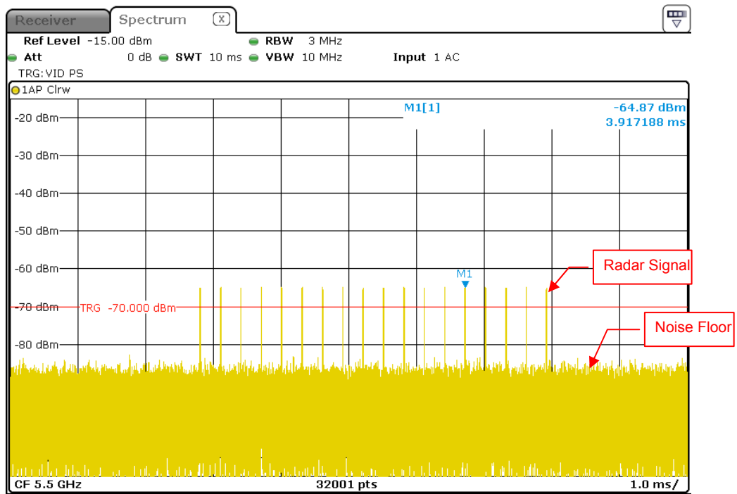
Radar Signal 3
