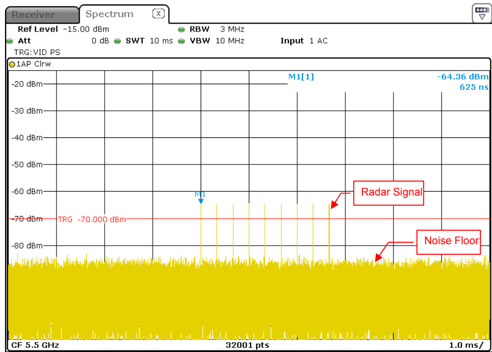
Radar Signal 6
