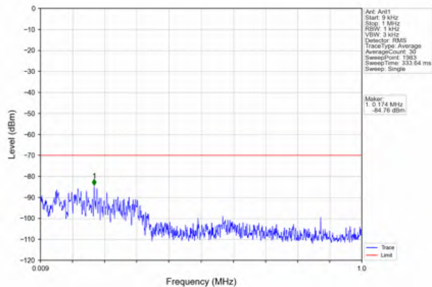
n78d_30kHz_SISO_NTNV_25MHz_DFT-s-OFDM QPSK_3687.48MHz_Inner_1RB_Right
