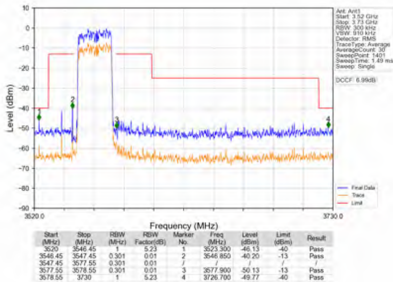
n78d_30kHz_SISO_NTNV_25MHz_CP-OFDM QPSK_3562.5MHz_Outer_Full
