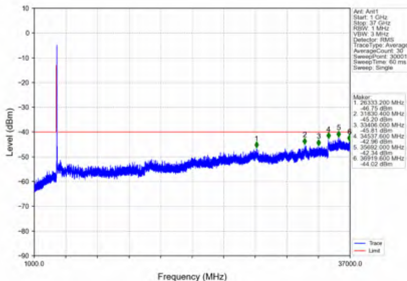
n78d_30kHz_SISO_NTNV_50MHz_DFT-s-OFDM_QPSK_3575.01MHz_Inner_1RB_Left
