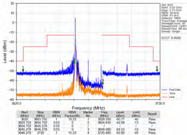
n78d_30kHz_SISO_NTNV_40MHz_DFT-s-OFDM_PI/2_BPSK_3624.99MHz_Edge_1RB_Left
