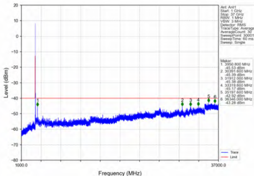
n78d_30kHz_SISO_NTV_50MHz_CP-OFDM QPSK_3575.01MHz_Outer_Full
