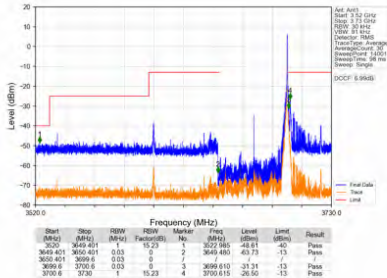
n78d_30kHz_SISO_NTNV_50MHz_CP-OFDM QPSK_3675MHz_Edge_1RB_Right
