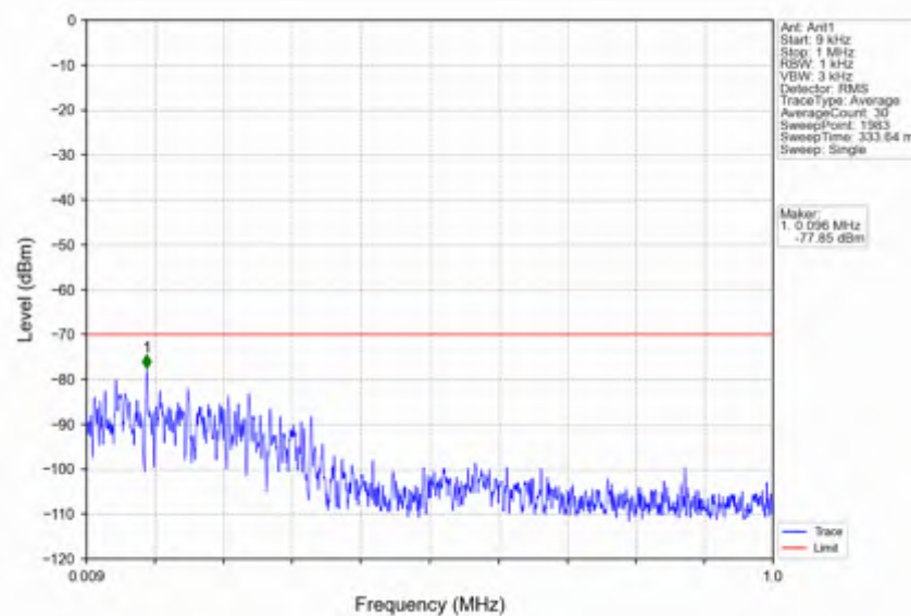
n78d_30kHz_SISO_NTNV_50MHz_CP-OFDM QPSK_3675MHz_Edge_1RB_Right
