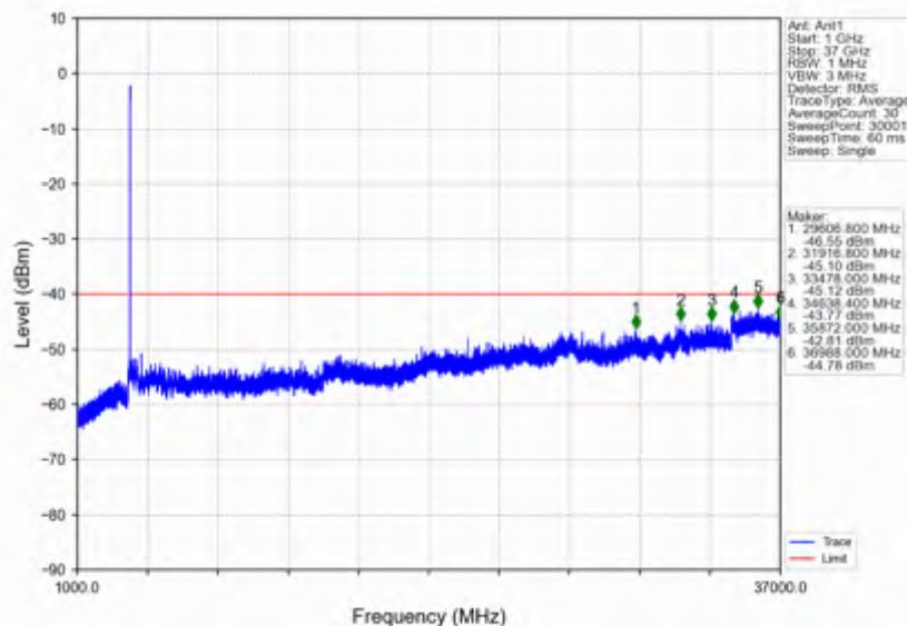
n78d_30kHz_SISO_NTNV_30MHz_DFT-s-OFDM QPSK_3684.99MHz_Inner_1RB_Right
