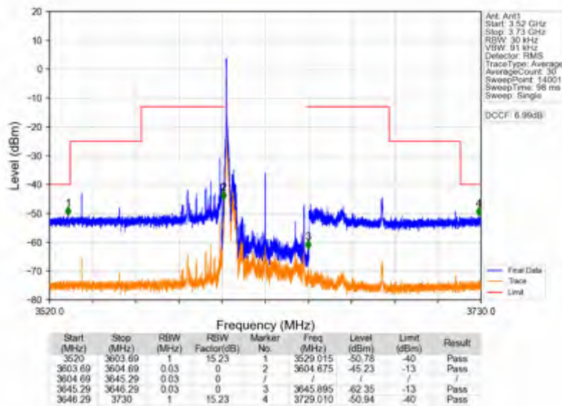
n78d_30kHz_SISO_NTV_40MHz_CP-OFDM QPSK_3624.99MHz_Edge_1RB_Left
