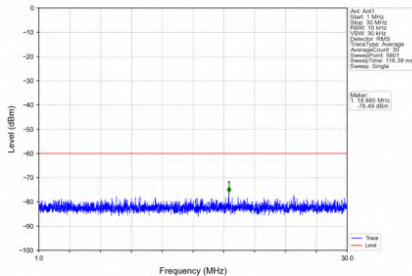
n78d_30kHz_SISO_NTNV_25MHz_CP-OFDM QPSK_3687.48MHz_Edge_1RB_Right
