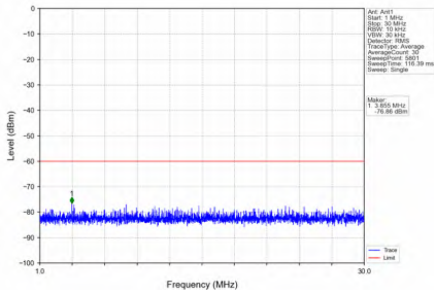
n78d_30kHz_SISO_NTNV_50MHz_DFT-s-OFDM_QPSK_3575.01MHz_Outer_Full
