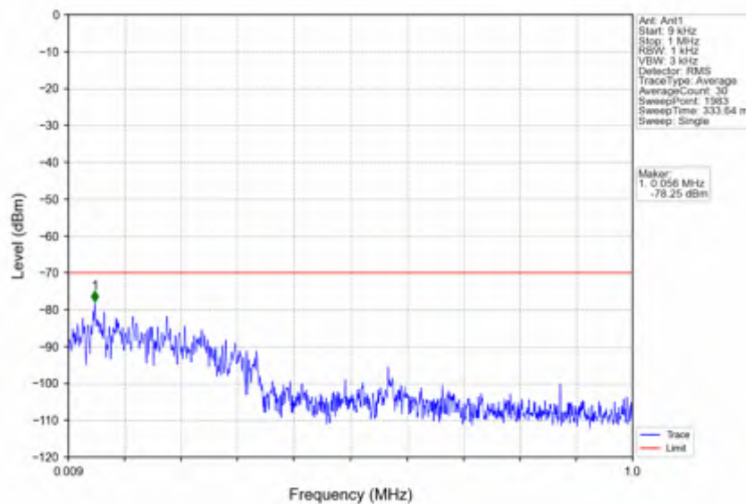
n78d_30kHz_SISO_NTNV_40MHz_CP-OFDM_QPSK_3570MHz_Inner_1RB_Left
