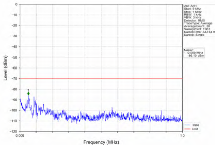
n78d_30kHz_SISO_NTNV_25MHz_DFT-s-OFDM_QPSK_3687.48MHz_Outer_Full
