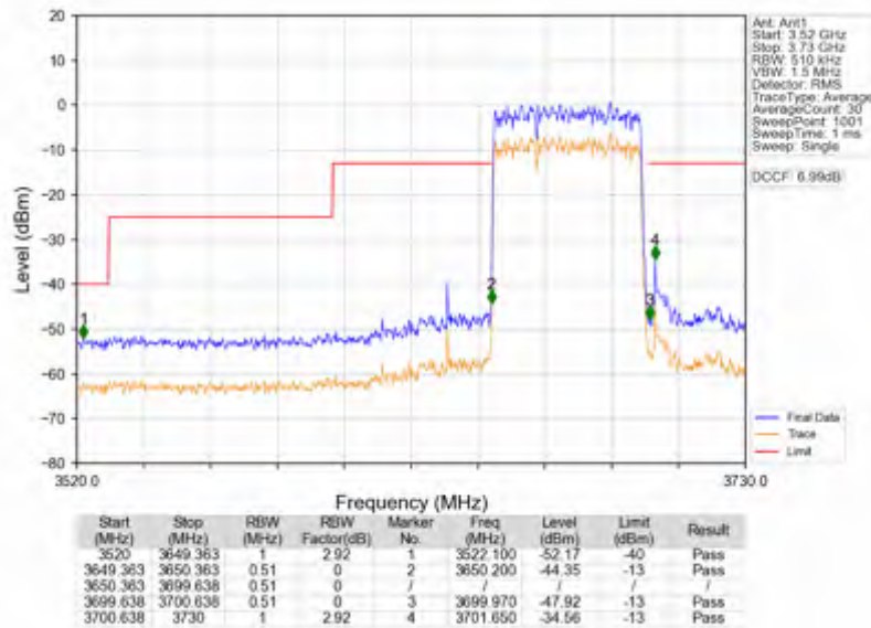
n78d_30kHz_SISO_NTNV_50MHz_DFT-s-OFDM_PI/2_BPSK_3675MHz_Outer_Full
