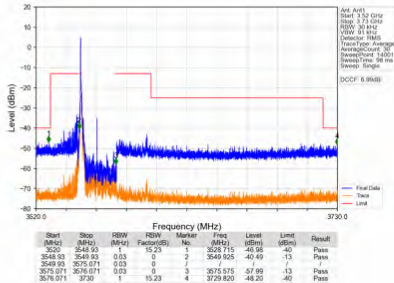
n78d_30kHz_SISO_NTNV_25MHz_CP-OFDM QPSK_3562.5MHz_Edge_1RB_Left
