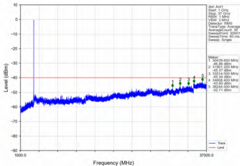
n78d_30kHz_SISO_NTNV_30MHz_DFT-s-OFDM_QPSK_3565.02MHz_Inner_1RB_Left
