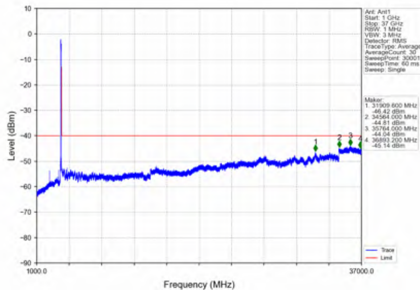
n78d_30kHz_SISO_NTNV_50MHz_DFT-s-OFDM QPSK_3675MHz_Inner_1RB_Right
