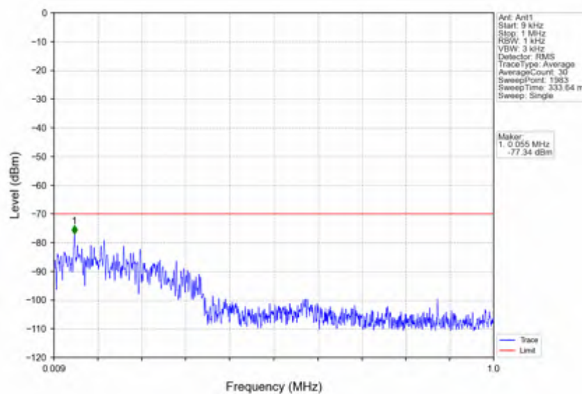
n78d_30kHz_SISO_NTNV_25MHz_CP-OFDM QPSK_3562.5MHz_Edge_1RB_Left
