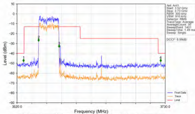
n78d_30kHz_SISO_NTNV_30MHz_CP-OFDM_QPSK_3565.02MHz_Outer_Full
