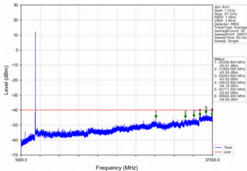
n78d_30kHz_SISO_NTNV_25MHz_CP-OFDM QPSK_3687.48MHz_Outer_Full
