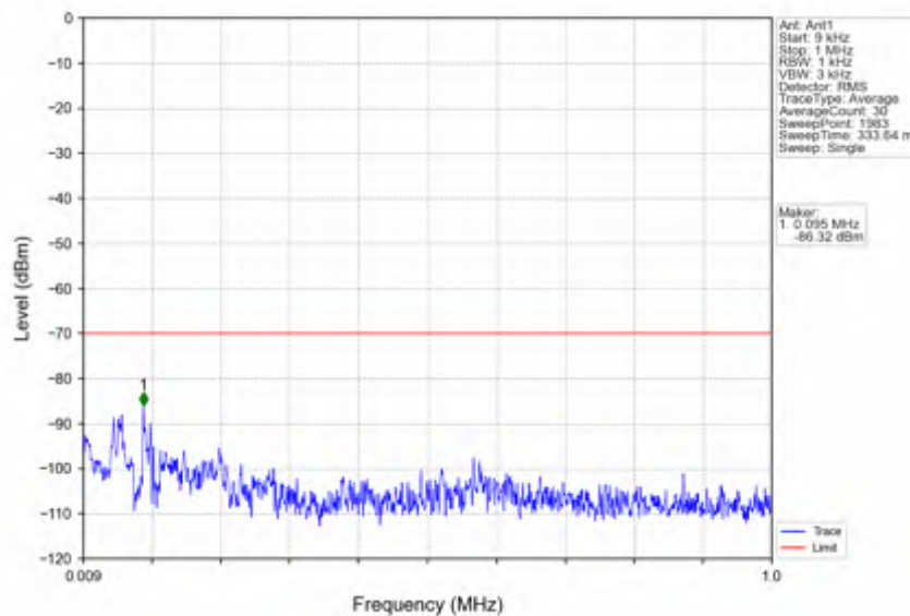
n78d_30kHz_SISO_NTNV_30MHz_DFT-s-OFDM_QPSK_3684.99MHz_Outer_Full
