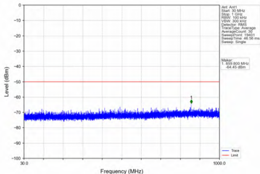
n78d_30kHz_SISO_NTNV_30MHz_CP-OFDM QPSK_3684.99MHz_Outer_Full
