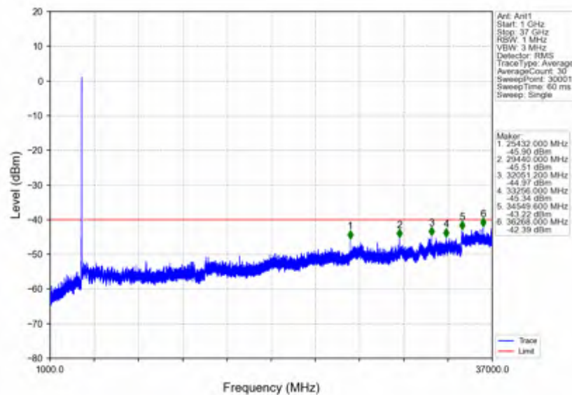
n78d_30kHz_SISO_NTNV_30MHz_CP-OFDM QPSK_3565.02MHz_Outer_Full
