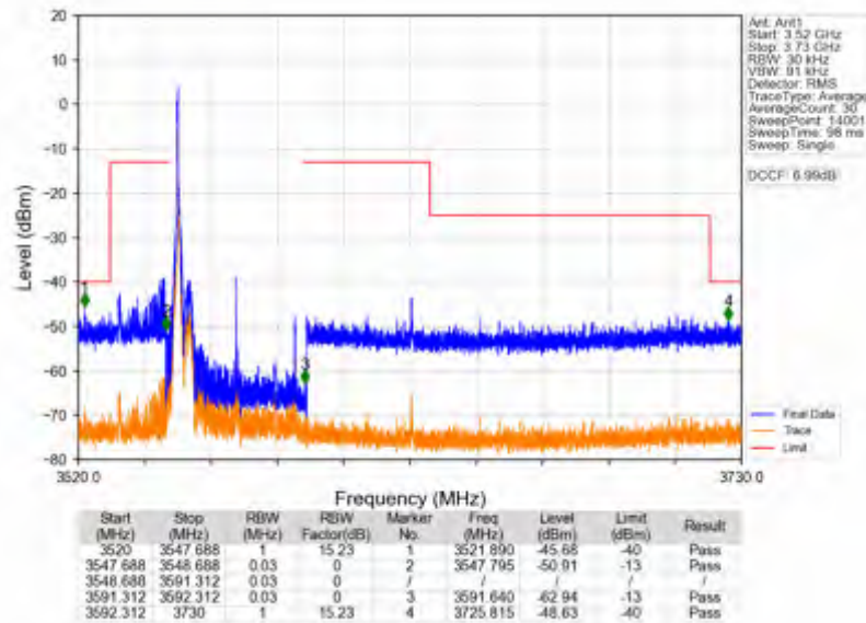
n78d_30kHz_SISO_NTNV_40MHz_DFT-s-OFDM_QPSK_3570MHz_Inner_1RB_Left
