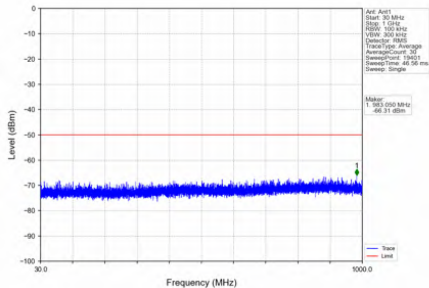
n78d_30kHz_SISO_NTNV_25MHz_CP-OFDM QPSK_3562.5MHz_Inner_1RB_Left
