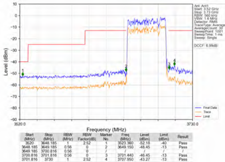
n78d_30kHz_SISO_NTNV_50MHz_DFT-s-OFDM_QPSK_3675MHz_Outer_Full
