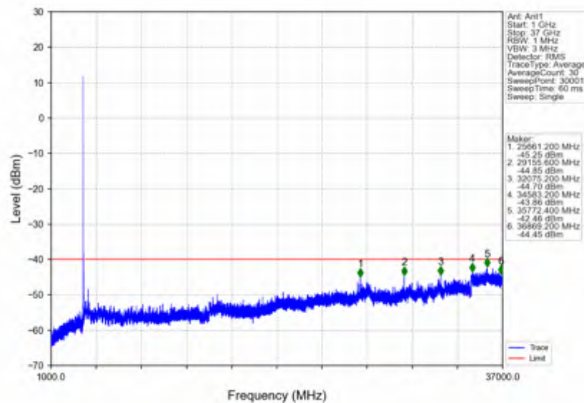
n78d_30kHz_SISO_NTNV_25MHz_CP-OFDM QPSK_3624.99MHz_Edge_1RB_Left
