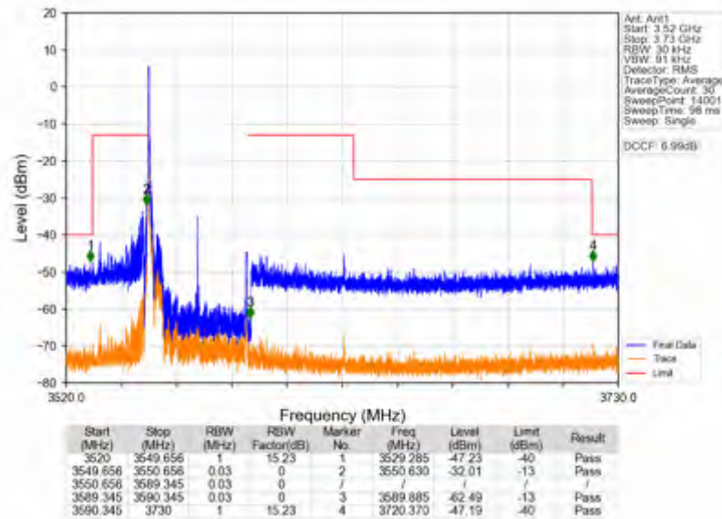
n78d_30kHz_SISO_NTNV_40MHz_CP-OFDM_QPSK_3570MHz_Inner_1RB_Left
