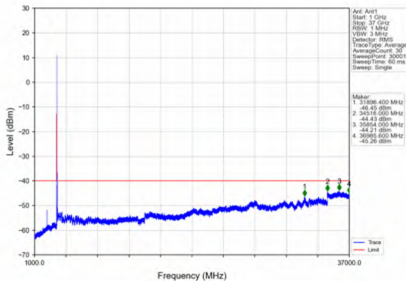
n78d_30kHz_SISO_NTNV_40MHz_DFT-s-OFDM_PI/2_BPSK_3624.99MHz_Edge_1RB_Left
