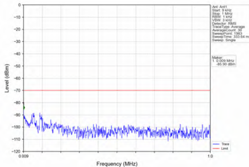
n78d_30kHz_SISO_NTNV_40MHz_CP-OFDM QPSK_3679.98MHz_Outer_Full
