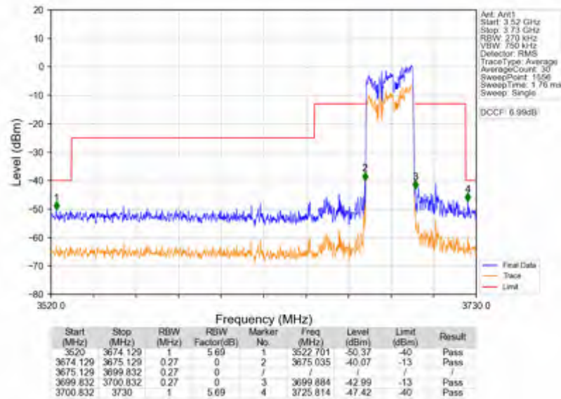
n78d_30kHz_SISO_NTNV_25MHz_DFT-s-OFDM_QPSK_3687.48MHz_Outer_Full
