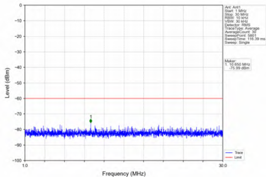
n78d_30kHz_SISO_NTNV_40MHz_CP-OFDM QPSK_3679.98MHz_Inner_1RB_Right
