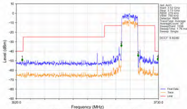
n78d_30kHz_SISO_NTNV_25MHz_CP-OFDM QPSK_3687.48MHz_Outer_Full
