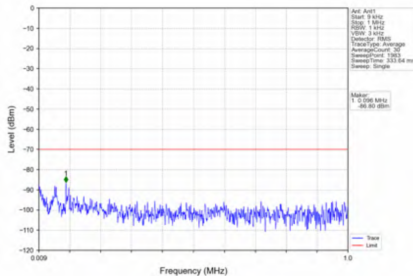
n78d_30kHz_SISO_NTNV_25MHz_CP-OFDM QPSK_3562.5MHz_Outer_Full
