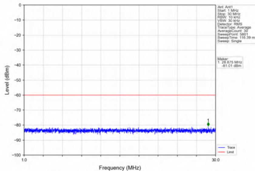
n78d_30kHz_SISO_NTNV_40MHz_DFT-s-OFDM_QPSK_3679.98MHz_Outer_Full
