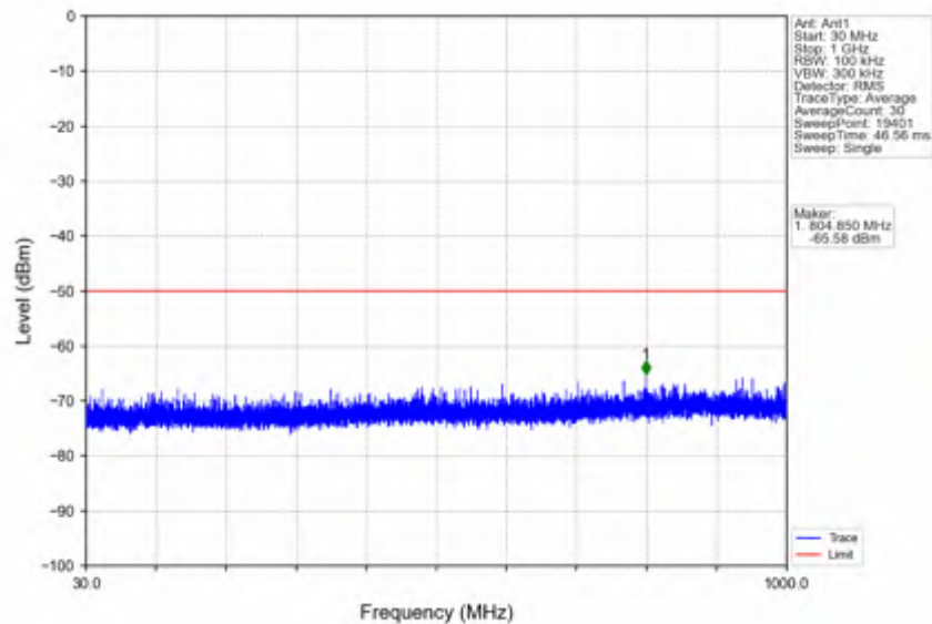
n78d_30kHz_SISO_NTNV_50MHz_CP-OFDM_QPSK_3675MHz_Outer_Full
