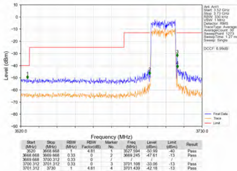
n78d_30kHz_SISO_NTNV_30MHz_CP-OFDM QPSK_3684.99MHz_Outer_Full
