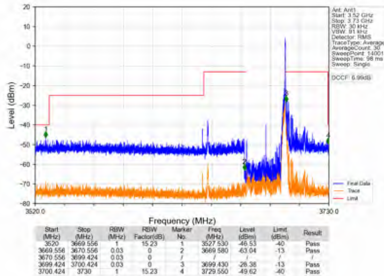
n78d_30kHz_SISO_NTNV_30MHz_CP-OFDM_QPSK_3684.99MHz_Edge_1RB_Right
