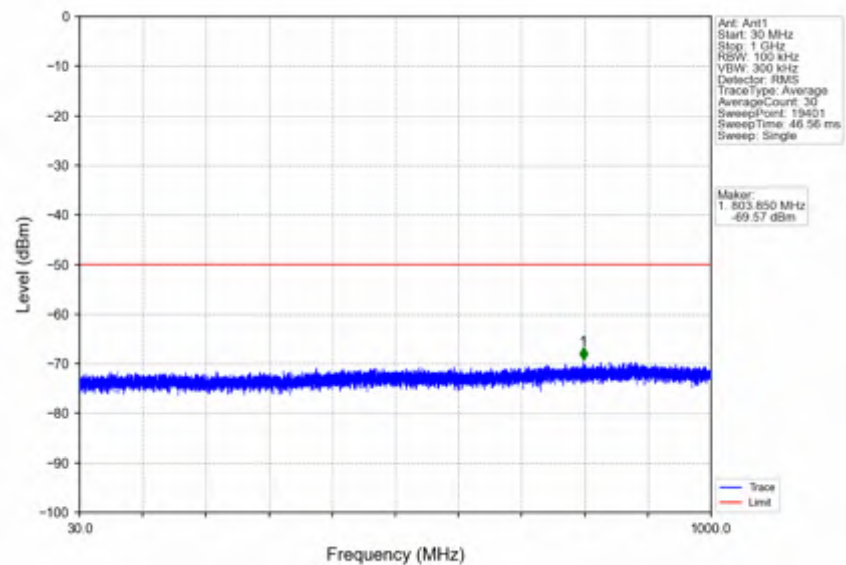
n78d_30kHz_SISO_NTNV_50MHz_DFT-s-OFDM_QPSK_3675MHz_Outer_Full
