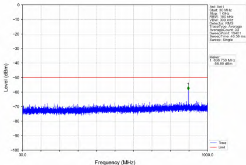
n78d_30kHz_SISO_NTNV_50MHz_DFT-s-OFDM_QPSK_3575.01MHz_Edge_1RB_Left
