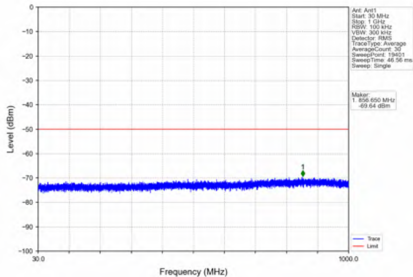
n78d_30kHz_SISO_NTNV_40MHz_CP-OFDM_QPSK_3570MHz_Outer_Full
