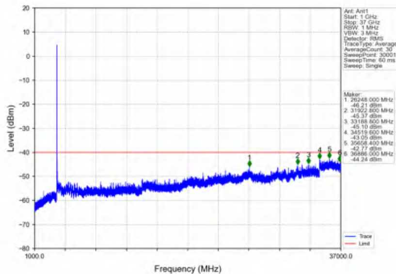
n78d_30kHz_SISO_NTNV_30MHz_CP-OFDM QPSK_3624.99MHz_Edge_1RB_Left
