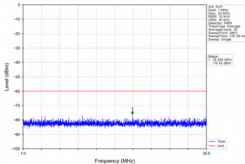
n78d_30kHz_SISO_NTNV_30MHz_CP-OFDM QPSK_3565.02MHz_Outer_Full
