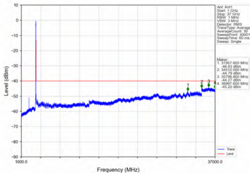
n78d_30kHz_SISO_NTNV_40MHz_DFT-s-OFDM_QPSK_3679.98MHz_Inner_1RB_Right
