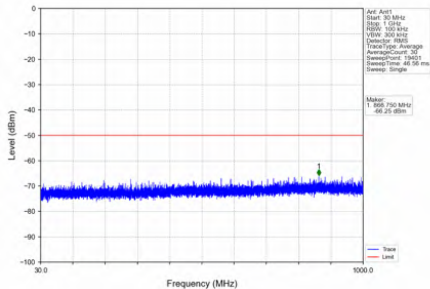
n78d_30kHz_SISO_NTNV_40MHz_CP-OFDM QPSK_3679.98MHz_Inner_1RB_Right
