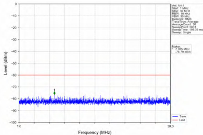
n78d_30kHz_SISO_NTNV_40MHz_CP-OFDM QPSK_3679.98MHz_Edge_1RB_Right
