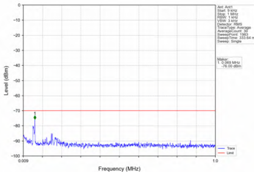
n78d_30kHz_SISO_NTNV_50MHz_DFT-s-OFDM_QPSK_3675MHz_Outer_Full
