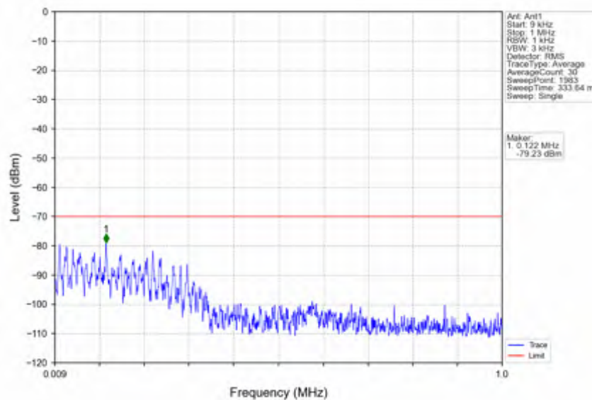
n78d_30kHz_SISO_NTNV_30MHz_CP-OFDM_QPSK_3684.99MHz_Edge_1RB_Right
