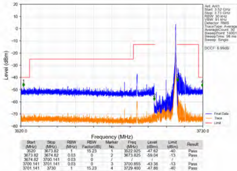
n78d_30kHz_SISO_NTNV_25MHz_DFT-s-OFDM QPSK_3687.48MHz_Inner_1RB_Right
