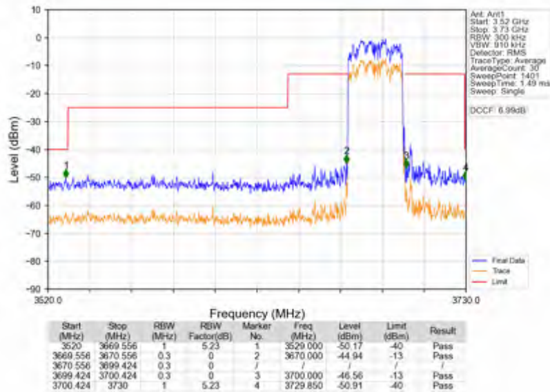
n78d_30kHz_SISO_NTNV_30MHz_DFT-s-OFDM_QPSK_3684.99MHz_Outer_Full
