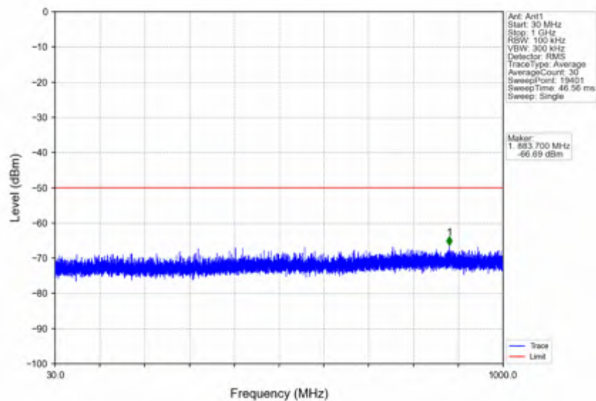
n78d_30kHz_SISO_NTNV_50MHz_DFT-s-OFDM_QPSK_3575.01MHz_Outer_Full
