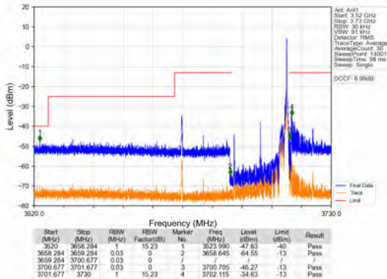
n78d_30kHz_SISO_NTNV_40MHz_DFT-s-OFDM_QPSK_3679.98MHz_Inner_1RB_Right
