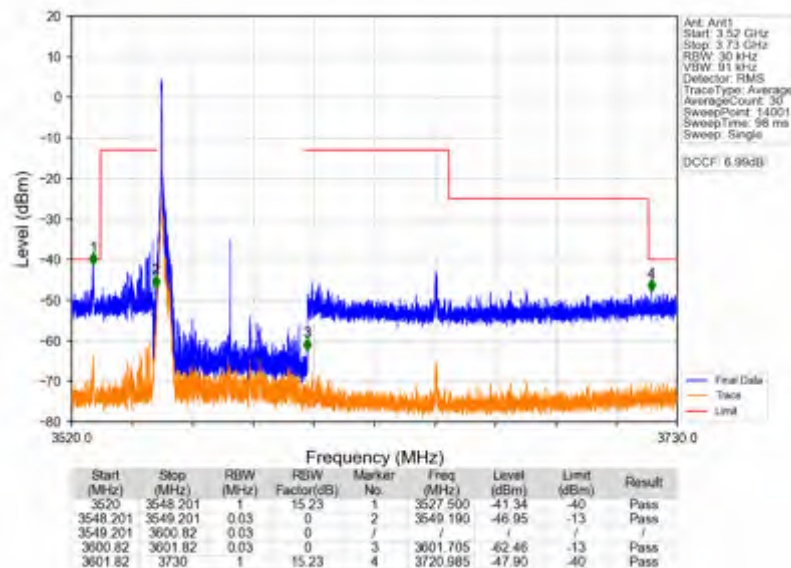
n78d_30kHz_SISO_NTNV_50MHz_DFT-s-OFDM QPSK_3575.01MHz_Edge_1RB_Left
