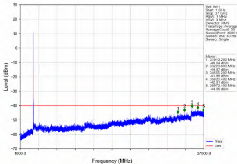
n78d_30kHz_SISO_NTV_40MHz_CP-OFDM QPSK_3624.99MHz_Edge_1RB_Left
