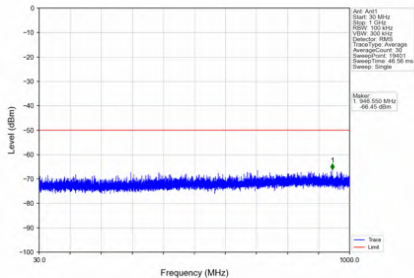
n78d_30kHz_SISO_NTNV_40MHz_CP-OFDM QPSK_3679.98MHz_Edge_1RB_Right
