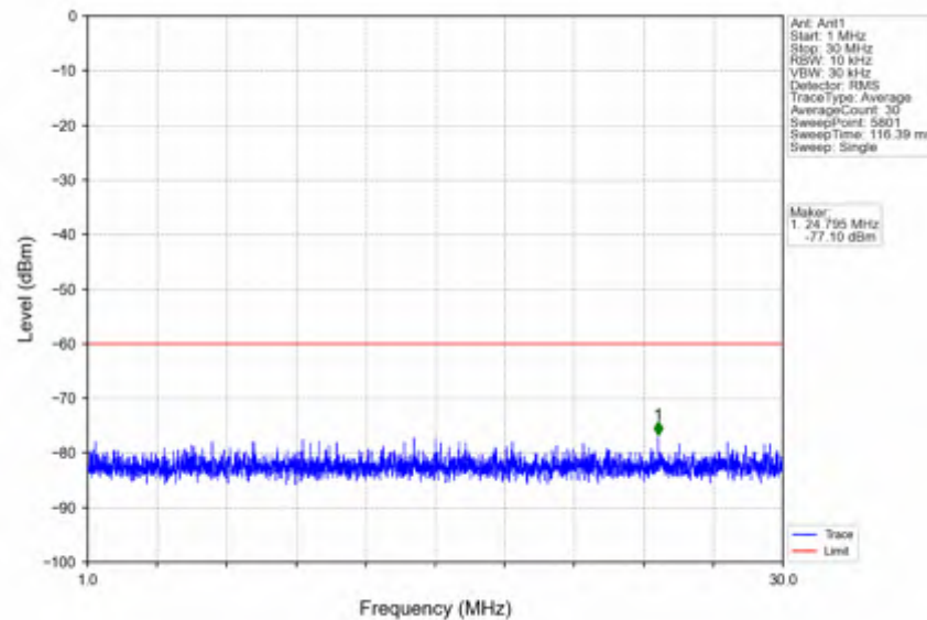
n78d_30kHz_SISO_NTNV_25MHz_CP-OFDM QPSK_3562.5MHz_Edge_1RB_Left
