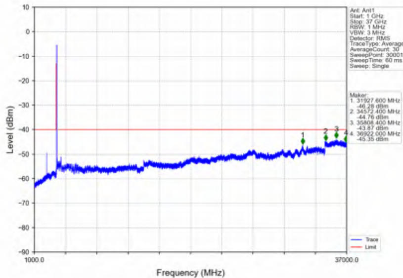
n78d_30kHz_SISO_NTNV_40MHz_CP-OFDM_QPSK_3570MHz_Outer_Full
