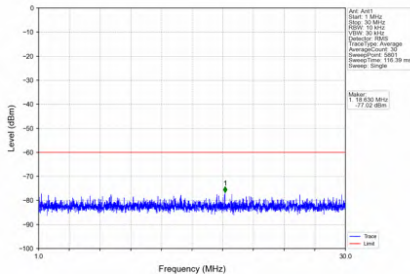
n78d_30kHz_SISO_NTNV_40MHz_CP-OFDM_QPSK_3570MHz_Edge_1RB_Left
