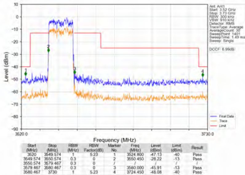
n78d_30kHz_SISO_NTNV_30MHz_DFT-s-OFDM_QPSK_3565.02MHz_Outer_Full
