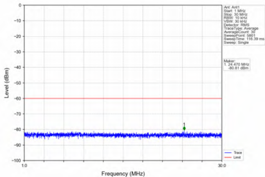
n78d_30kHz_SISO_NTNV_40MHz_CP-OFDM_QPSK_3570MHz_Outer_Full
