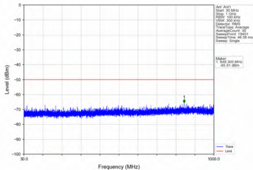
n78d_30kHz_SISO_NTNV_30MHz_CP-OFDM QPSK_3684.99MHz_Edge_1RB_Right
