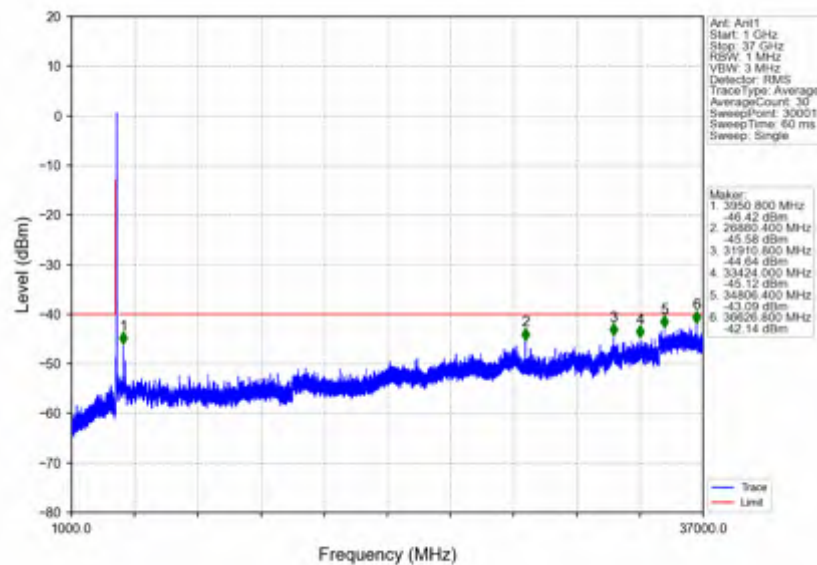
n78d_30kHz_SISO_NTNV_40MHz_DFT-s-OFDM_QPSK_3570MHz_Inner_1RB_Left
