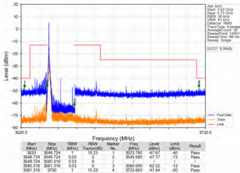
n78d_30kHz_SISO_NTNV_30MHz_DFT-s-OFDM_QPSK_3565.02MHz_Inner_1RB_Left
