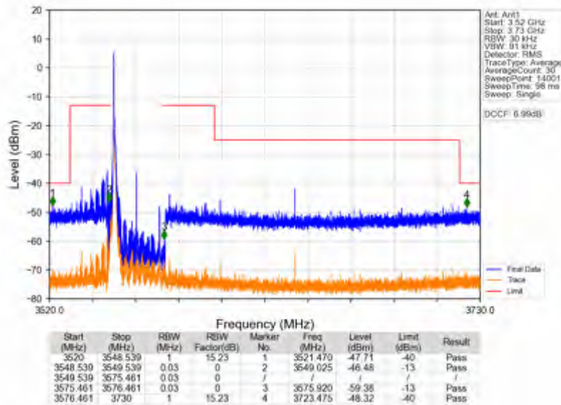
n78d_30kHz_SISO_NTNV_25MHz_DFT-s-OFDM QPSK_3562.5MHz_Inner_1RB_Left
