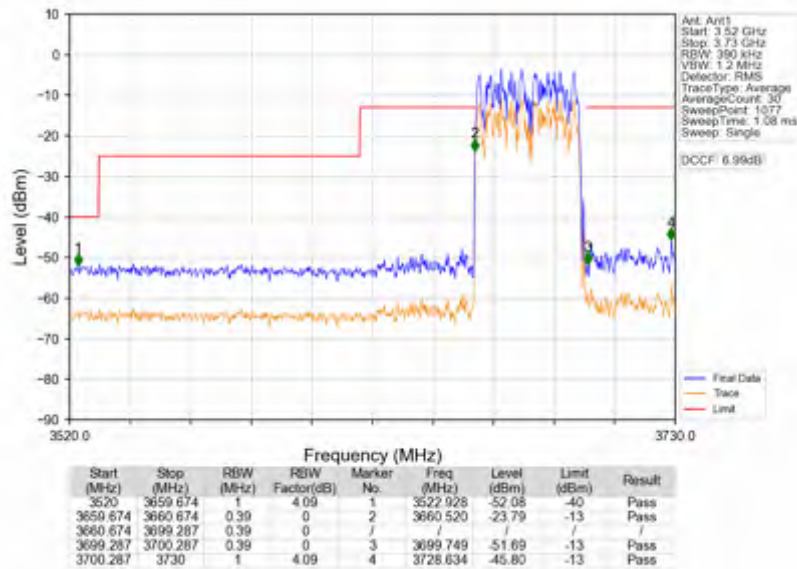
n78d_30kHz_SISO_NTNV_40MHz_DFT-s-OFDM_QPSK_3679.98MHz_Outer_Full
