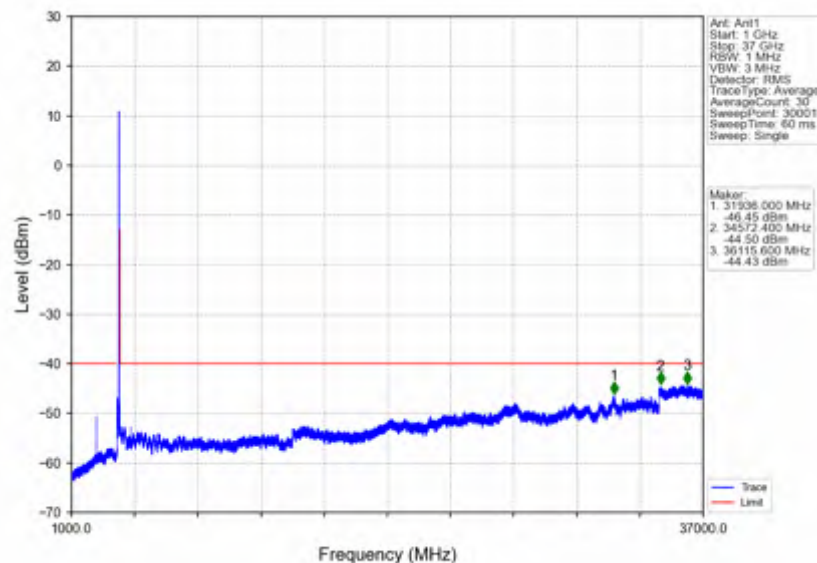
n78d_30kHz_SISO_NTNV_50MHz_DFT-s-OFDM QPSK_3575.01MHz_Edge_1RB_Left
