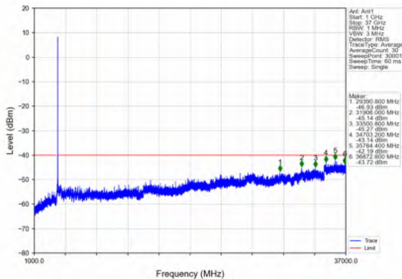
n78d_30kHz_SISO_NTNV_30MHz_CP-OFDM QPSK_3684.99MHz_Outer_Full
