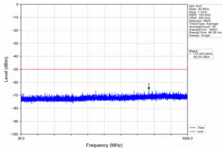
n78d_30kHz_SISO_NTNV_30MHz_CP-OFDM QPSK_3624.99MHz_Edge_1RB_Left
