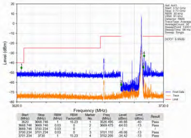
n78d_30kHz_SISO_NTNV_30MHz_DFT-s-OFDM QPSK_3684.99MHz_Inner_1RB_Right
