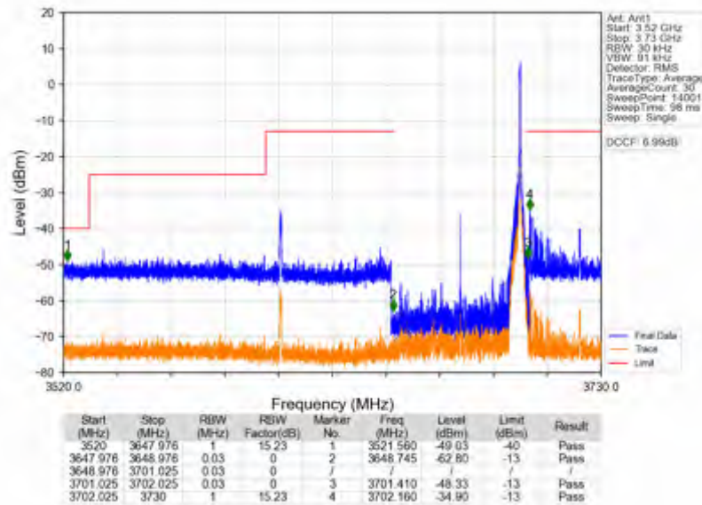
n78d_30kHz_SISO_NTNV_50MHz_DFT-s-OFDM QPSK_3675MHz_Inner_1RB_Right
