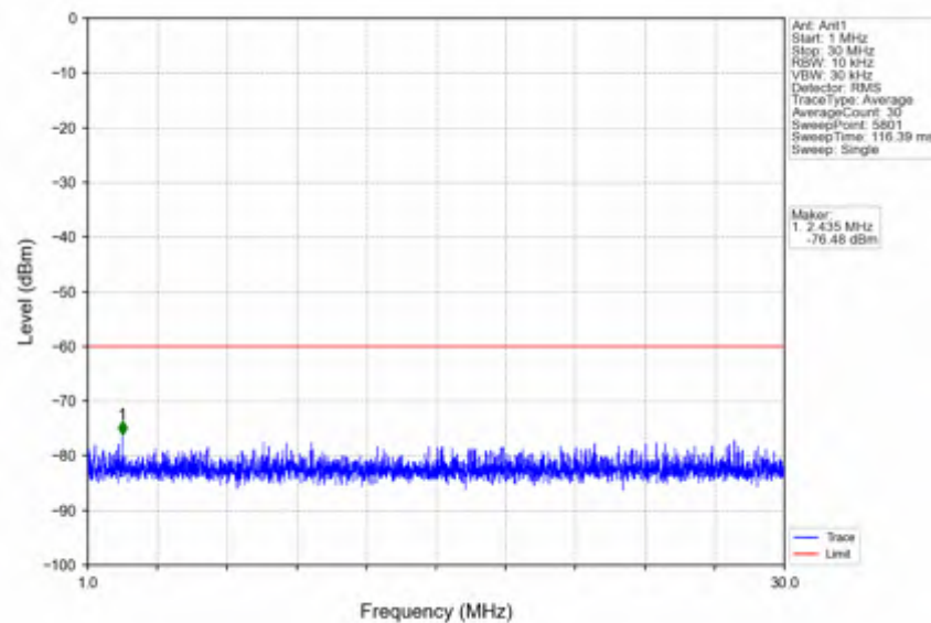
n78d_30kHz_SISO_NTNV_30MHz_CP-OFDM QPSK_3684.99MHz_Outer_Full
