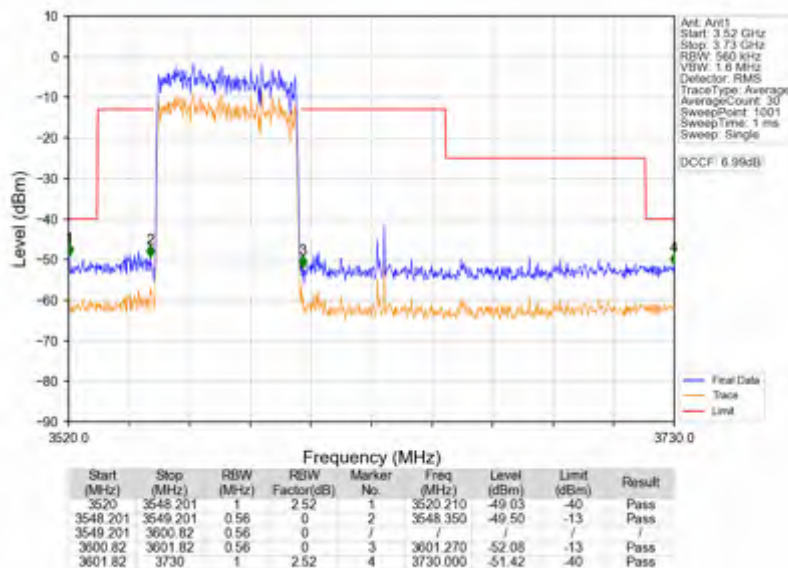
n78d_30kHz_SISO_NTV_50MHz_CP-OFDM QPSK_3575.01MHz_Outer_Full
