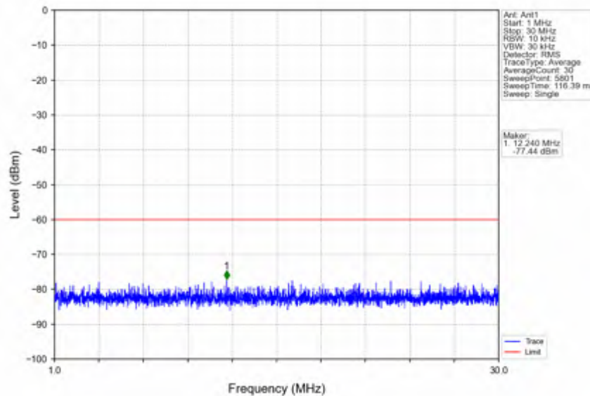
n78d_30kHz_SISO_NTNV_40MHz_CP-OFDM QPSK_3570MHz_Inner_1RB_Left
