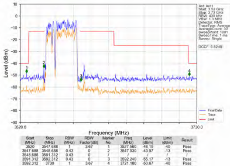
n78d_30kHz_SISO_NTNV_40MHz_DFT-s-OFDM_QPSK_3570MHz_Outer_Full
