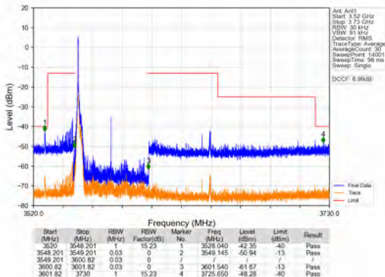
n78d_30kHz_SISO_NTNV_50MHz_DFT-s-OFDM_QPSK_3575.01MHz_Inner_1RB_Left
