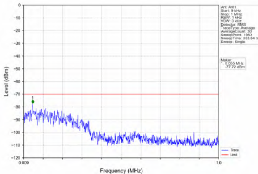
n78d_30kHz_SISO_NTNV_25MHz_CP-OFDM QPSK_3562.5MHz_Inner_1RB_Left
