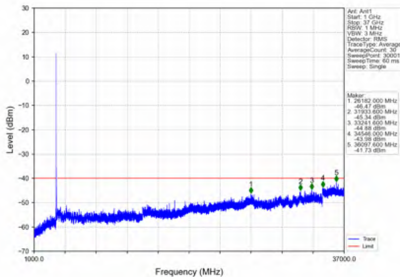
n78d_30kHz_SISO_NTNV_25MHz_CP-OFDM QPSK_3562.5MHz_Outer_Full
