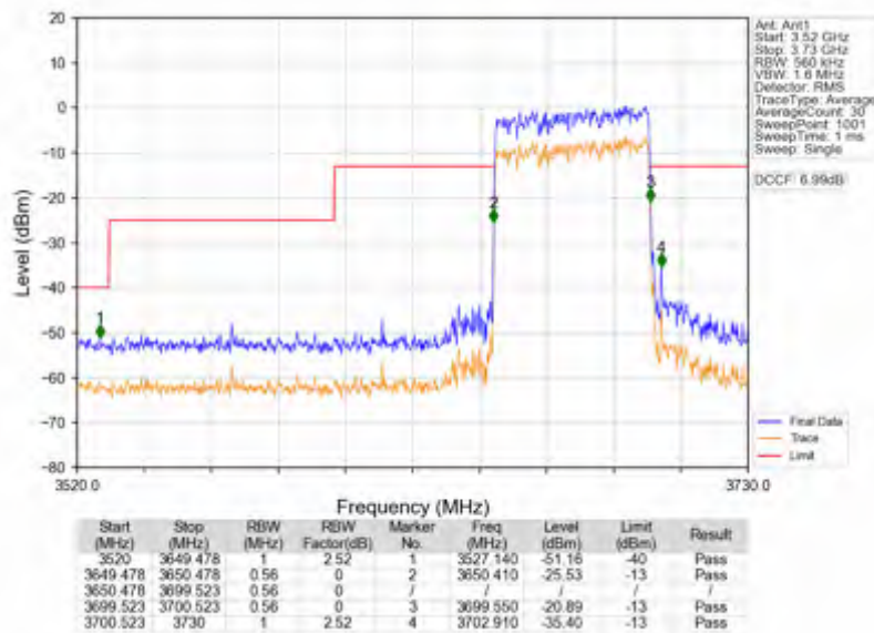
n78d_30kHz_SISO_NTNV_50MHz_CP-OFDM QPSK_3675MHz_Outer_Full
