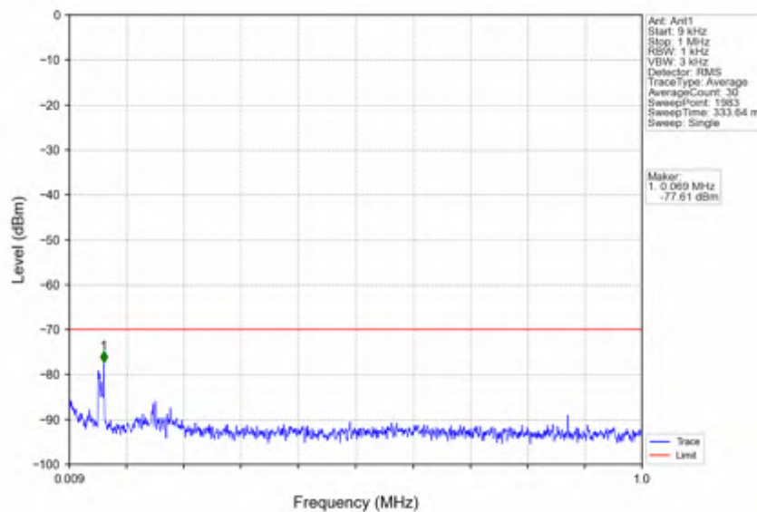
n78d_30kHz_SISO_NTNV_40MHz_DFT-s-OFDM_QPSK_3679.98MHz_Outer_Full
