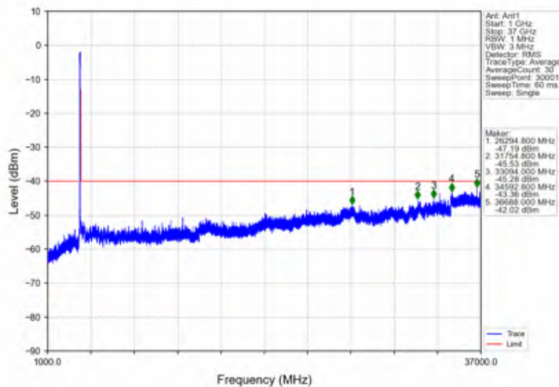
n78d_30kHz_SISO_NTNV_50MHz_CP-OFDM_QPSK_3675MHz_Outer_Full
