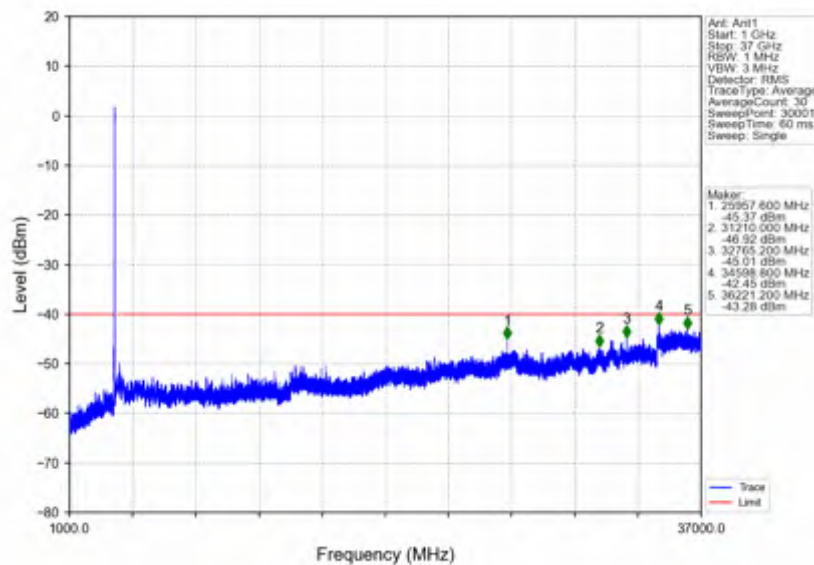
n78d_30kHz_SISO_NTNV_25MHz_DFT-s-OFDM QPSK_3562.5MHz_Inner_1RB_Left
