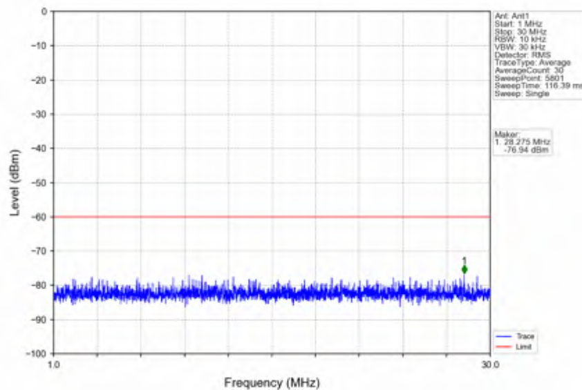
n78d_30kHz_SISO_NTNV_40MHz_DFT-s-OFDM QPSK_3570MHz_Edge_1RB_Left
