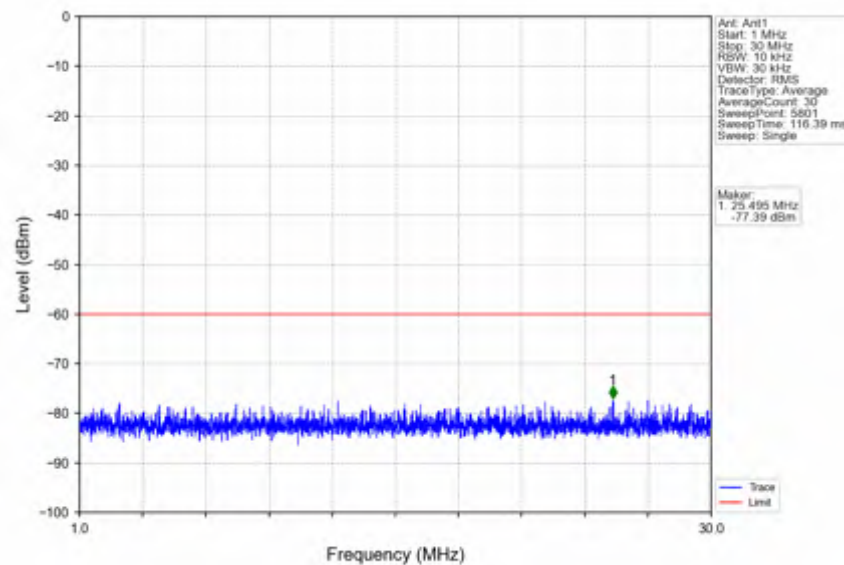
n78d_30kHz_SISO_NTNV_30MHz_DFT-s-OFDM QPSK_3684.99MHz_Inner_1RB_Right
