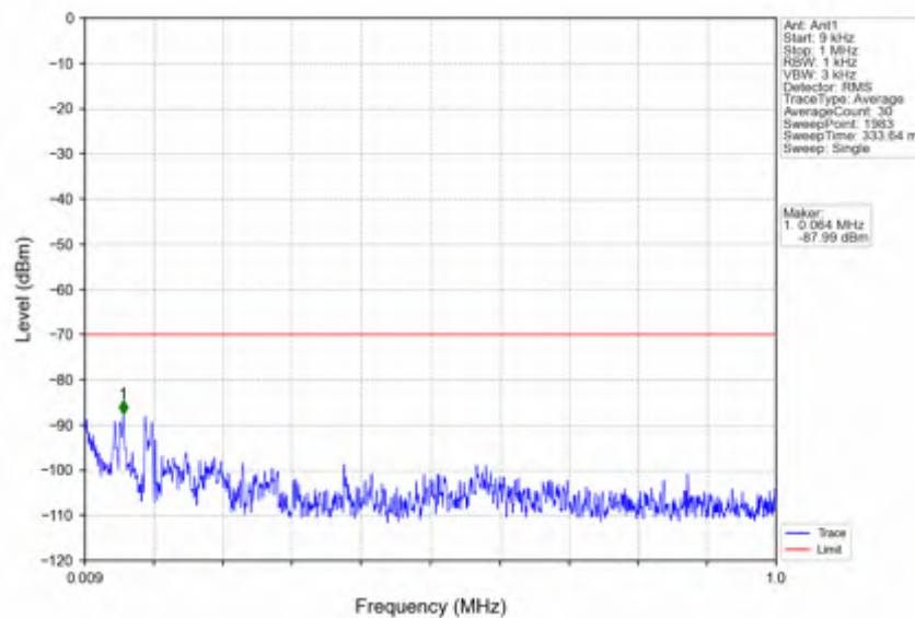
n78d_30kHz_SISO_NTNV_40MHz_DFT-s-OFDM_QPSK_3570MHz_Outer_Full
