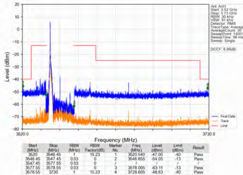
n78d_30kHz_SISO_NTNV_25MHz_CP-OFDM QPSK_3562.5MHz_Inner_1RB_Left
