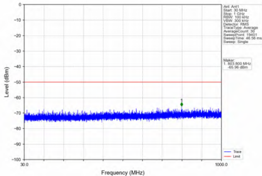
n78d_30kHz_SISO_NTNV_25MHz_DFT-s-OFDM_QPSK_3687.48MHz_Outer_Full
