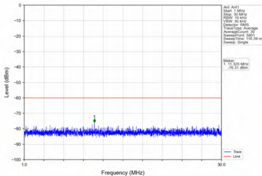
n78d_30kHz_SISO_NTNV_30MHz_DFT-s-OFDM_QPSK_3565.02MHz_Outer_Full
