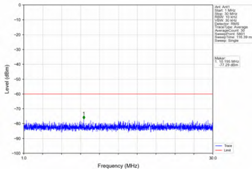
n78d_30kHz_SISO_NTNV_50MHz_CP-OFDM QPSK_3675MHz_Edge_1RB_Right
