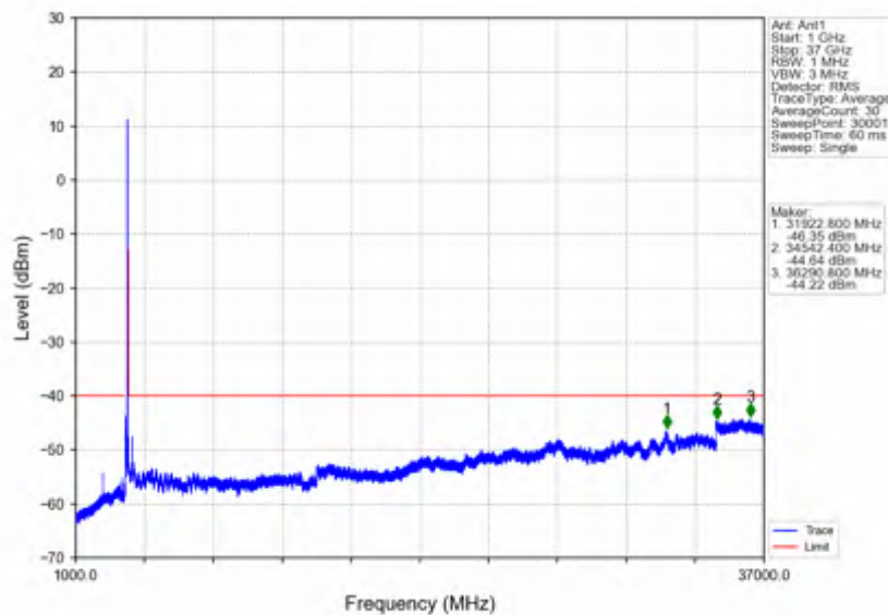
n78d_30kHz_SISO_NTNV_50MHz_DFT-s-OFDM_PI/2_BPSK_3675MHz_Outer_Full
