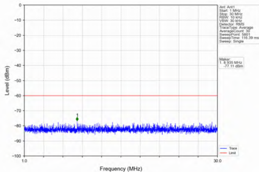
n78d_30kHz_SISO_NTNV_50MHz_DFT-s-OFDM QPSK_3675MHz_Edge_1RB_Right
