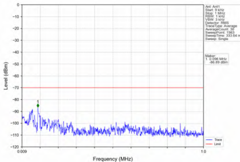
n78d_30kHz_SISO_NTNV_30MHz_DFT-s-OFDM_QPSK_3565.02MHz_Outer_Full
