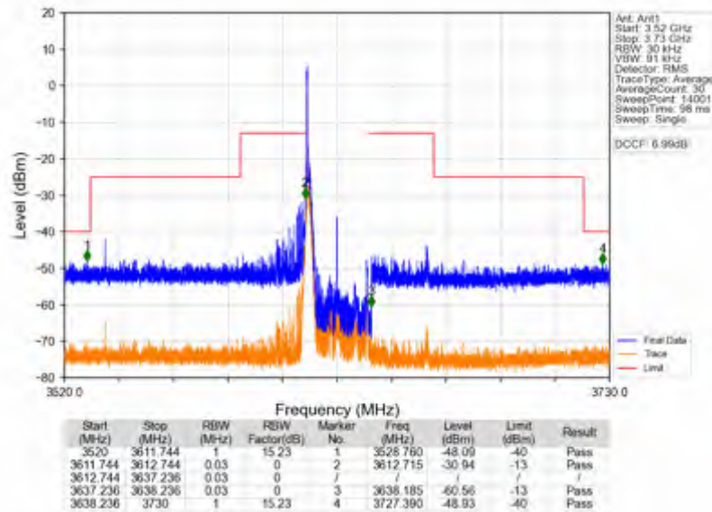
n78d_30kHz_SISO_NTNV_25MHz_CP-OFDM QPSK_3624.99MHz_Edge_1RB_Left
