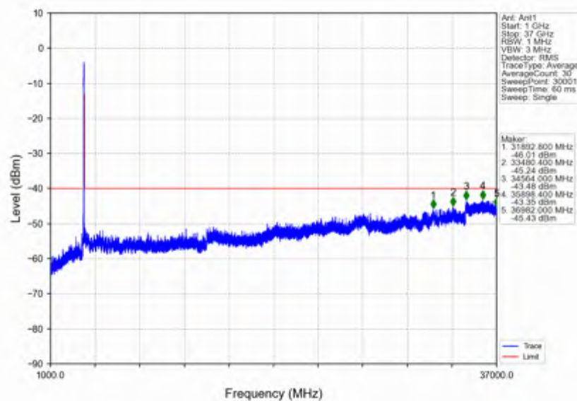
n78d_30kHz_SISO_NTNV_40MHz_CP-OFDM QPSK_3679.98MHz_Outer_Full
