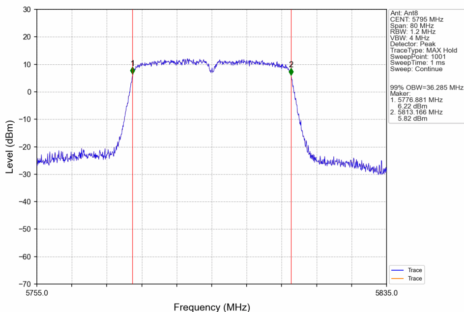
802.11ac(VHT40)_HCH_5795MHz_Ant8_NTNV
