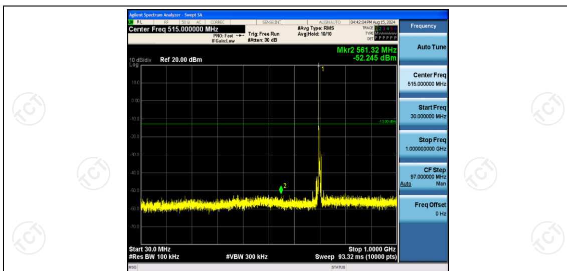
Band17-5MHz-QPSK-23755-1RB#0-Range1:30~1000MHz
