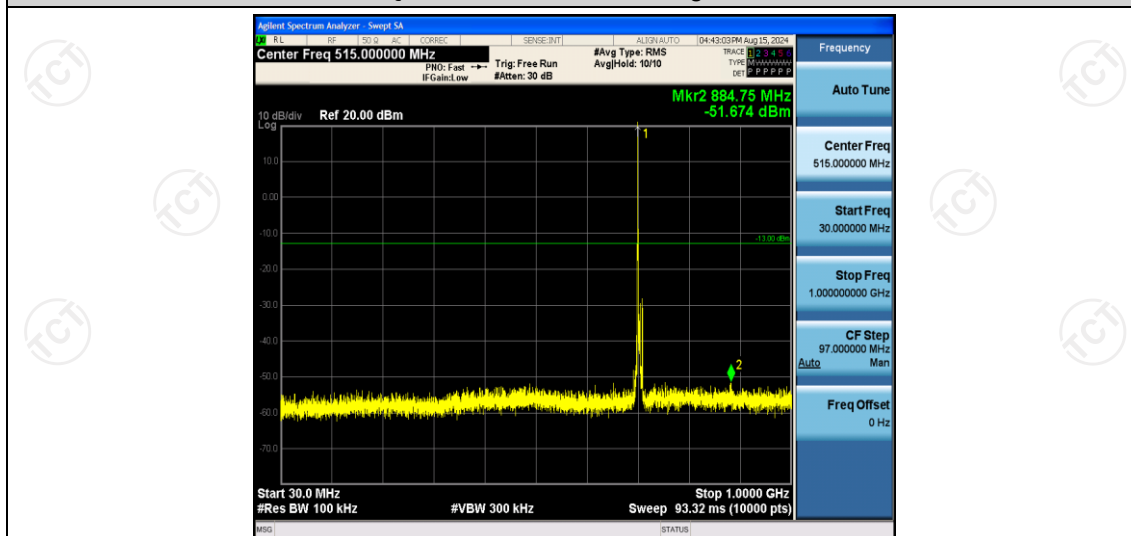
Band17-5MHz-QPSK-23790-1RB#0-Range1:30~1000MHz
