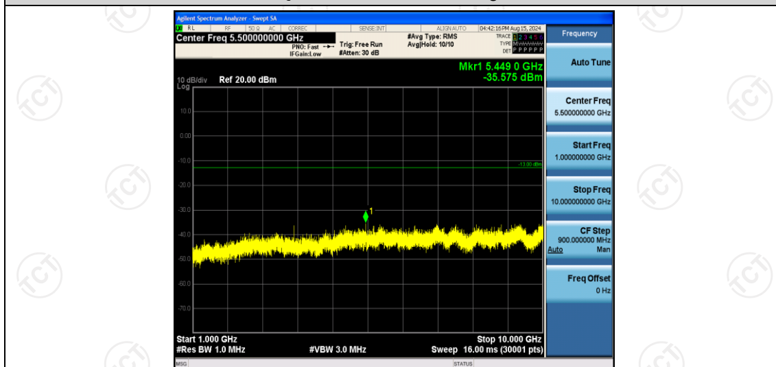
Band17-5MHz-QPSK-23755-1RB#0-Range2:1000~10000MHz
