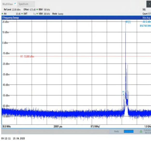
Band26(824-849)-15MHz-QPSK-26915-1RB#0-30~1000-PASS
