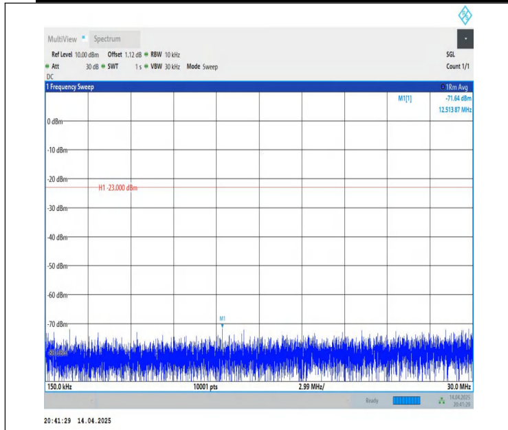
Band26(824-849)-10MHz-QPSK-26840-1RB#49-0.15~30-PASS
