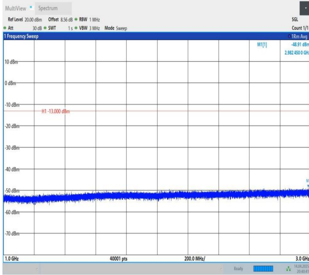
Band26(824-849)-5MHz-QPSK-27015-1RB#24-1000~3000-PASS
