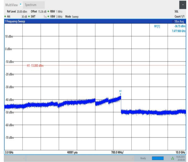
Band26(824-849)-5MHz-QPSK-27015-1RB#24-3000~10000-PASS
