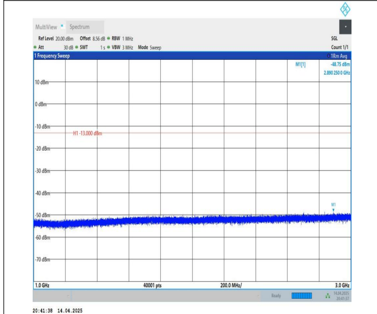
Band26(824-849)-10MHz-QPSK-26840-1RB#49-1000~3000-PAS
