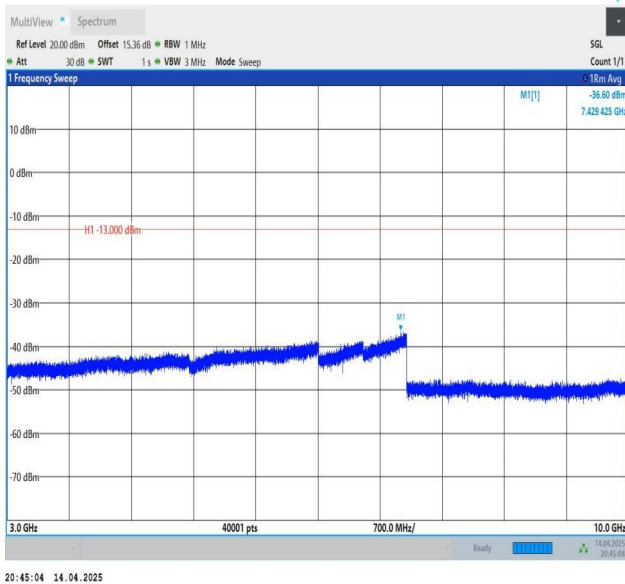
Band26(824-849)-15MHz-QPSK-26915-1RB#0-3000~10000-PAS
