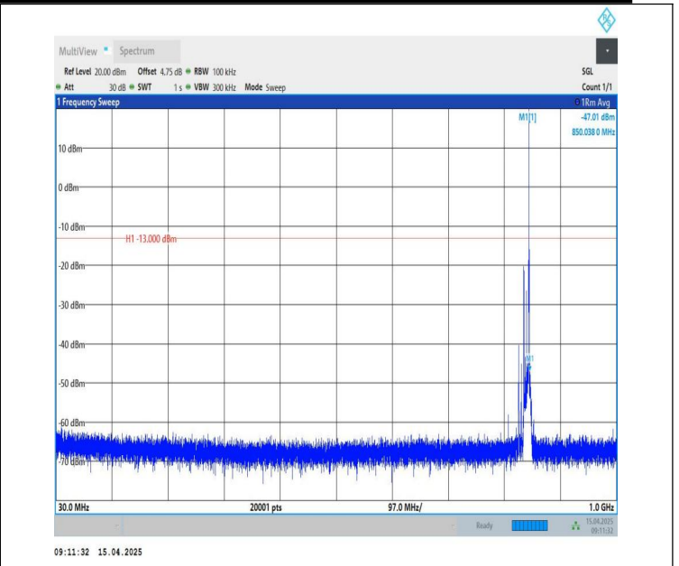
Band26(824-849)-10MHz-QPSK-26990-1RB#49-30~1000-PASS
