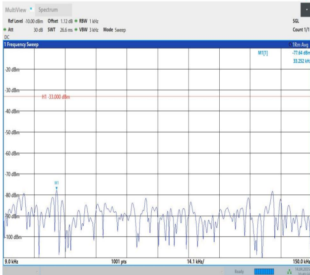
Band26(824-849)-10MHz-QPSK-26840-1RB#0-0.009~0.15-PASS
