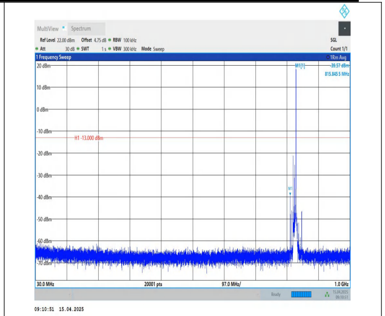
Band26(824-849)-10MHz-QPSK-26840-1RB#49-30~1000-PASS
