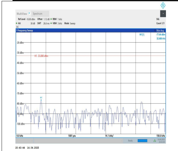
Band26(824-849)-15MHz-QPSK-26865-1RB#0-0.009~0.15-PASS
