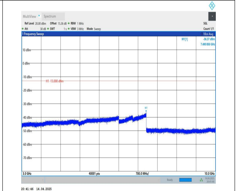
Band26(824-849)-10MHz-QPSK-26840-1RB#49-3000~10000-PAS
