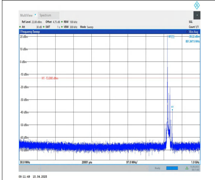
Band26(824-849)-15MHz-QPSK-26865-1RB#0-30~1000-PASS
