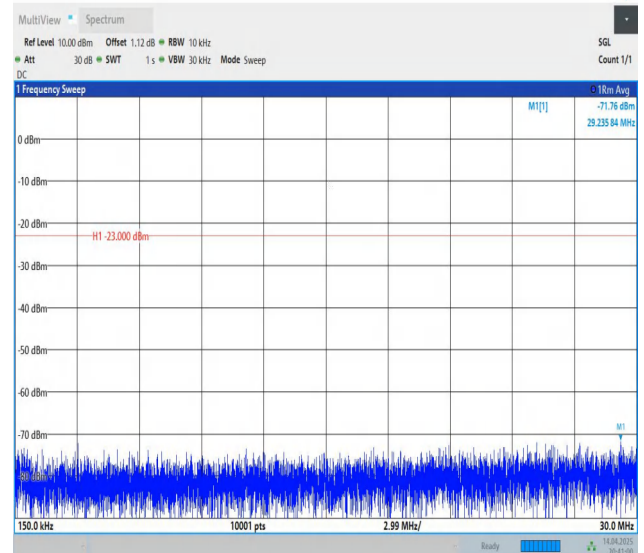
Band26(824-849)-10MHz-QPSK-26840-1RB#0-0.15~30-PASS
