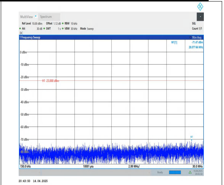
Band26(824-849)-15MHz-QPSK-26865-1RB#0-0.15~30-PASS
