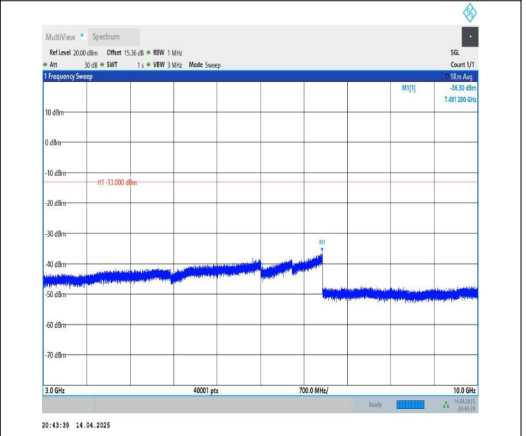
Band26(824-849)-10MHz-QPSK-26990-1RB#49-3000~10000-PAS
