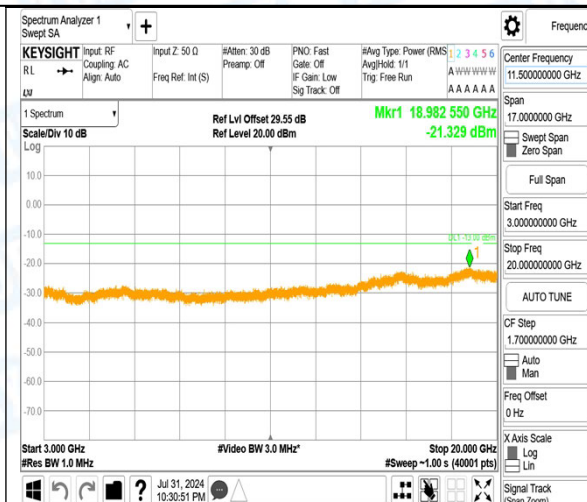
Band4_10MHz_QPSK_20175_50RB#0_0.15~30_0.15~30
