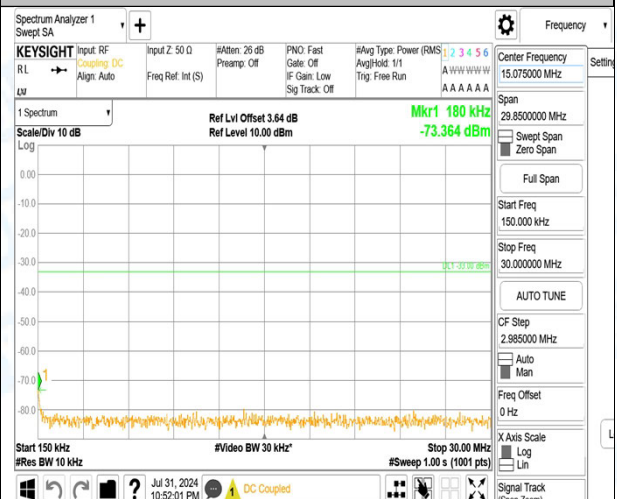
Band4_10MHz_QPSK_20000_50RB#0_1000~3000_1000~3000
