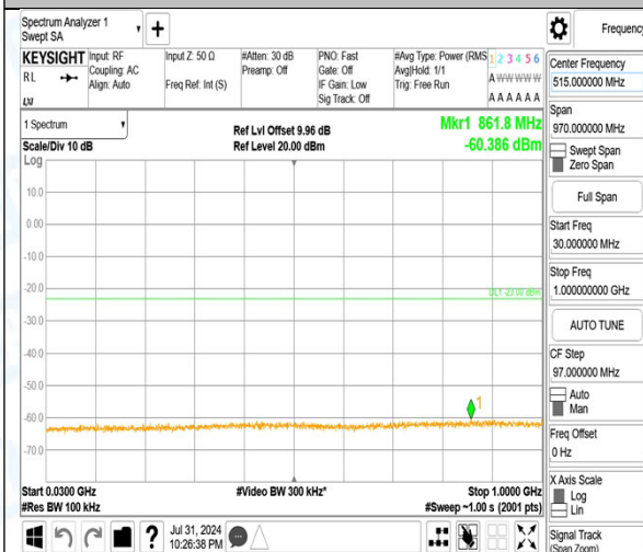
Band4_10MHz_16QAM_20000_1RB#49_3000~20000_3000~200
