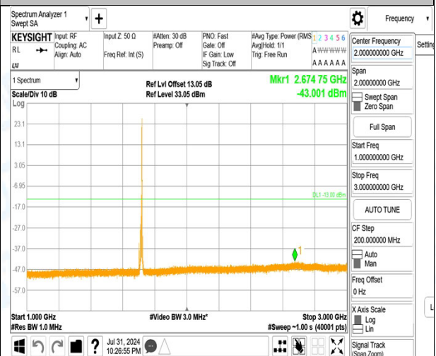
Band4_10MHz_16QAM_20000_1RB#49_1000~3000_1000~3000
