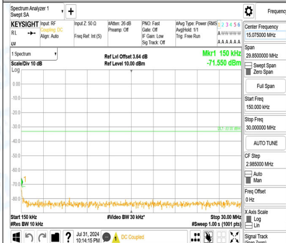
Band4_10MHz_16QAM_20000_1RB#0_0.15~30_0.15~30
