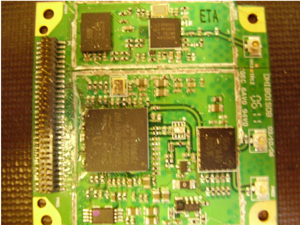
Shields Removed
