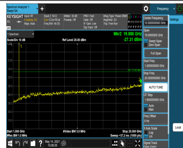
Band2-1.4MHz-QPSK-18900-1RB#0-Range2:1000~20
