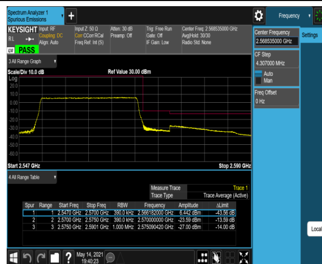
Band7-20MHz-QPSK-21350-100RB#0
