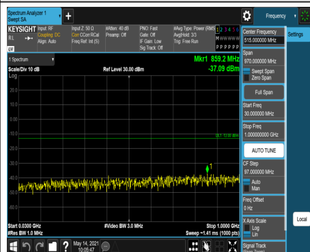
Band2-1.4MHz-16QAM-18607-1RB#0-Range1:30~1
