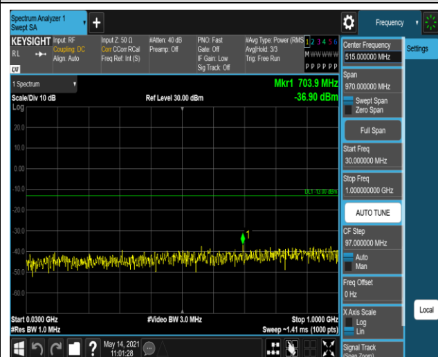
Band2-20MHz-QPSK-18900-1RB#0-Range1:30~10
