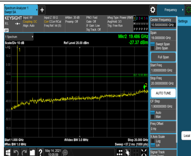
Band2-1.4MHz-16QAM-18607-1RB#0-Range2:1000~2
