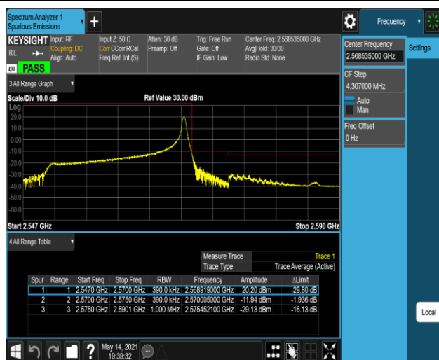
Band7-20MHz-QPSK-21350-1RB#99
