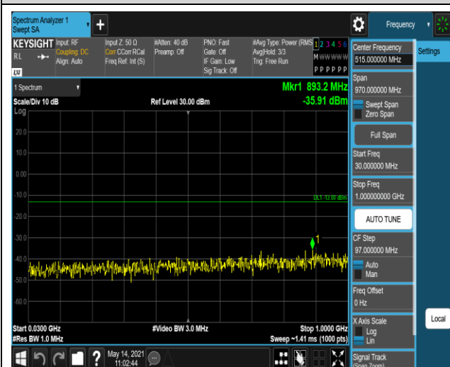
Band2-20MHz-16QAM-19100-1RB#0-Range1:30~1
