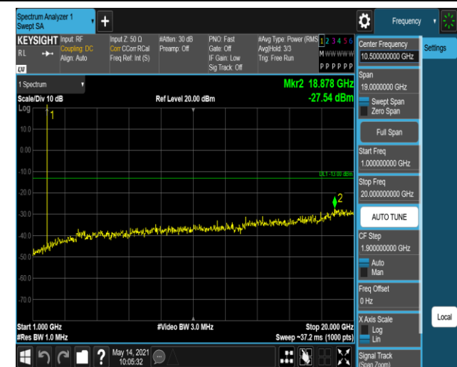
Band2-1.4MHz-QPSK-18900-1RB#0-Range2:1000~20
