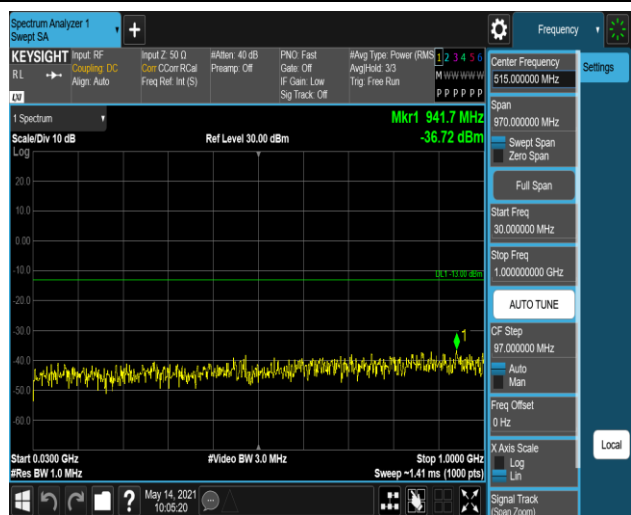
Band2-1.4MHz-QPSK-18900-1RB#0-Range1:30~10
