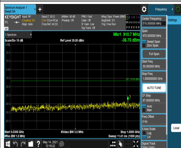
Band4-20MHz-QPSK-20175-1RB#0-Range1:30~10
