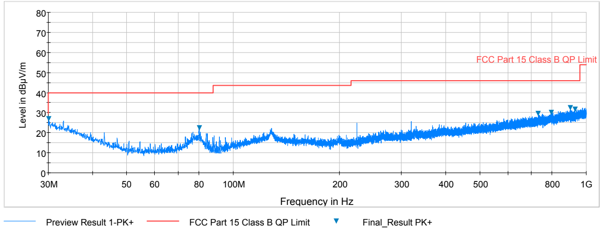
Plot 7-23. Radiated Spurious Plot below 1GHz (Pol. H)
