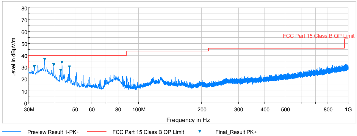
Plot 7-24. Radiated Spurious Plot below 1GHz (Pol. V)
