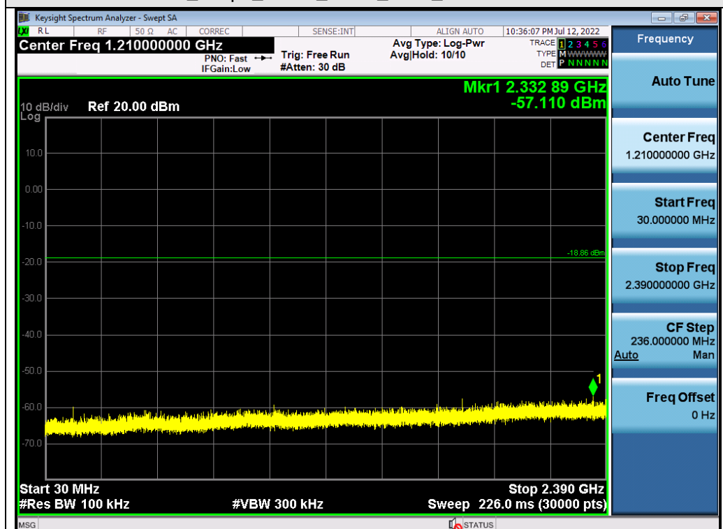
Test_Graph_GFSK_ANT1_2420_Lower Band Emissions
