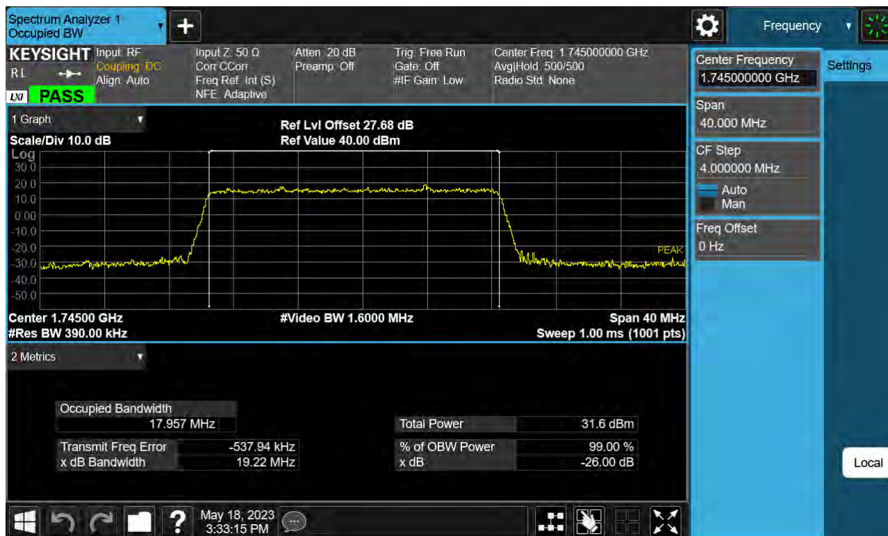
Sub6 n66. Occupied Bandwidth Plot (20 M BW Ch.349000 BPSK Full RB)
