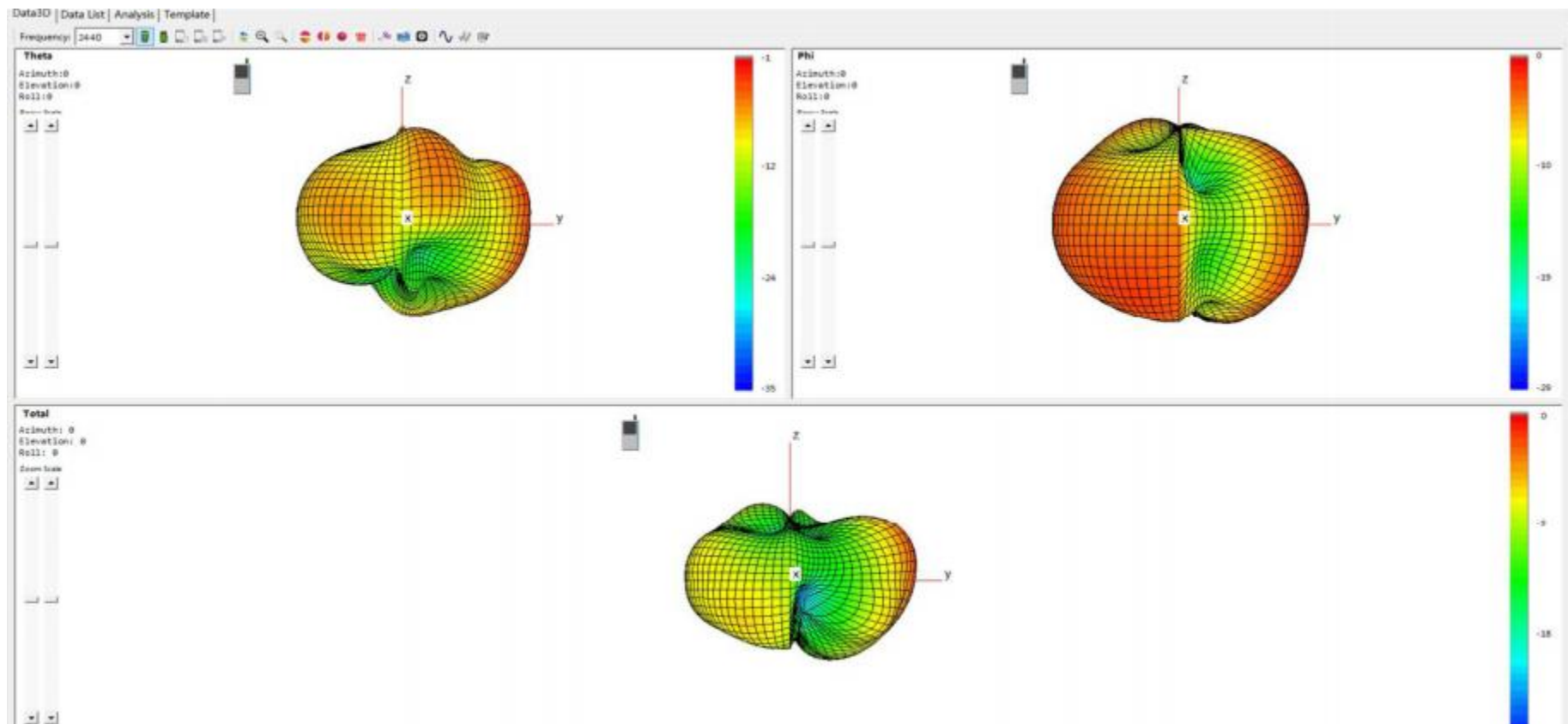
3D Radiation Pattern for 2440MHz
