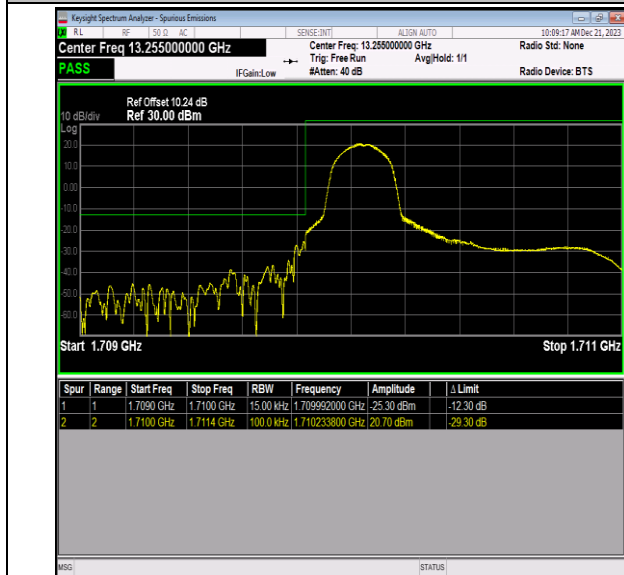
Band66_1.4MHz_QPSK_131979_1RB#0
