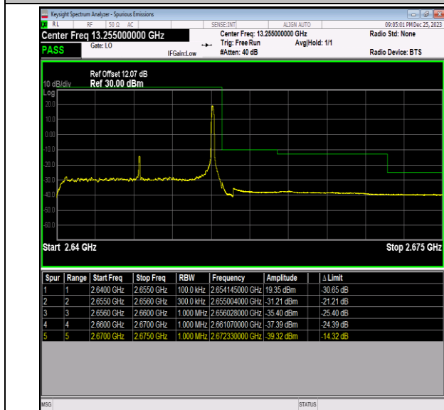
Band41_15MHz_QPSK_41165_1RB#74
