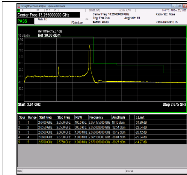
Band41_15MHz_16QAM_41165_1RB#74
