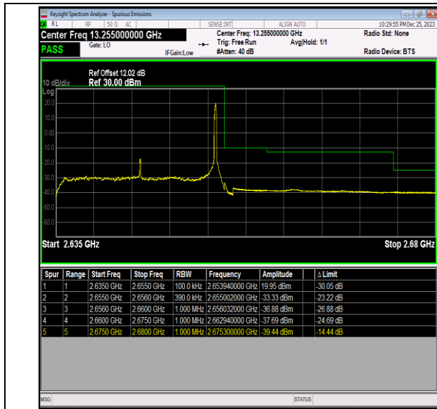
Band41_20MHz_QPSK_41140_1RB#99
