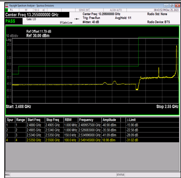
Band41_15MHz_QPSK_40115_1RB#74
