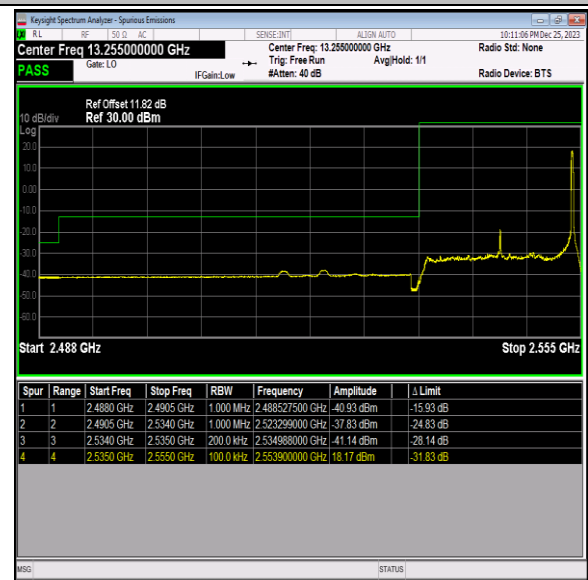
Band41_20MHz_16QAM_40140_1RB#99
