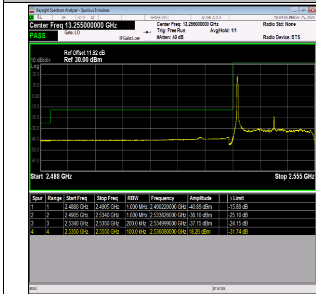
Band41_20MHz_16QAM_40140_1RB#0
