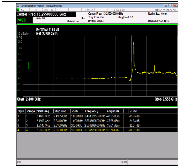
Band41_20MHz_64QAM_40140_1RB#0
