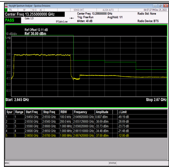
Band41_10MHz_64QAM_41190_50RB#0
