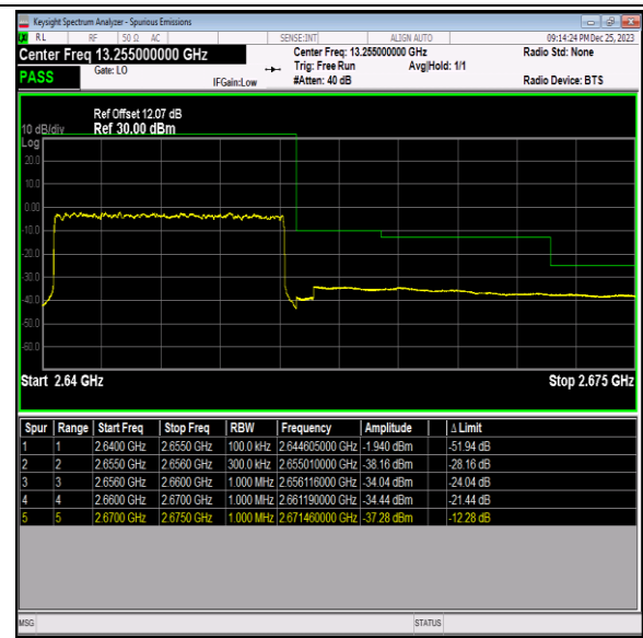
Band41_15MHz_16QAM_41165_75RB#0
