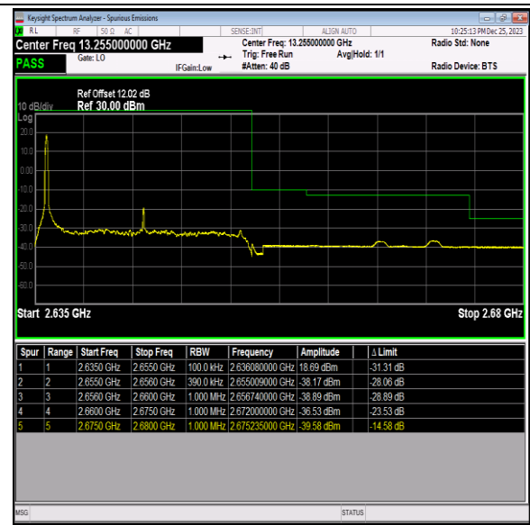
Band41_20MHz_16QAM_41140_1RB#0
