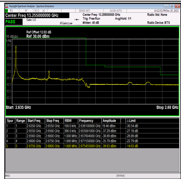
Band41_20MHz_QPSK_41140_1RB#0
