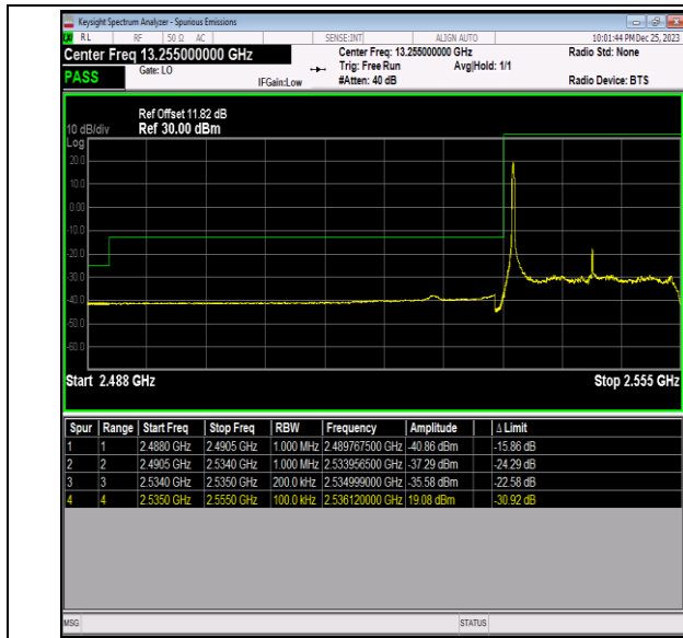
Band41_20MHz_QPSK_40140_1RB#0
