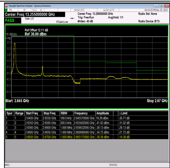
Band41_10MHz_64QAM_41190_1RB#0
