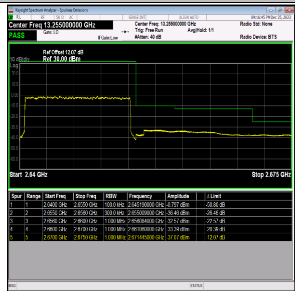
Band41_15MHz_64QAM_41165_75RB#0
