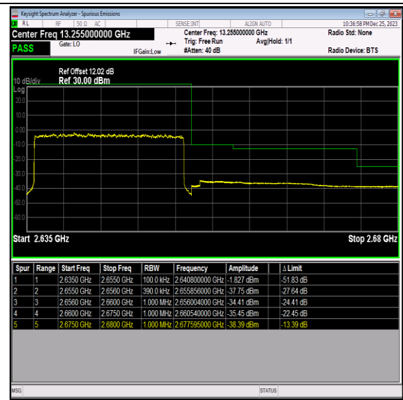
Band41_20MHz_QPSK_41140_100RB#0
