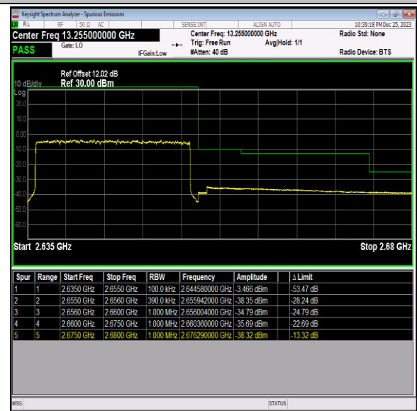
Band41_20MHz_16QAM_41140_100RB#0
