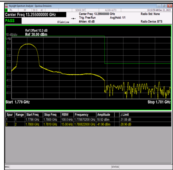
Band66_1.4MHz_16QAM_132665_1RB#0
