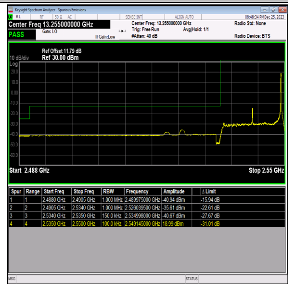
Band41_15MHz_64QAM_40115_1RB#74
