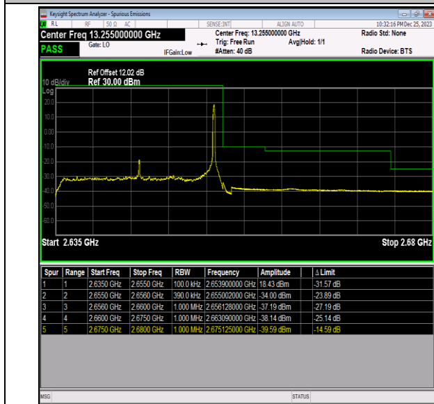
Band41_20MHz_16QAM_41140_1RB#99
