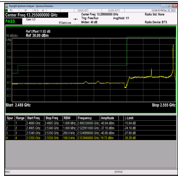
Band41_20MHz_QPSK_40140_1RB#99
