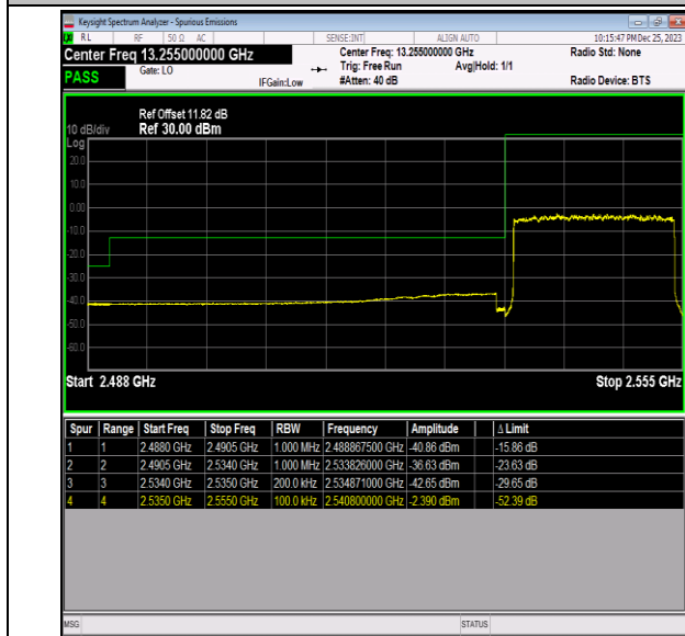
Band41_20MHz_QPSK_40140_100RB#0
