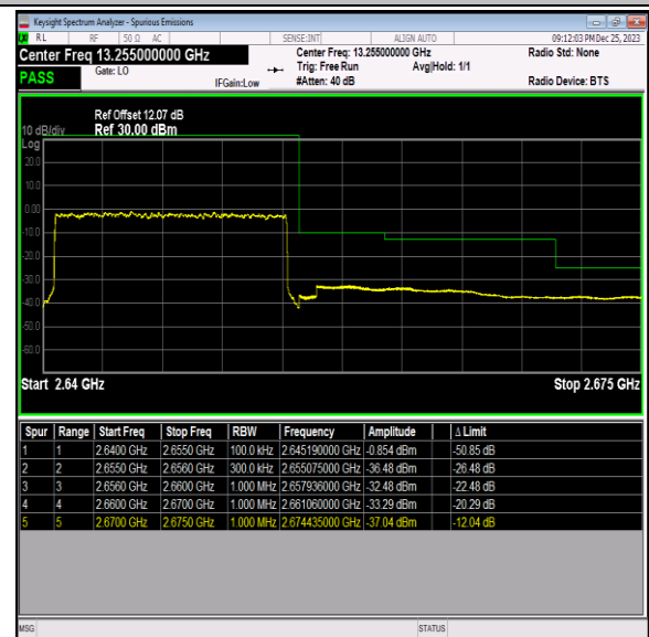
Band41_15MHz_QPSK_41165_75RB#0
