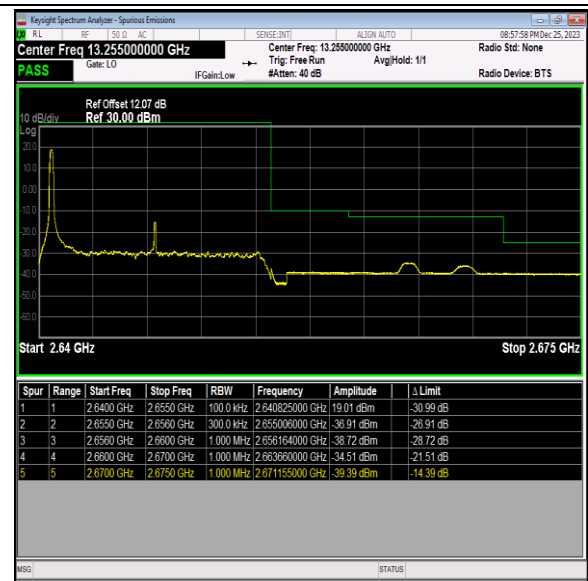
Band41_15MHz_QPSK_41165_1RB#0
