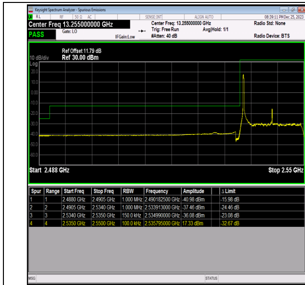
Band41_15MHz_16QAM_40115_1RB#0
