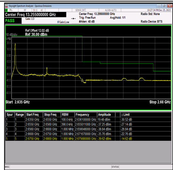
Band41_20MHz_64QAM_41140_1RB#0
