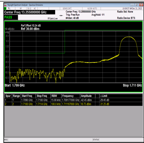
Band66_1.4MHz_16QAM_131979_1RB#5
