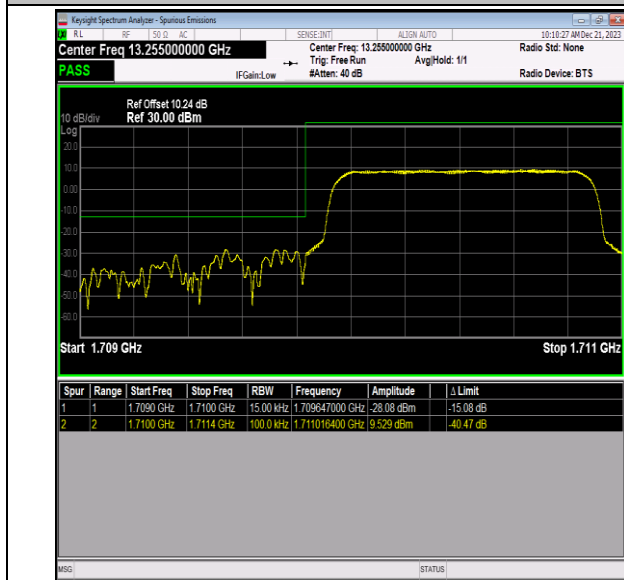
Band66_1.4MHz_16QAM_131979_6RB#0
