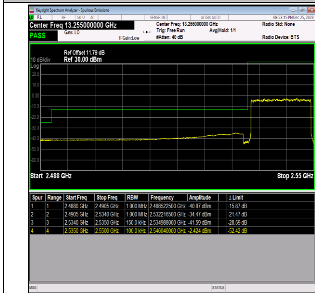
Band41_15MHz_16QAM_40115_75RB#0
