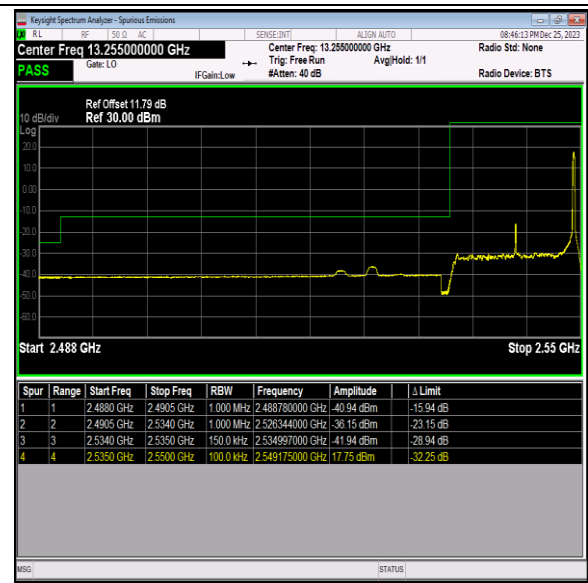
Band41_15MHz_16QAM_40115_1RB#74
