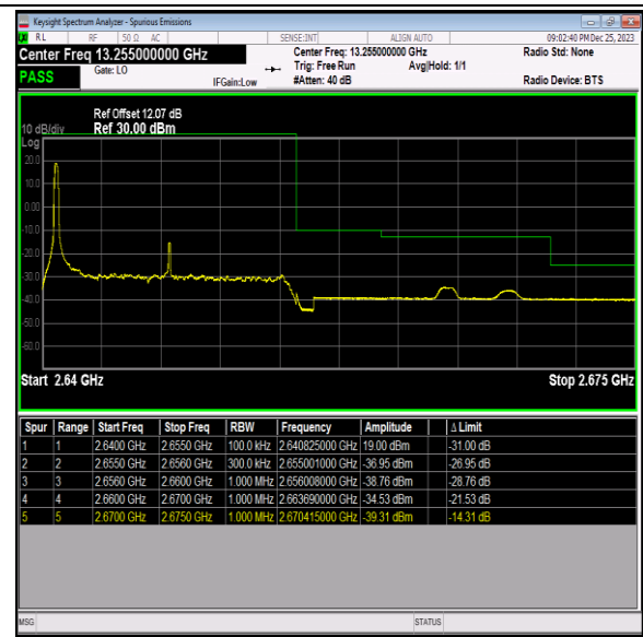
Band41_15MHz_64QAM_41165_1RB#0
