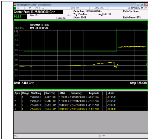
Band41_15MHz_64QAM_40115_75RB#0
