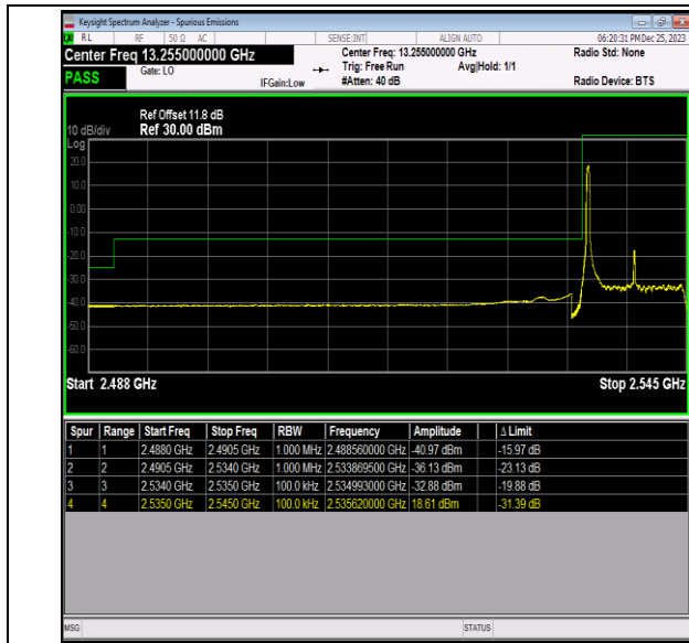
Band41_10MHz_64QAM_40090_1RB#0
