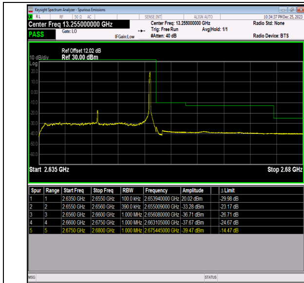
Band41_20MHz_64QAM_41140_1RB#99
