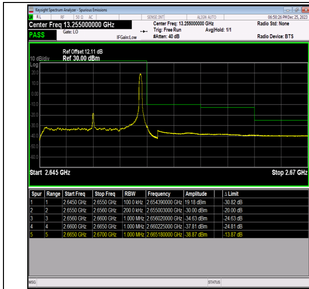
Band41_10MHz_64QAM_41190_1RB#49
