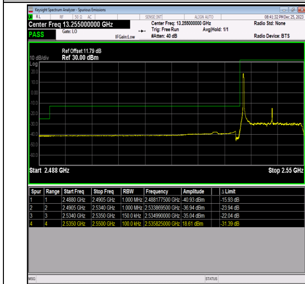
Band41_15MHz_64QAM_40115_1RB#0
