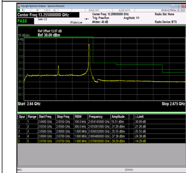
Band41_15MHz_64QAM_41165_1RB#74
