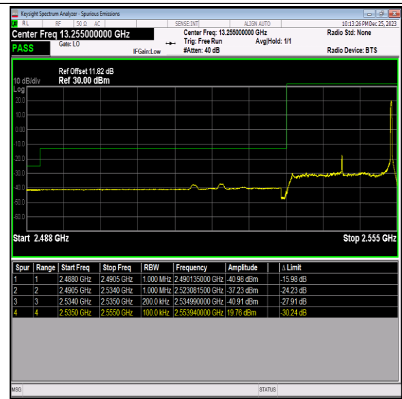
Band41_20MHz_64QAM_40140_1RB#99
