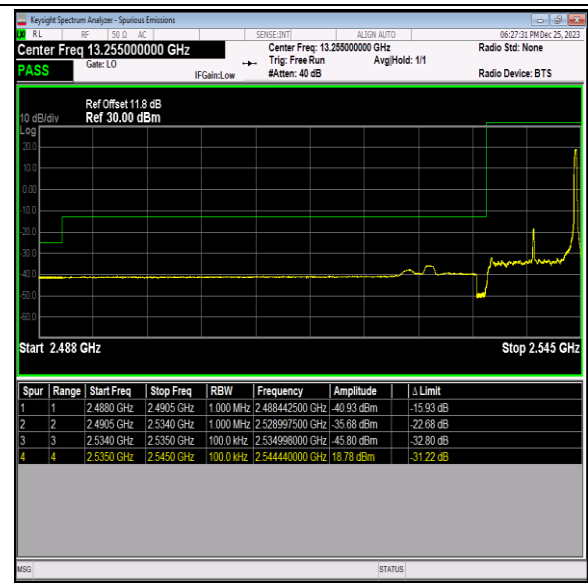
Band41_10MHz_64QAM_40090_1RB#49
