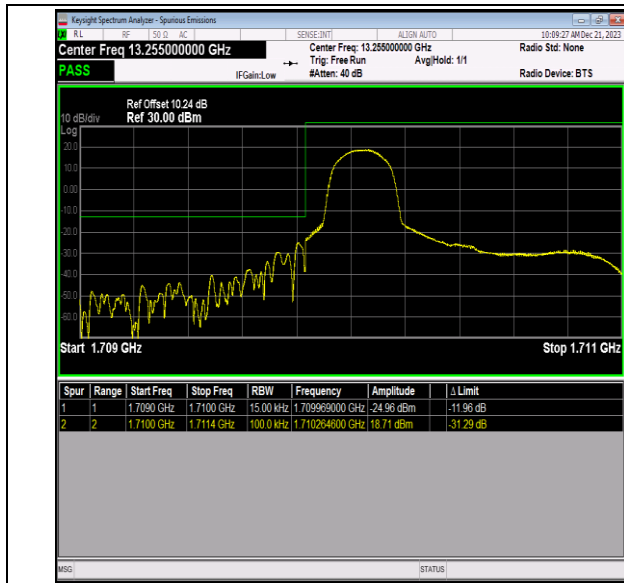
Band66_1.4MHz_16QAM_131979_1RB#0
