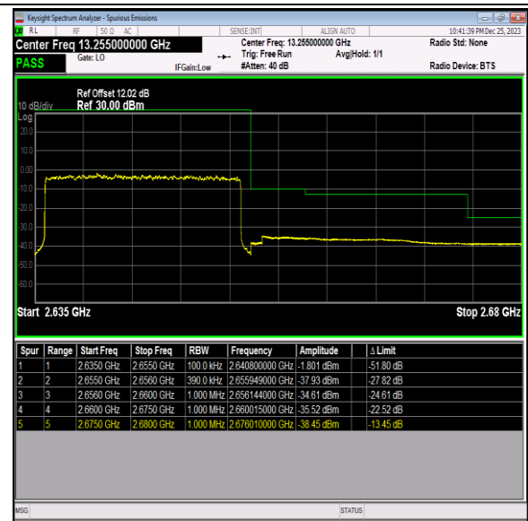
Band41_20MHz_64QAM_41140_100RB#0
