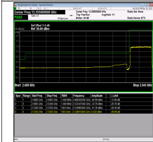
Band41_10MHz_64QAM_40090_50RB#0
