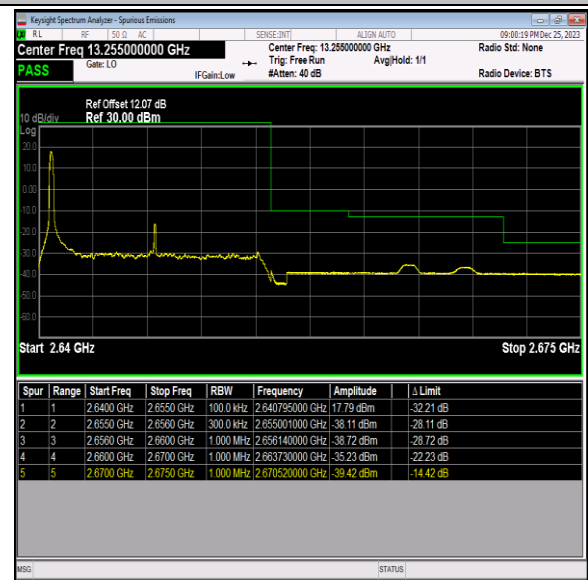
Band41_15MHz_16QAM_41165_1RB#0
