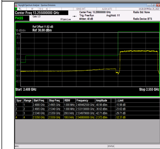
Band41_20MHz_64QAM_40140_100RB#0
