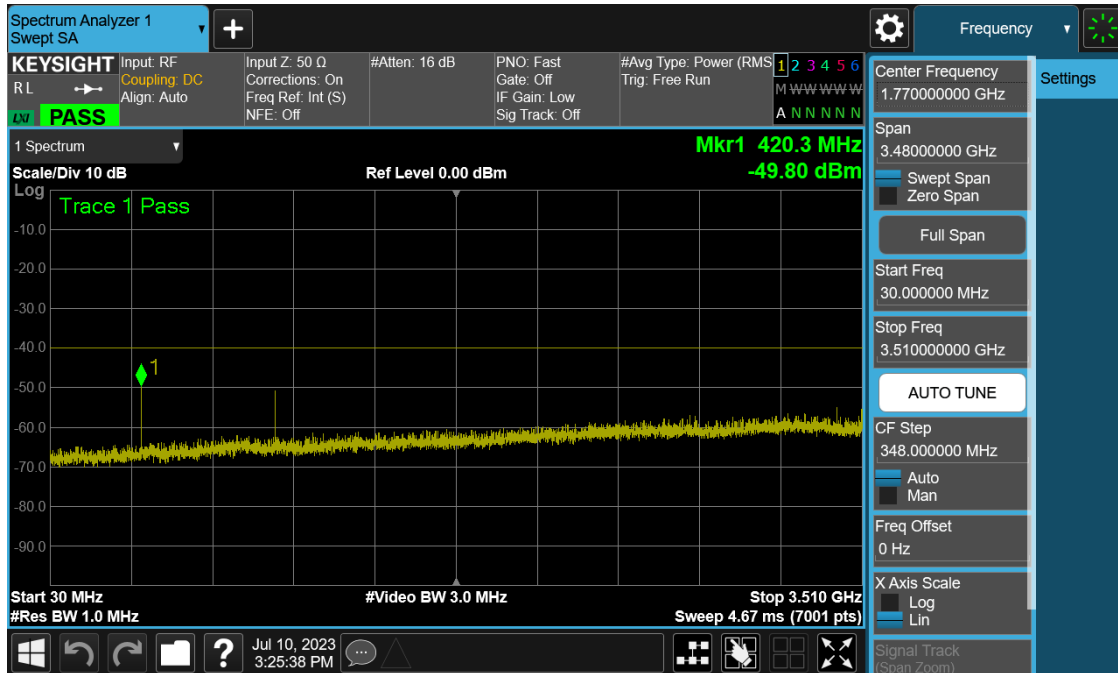
Plot 7-8. Conducted Spurious Plot (NR Band n48 - 10MHz QPSK – Low Channel)
