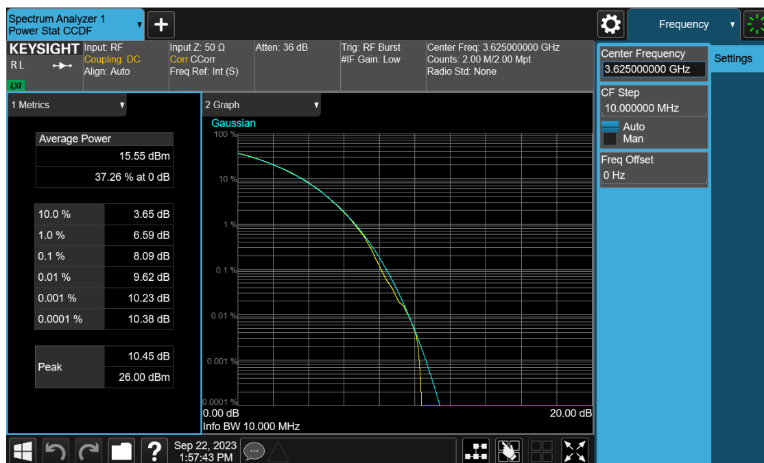
Plot 7-56. PAR Plot (NR Band n78 - 10MHz CP-OFDM 256-QAM- Full RB)
