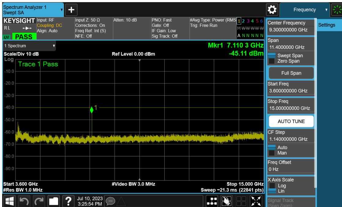
Plot 7-9. Conducted Spurious Plot (NR Band n48 - 10MHz QPSK – Low Channel)
