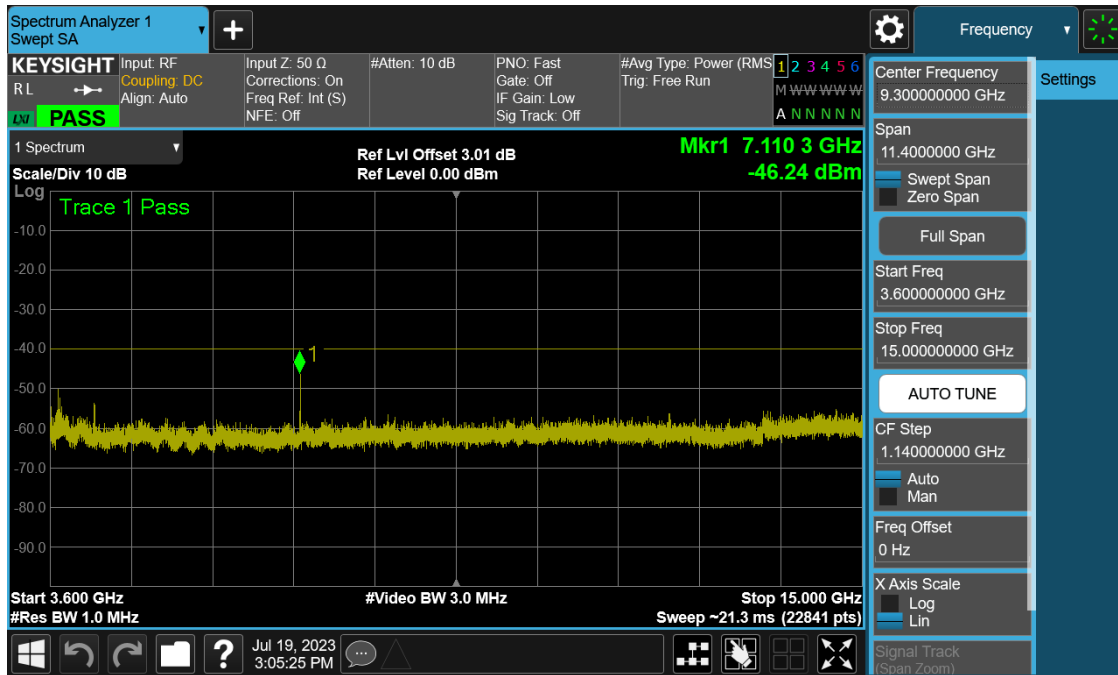
Plot 7-21. Conducted Spurious Plot (NR Band n48 - 10MHz QPSK – Low Channel)
