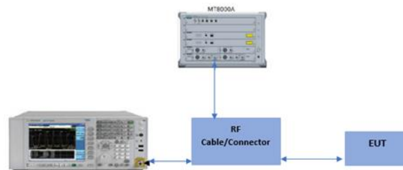
Figure 7-5. Test Instrument & Measurement Setup
