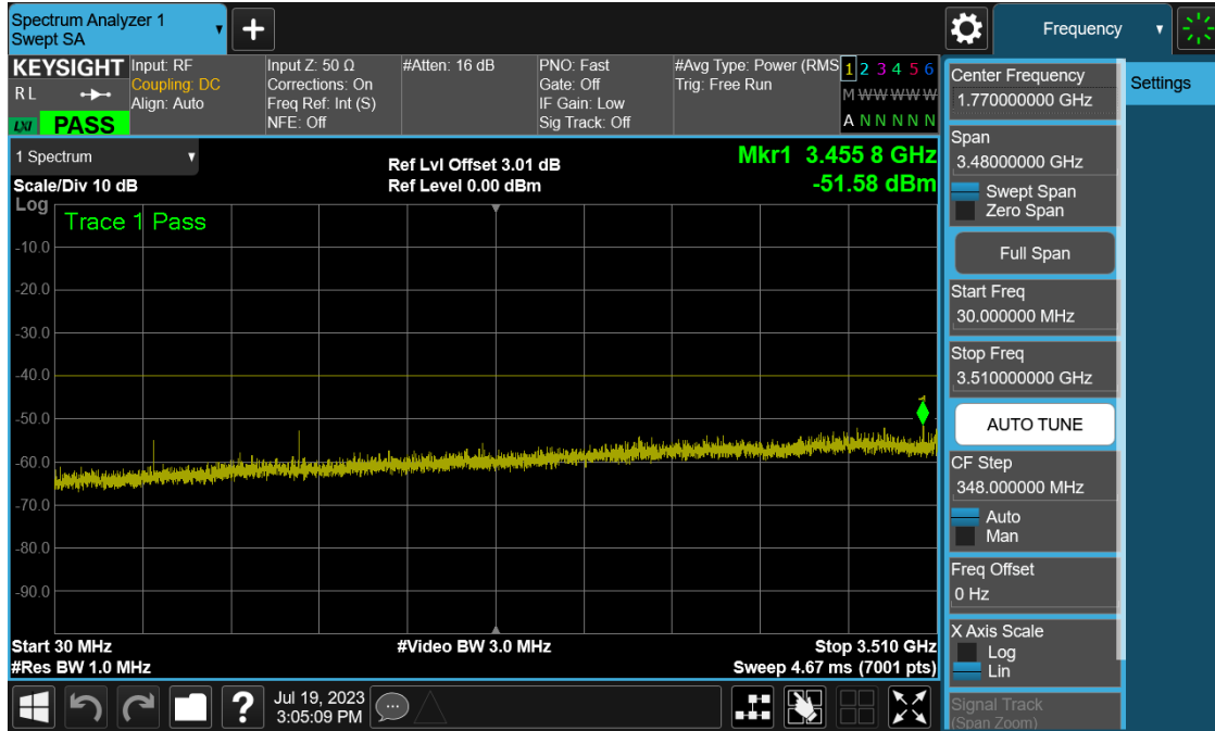
Plot 7-20. Conducted Spurious Plot (NR Band n48 - 10MHz QPSK – Low Channel)
