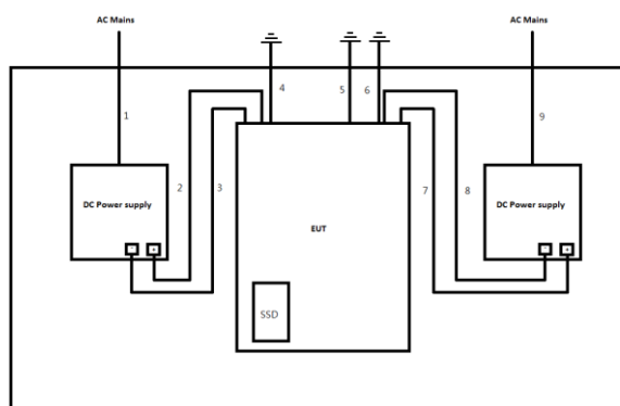
Test Setup Diagram - Radiated Test (Mode 6)
