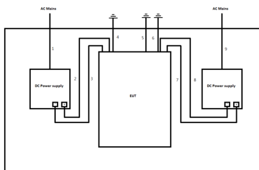
Test Setup Diagram - Radiated Test (Mode 12)
