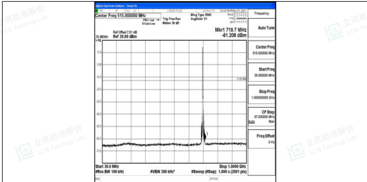
Band17_5MHz_16QAM_23755_1RB#0_30~1000_30~1000
