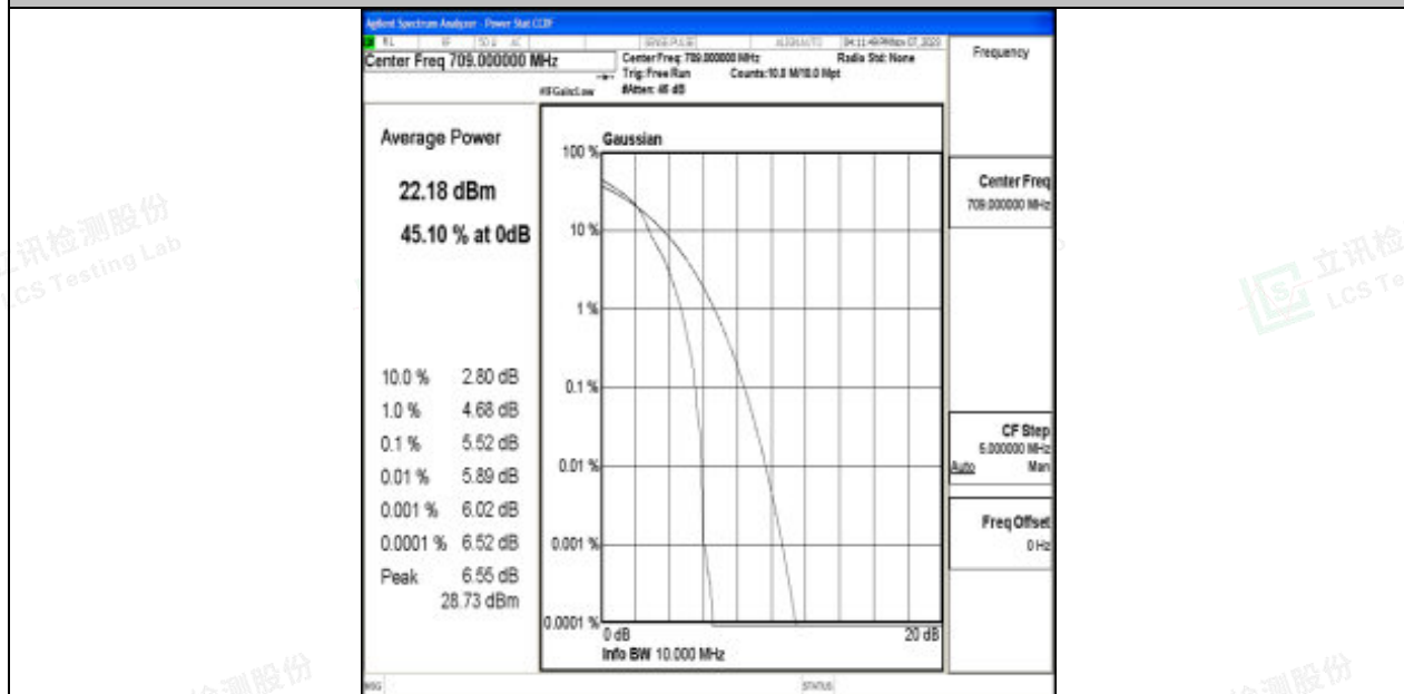
Band17-10MHz-16QAM-23780-1RB#0-PASS
