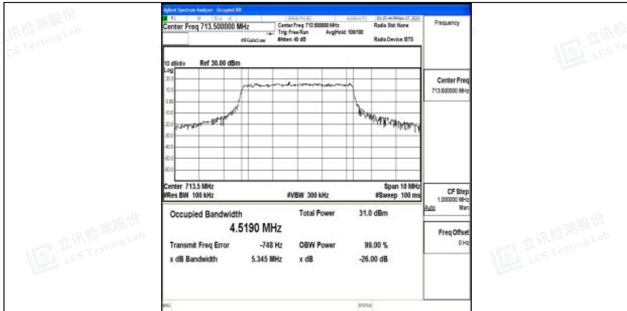
Band17-5MHz-QPSK-23825-25RB#0-PASS
