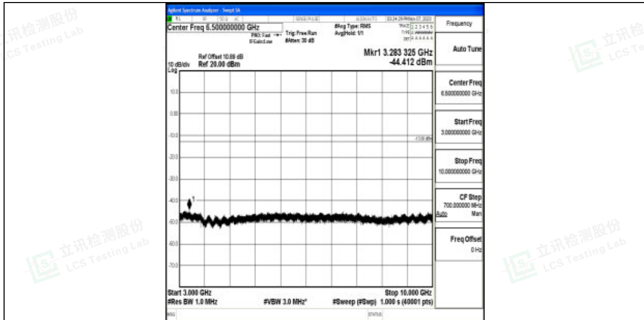
Band17_5MHz_64QAM_23790_1RB#0_3000~10000_3000~10000
