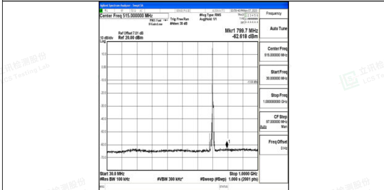
Band17_10MHz_16QAM_23800_1RB#0_30~1000_30~1000
