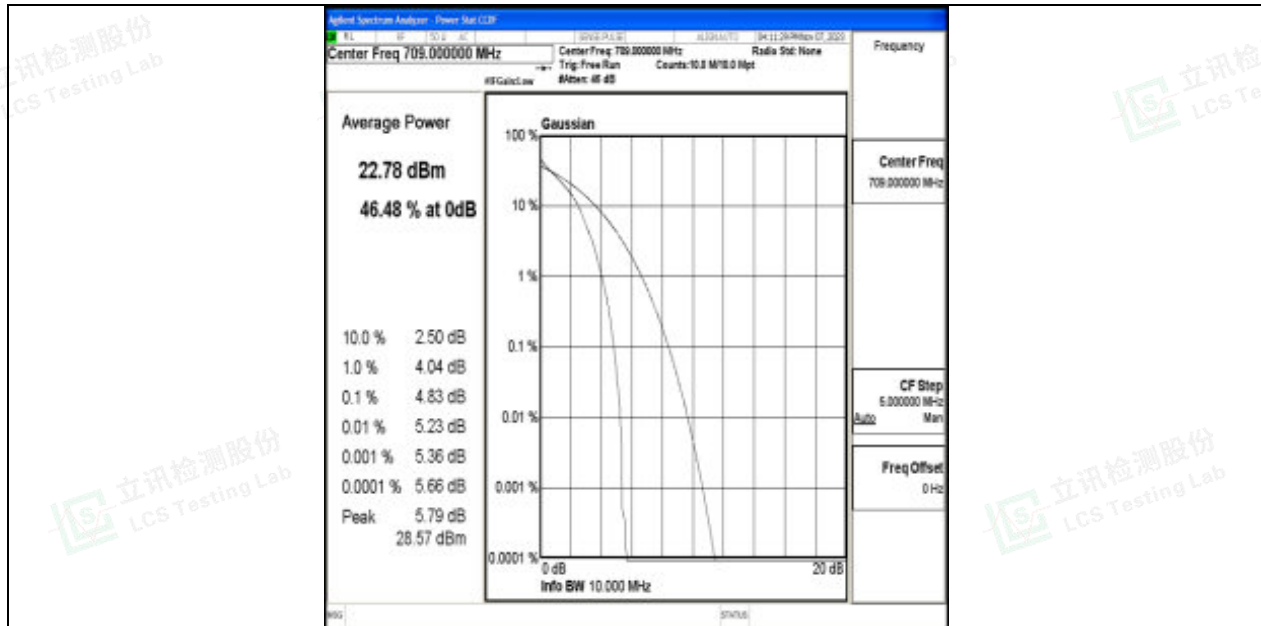
Band17-10MHz-QPSK-23780-1RB#0-PASS
