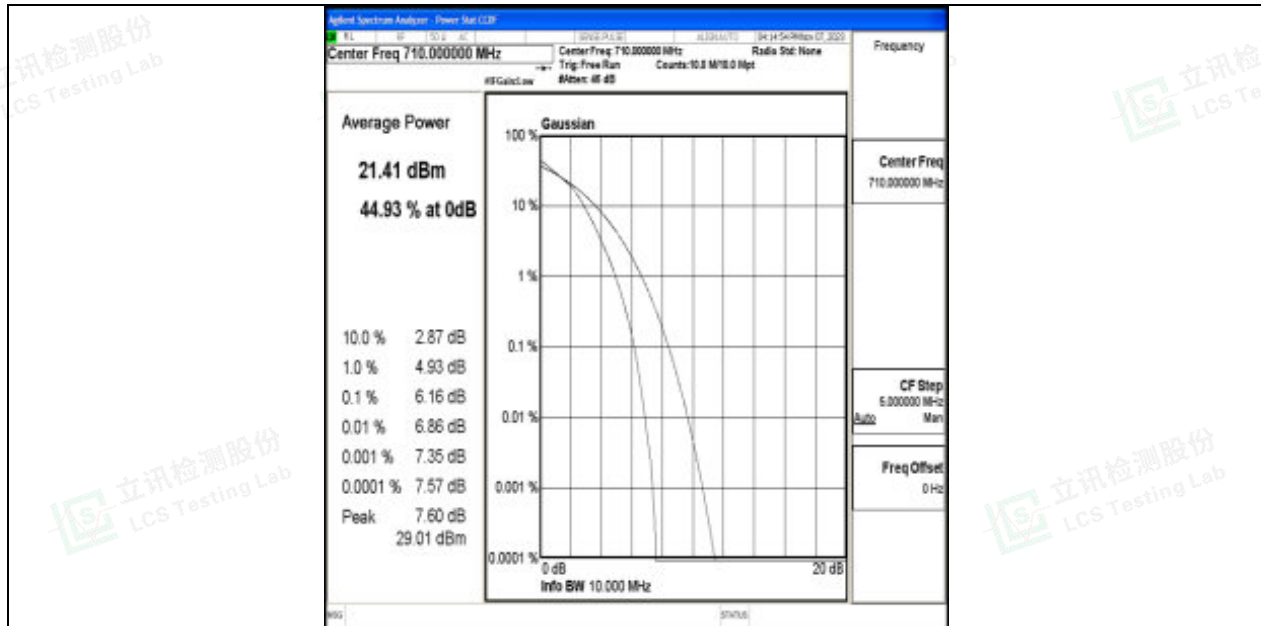
Band17-10MHz-16QAM-23790-50RB#0-PASS
