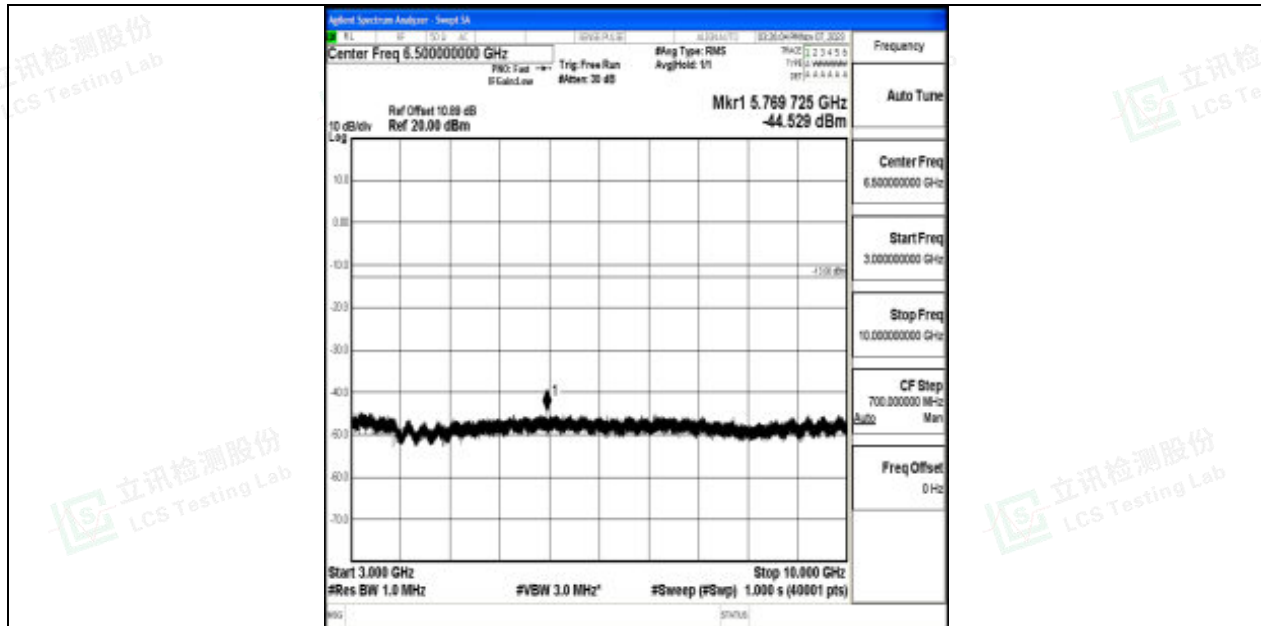
Band17_5MHz_16QAM_23825_1RB#0_3000~10000_3000~10000
