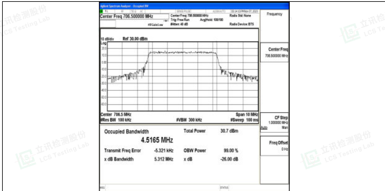
Band17-5MHz-64QAM-23755-25RB#0-PASS
