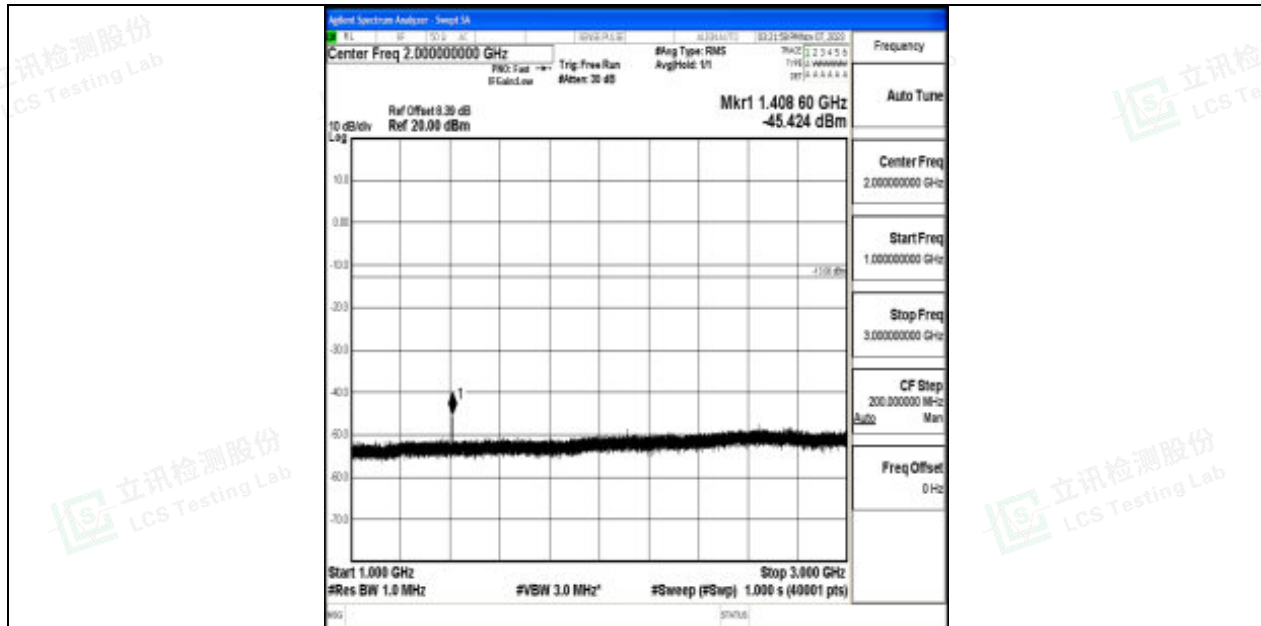
Band17_5MHz_64QAM_23755_1RB#0_1000~3000_1000~3000
