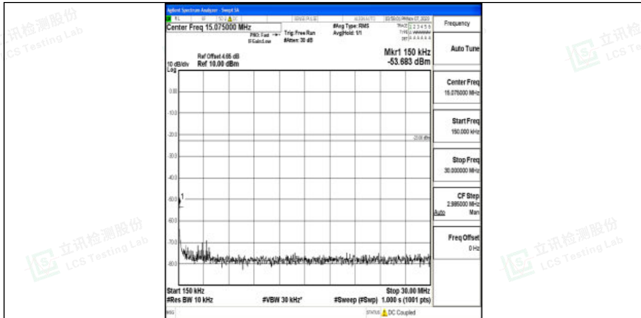
Band17_10MHz_64QAM_23790_1RB#0_0.15~30_0.15~30
