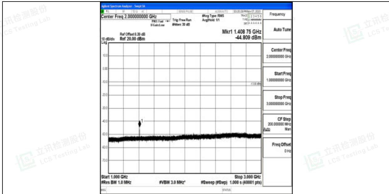
Band17_5MHz_QPSK_23755_1RB#0_1000~3000_1000~3000
