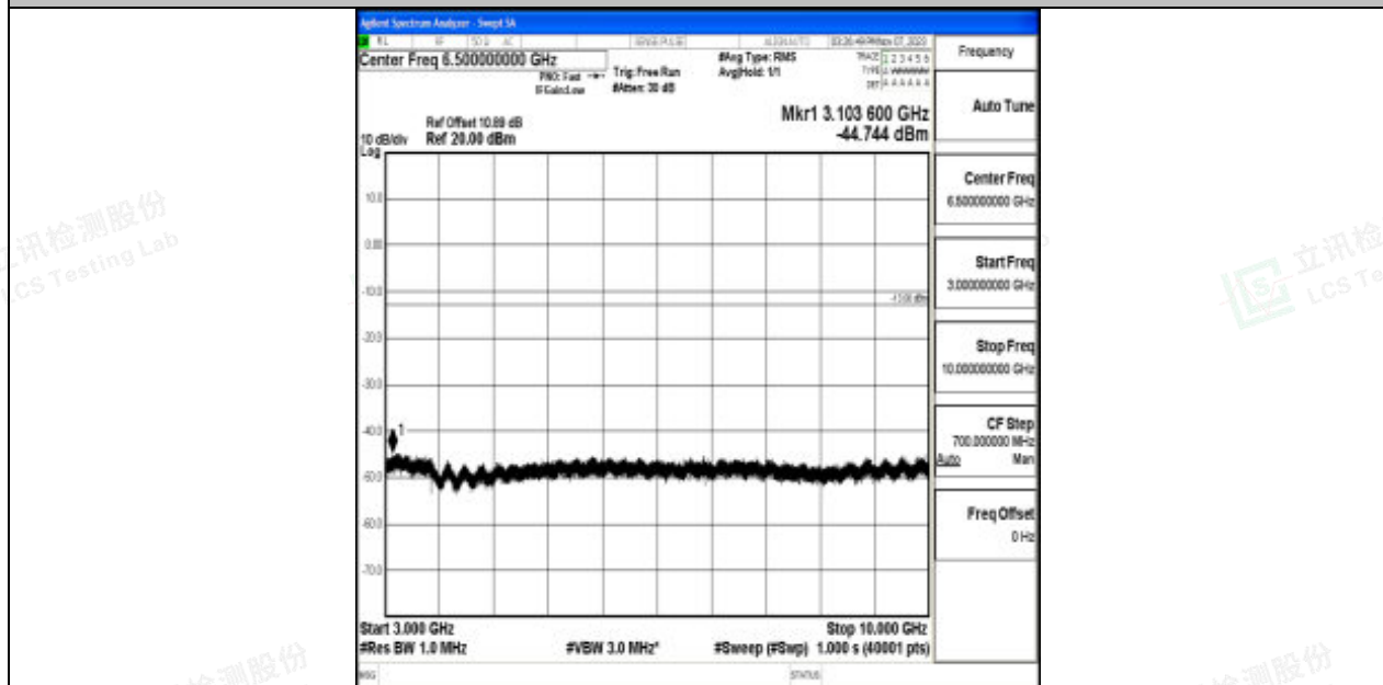
Band17_5MHz_64QAM_23825_1RB#0_3000~10000_3000~10000
