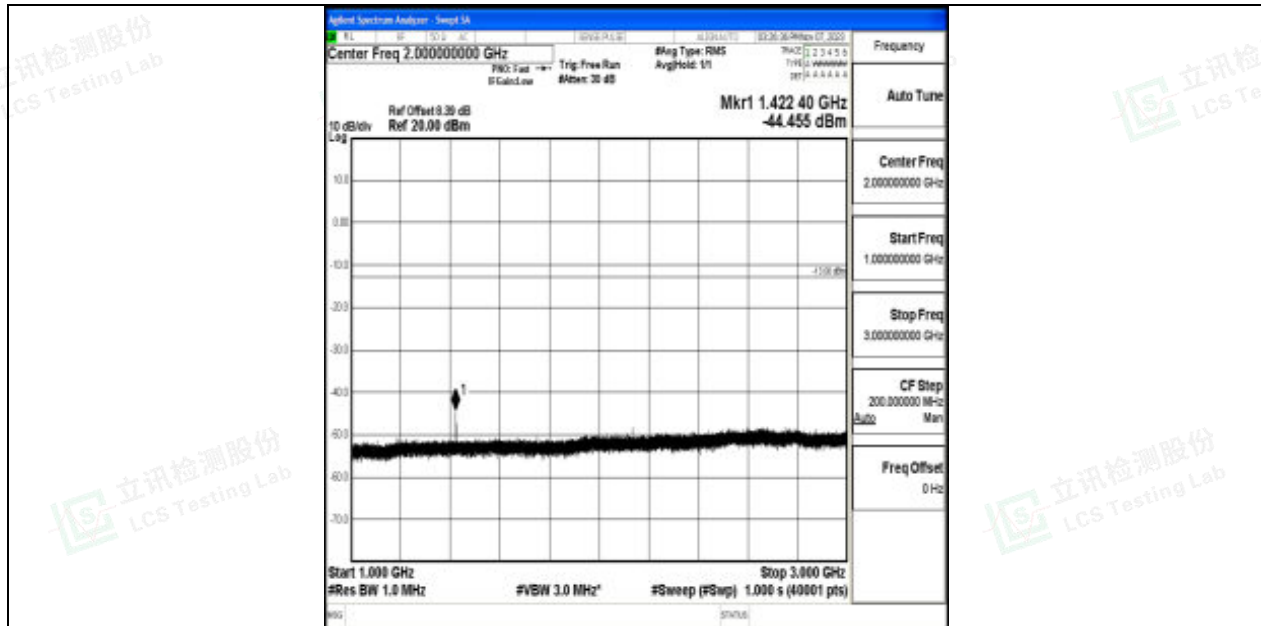
Band17_5MHz_64QAM_23825_1RB#0_1000~3000_1000~3000
