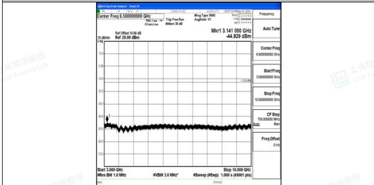
Band17_10MHz_QPSK_23790_1RB#0_3000~10000_3000~10000
