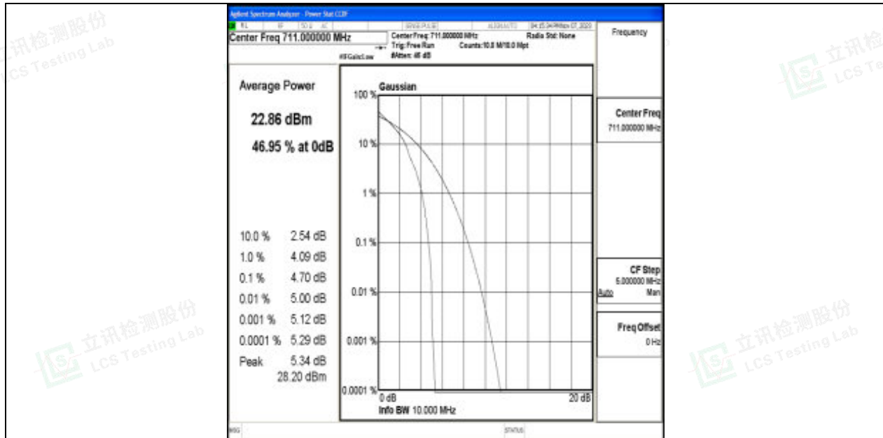
Band17-10MHz-QPSK-23800-1RB#0-PASS
