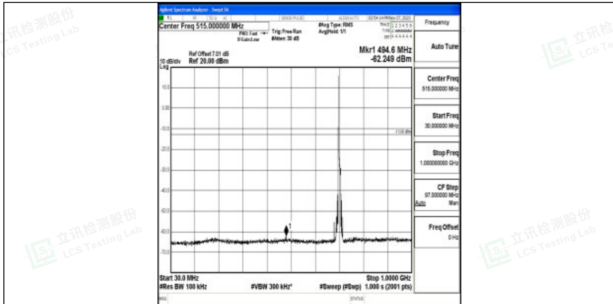
Band17_10MHz_QPSK_23780_1RB#0_30~1000_30~1000
