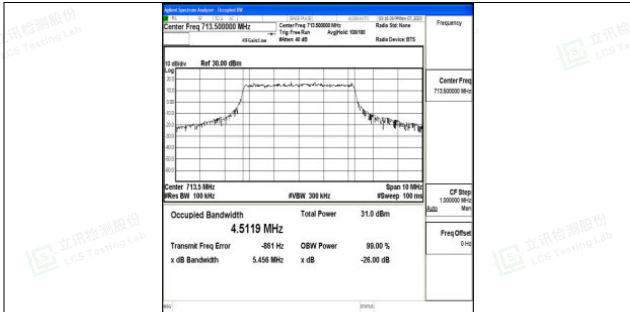
Band17-5MHz-64QAM-23825-25RB#0-PASS
