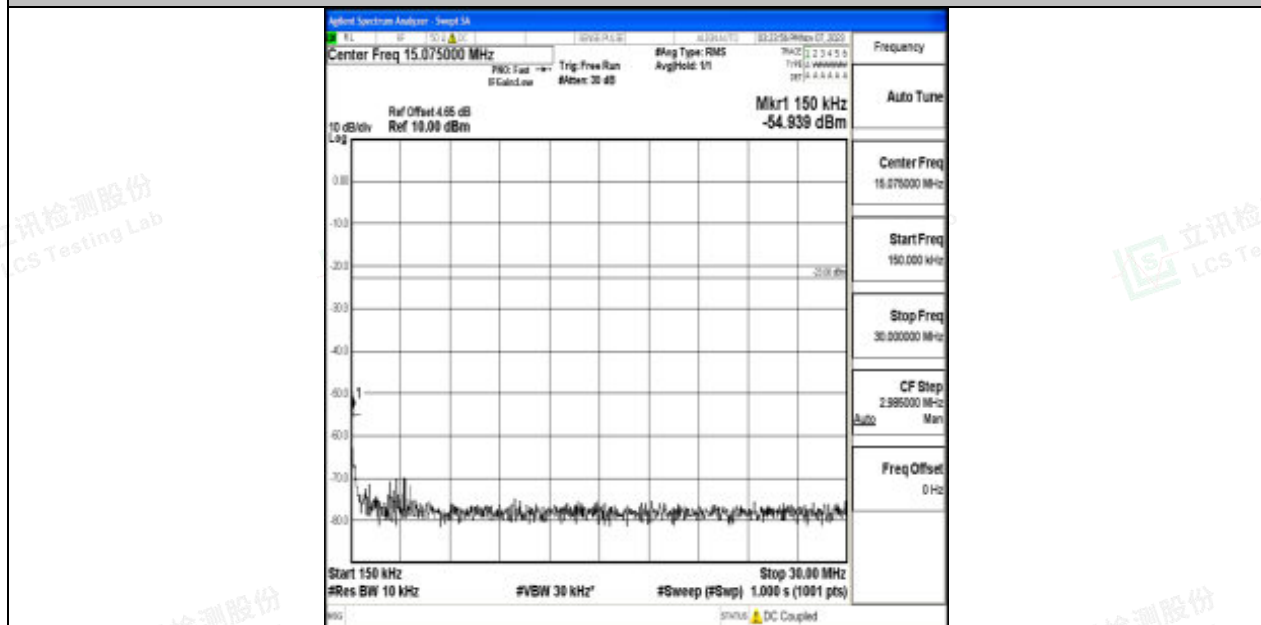
Band17_5MHz_64QAM_23790_1RB#0_0.15~30_0.15~30
