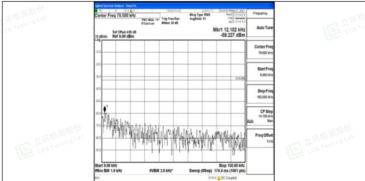
Band17_5MHz_64QAM_23790_1RB#0_0.009~0.15_0.009~0.15
