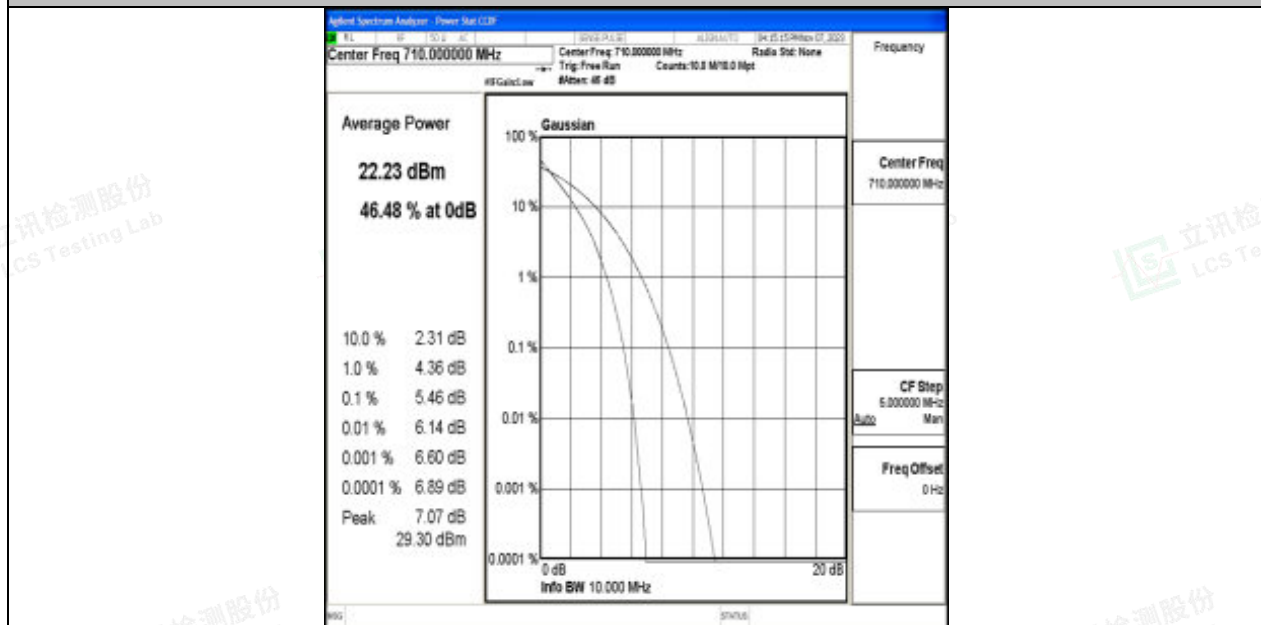
Band17-10MHz-64QAM-23790-50RB#0-PASS
