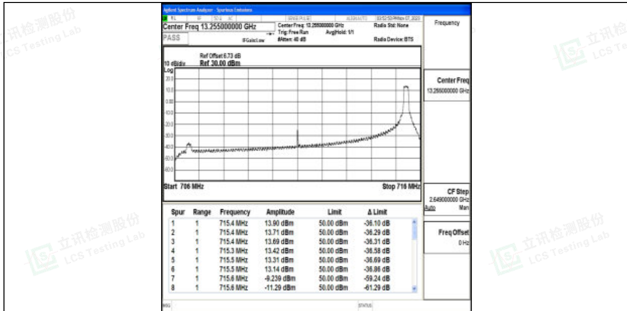
Band17_10MHz_QPSK_23800_1RB#49
