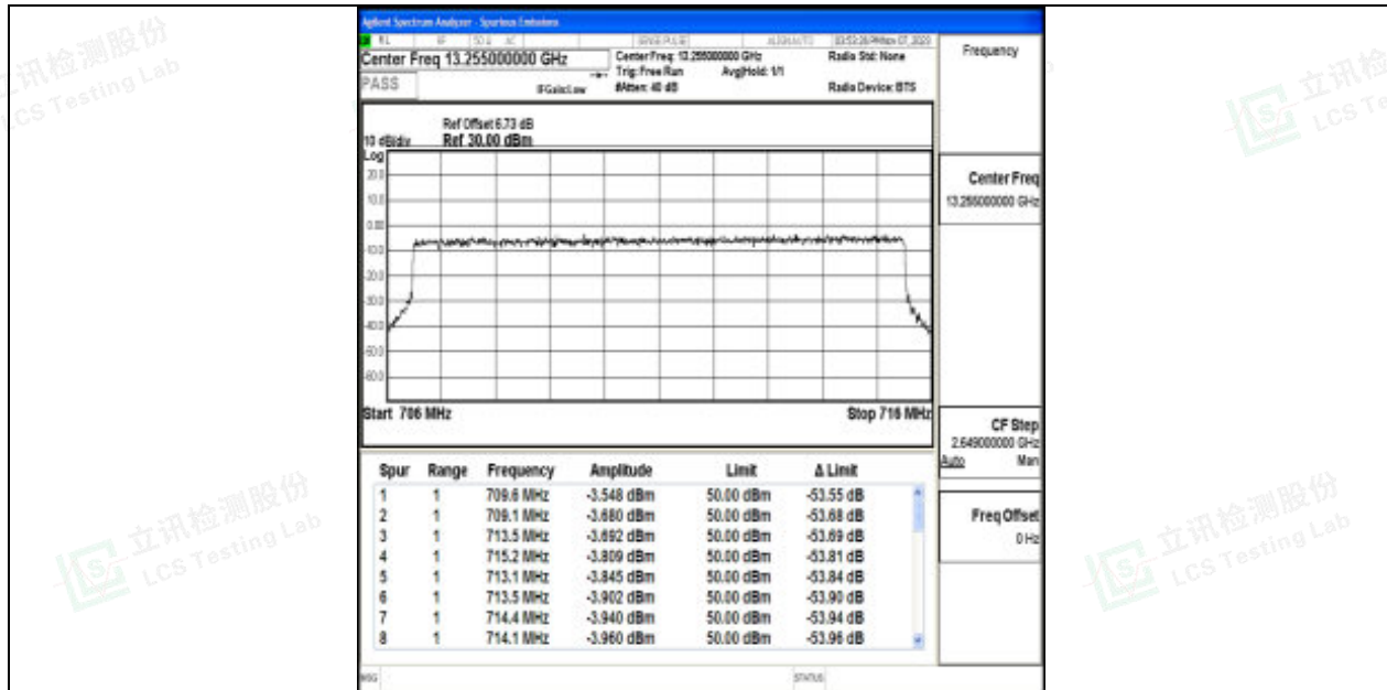
Band17_10MHz_16QAM_23800_50RB#0
