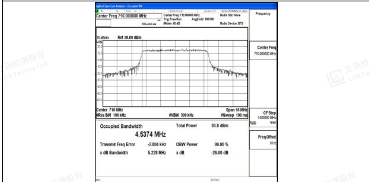
Band17-5MHz-QPSK-23790-25RB#0-PASS
