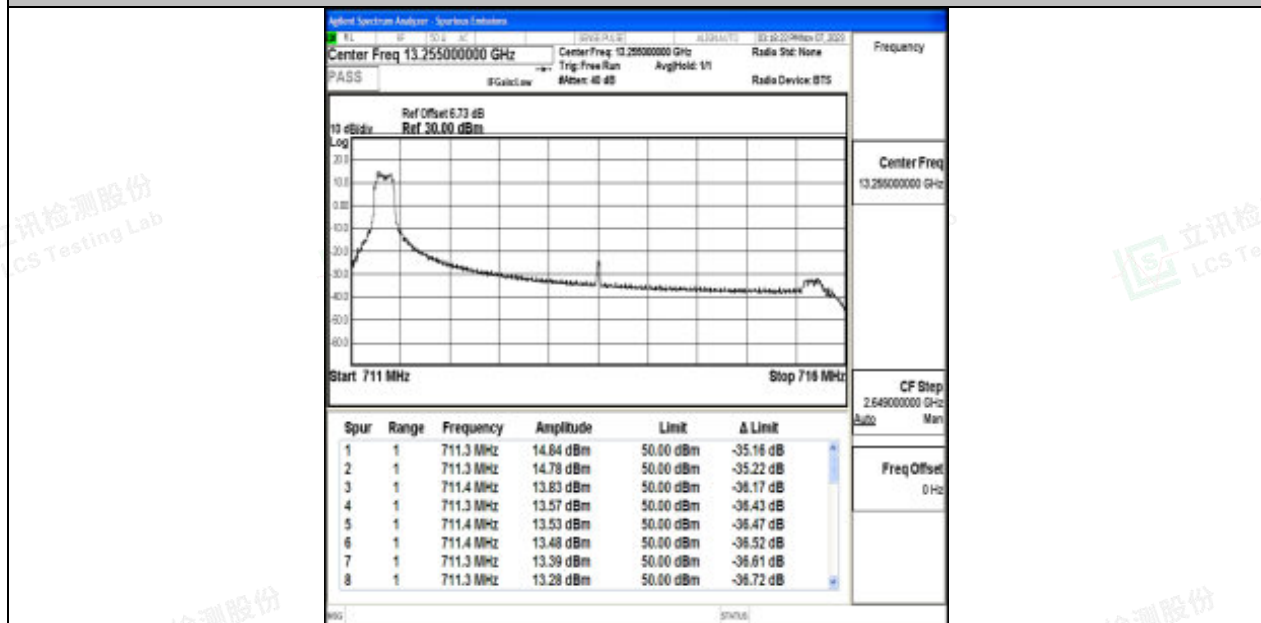
Band17_5MHz_QPSK_23825_1RB#0
