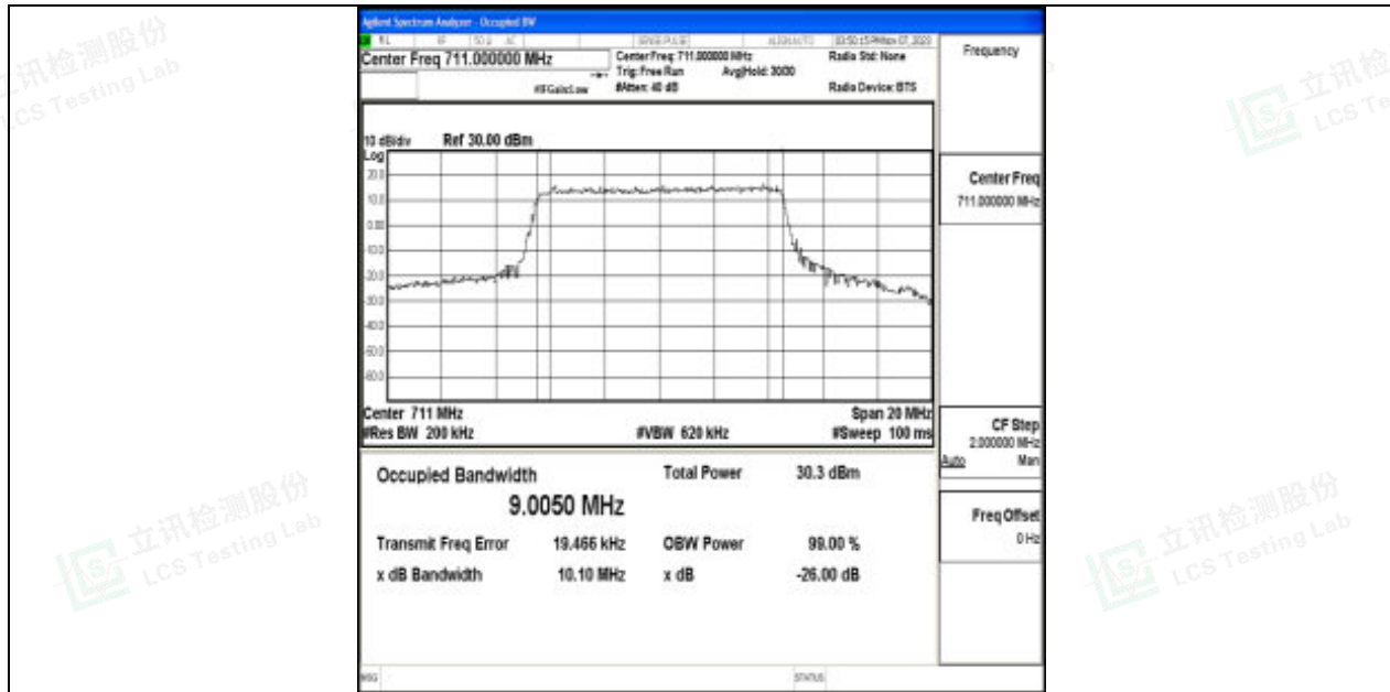
Band17-10MHz-16QAM-23800-50RB#0-PASS
