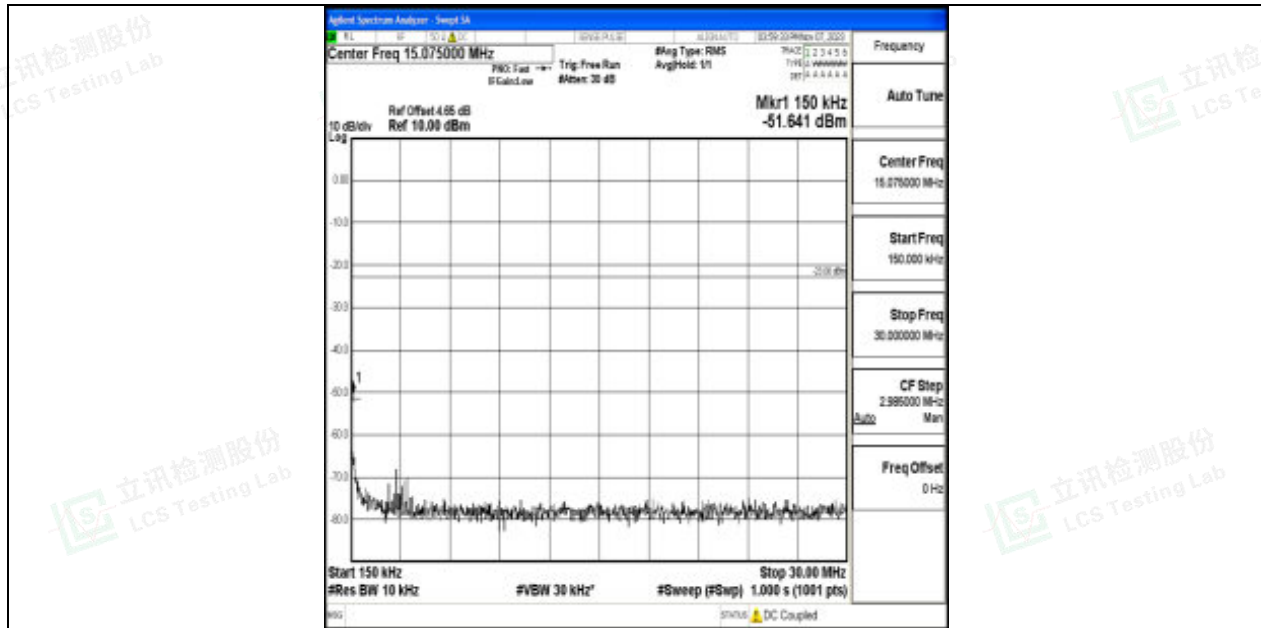
Band17_10MHz_16QAM_23800_1RB#0_0.15~30_0.15~30
