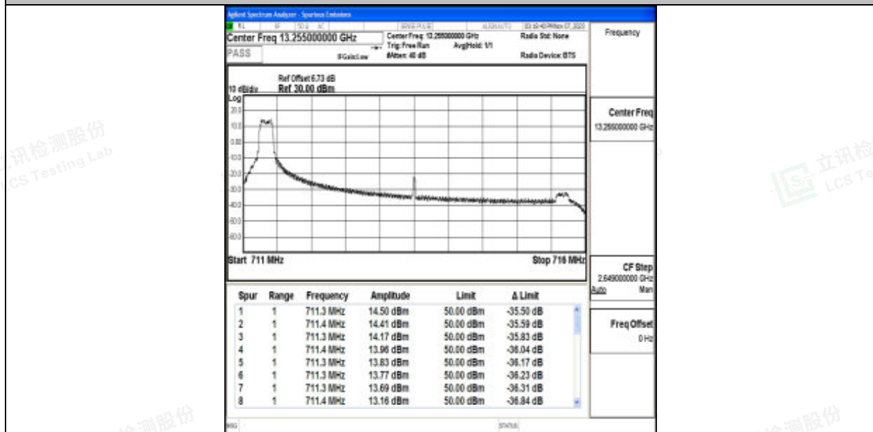
Band17_5MHz_64QAM_23825_1RB#0
