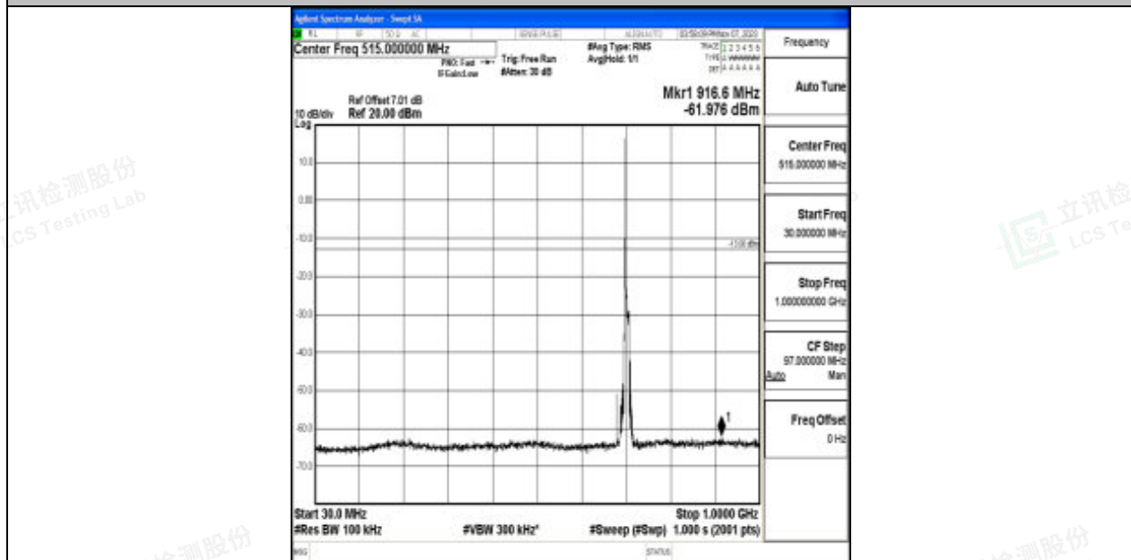
Band17_10MHz_64QAM_23790_1RB#0_30~1000_30~1000
