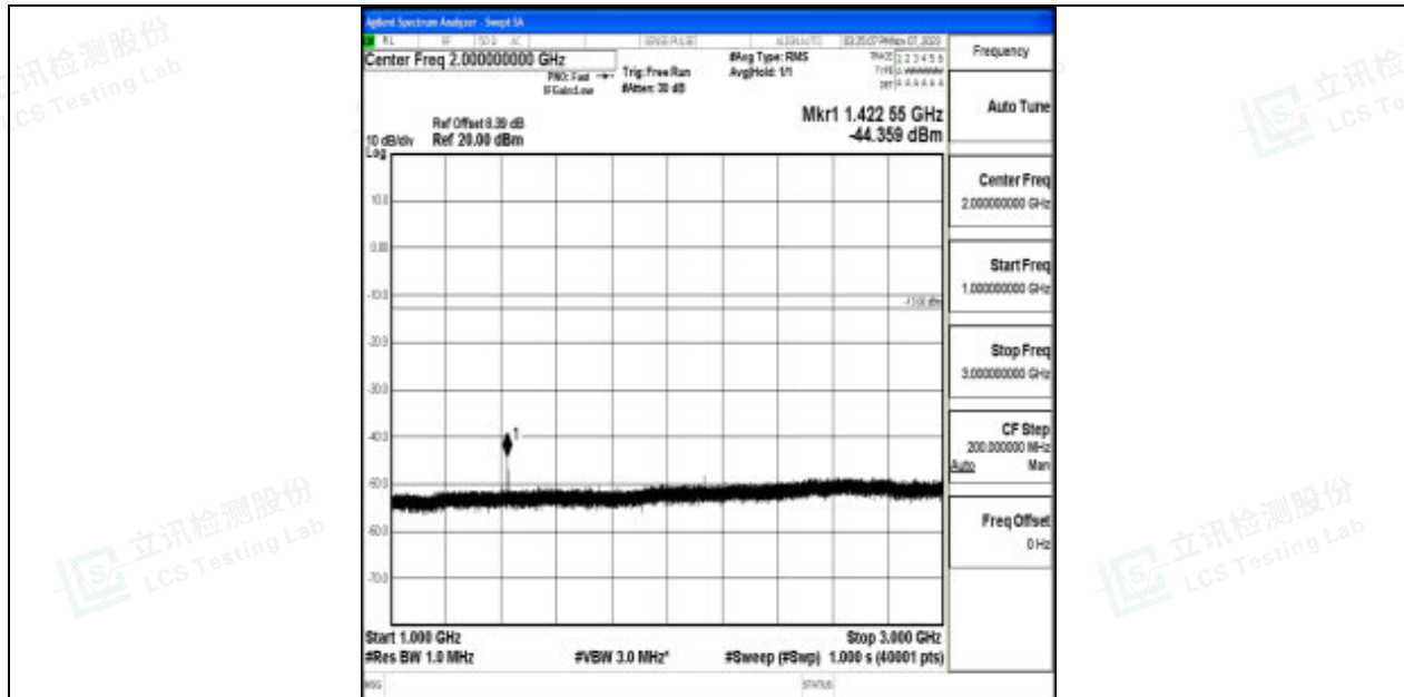
Band17_5MHz_QPSK_23825_1RB#0_1000~3000_1000~3000
