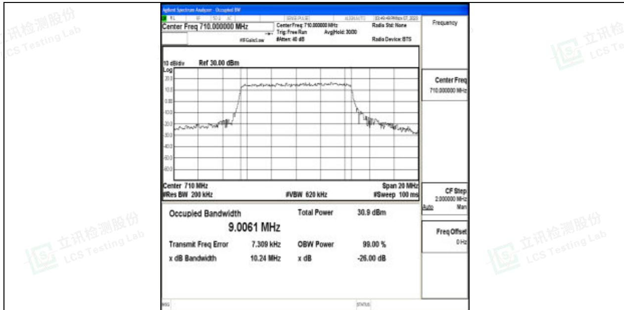
Band17-10MHz-64QAM-23790-50RB#0-PASS
