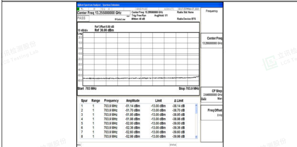
Band17_5MHz_QPSK_23755_1RB#24
