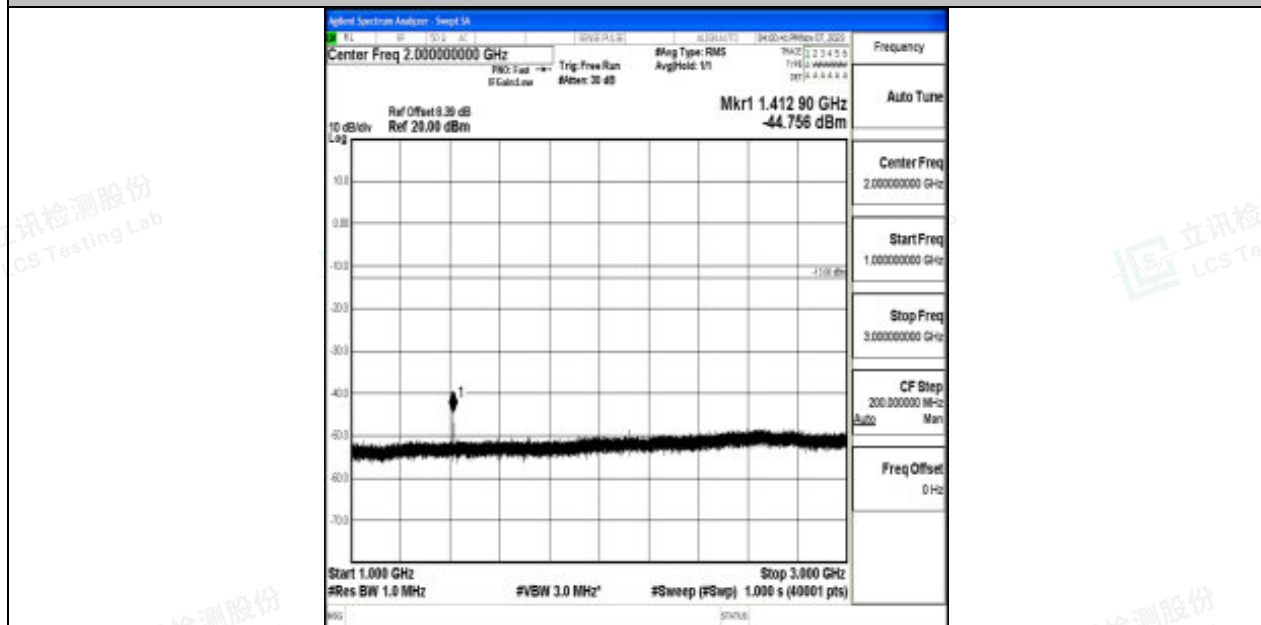
Band17_10MHz_64QAM_23800_1RB#0_1000~3000_1000~3000
