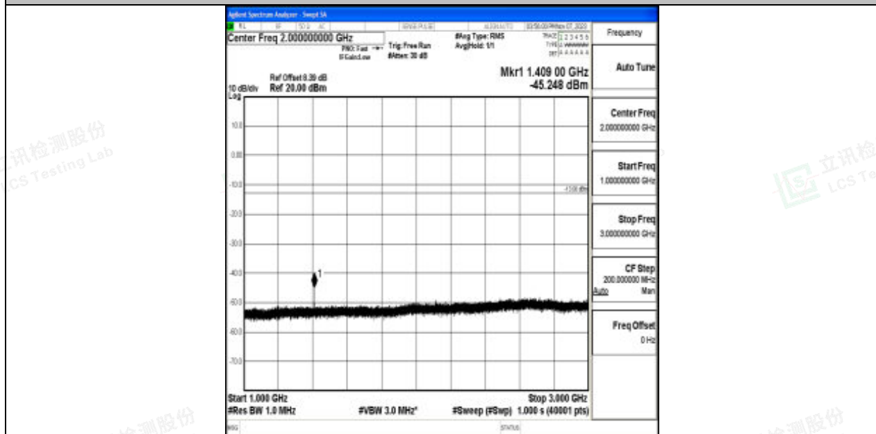
Band17_10MHz_64QAM_23780_1RB#0_1000~3000_1000~3000
