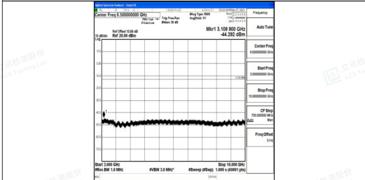
Band17_5MHz_QPSK_23755_1RB#0_3000~10000_3000~10000
