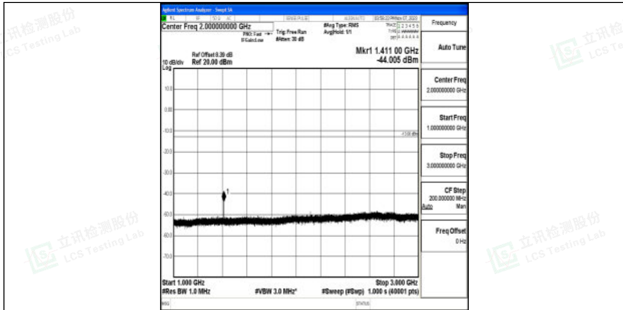
Band17_10MHz_64QAM_23790_1RB#0_1000~3000_1000~3000
