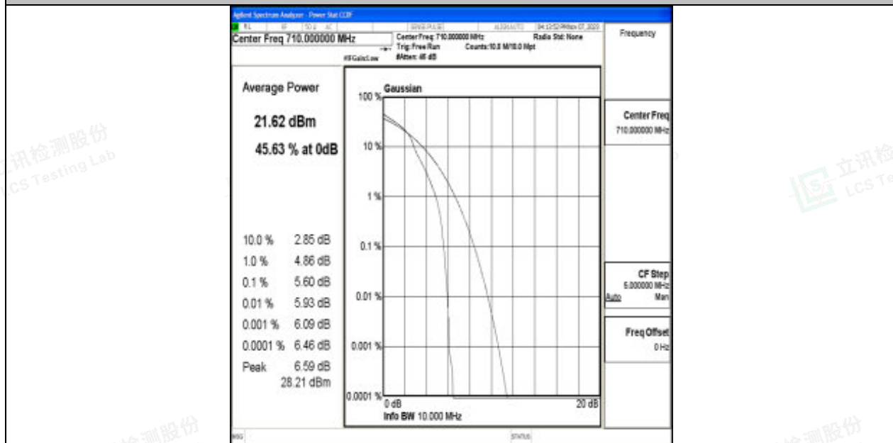
Band17-10MHz-16QAM-23790-1RB#0-PASS
