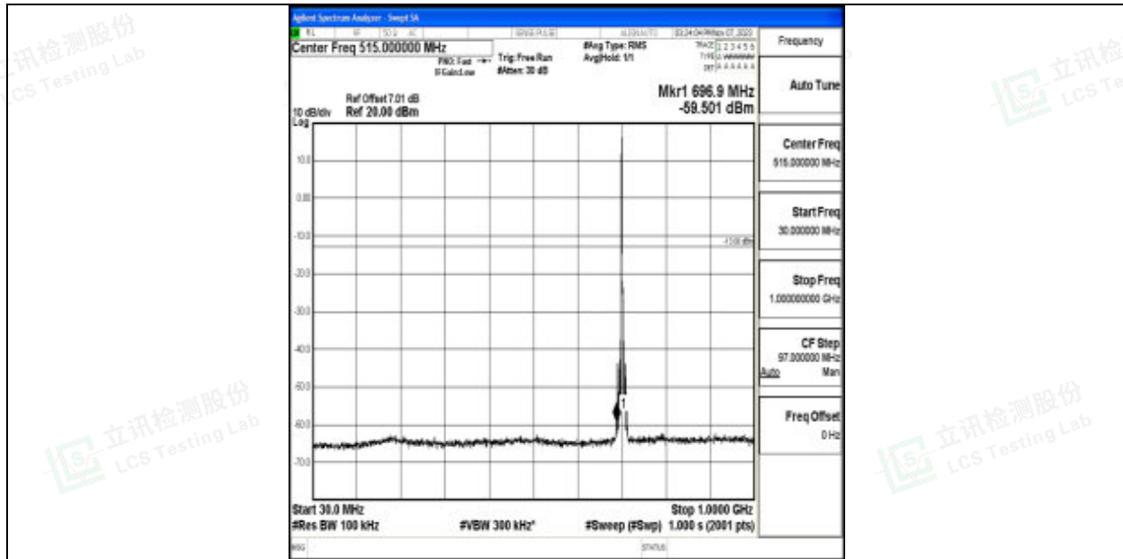
Band17_5MHz_64QAM_23790_1RB#0_30~1000_30~1000
