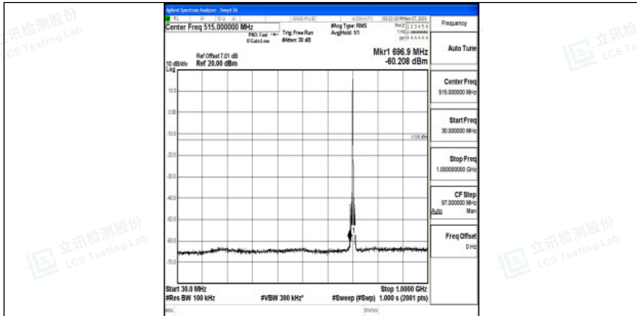
Band17_5MHz_QPSK_23790_1RB#0_30~1000_30~1000
