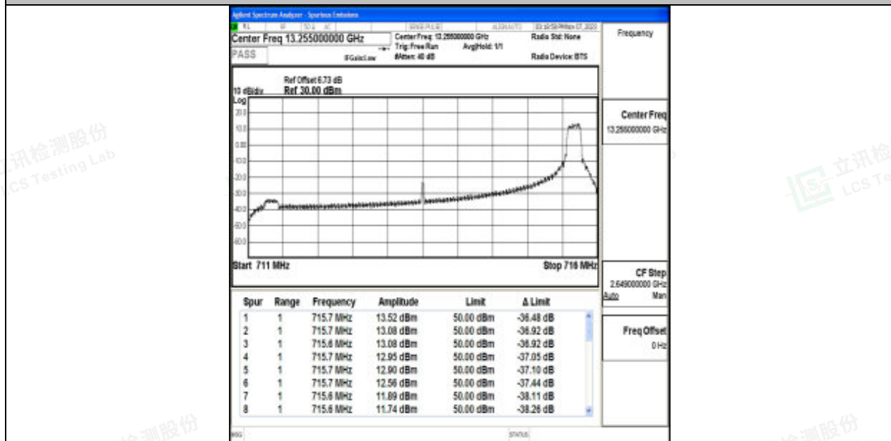
Band17_5MHz_16QAM_23825_1RB#24
