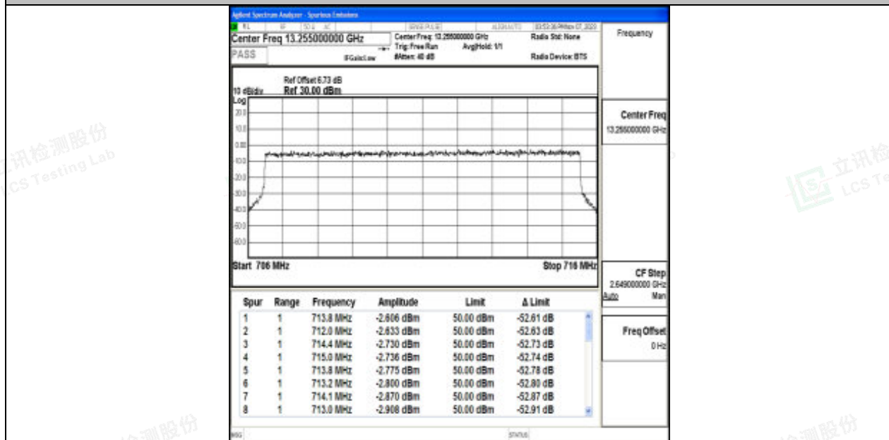
Band17_10MHz_64QAM_23800_50RB#0
