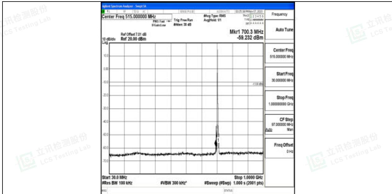
Band17_5MHz_16QAM_23825_1RB#0_30~1000_30~1000
