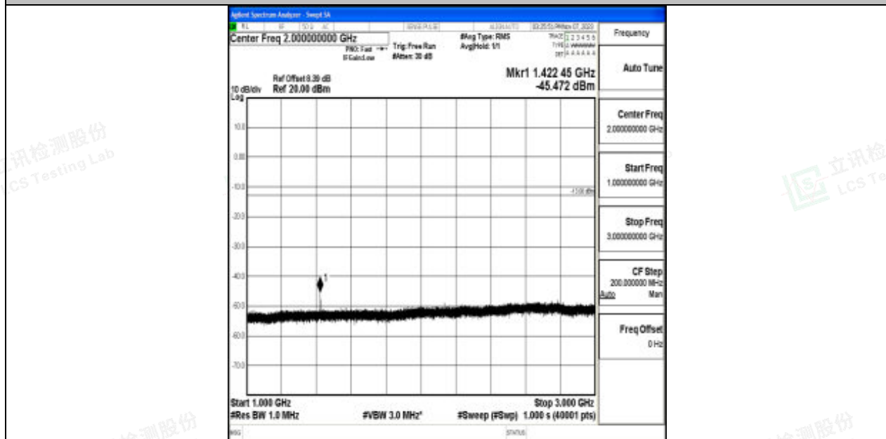
Band17_5MHz_16QAM_23825_1RB#0_1000~3000_1000~3000
