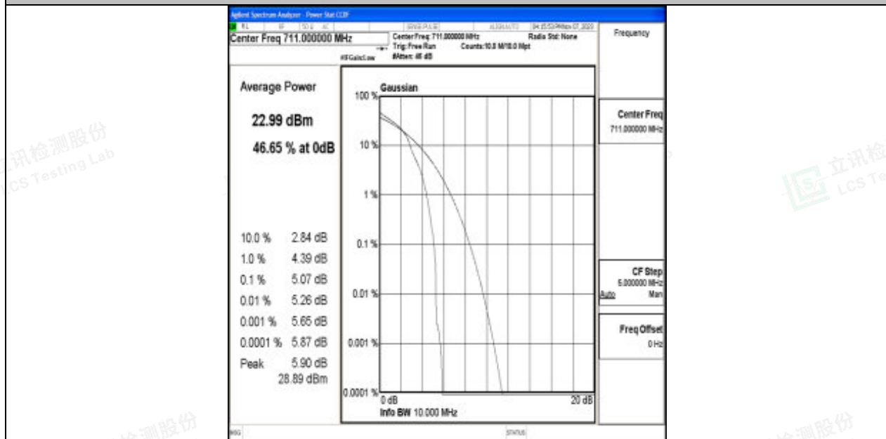
Band17-10MHz-16QAM-23800-1RB#0-PASS
