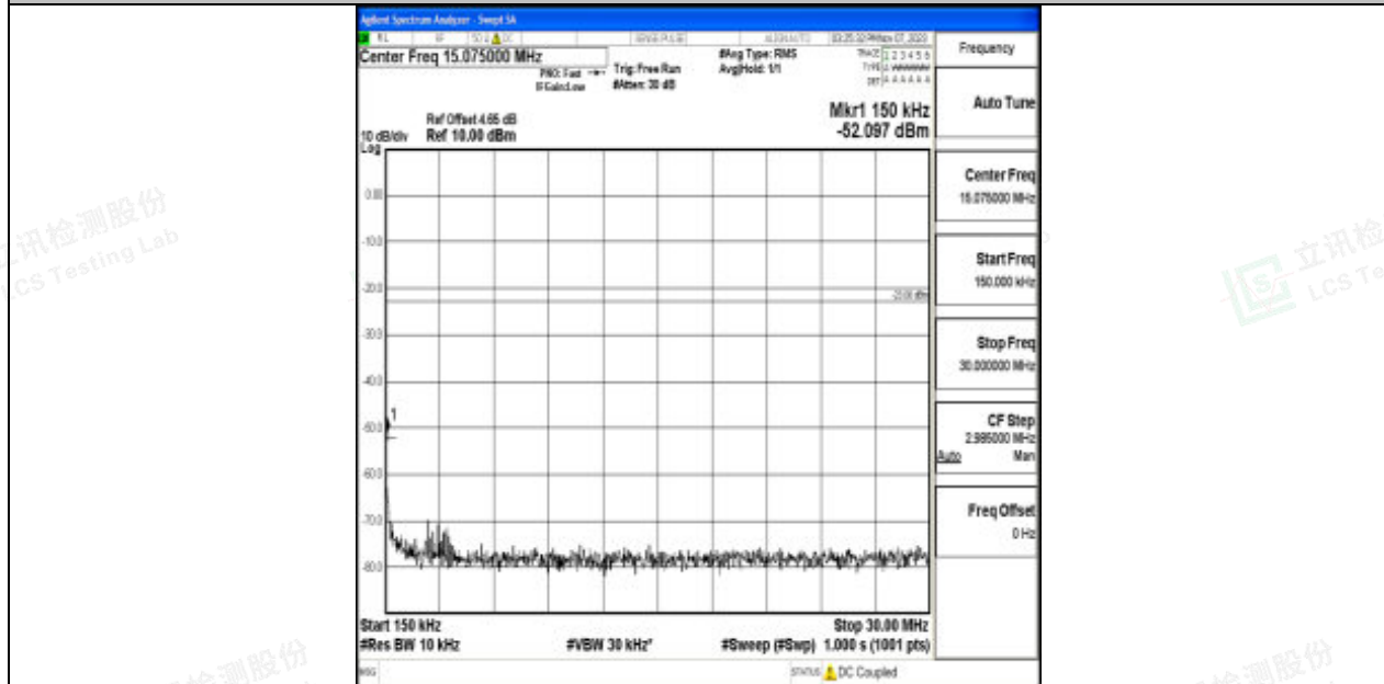
Band17_5MHz_16QAM_23825_1RB#0_0.15~30_0.15~30
