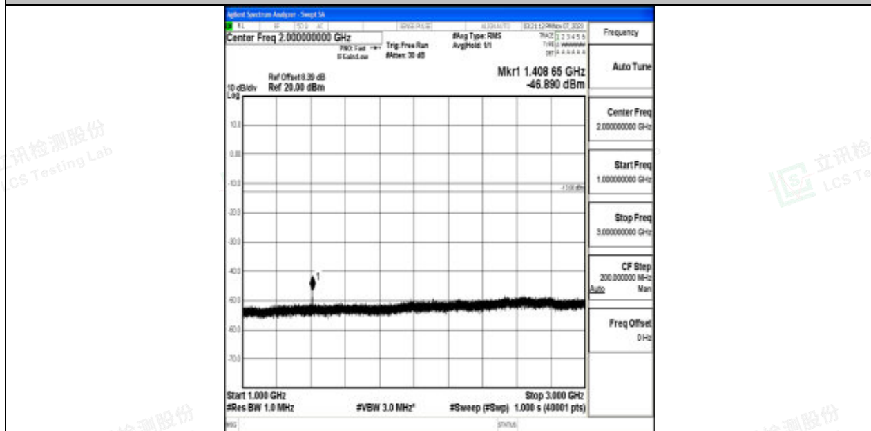
Band17_5MHz_16QAM_23755_1RB#0_1000~3000_1000~3000
