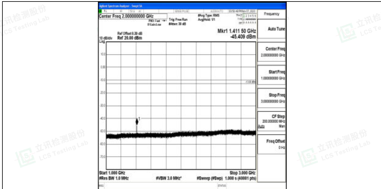
Band17_10MHz_QPSK_23790_1RB#0_1000~3000_1000~3000
