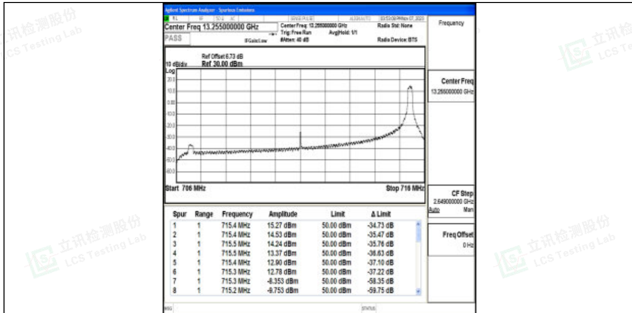
Band17_10MHz_64QAM_23800_1RB#49
