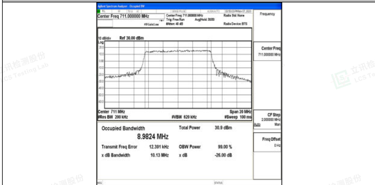
Band17-10MHz-QPSK-23800-50RB#0-PASS
