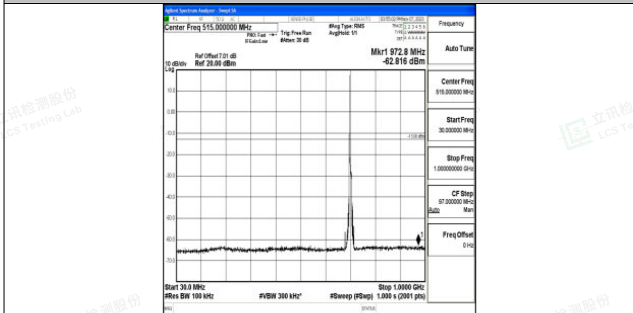
Band17_10MHz_16QAM_23780_1RB#0_30~1000_30~1000
