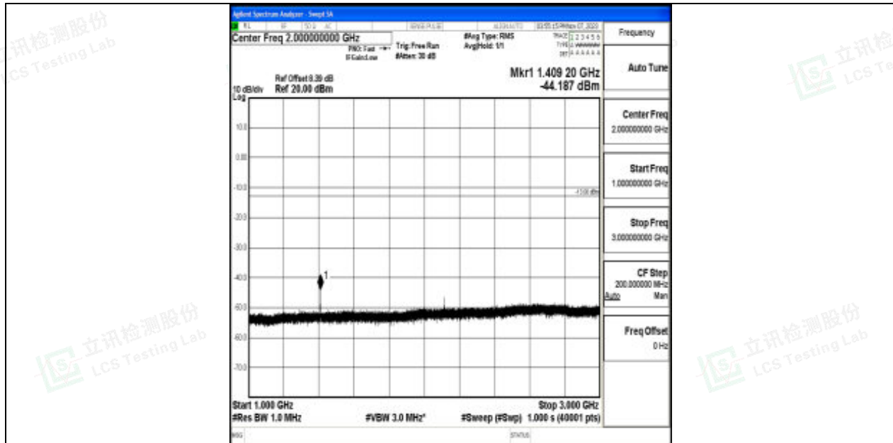
Band17_10MHz_16QAM_23780_1RB#0_1000~3000_1000~3000
