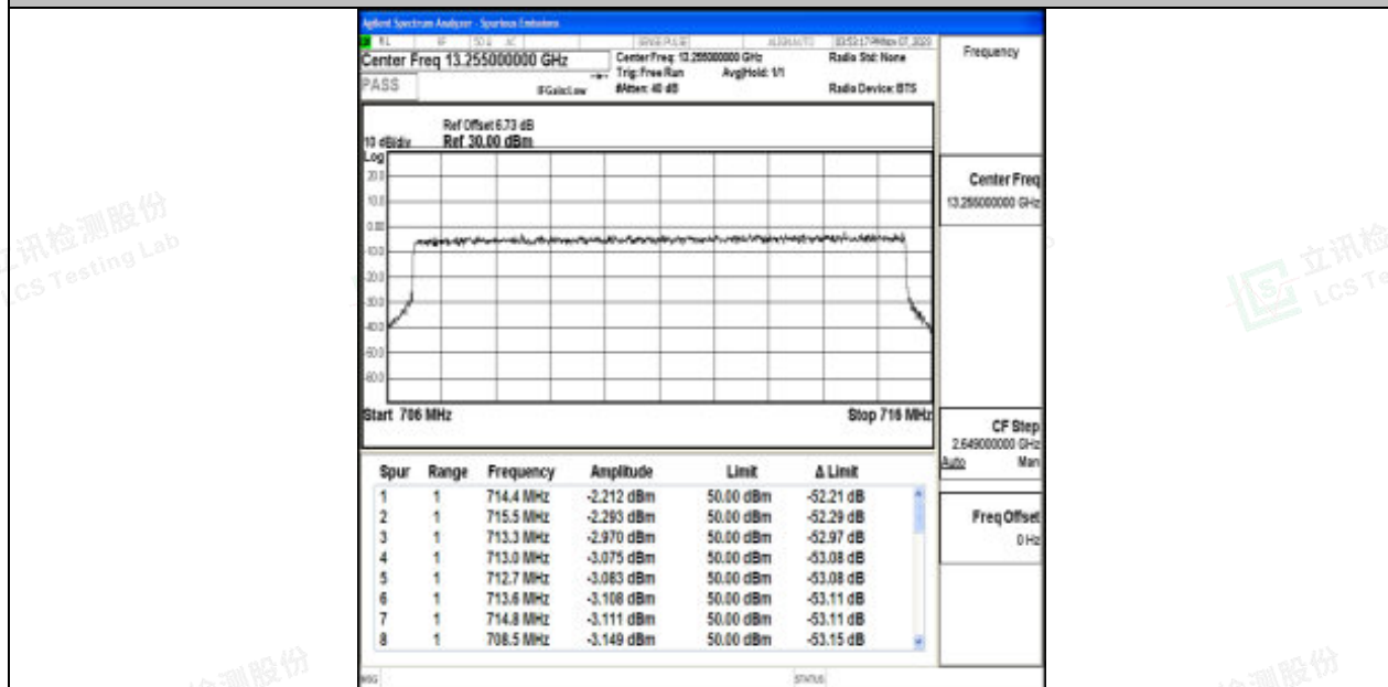
Band17_10MHz_QPSK_23800_50RB#0
