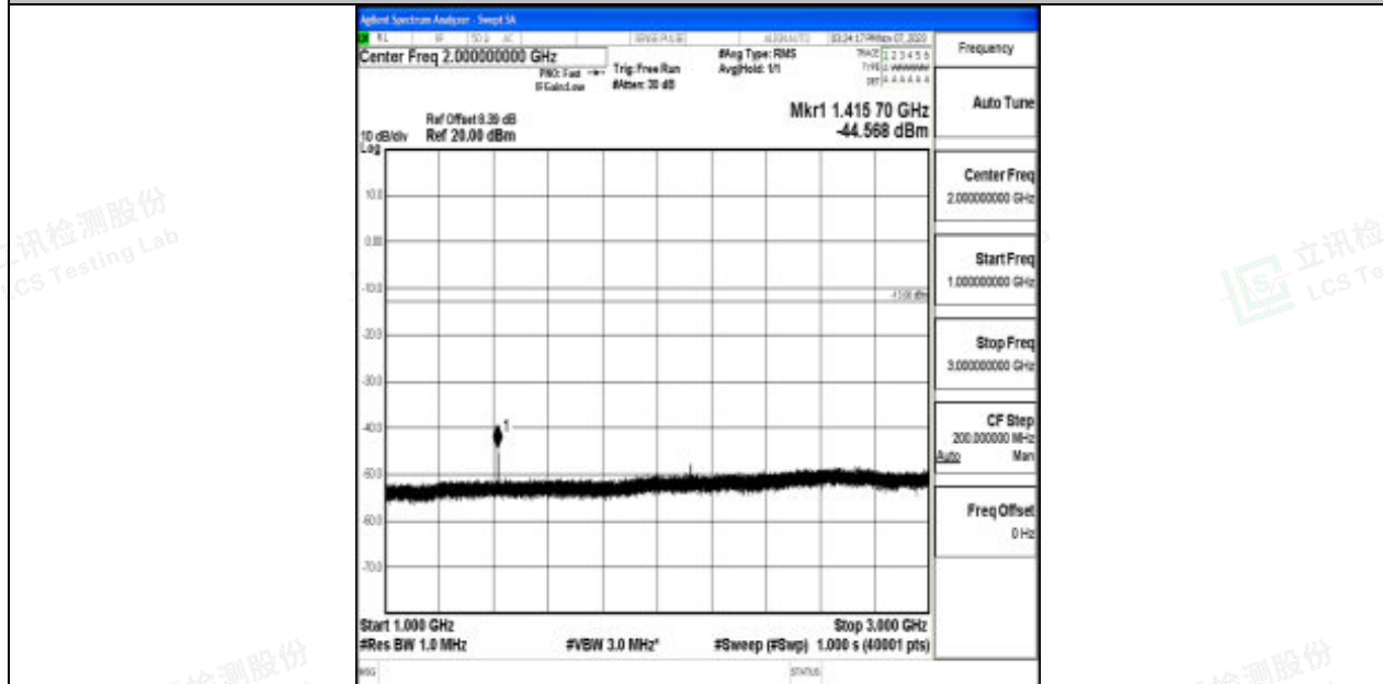
Band17_5MHz_64QAM_23790_1RB#0_1000~3000_1000~3000
