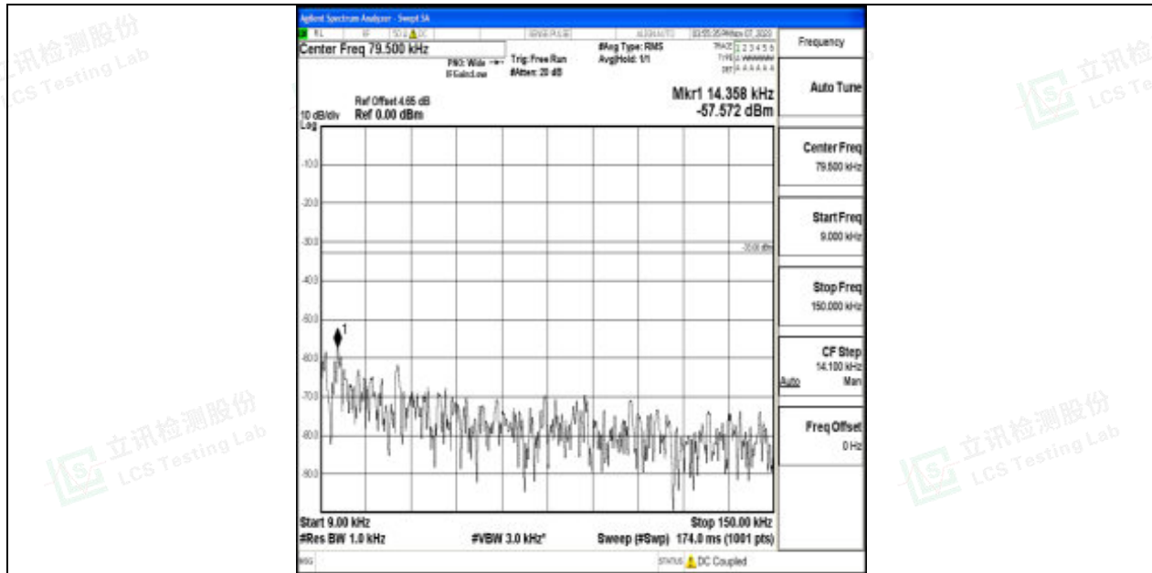
Band17_10MHz_64QAM_23780_1RB#0_0.009~0.15_0.009~0.15
