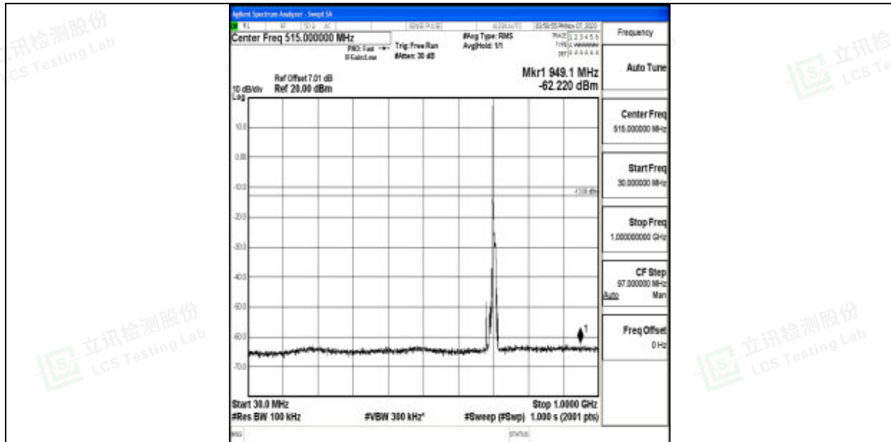
Band17_10MHz_QPSK_23800_1RB#0_30~1000_30~1000
