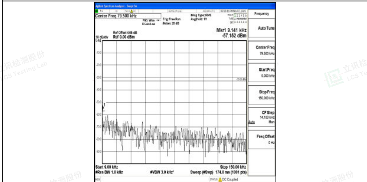
Band17_5MHz_64QAM_23825_1RB#0_0.009~0.15_0.009~0.15
