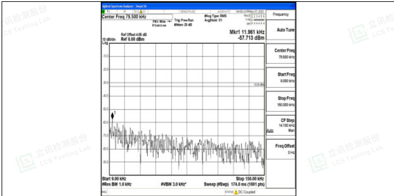
Band17_10MHz_64QAM_23800_1RB#0_0.009~0.15_0.009~0.15
