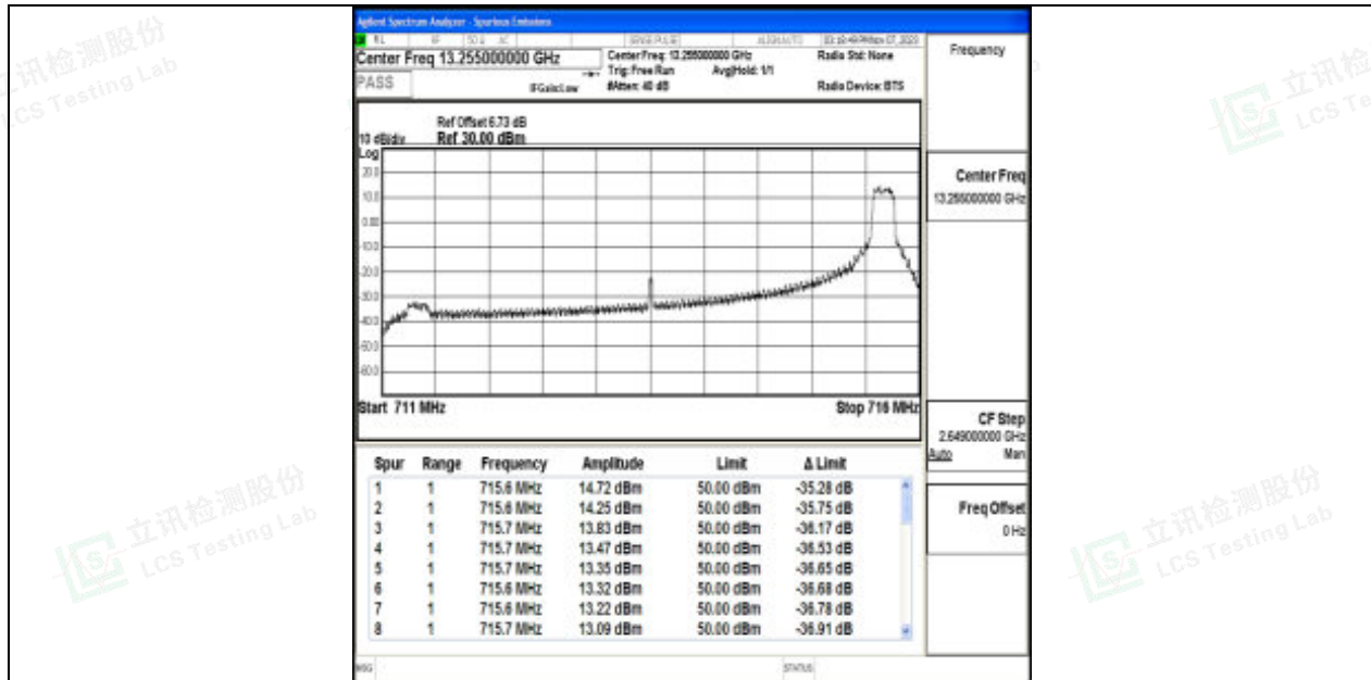
Band17_5MHz_QPSK_23825_1RB#24
