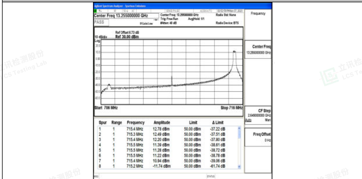
Band17_10MHz_16QAM_23800_1RB#49
