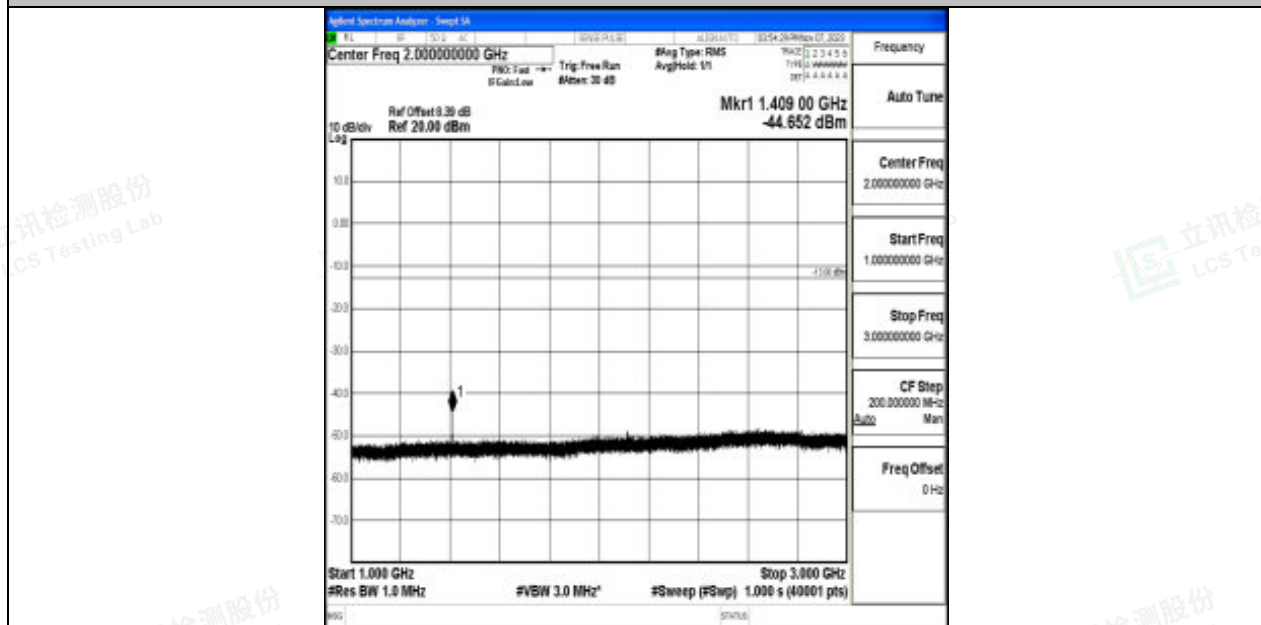
Band17_10MHz_QPSK_23780_1RB#0_1000~3000_1000~3000
