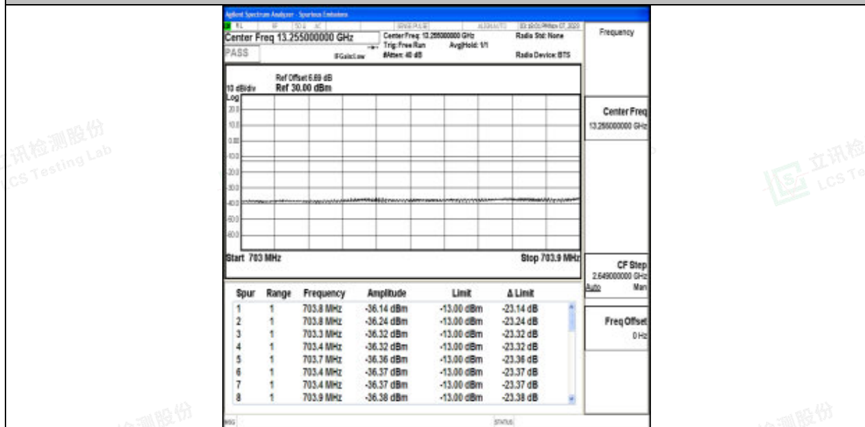
Band17_5MHz_16QAM_23755_25RB#0
