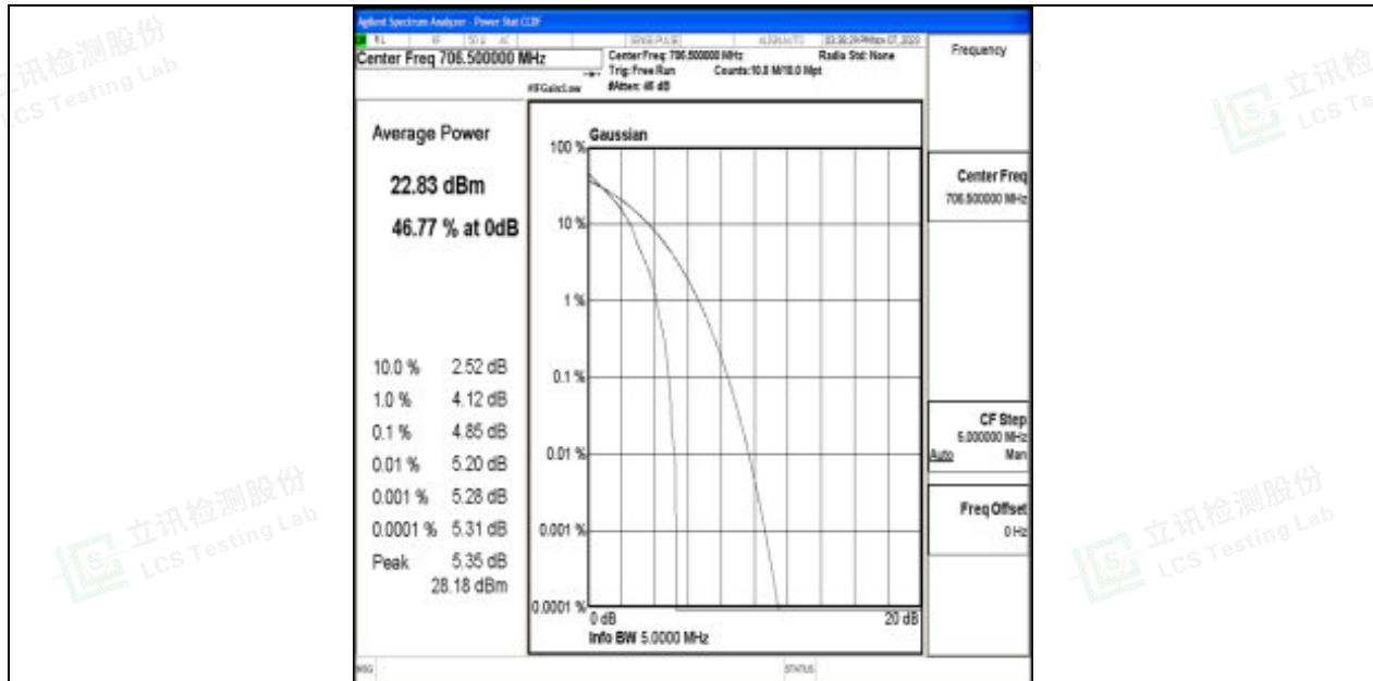
Band17-5MHz-64QAM-23755-1RB#0-PASS
