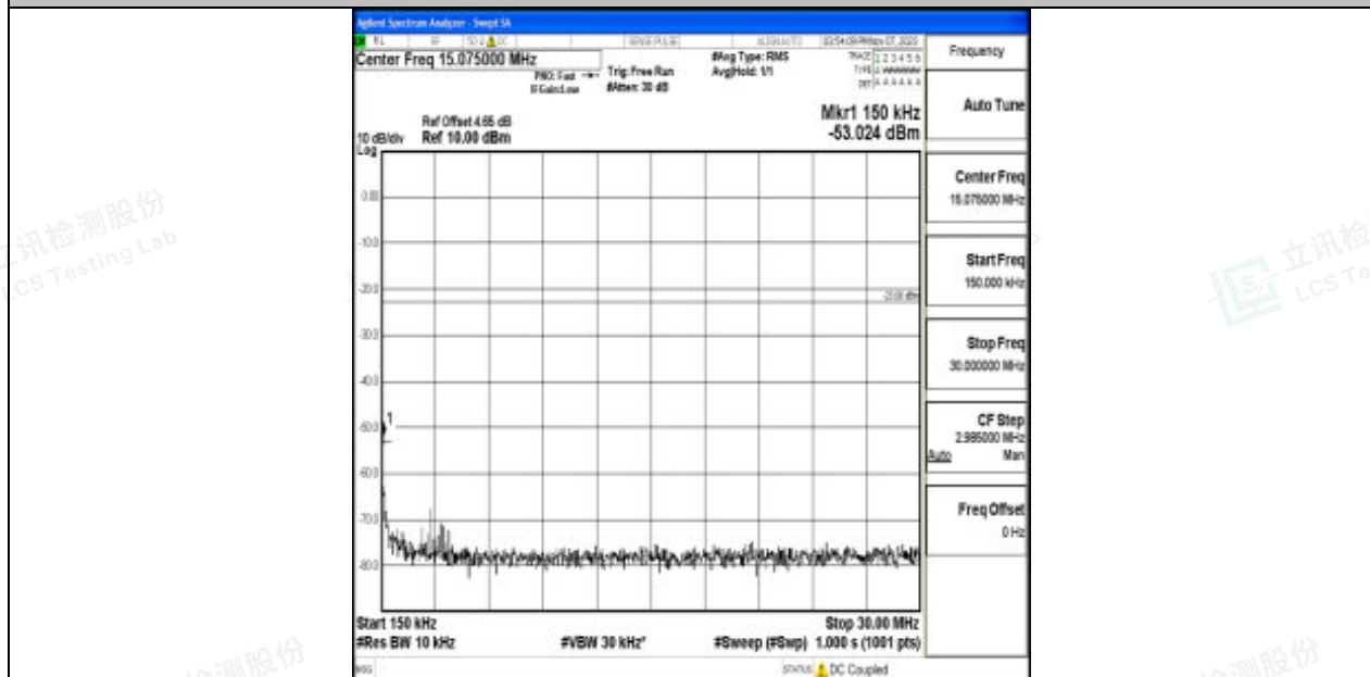
Band17_10MHz_QPSK_23780_1RB#0_0.15~30_0.15~30
