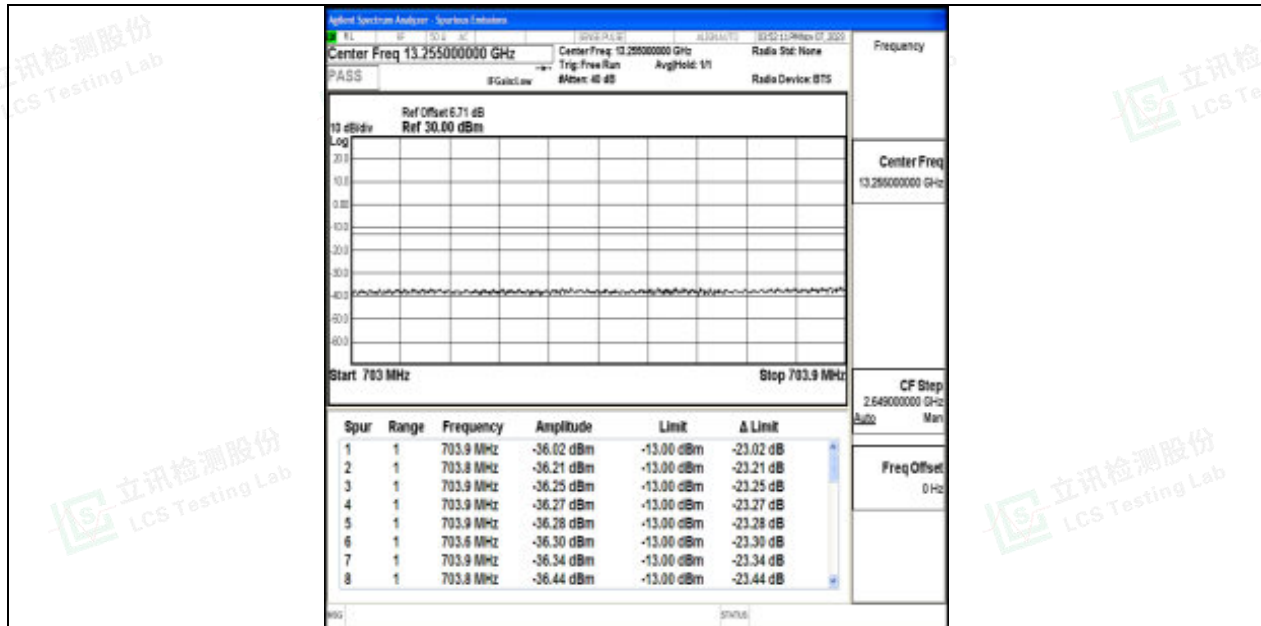
Band17_10MHz_64QAM_23780_50RB#0
