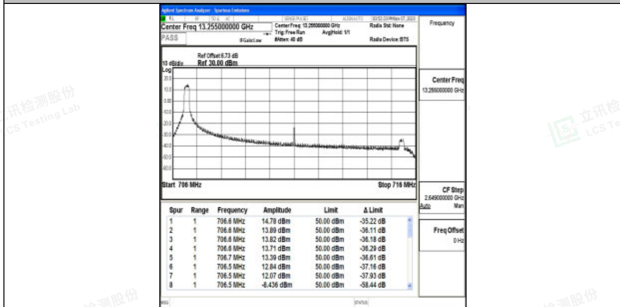
Band17_10MHz_QPSK_23800_1RB#0
