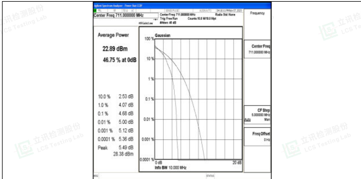
Band17-10MHz-64QAM-23800-1RB#0-PASS
