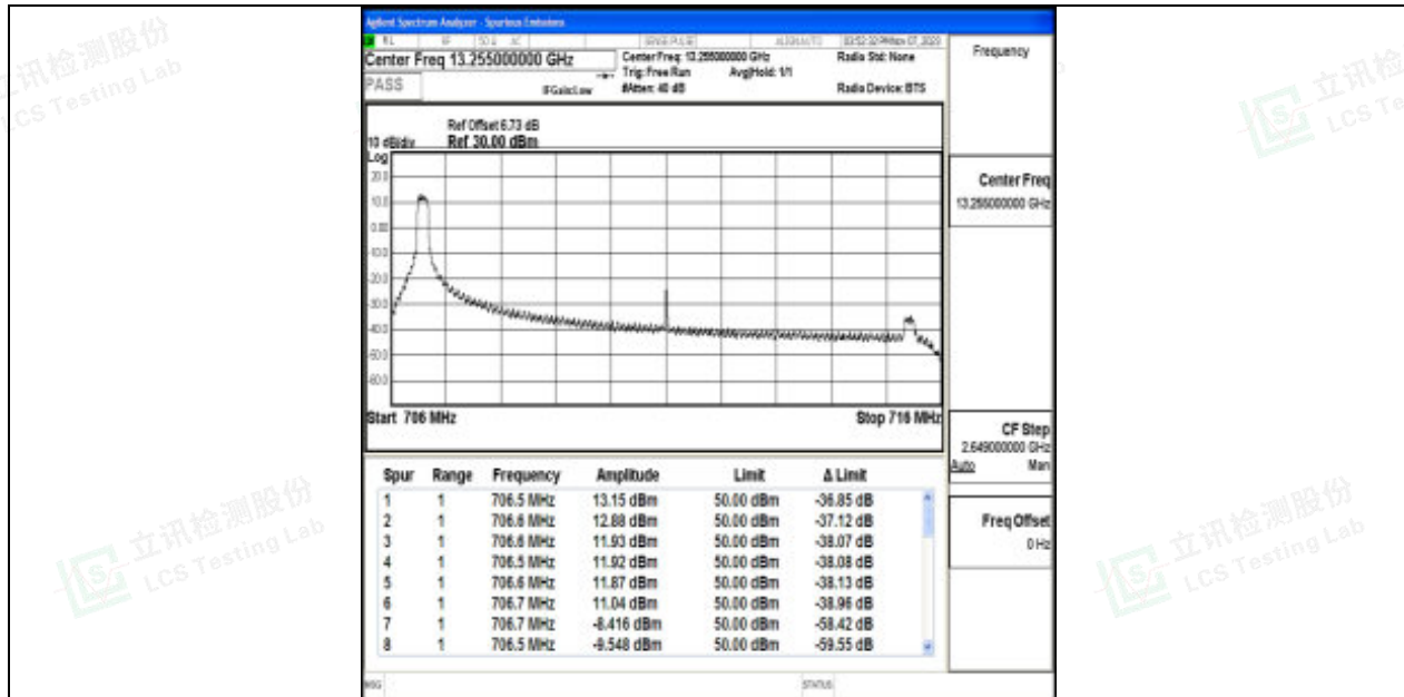
Band17_10MHz_16QAM_23800_1RB#0
