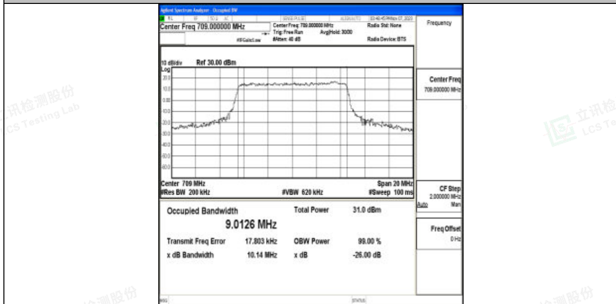
Band17-10MHz-QPSK-23780-50RB#0-PASS
