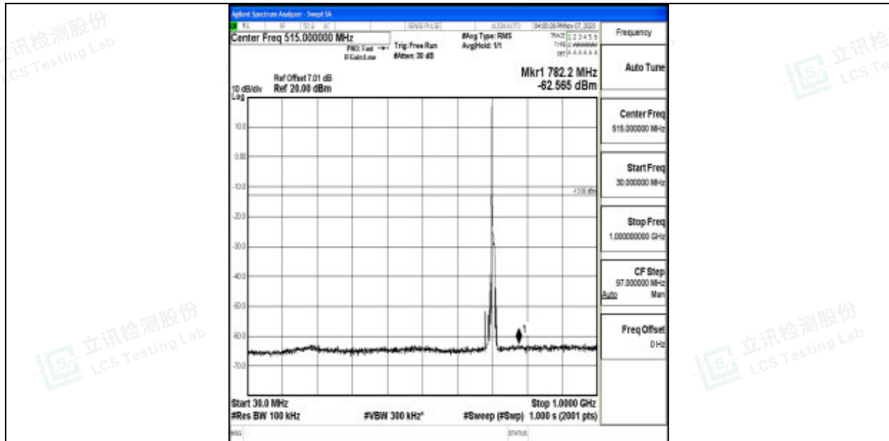
Band17_10MHz_64QAM_23800_1RB#0_30~1000_30~1000
