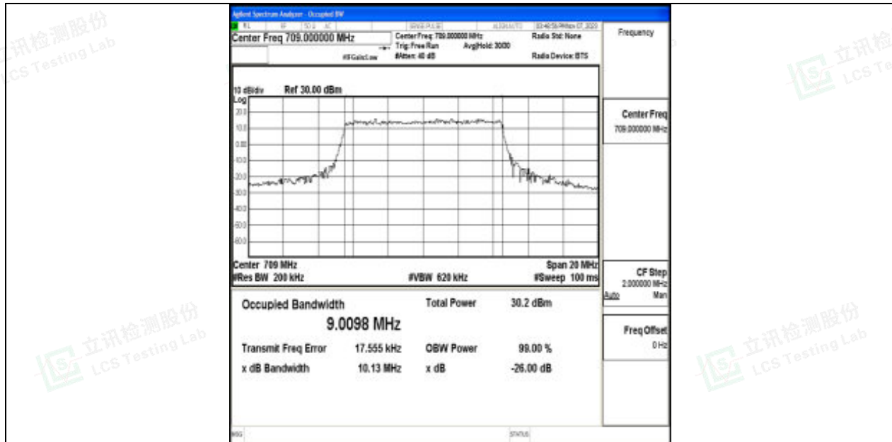
Band17-10MHz-16QAM-23780-50RB#0-PASS
