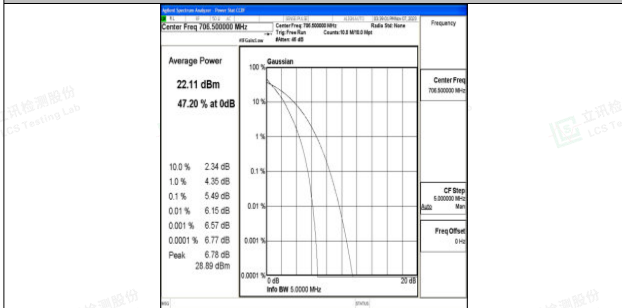
Band17-5MHz-QPSK-23755-25RB#0-PASS
