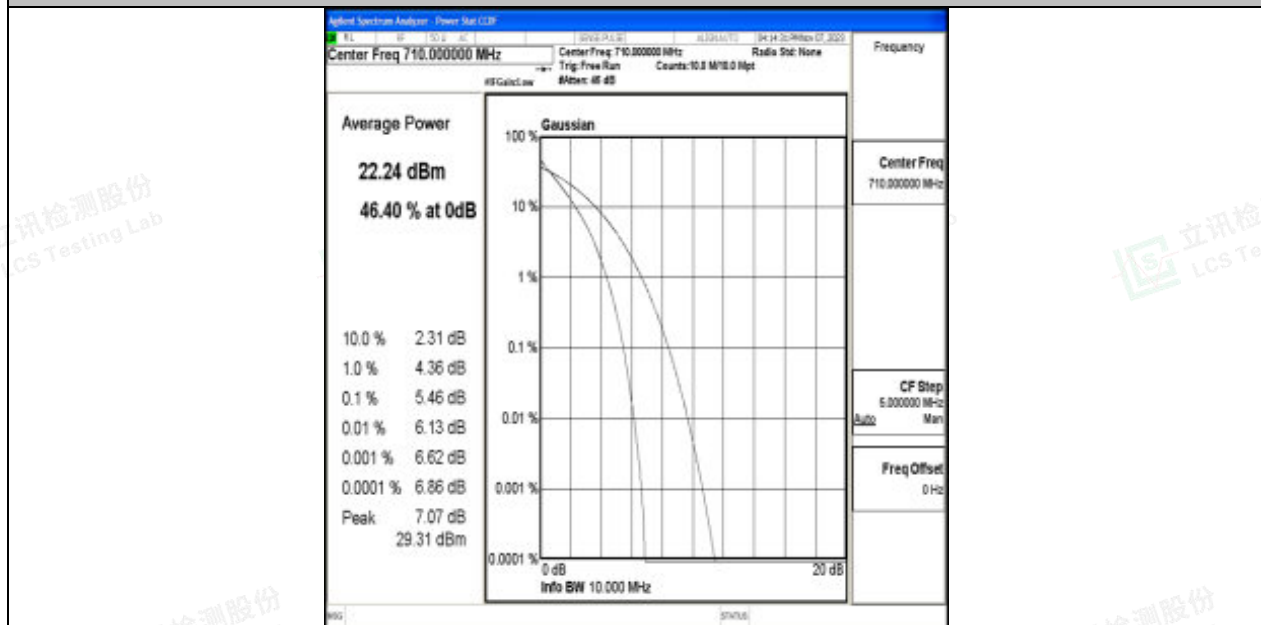
Band17-10MHz-QPSK-23790-50RB#0-PASS
