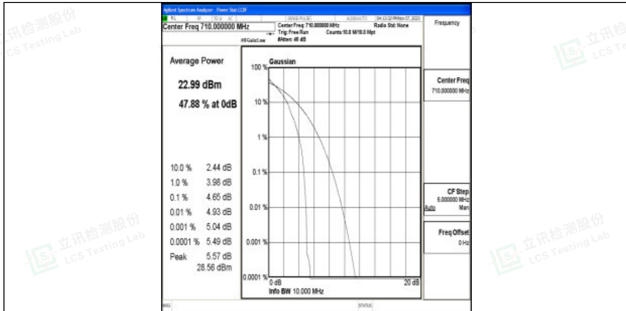
Band17-10MHz-QPSK-23790-1RB#0-PASS
