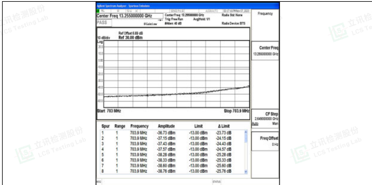
Band17_5MHz_64QAM_23755_1RB#0
