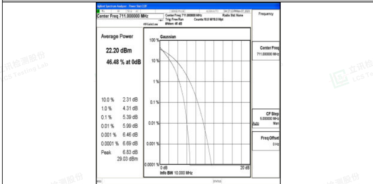
Band17-10MHz-64QAM-23800-50RB#0-PASS
