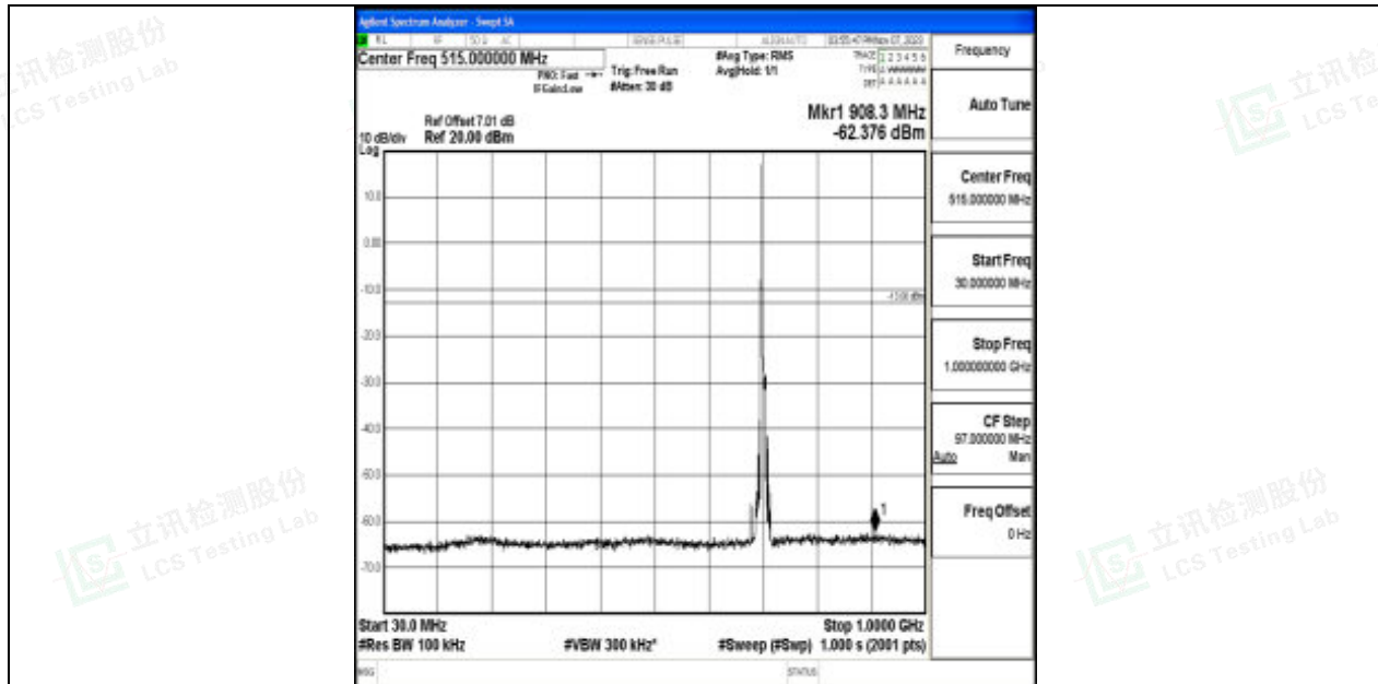
Band17_10MHz_64QAM_23780_1RB#0_30~1000_30~1000
