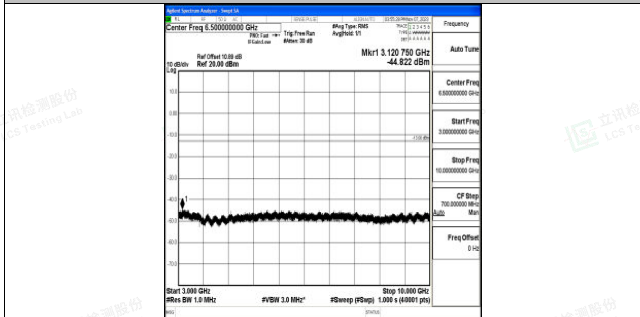
Band17_10MHz_16QAM_23780_1RB#0_3000~10000_3000~10000
