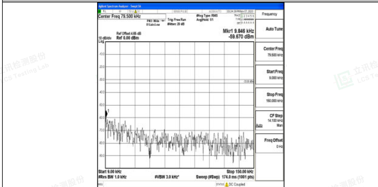
Band17_5MHz_QPSK_23825_1RB#0_0.009~0.15_0.009~0.15
