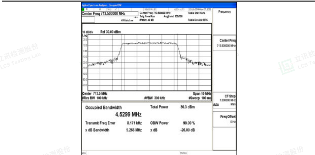
Band17-5MHz-16QAM-23825-25RB#0-PASS
