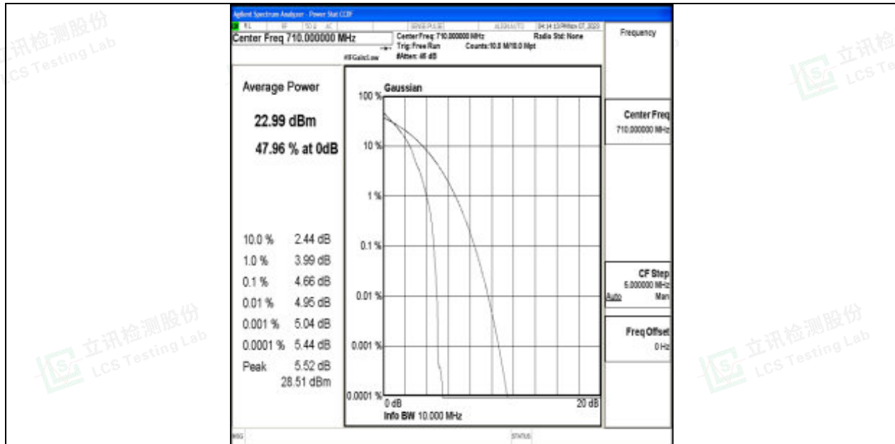
Band17-10MHz-64QAM-23790-1RB#0-PASS
