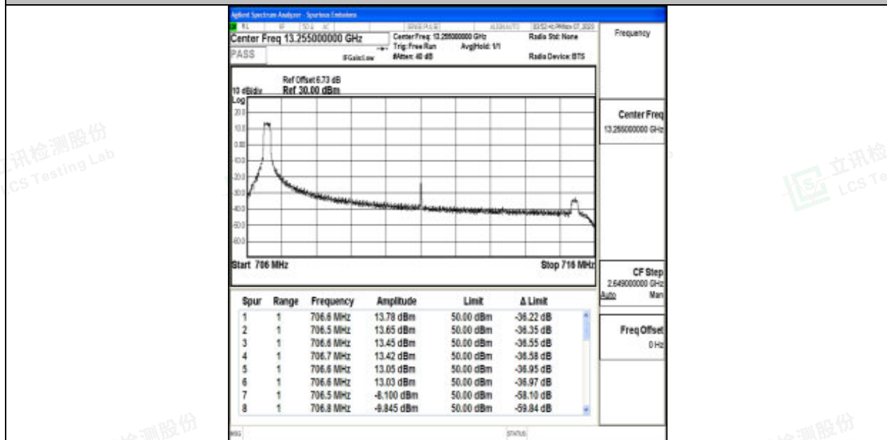
Band17_10MHz_64QAM_23800_1RB#0
