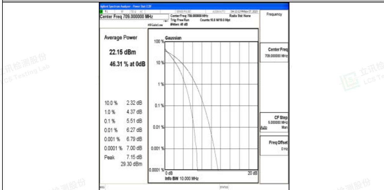
Band17-10MHz-64QAM-23780-50RB#0-PASS
