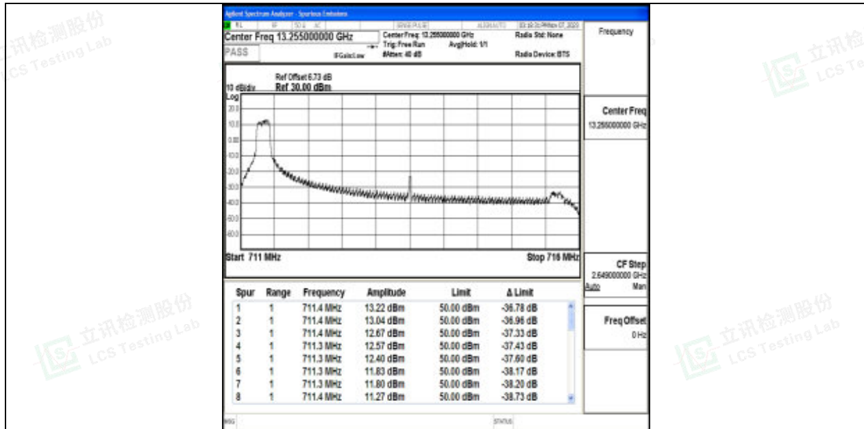
Band17_5MHz_16QAM_23825_1RB#0
