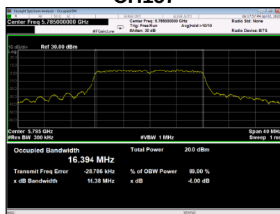
99% Emission Bandwidth CH149 CH157
