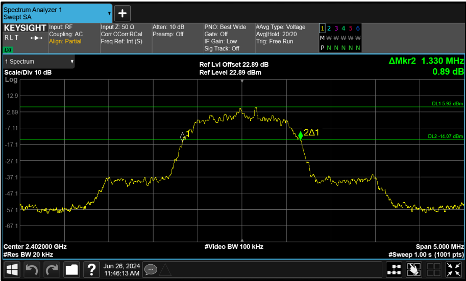
Figure 155 - Core 1 (B) 2402 MHz (CH0) 20 dB Bandwidth
