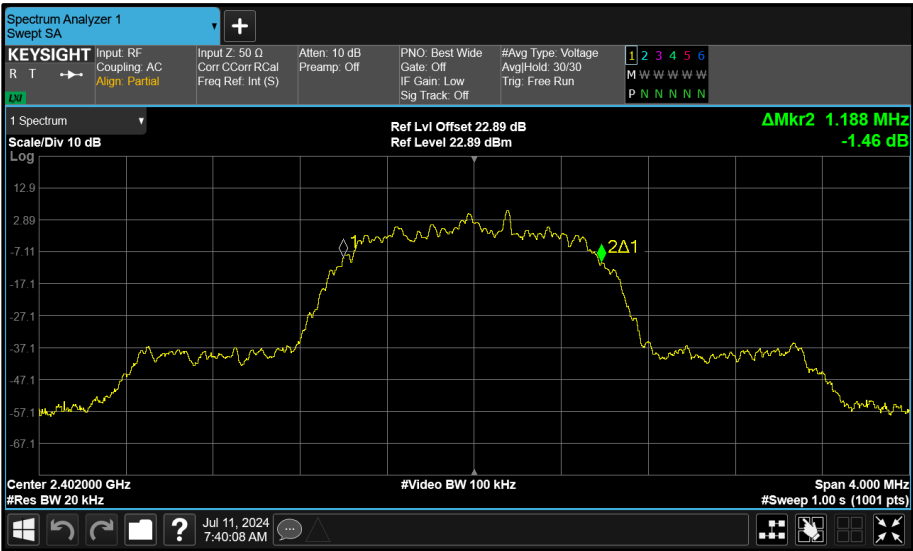
Figure 156 - Core 1 (B) 2402 MHz (CH0) 99% Bandwidth
