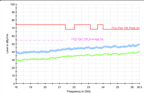
Radiated Spurious Emission (802.11ax 20M-MIMO, ch100, 18GHz-26.5GHz)
