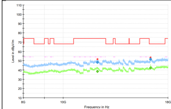
Radiated Spurious Emission (802.11ax 20M-MIMO, ch100, 8GHz-18GHz)
