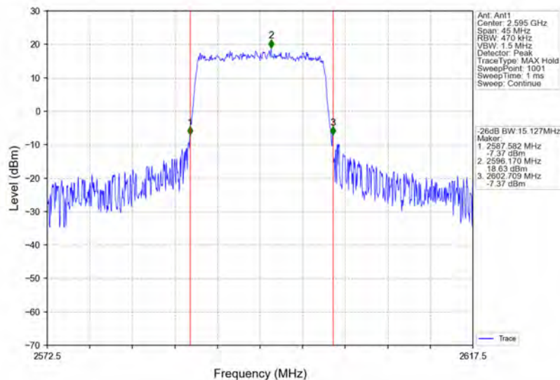
Band38_15MHz_QPSK_MCH_2595MHz_RB_75_0_NTNV
