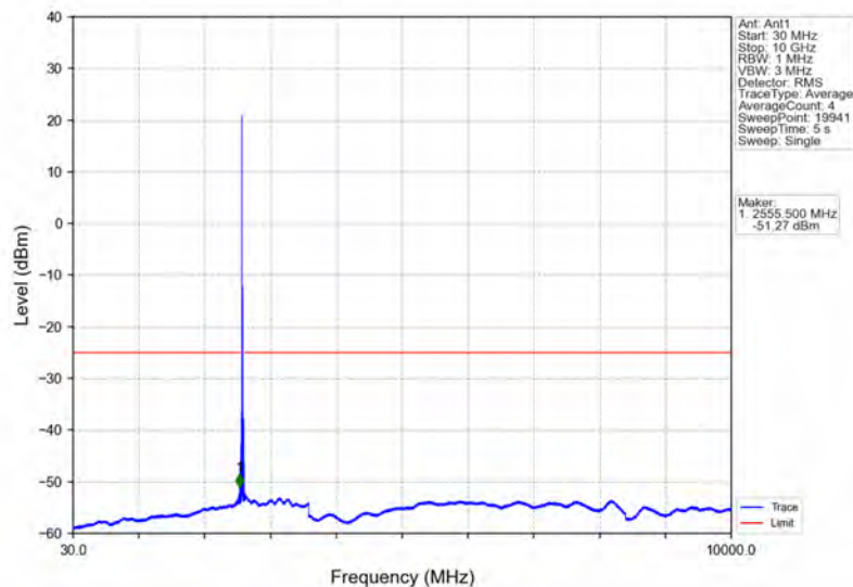
Band38_15MHz_QPSK_MCH_2595MHz_RB_1_0_NTNV
