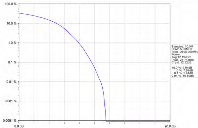
Band38_20MHz_64QAM_MCH_2595MHz_RB_100_0_NTNV
