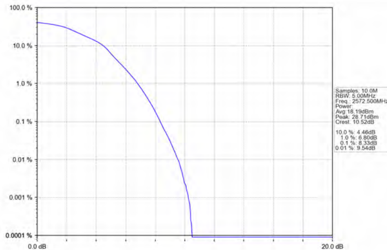
Band38_5MHz_16QAM_LCH_2572.5MHz_RB_25_0_NTNV
