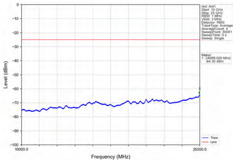
Band38_20MHz_64QAM_HCH_2610MHz_RB_1_0_NTNV
