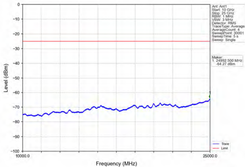
Band38_15MHz_64QAM_MCH_2595MHz_RB_1_0_NTNV
