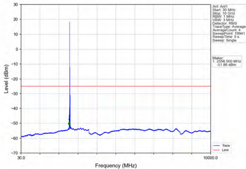
Band38_15MHz_16QAM_MCH_2595MHz_RB_1_0_NTNV
