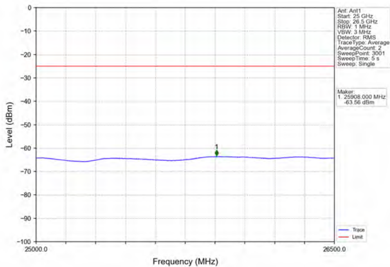
Band38_5MHz_64QAM_LCH_2572.5MHz_RB_1_0_NTNV
