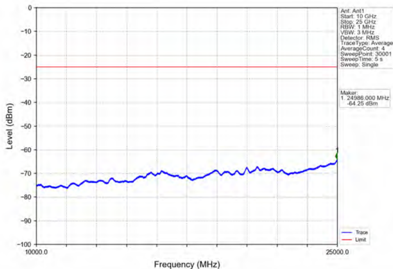
Band38_15MHz_QPSK_HCH_2612.5MHz_RB_1_0_NTNV
