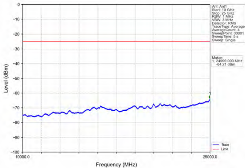
Band38_10MHz_64QAM_LCH_2575MHz_RB_1_0_NTNV
