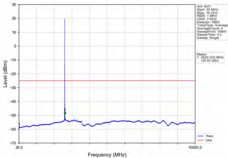
Band38_5MHz_16QAM_HCH_2617.5MHz_RB_1_0_NTNV
