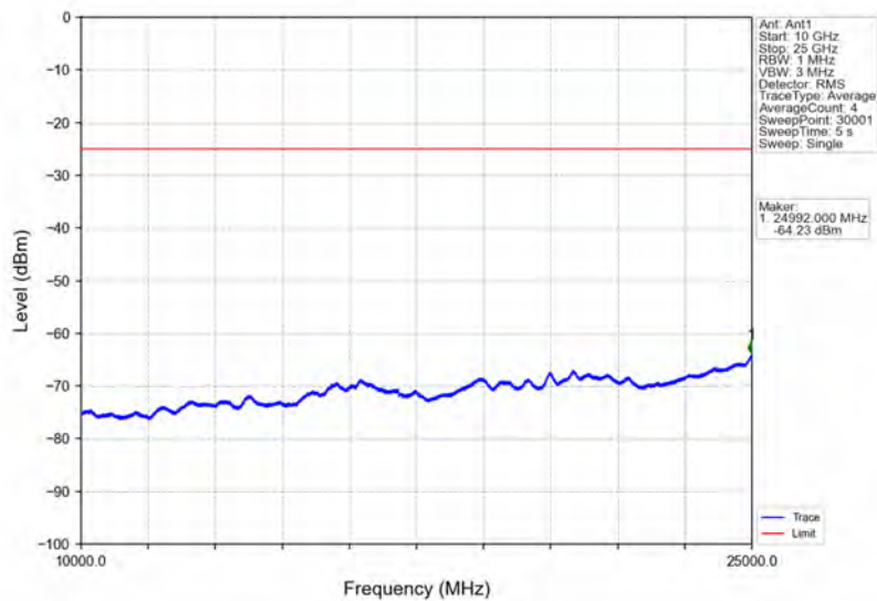
Band38_15MHz_16QAM_LCH_2577.5MHz_RB_1_0_NTNV
