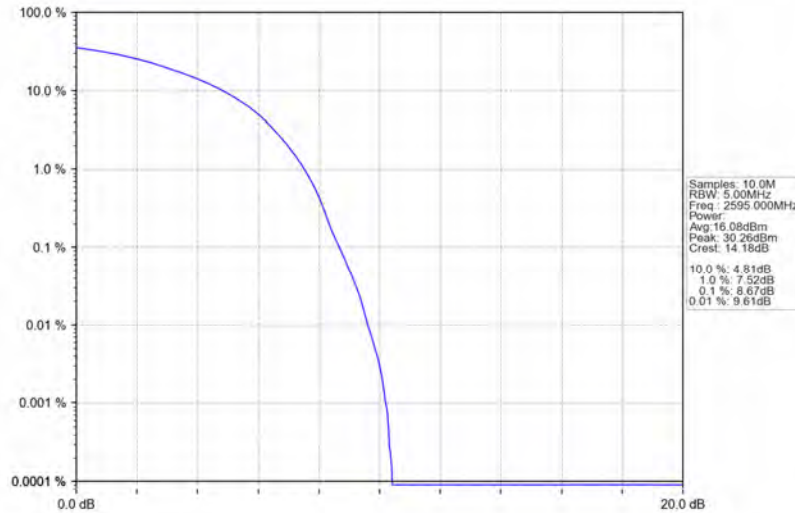
Band38_10MHz_16QAM_MCH_2595MHz_RB_50_0_NTNV
