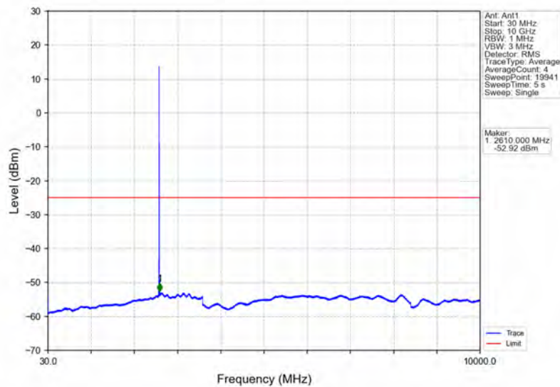
Band38_5MHz_64QAM_MCH_2595MHz_RB_1_0_NTNV
