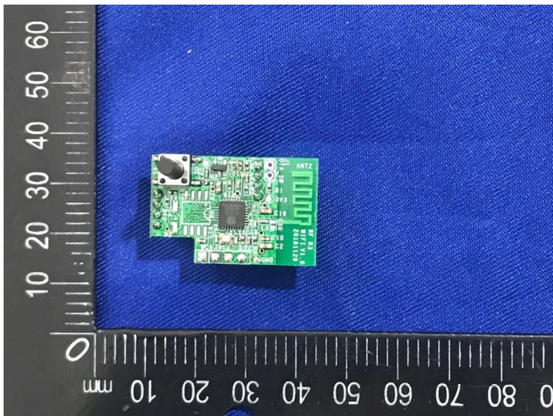
Wi-Fi Chip
