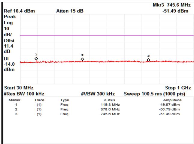
Channel Frequency 2402MHz Frequency Range 30 MHz – 1GHz
