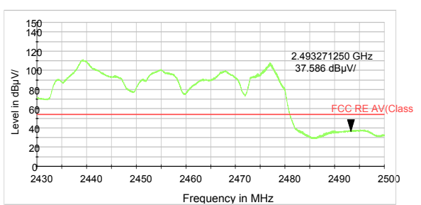
802.11n HT40 -Channel 9 Average
