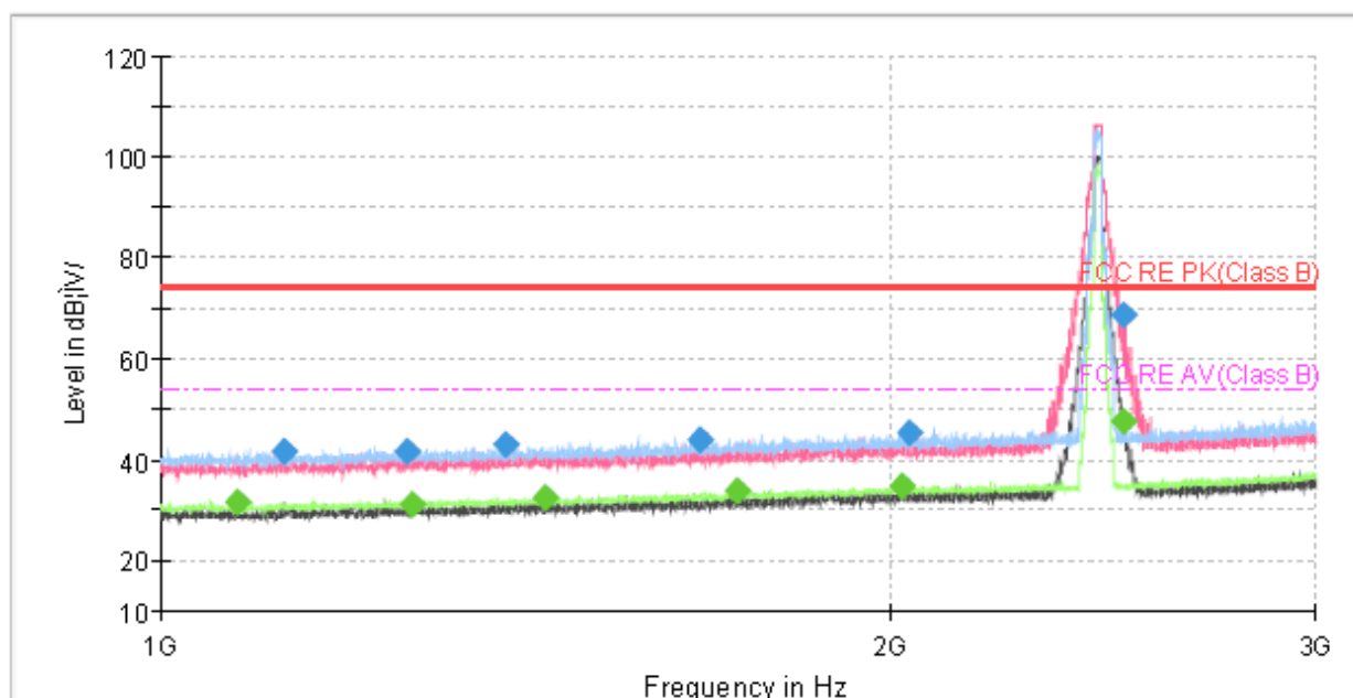
Radiates Emission from 1GHz to 3GHz Note: The signal beyond the limit is carrier.
