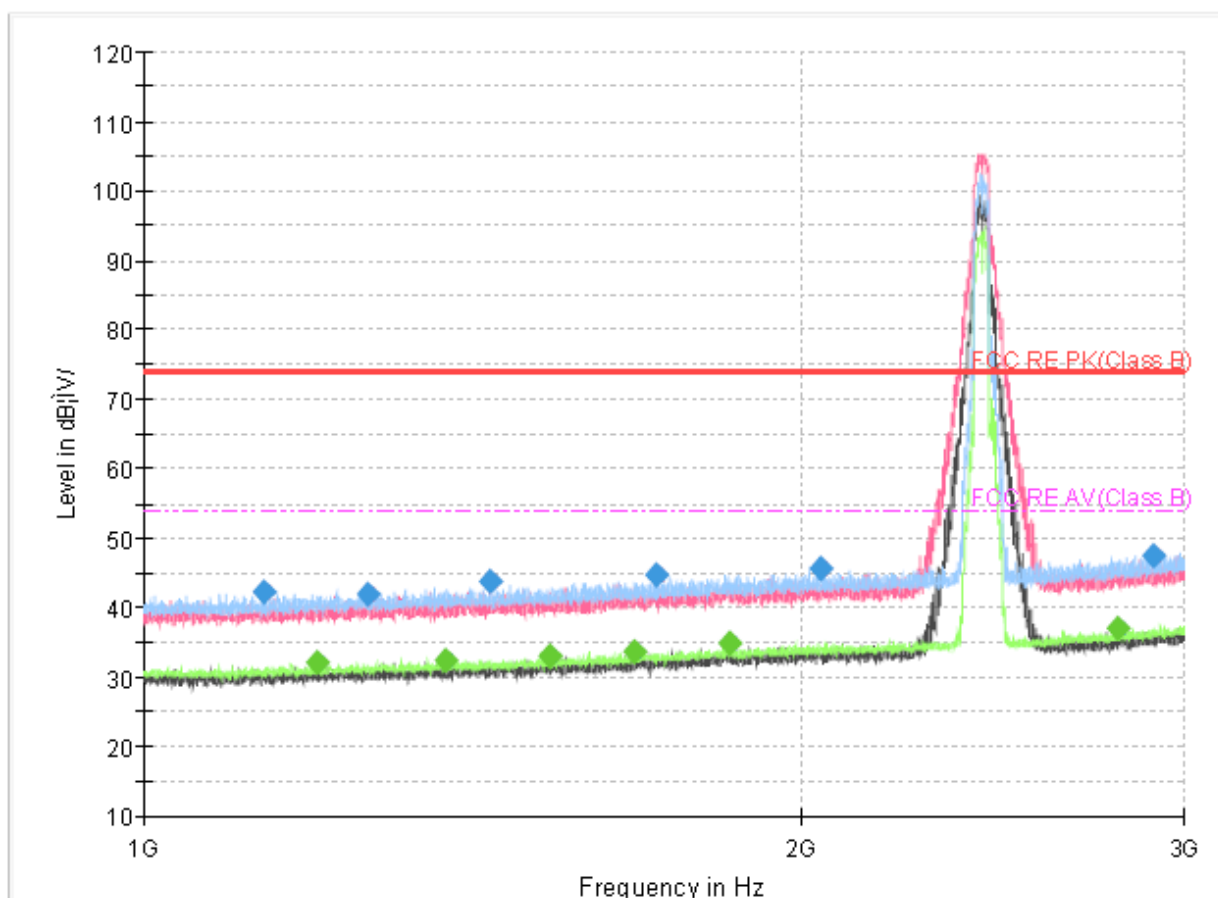
Radiates Emission from 1GHz to 3GHz Note: The signal beyond the limit is carrier.
