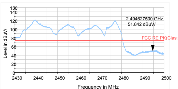
802.11n HT40 -Channel 9 Peak
