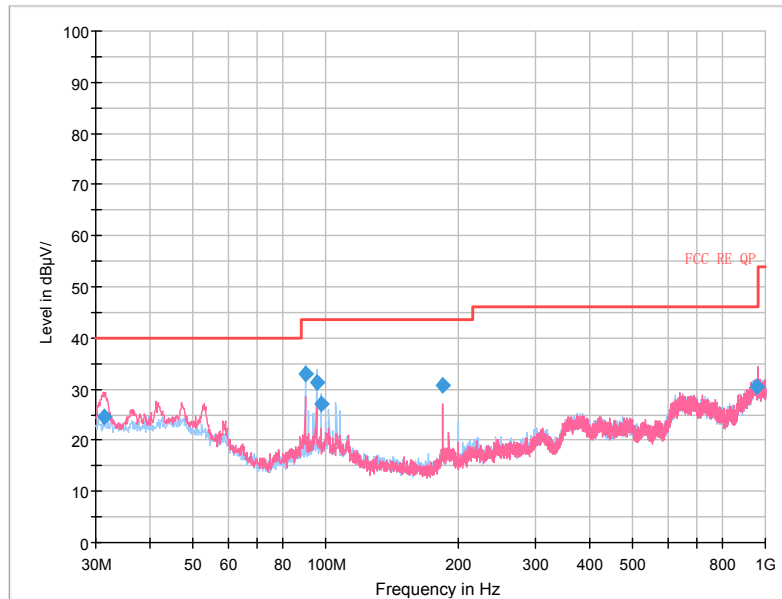
Radiates Emission from 30MHz to 1GHz
