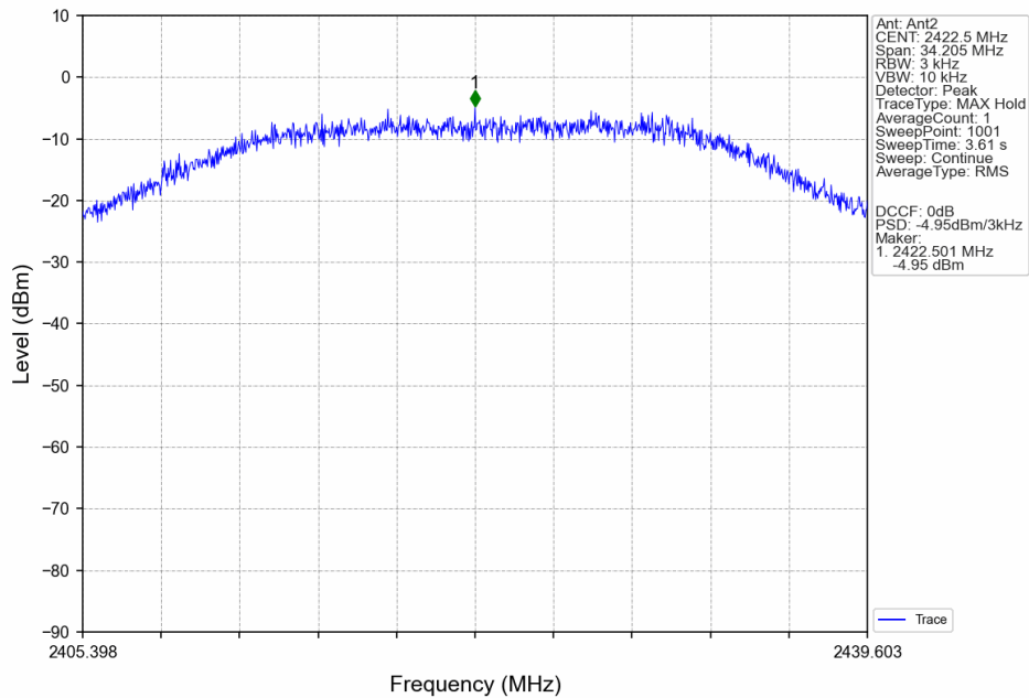
40M_LCH_2422.5MHz_Ant2_NTNV
