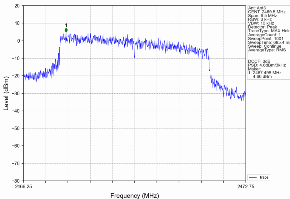
5M_HCH_2469.5MHz_Ant3_NTNV
