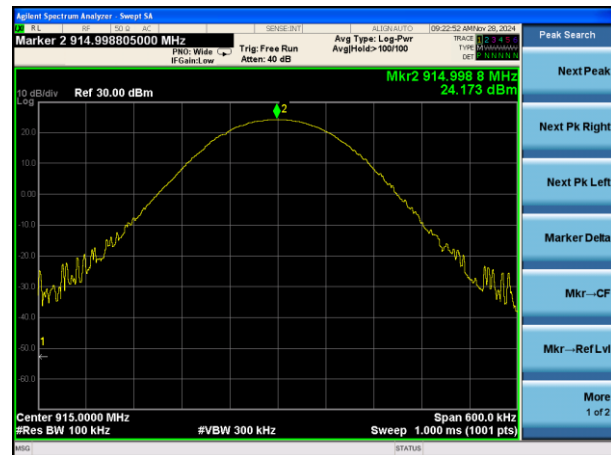
Peak output Power plot on channel 31 (1Mbps)
