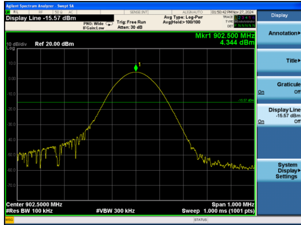
GFSK on channel 06
