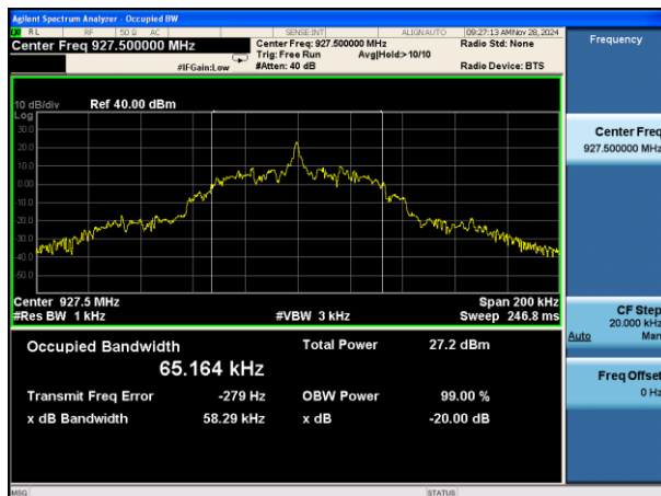
20dB Bandwidth plot on channel 56 (1Mbps)
