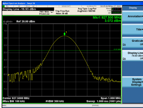
GFSK on channel 56
