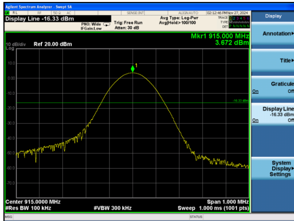
GFSK on channel 31
