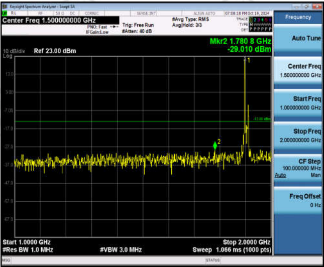
Band25-20MHz-16QAM-26590-1RB#0-Range2:1000~2000MHz
