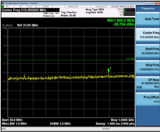
Band25-15MHz-QPSK-26615-1RB#0-Range1:30~1000MHz
