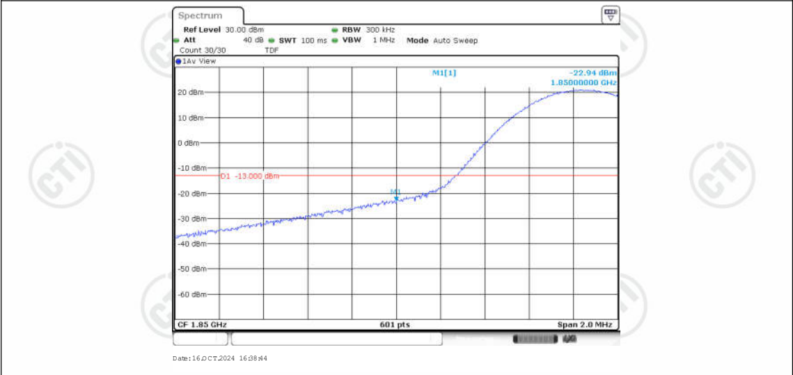
Band25-15MHz-QPSK-26115-1RB#0
