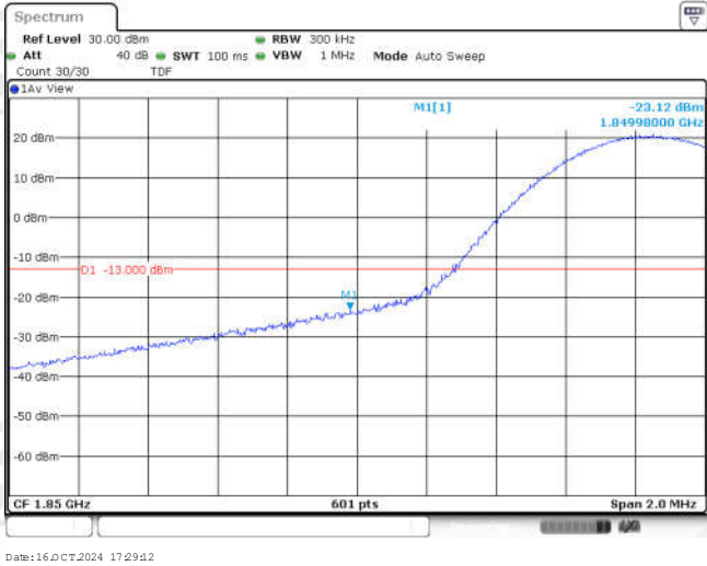
Band25-15MHz-16QAM-26115-1RB#0
