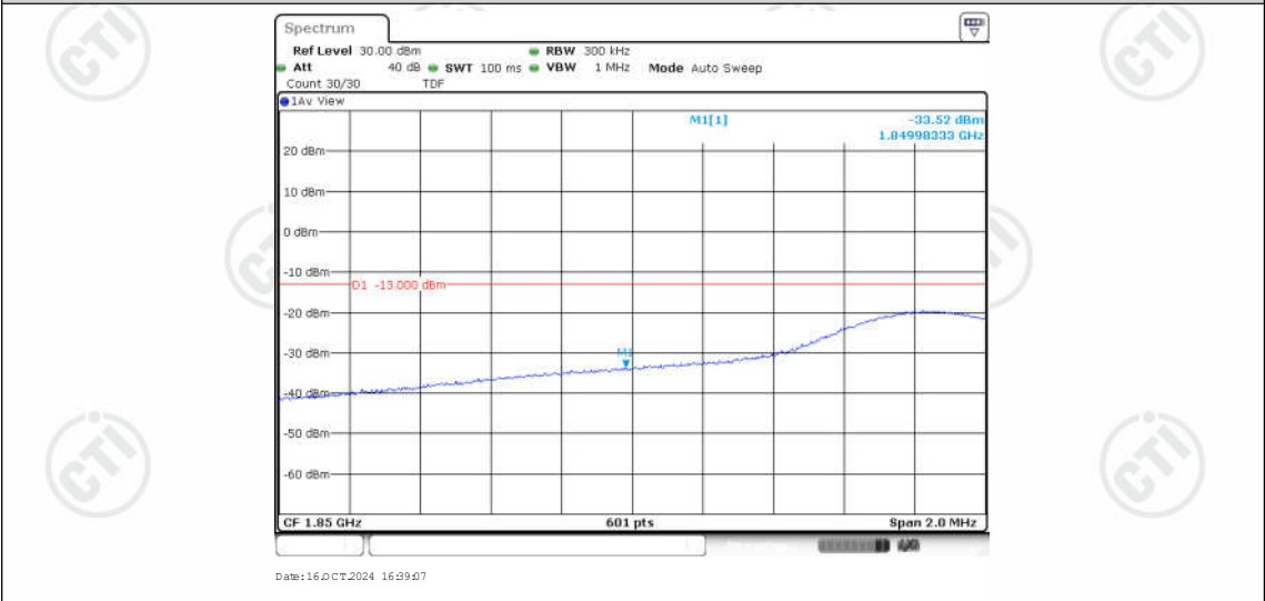
Band25-15MHz-QPSK-26115-1RB#74
