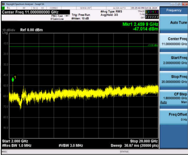
Band25-15MHz-QPSK-26365-1RB#0-Range3:2000~20000MHz
