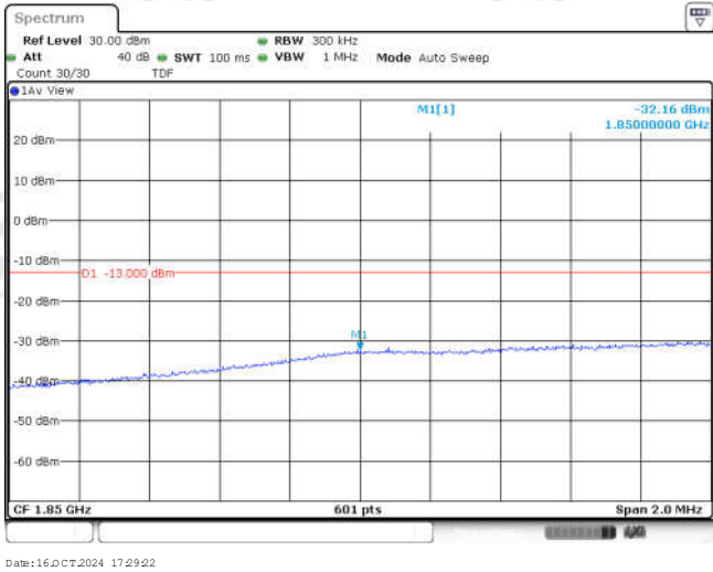
Band25-15MHz-16QAM-26115-1RB#24
