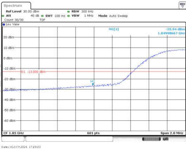
Band25-15MHz-16QAM-26115-25RB#0
