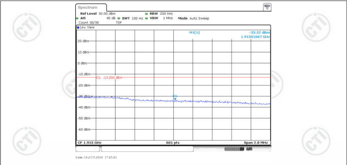
Band25-10MHz-16QAM-26640-25RB#0
