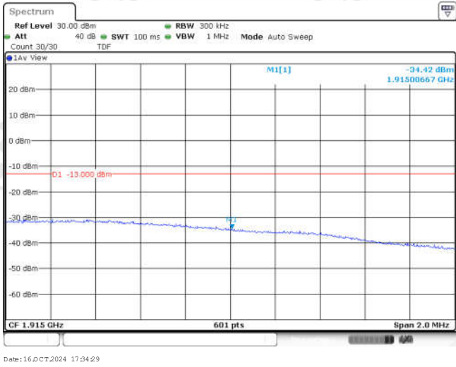
Band25-15MHz-16QAM-26615-1RB#24
