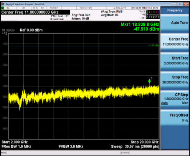
Band25-20MHz-16QAM-26365-1RB#0-Range3:2000~20000MHz
