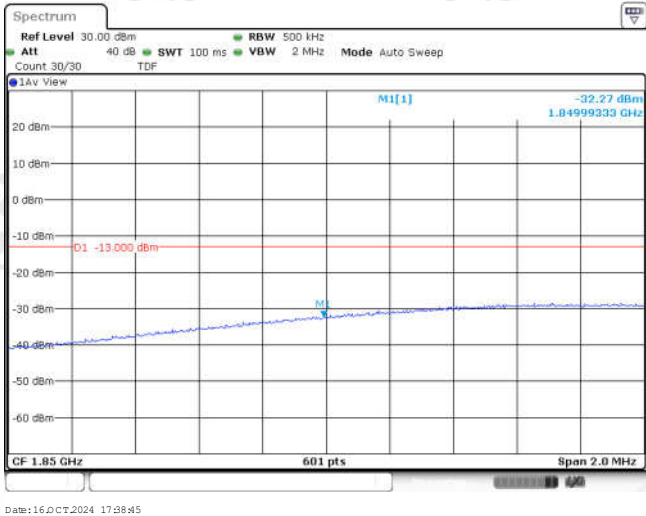
Band25-20MHz-16QAM-26140-1RB#24
