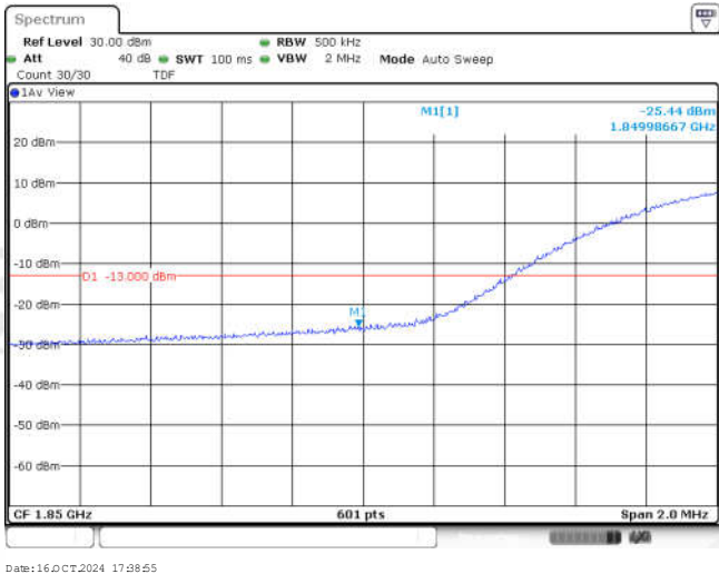
Band25-20MHz-16QAM-26140-25RB#0
