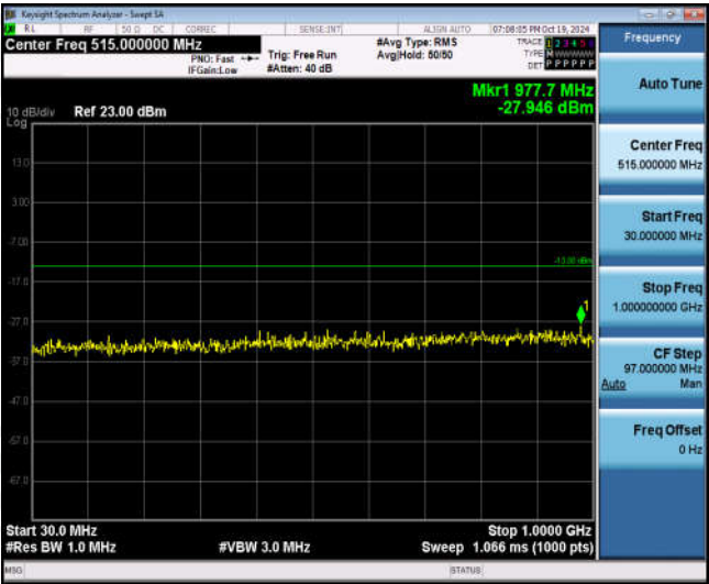
Band25-20MHz-16QAM-26590-1RB#0-Range1:30~1000MHz
