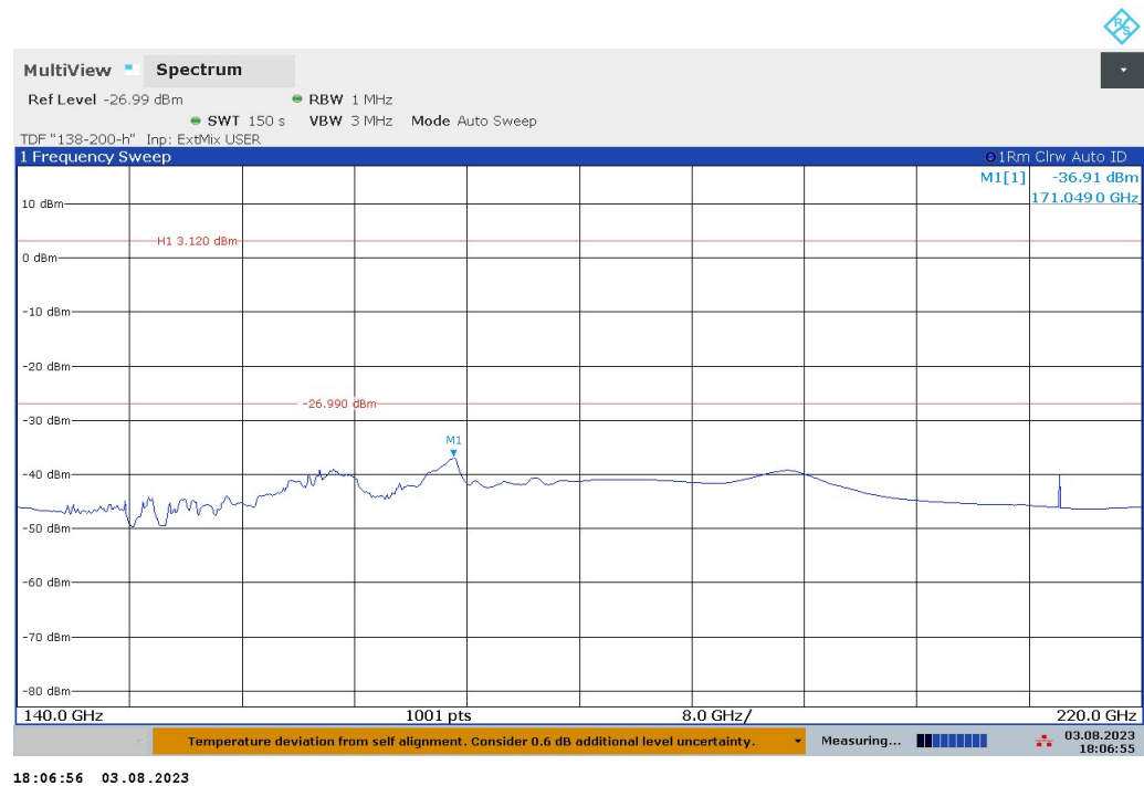
Plots No. 17: Radiated Emission, 140 GHz to 220 GHz, Horizontal / Vertical Polarization
