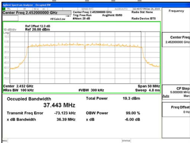
OBW 6dB_802.11ax_40MHz_Chain0_2452MHz
