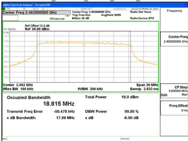
OBW 6dB_802.11ax_20MHz_Chain0_2462MHz
