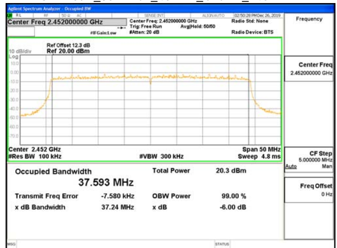
OBW 6dB_802.11ax_40MHz_Chain1_2452MHz
