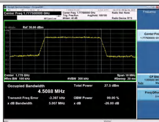
Band66-5MHz-16QAM-132647-25RB#0-PASS
