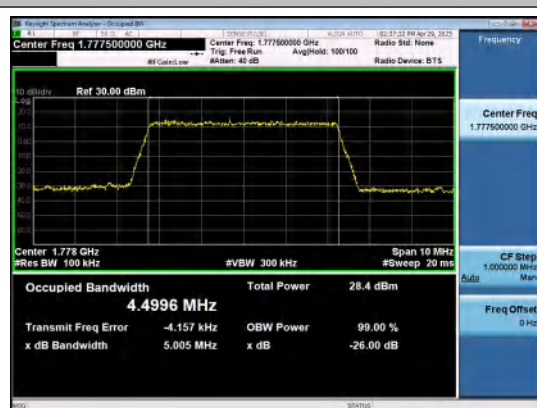
Band66-5MHz-QPSK-132647-25RB#0-PASS
