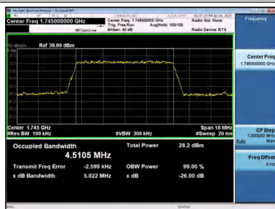
Band66-5MHz-QPSK-132322-25RB#0-PASS
