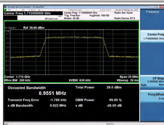
Band66-10MHz-QPSK-132022-50RB#0-PASS
