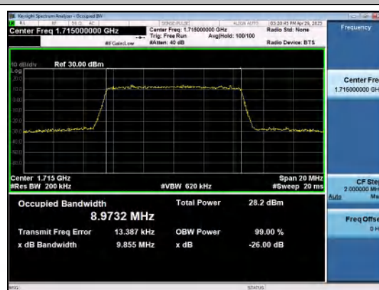
Band66-10MHz-16QAM-132022-50RB#0-PASS
