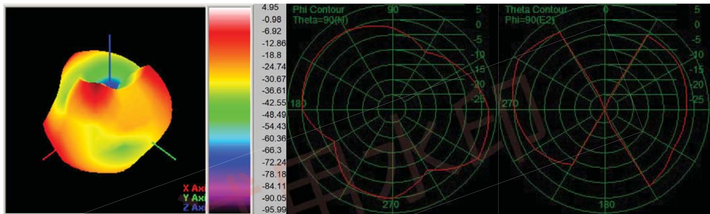
Passive -Freq5760.00MHZ
