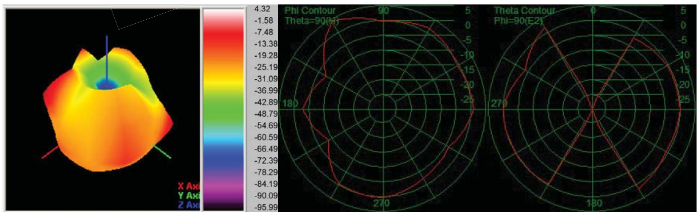
Passive -Freq5880.00MHZ
