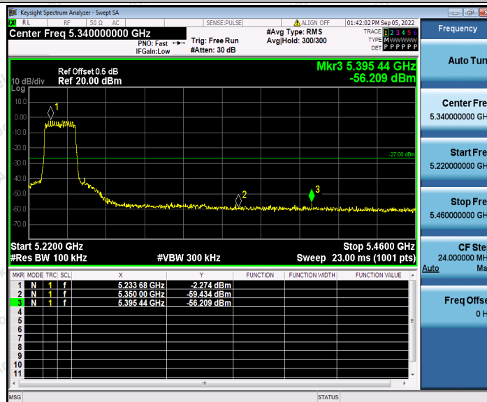
11AX20SISO_Ant2_High_5240
