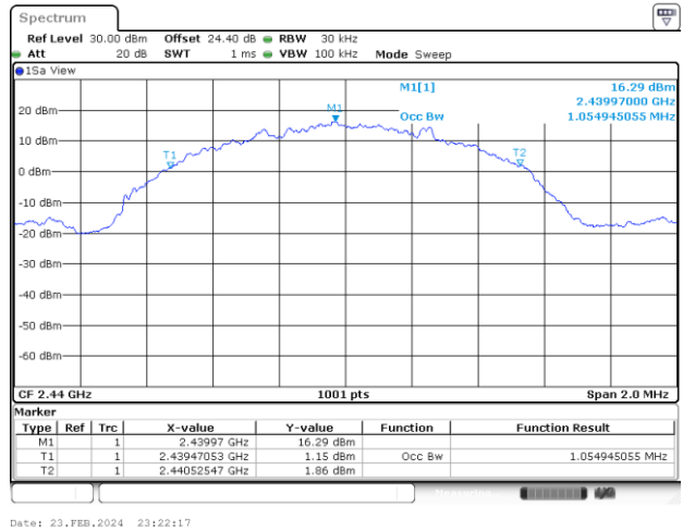
99% Occupied Plot Bandwidth on Channel 38
