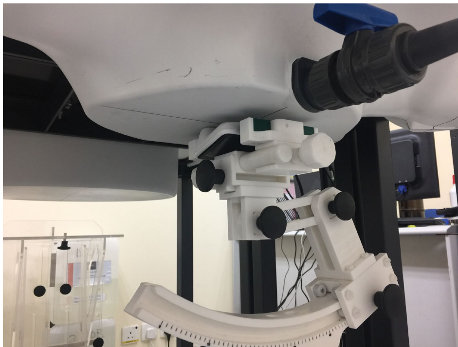
Figure 3 – Back with 0mm Separation
