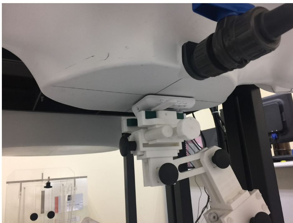
Figure 4 – Front with 0mm Separation (antenna extended)
