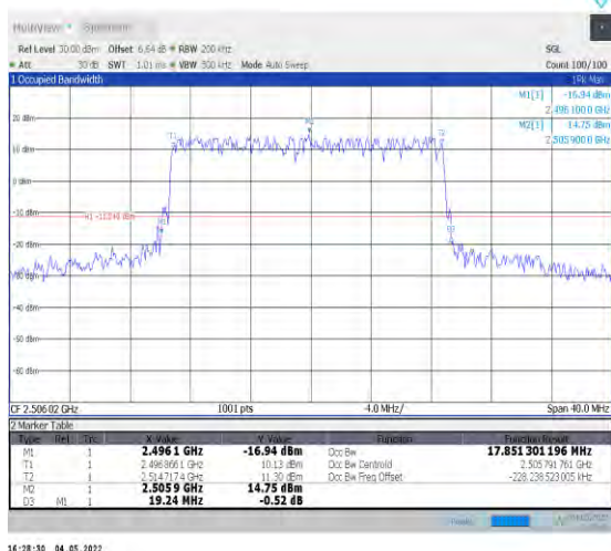
1-N41--30-20-L-3-DFT-16QAM-Outet_Full-50@0-Ant 1-17.851-19.240-≤20-PASS
