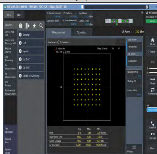
1-N41--30-100-M-8-CP-64QAM-Outer_Full-273@0- Ant1-see graph-PASS
