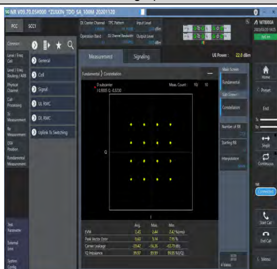
1-N41-30-100-M-7-CP-16QAM-Outer_Full-273@0-An t1-see graph-PASS
