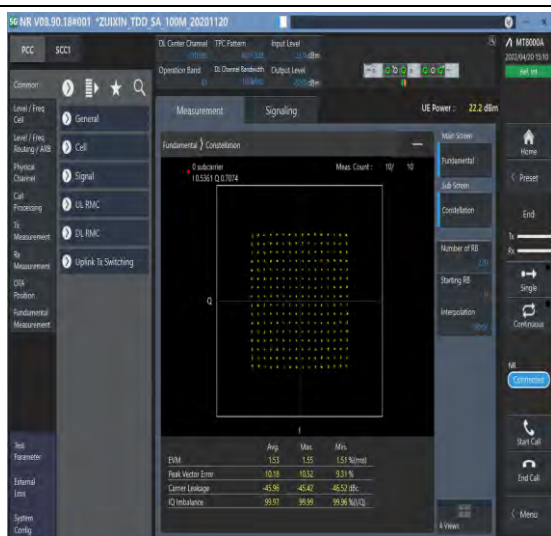
1-N41--30-100-M-5-DFT-256QAM-Outer_Full-270@0 -Ant1-see graph-PASS
