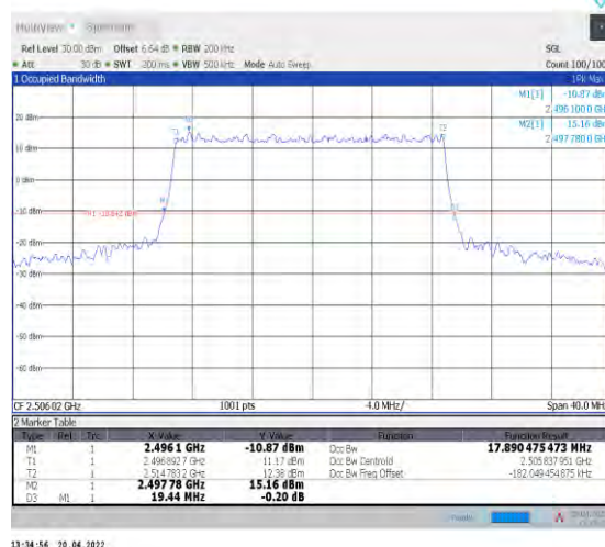
1-N41--30-20-L-4-DFT-64QAM-Outet_Full-50@0-Ant t1-17.89-19.440-≤20-PASS
