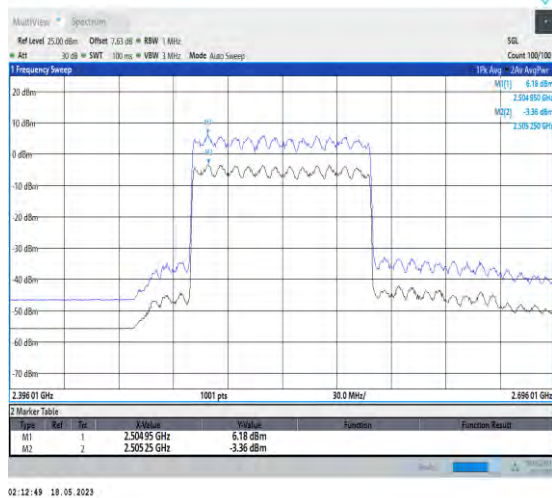
1-N41-PC1-30-100-L-1-DFT-256QAM-Outer_Full-270@0-Ant1-9.54-19.56%-7.09-2.45-PASS-≤13
