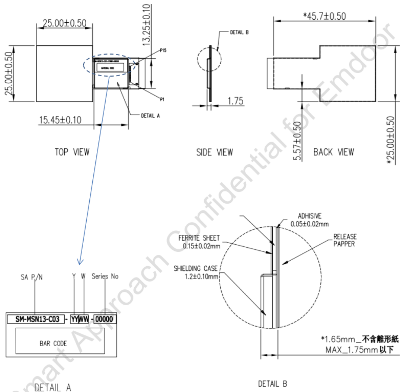
Figure 8 Antenna Module Drawing
