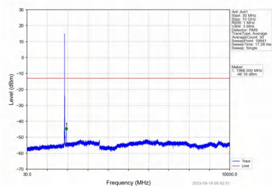
Band2_15MHz_16QAM_MCH_1880MHz_RB_1_0_NTNV
