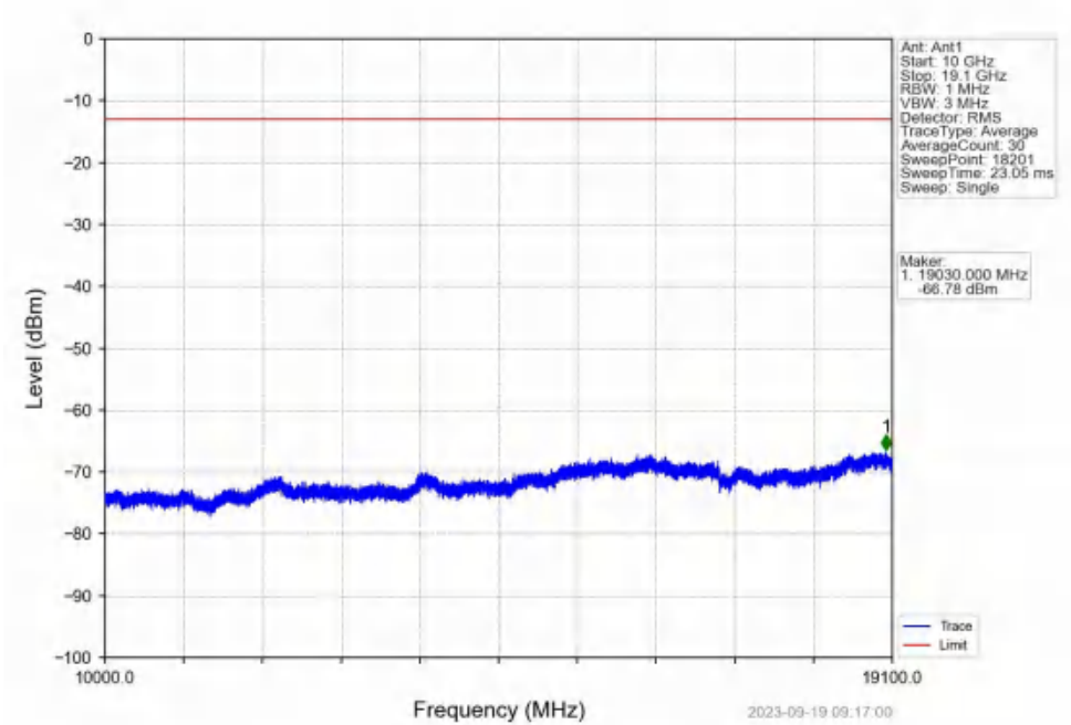
Band2_1.4MHz_16QAM_MCH_1880MHz_RB_1_0_NTNV
