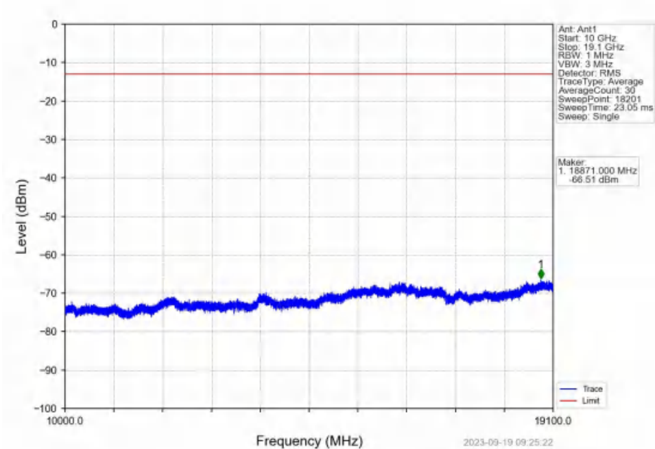
Band2_5MHz_16QAM_MCH_1880MHz_RB_1_0_NTNV
