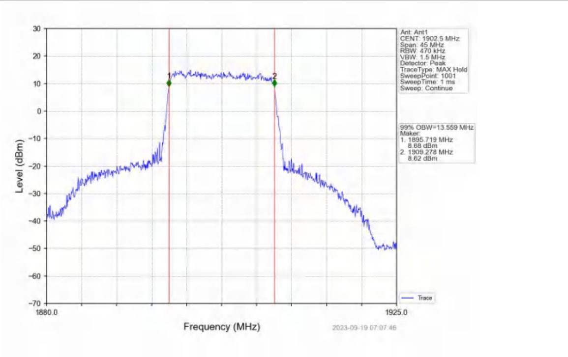
Band2_15MHz_16QAM_HCH_1902.5MHz_RB_75_0_NTNV
