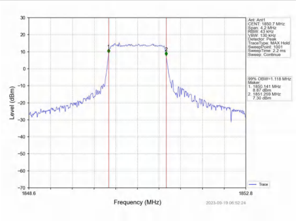
Band2_1.4MHz_16QAM_LCH_1850.7MHz_RB_6_0_NTNV
