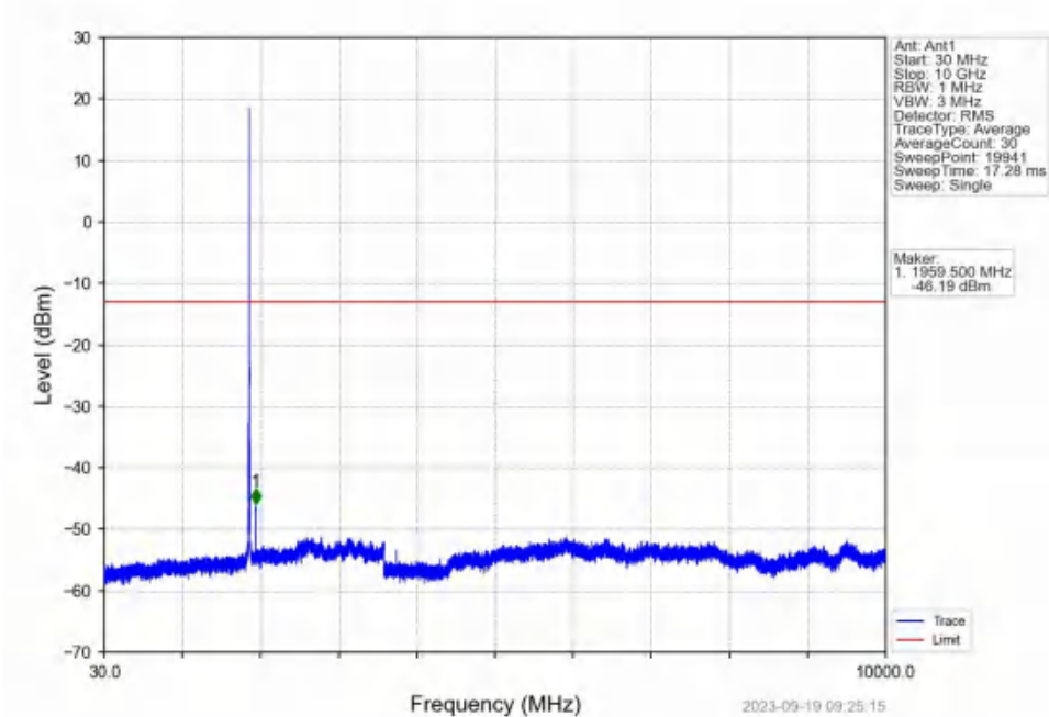
Band2_5MHz_16QAM_MCH_1880MHz_RB_1_0_NTNV
